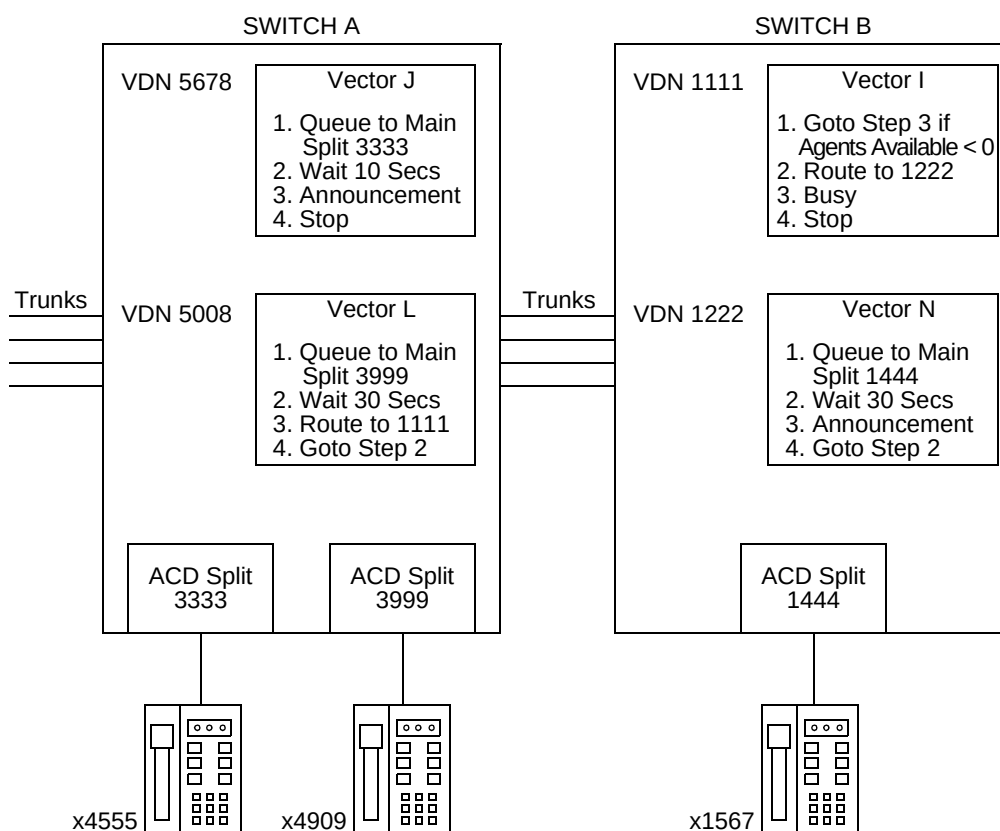
Figure A-1. Multiple Switch Configuration
