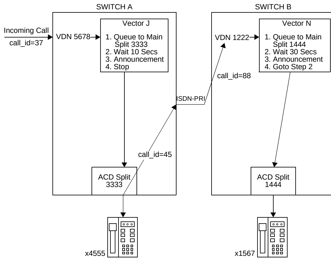
Figure A-2. Call Flow for Blind Transfer to Another Switch
