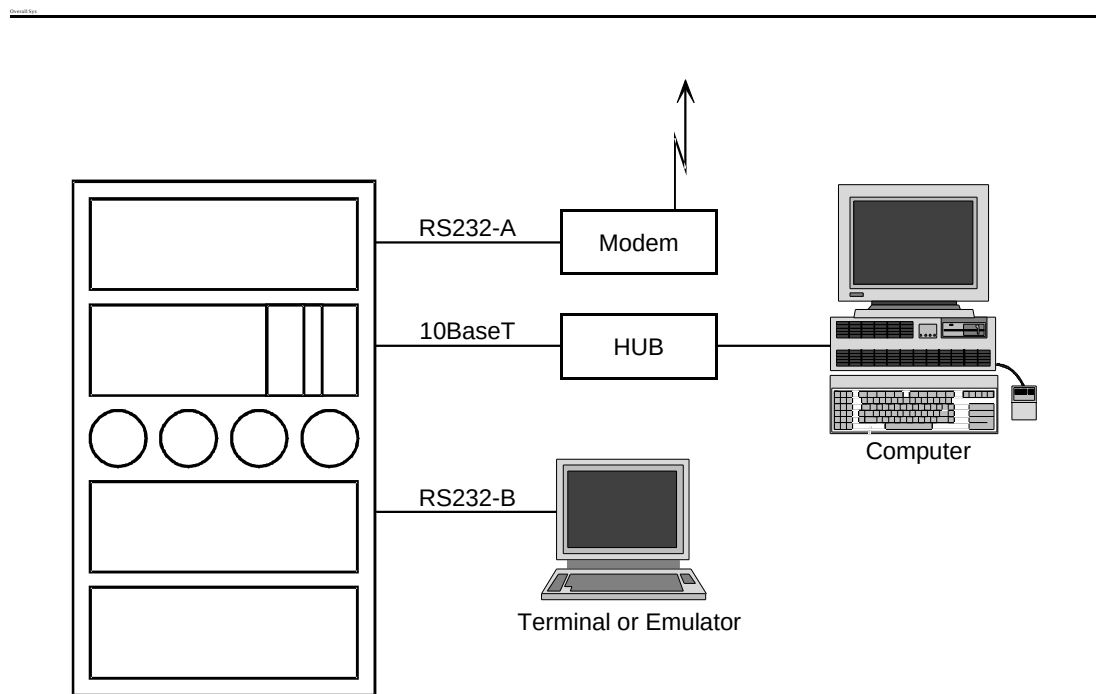
Figure 13-3. Overall System Connectivity
