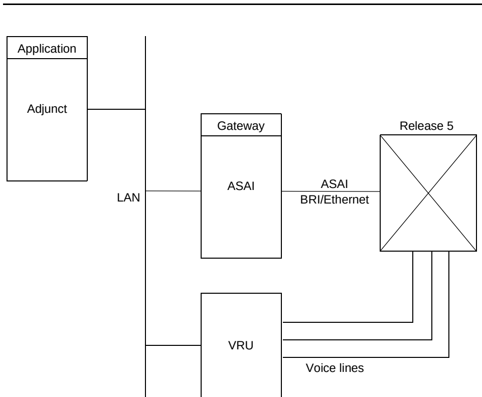
Figure 2-5. ASAI Integration with a VRU Configuration
