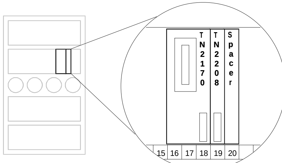
Figure 13-1. DEFINTY LAN Gateway System Assembly in a DEFINTY ECS Carrier
