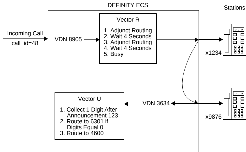
Figure A-14. Call Flow for an Agent who has a VDN in the Coverage Path
