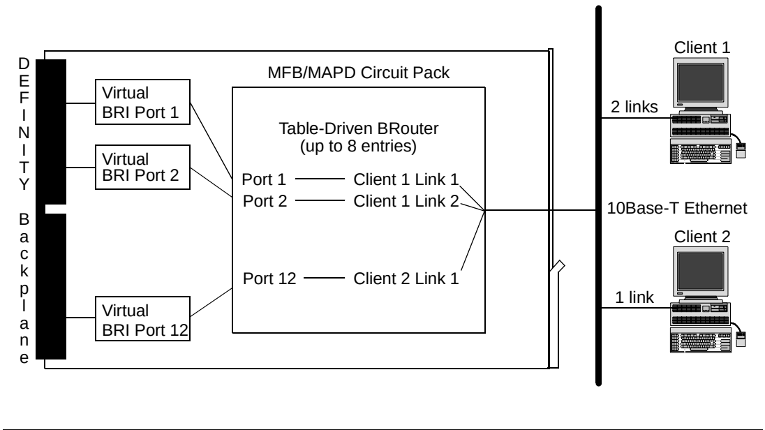
Figure 13-6. Relationship of Virtual BRI Ports, Brouter, and DEFINTY LAN Gateway Clients
