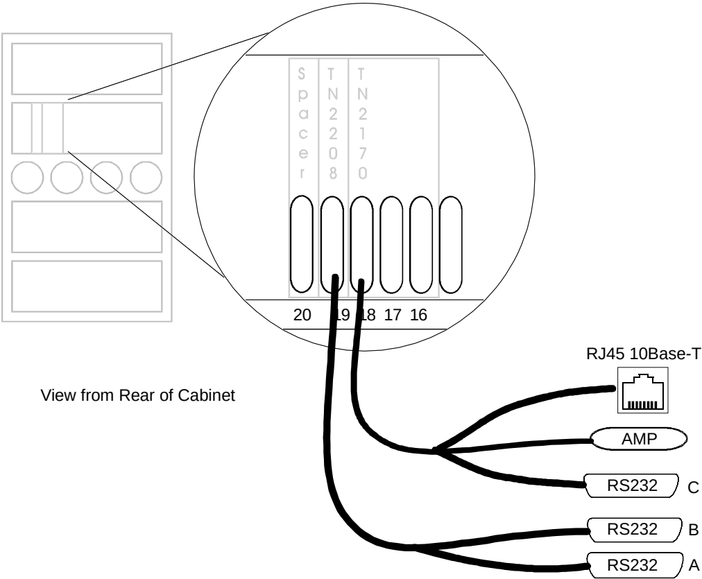
Figure 13-2. Cable Connectivity to the System Assembly
