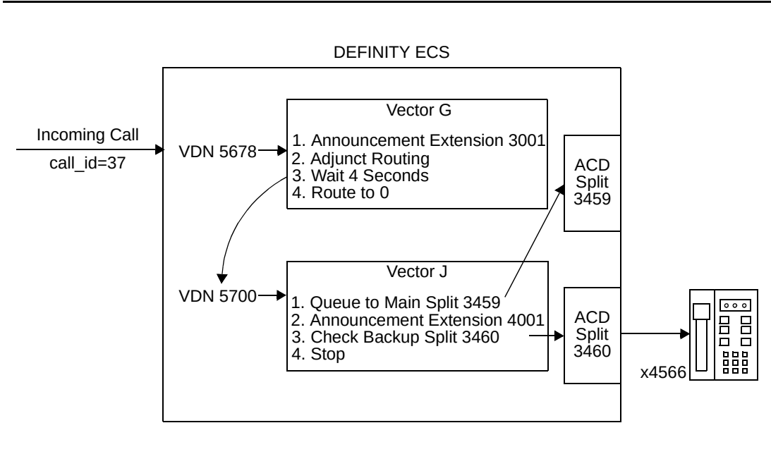
Figure A-15. Call Flow for Call to a VDN with Announcement and Routed to Another VDN
