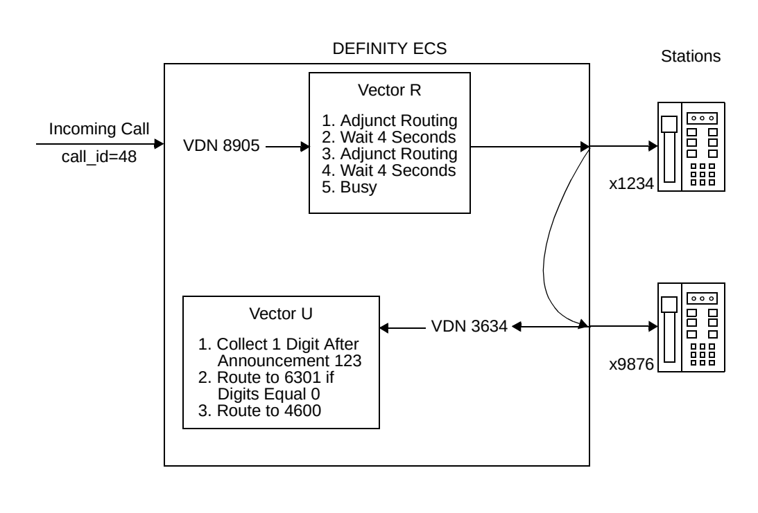
Figure B-45. Call Flow for an Agent who has a VDN in the Coverage Path
