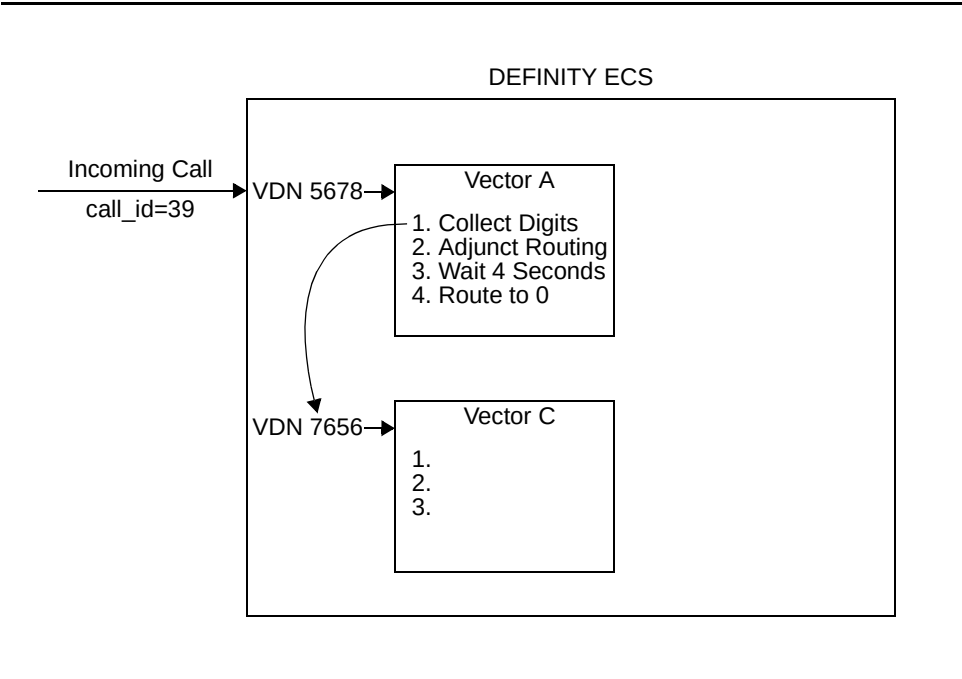
Figure B-5. Call Flow for Incoming Call to VDN Routed to Another VDN
