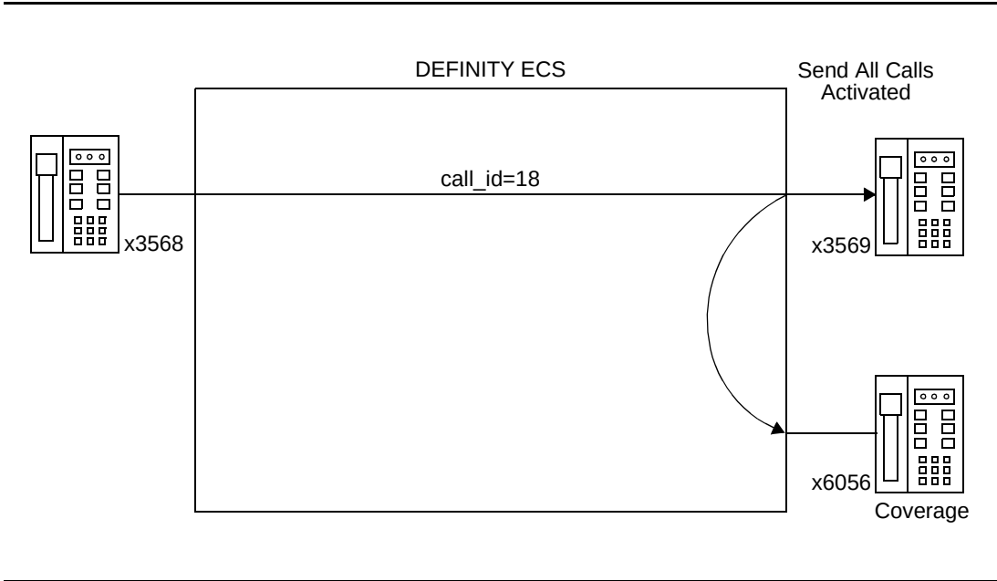
Figure B-28. Incoming Call to Station Sent to Coverage via Send All Calls (SAC)
