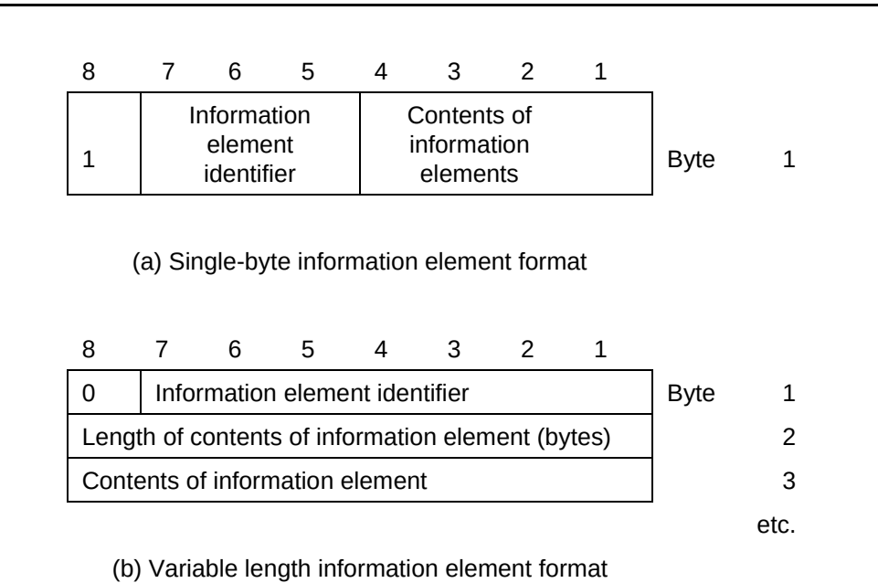
Figure 4-3. Formats of Information Elements
