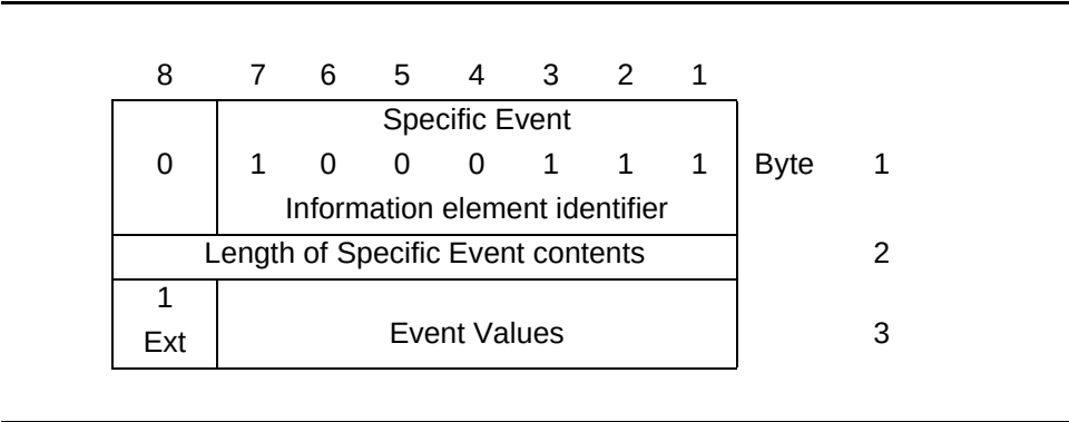
Figure 4-37. Specific Event Identifier Information Element
