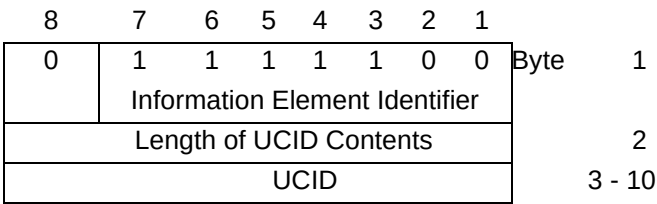
Figure 4-41. UCID Identifier Information Elements
