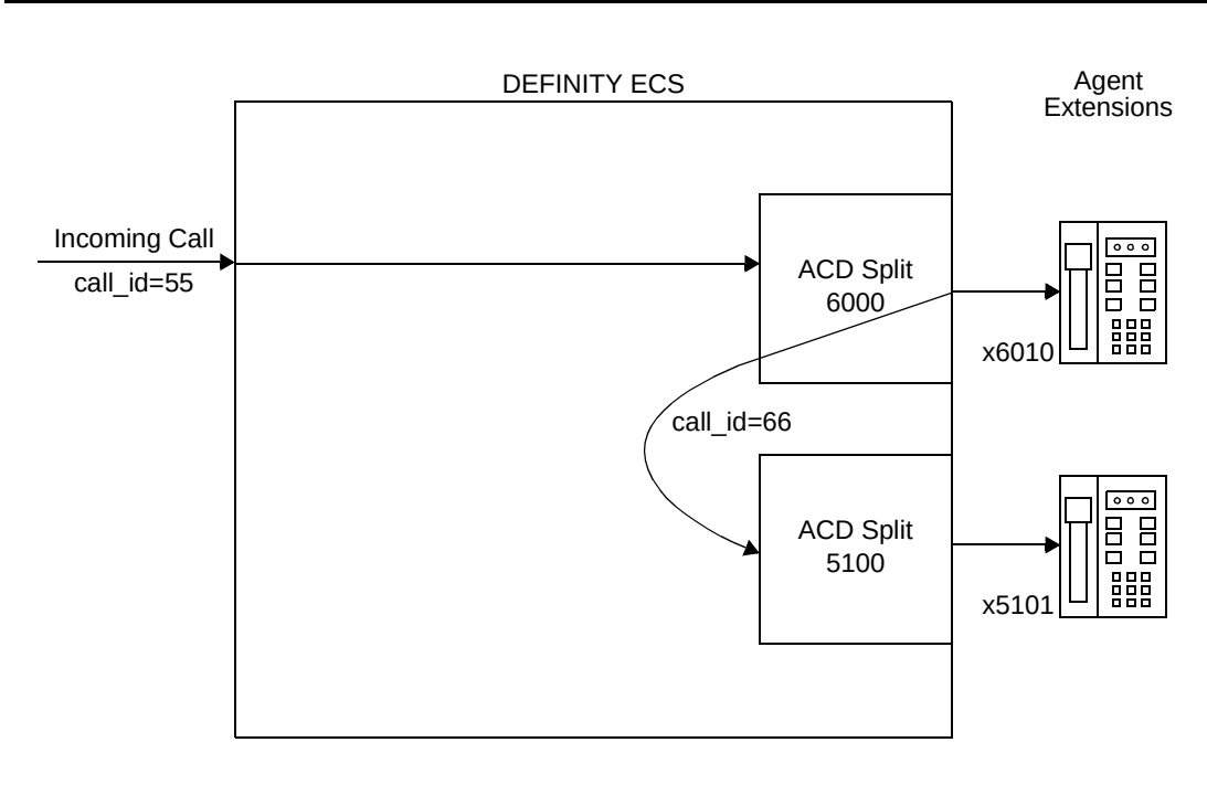
Figure B-18. Call Flow for Merging Two Calls with Event Notification and Call Control
