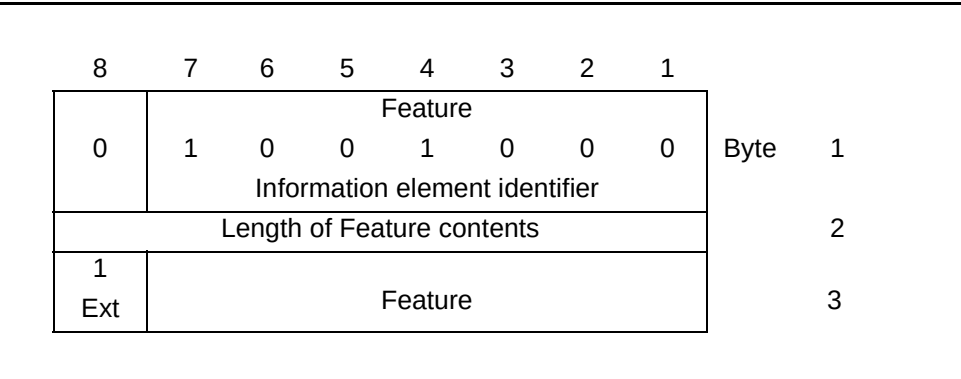
Figure 4-26. Feature Information Element
