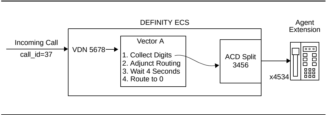
Figure B-3. Call Flow for Incoming Call to VDN Routed to ACD Split
