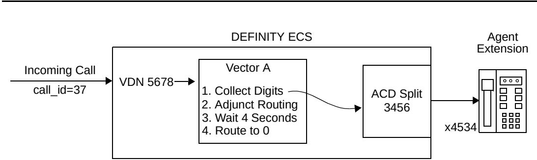
Figure B-12. Call Flow for Incoming Call to VDN Routed to ACD Split
