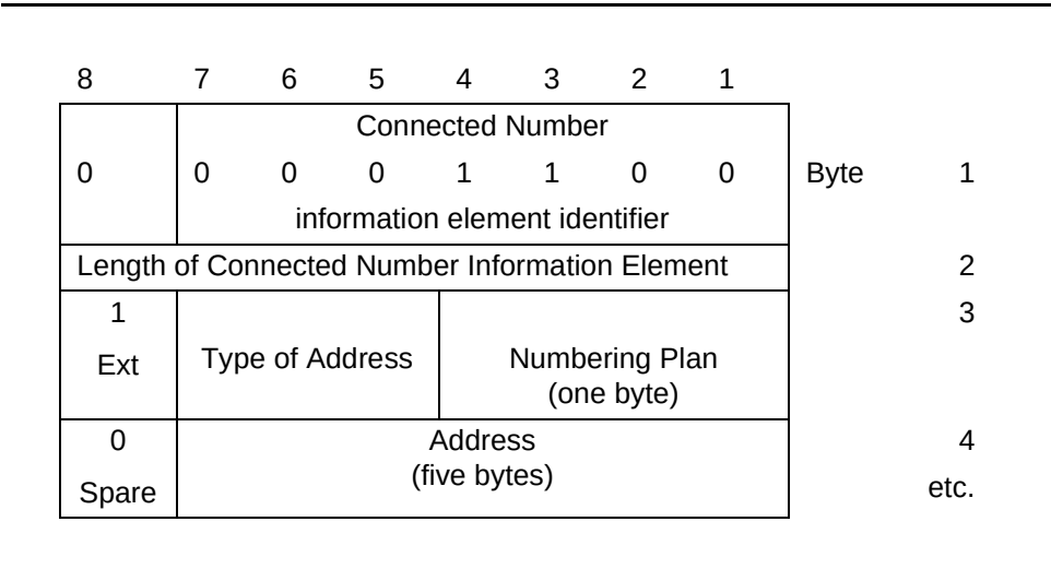
Figure 4-10. Connected Number Information Element
