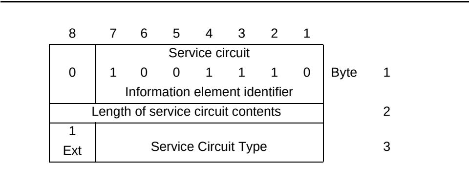
Figure 4-36. Service Circuit Information Element
