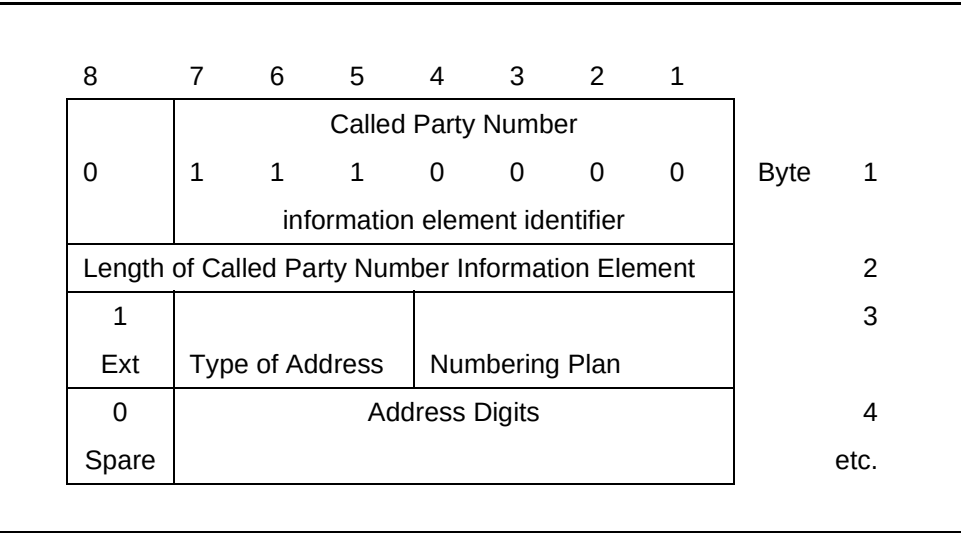
Figure 4-6. Called Party Number Information Element
