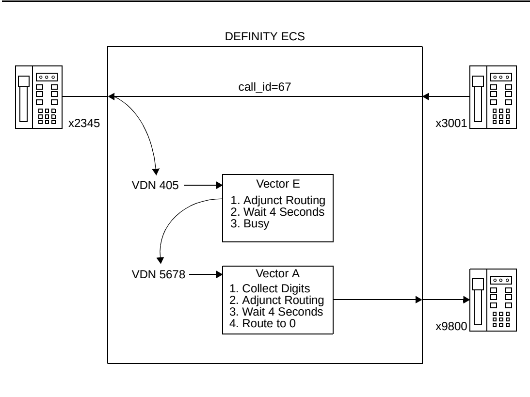
Figure B-25. Call Flow for Incoming Call to Station Forwarded to VDN
