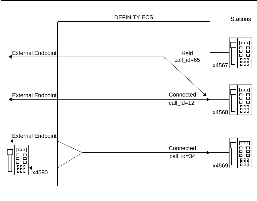
Figure B-22. Calls Present at Domain Controlled Stations 4567, 4568, and 4569
