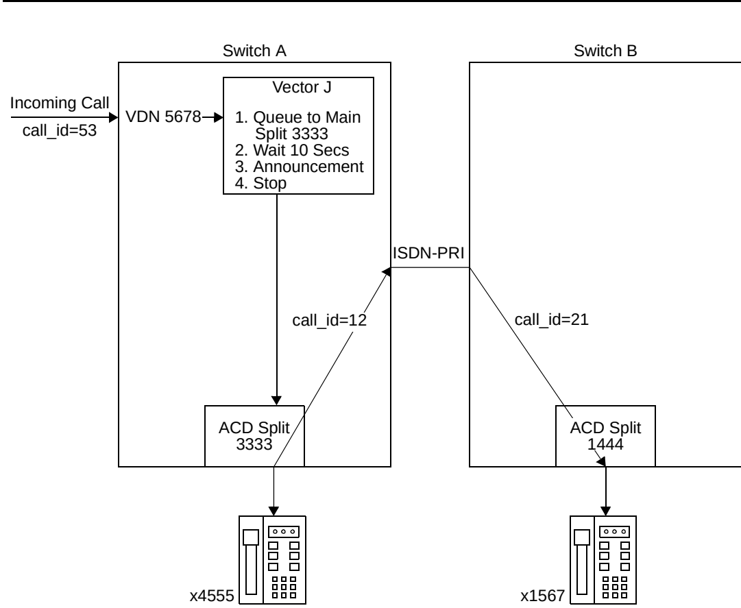
Figure B-34. Call Flow for Consultation Transfer to Another Switch
