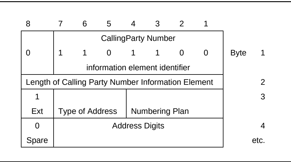
Figure 4-7. Calling Party Number
