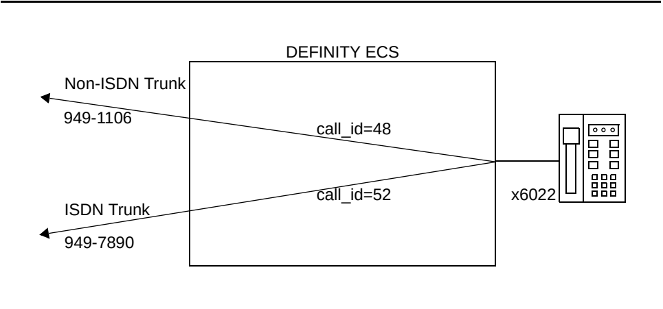
Figure B-14. Call Flow for Third Party Merge
