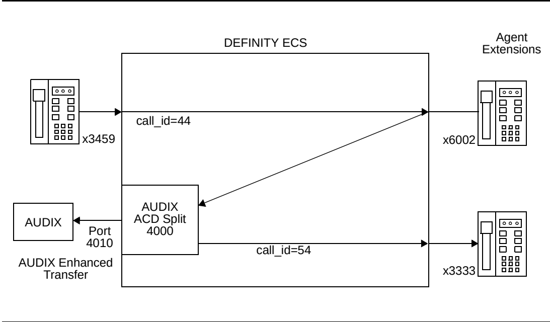
Figure B-31. Call Flow for Call Transferred out of AUDIX
