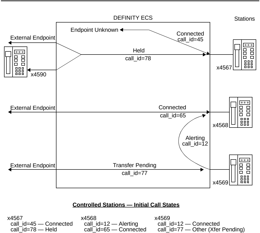
Figure B-19. Initial Call States for Domain (Station) Control
