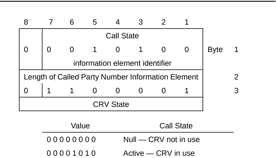
Figure 4-5. Call State Information Element
