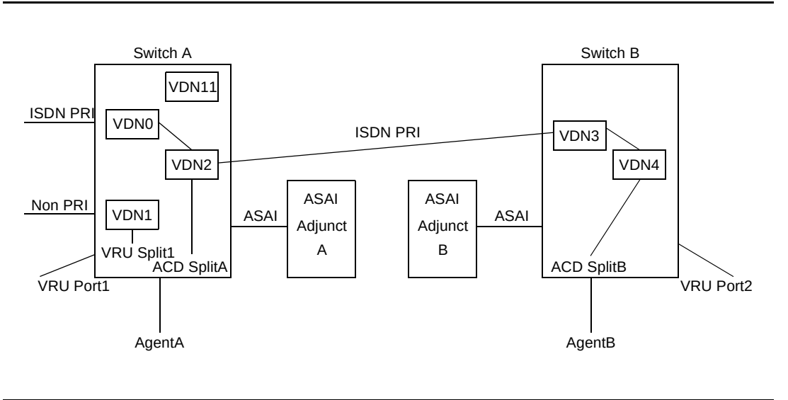
Figure B-49. Distributed ACD Configuration
