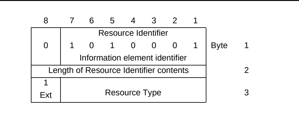
Figure 4-34. Resource Identifier Information Element
