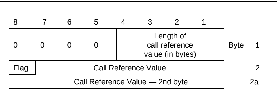
Figure 4-2. ISDN Call Reference Value
