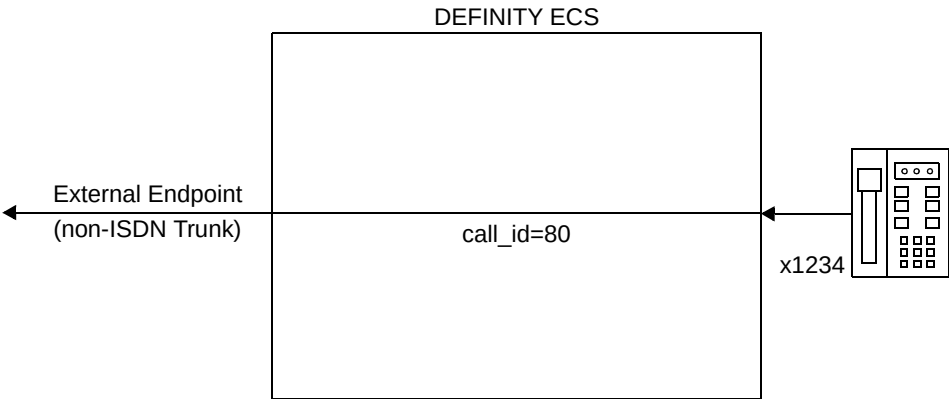
Figure B-47. Outgoing Call over Non-ISDN Trunk
