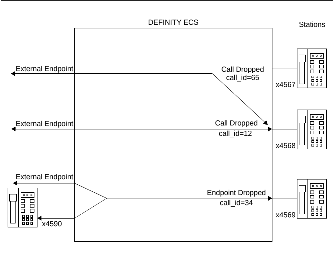
Figure B-23. Call Flow for Call Disconnects
