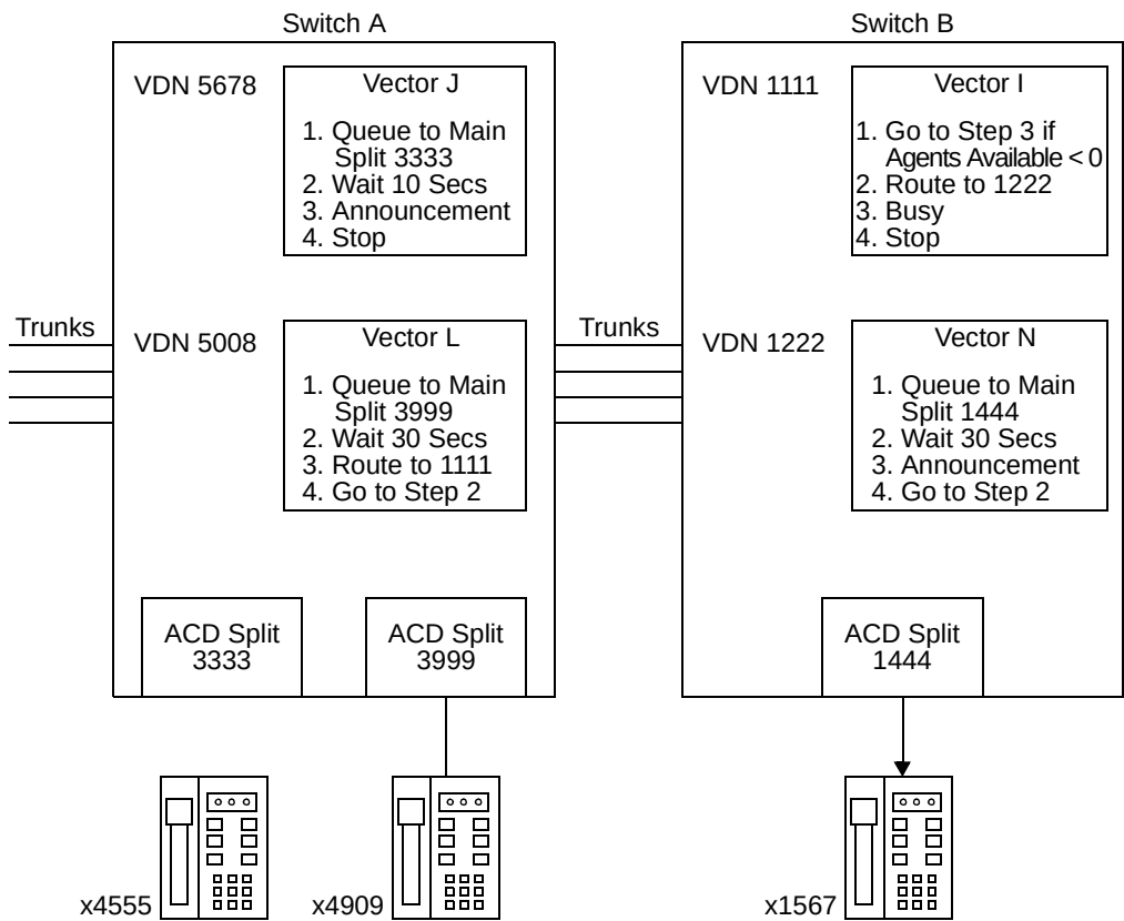
Figure B-32. Multiple Switch Configuration
