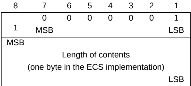
Figure 4-24. Long Form of the Length Field in the ECS Implementation (2 Bytes)
