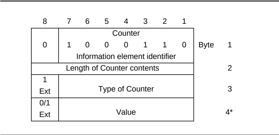
Figure 4-19. Counter Information Element
