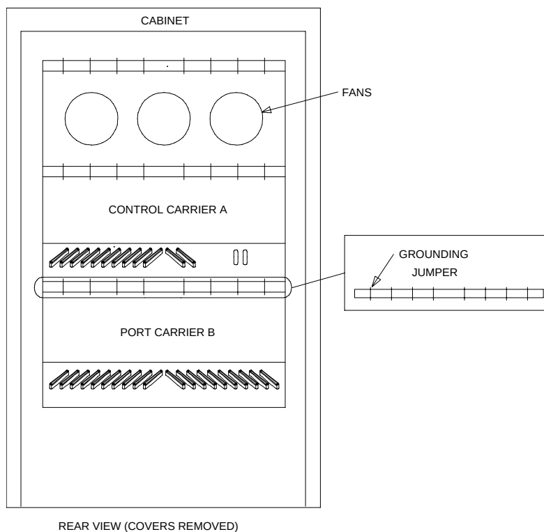
Figure 6-2. Locations of Grounding Jumpers (Small Cabinet)
