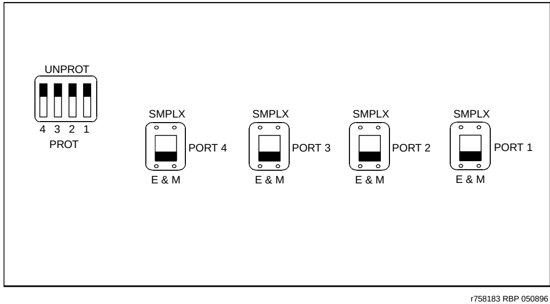
Figure 7-1. Tie Trunk Circuit Packs (Component Side)
