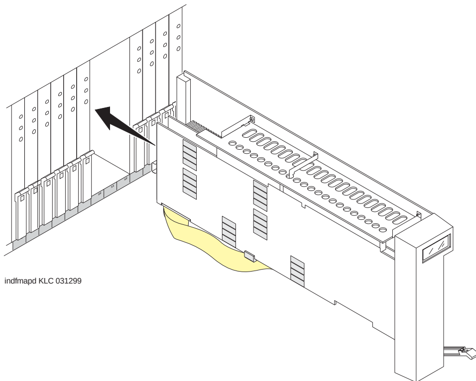
Figure 7-12. J58890MA-1 L30 IP Interface Assembly
