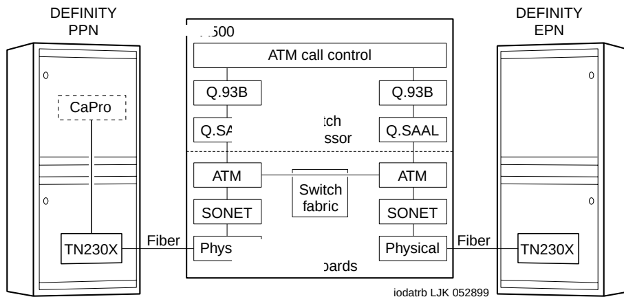
Figure 6-2. ATM signaling architecture
