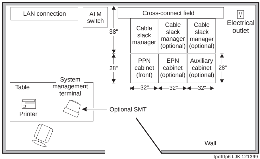
Figure 17. Typical Floor Plan with ATM Switch (Not available with Category B)
