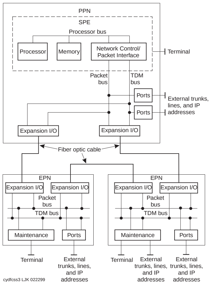
Figure 3. Components of a Direct-Connect System
