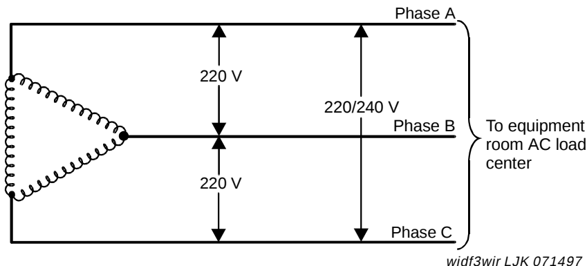
Figure 21. International Delta, 220 or 240 VAC, 50-Hz Source
