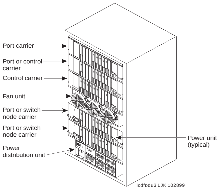
Figure 32. Typical Multi-Carrier PPN Cabinet (J58890A)
