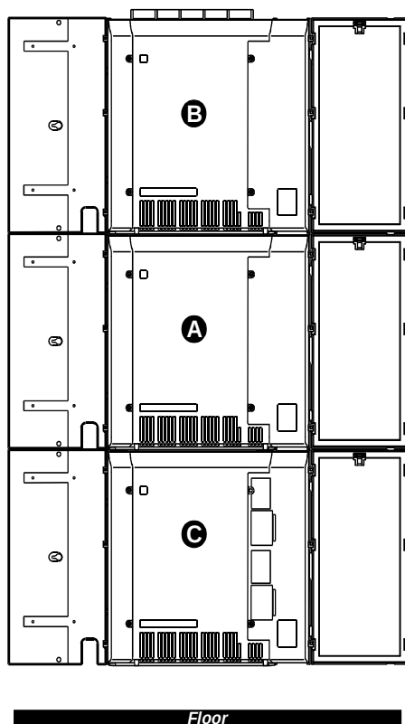
Figure 49. Typical Compact Modular Cabinet (csi model) Installation (Front)
