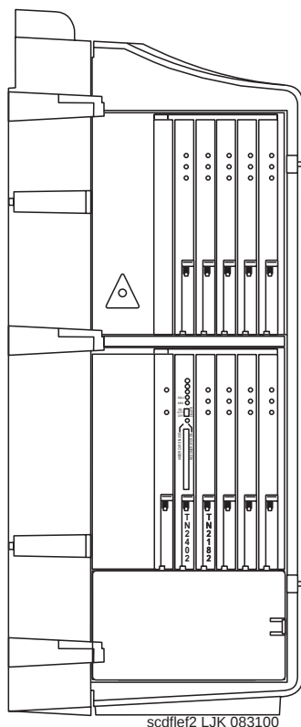
Figure 47. J58890T Compact Modular Cabinet (csi model) (Left Side)
