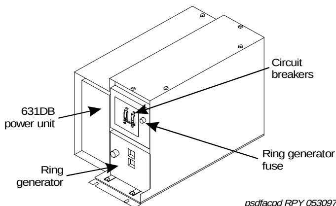
Figure 22. AC Power Distribution Unit (J58890CE-2) (Front)
