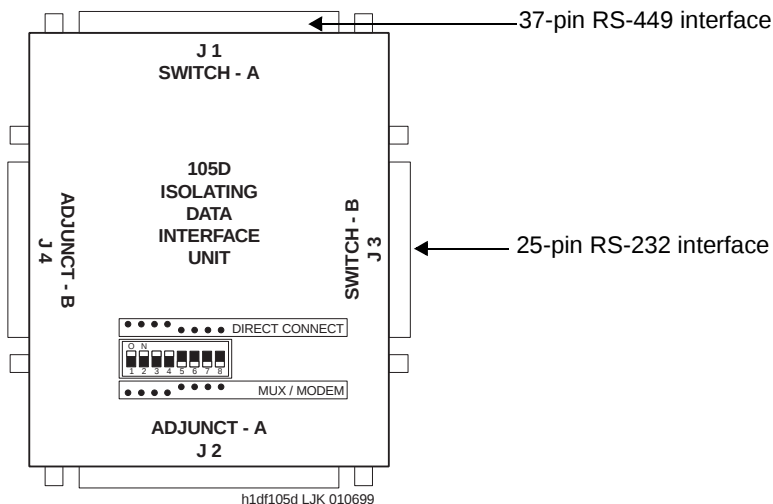
Figure 50. 105D Isolating Data Interface
