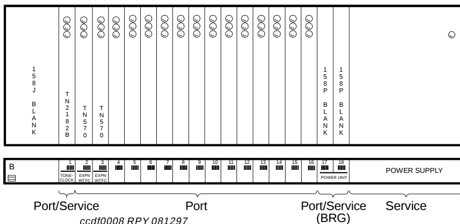
Figure 46. Port Cabinet (J58890H) (Front)
