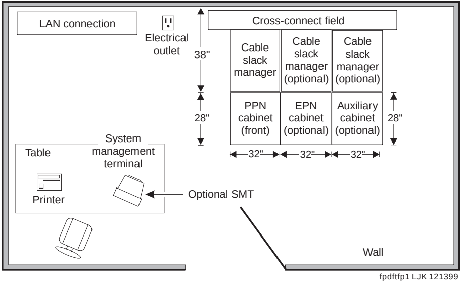
Figure 14. Typical Floor Plan with EPN and Auxiliary Cabinet
