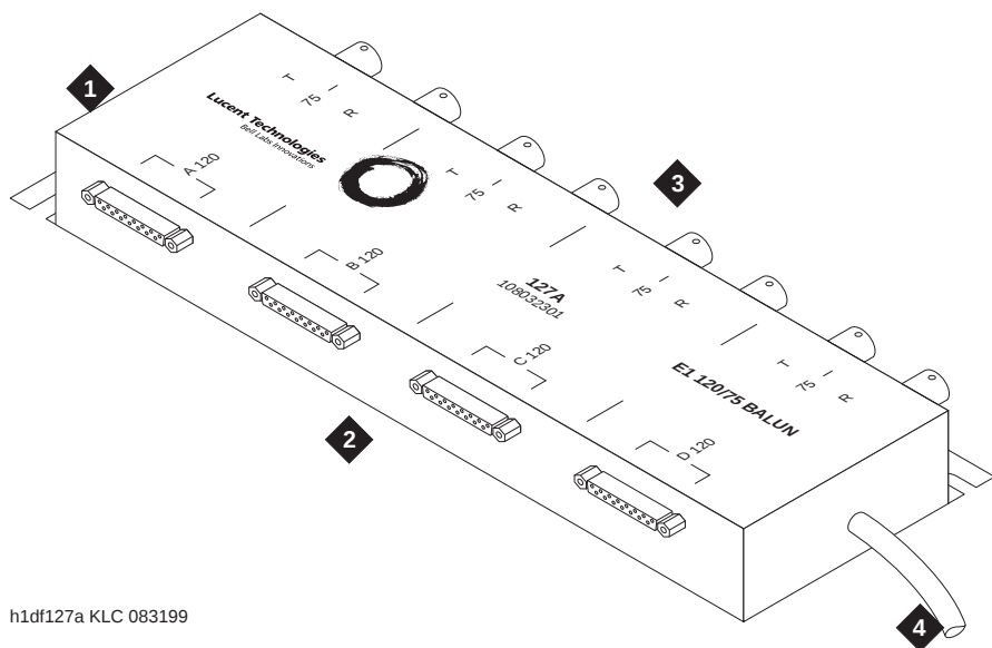
Figure 51. 127A E1 120 Ohm/75 Ohm Quad Balun Box
