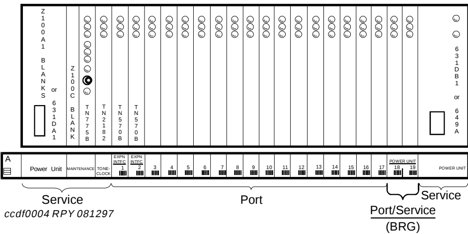
Figure 39. Expansion Control Carrier (J58890AF) (Front)
