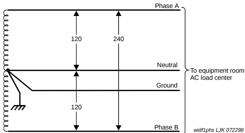
Figure 18. Single-Phase, 120/240 VAC, 60 Hz Source
