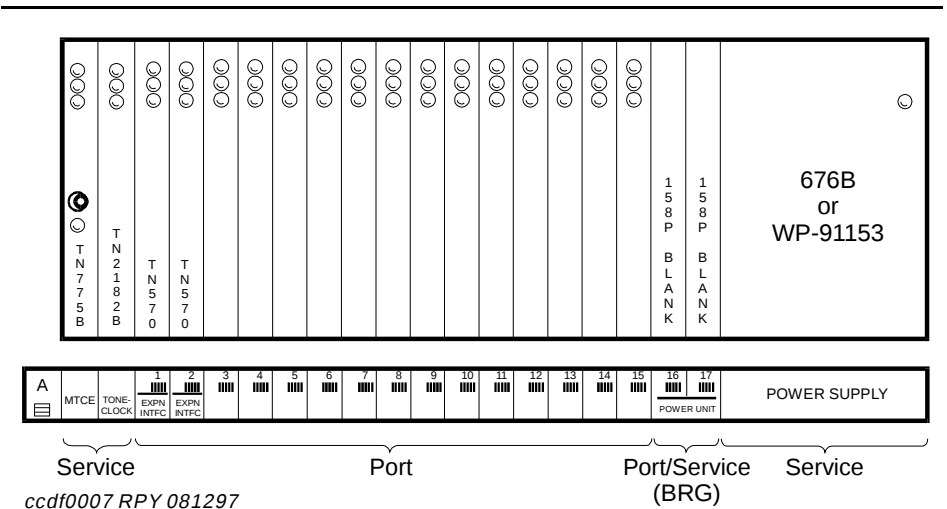
Figure 45. Expansion Control Cabinet (J58890N) (Front)
