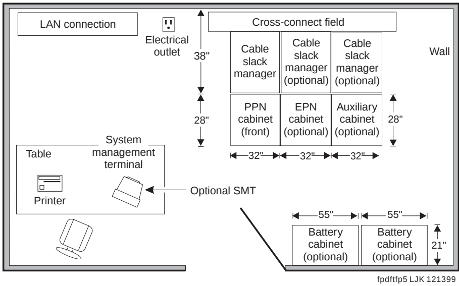
Figure 16. Typical Floor Plan with Battery Cabinets
