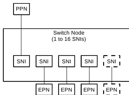
Figure 5. CSS with Switch Nodes (SNs)
