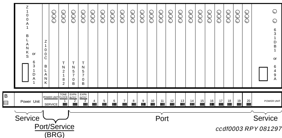
Figure 38. J58890BB Port Carrier (Front)
