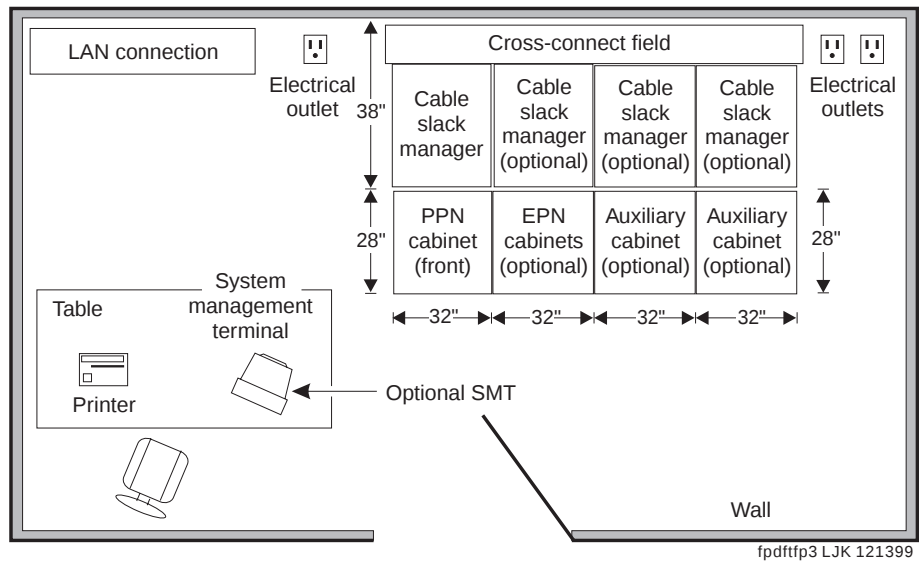
Figure 15. Typical Floor Plan with an additional EPN and Auxiliary Cabinets
