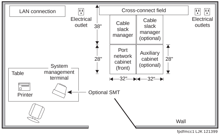
Figure 13. Typical Multi-Carrier Cabinet Floorplan
