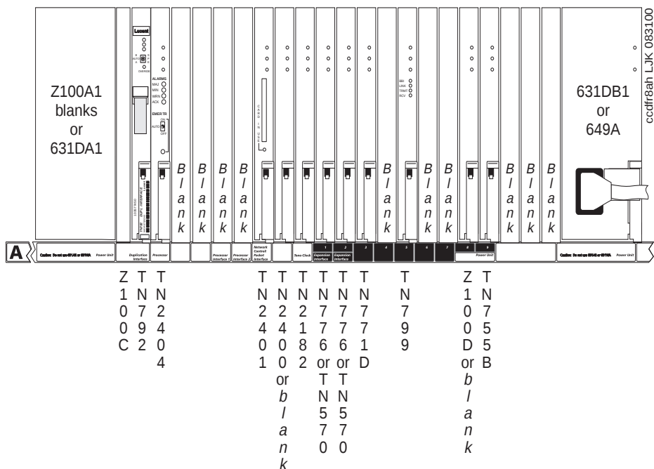
Figure 35. J58890AH Control Carrier (si model)
