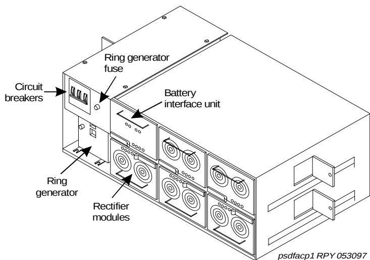
Figure 25. AC Power Distribution Unit (J58890CH-1) (Front)
