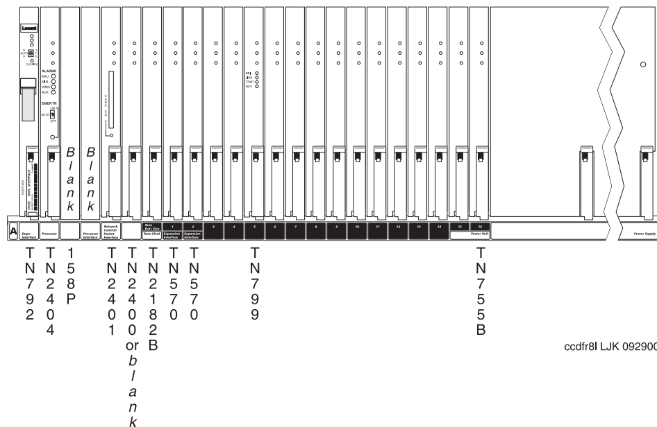
Figure 43. Basic Control Cabinet (si model) (J58890L) (Front)
