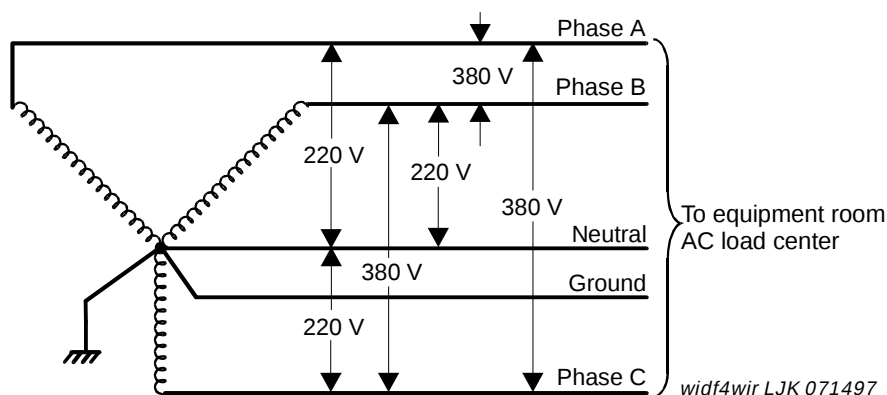
Figure 20. International, Three Phase, 220/380 VAC, 50-Hz Source
