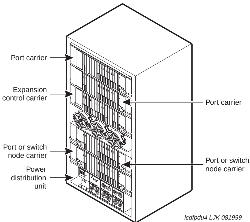
Figure 33. Typical Multi-Carrier EPN Cabinet (J58890A)
