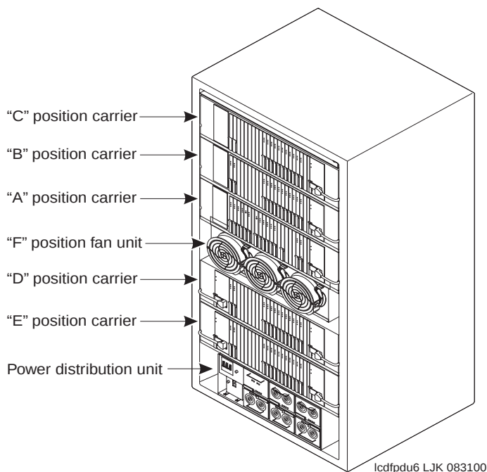
Figure 8. Typical Multi-Carrier Cabinet
