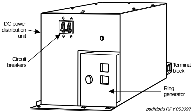
Figure 28. DC Power Distribution Unit (J58890CF-2) (Front)
