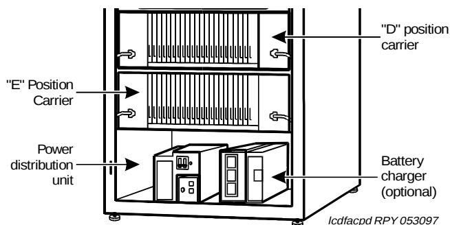
Figure 24. AC Power Distribution in Multi-Carrier Cabinets
