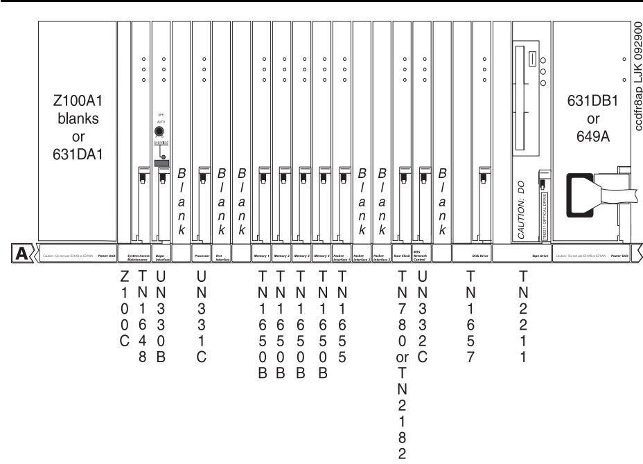
Figure 37. Processor Carrier (r model) (J58890AP) (Front)
