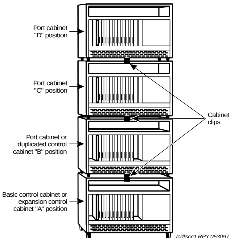
Figure 42. Typical SCC Stack
