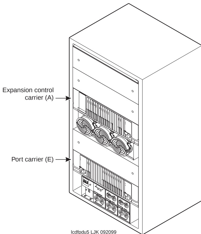
Figure 34. Dual EPN in an R7r or Later Multi-Carrier Cabinet
