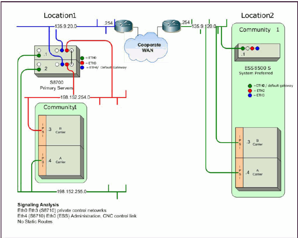
Figure 28: Multi-site CNC
