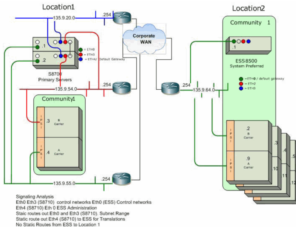
Figure 30: Multi-site, CNOCL (subnet routes)
