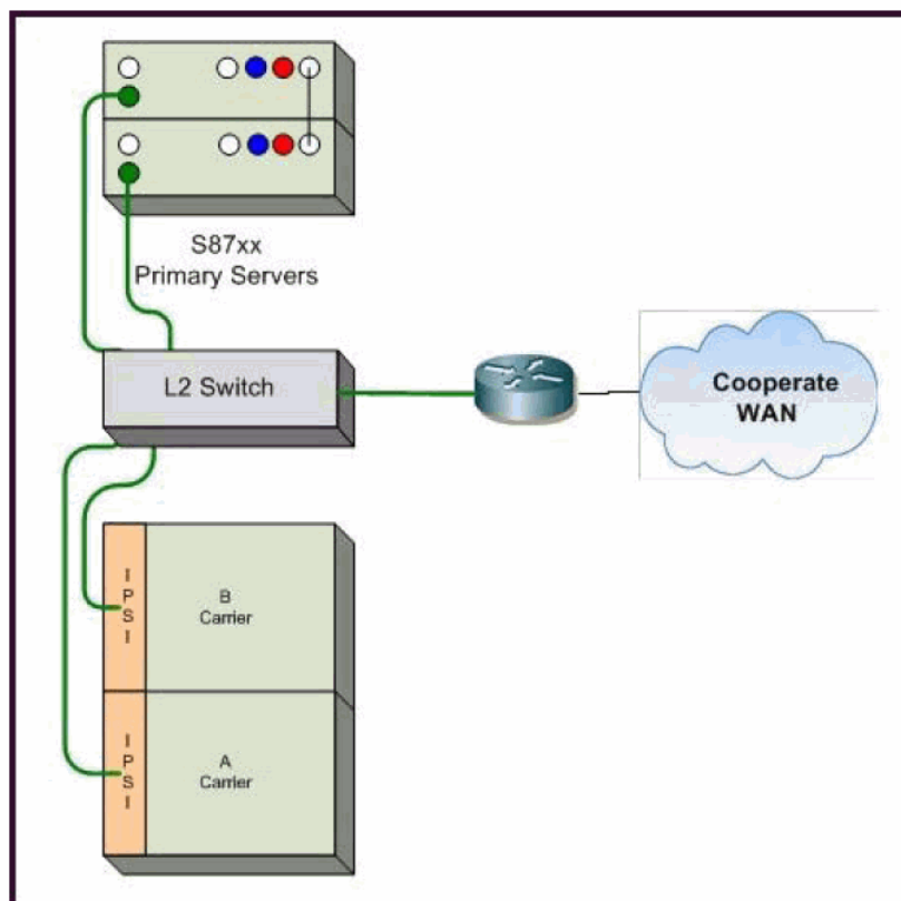
Figure 25: Layer 2 control network connectivity
