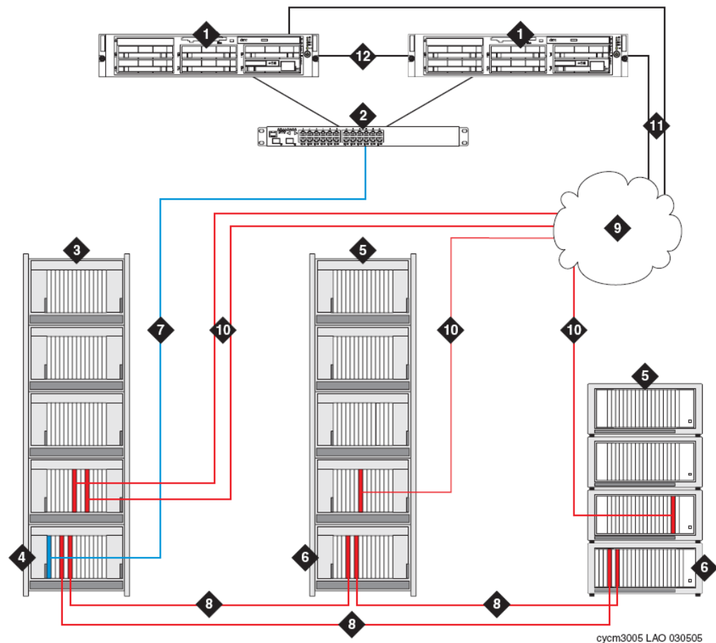
Figure notes: S8700-series direct-connect single control network
