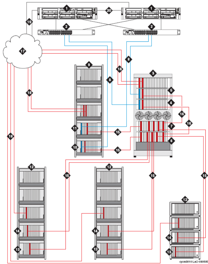
Figure 12: S8700-series Center Stage Switch duplicated control and duplicated voice-bearer networks
