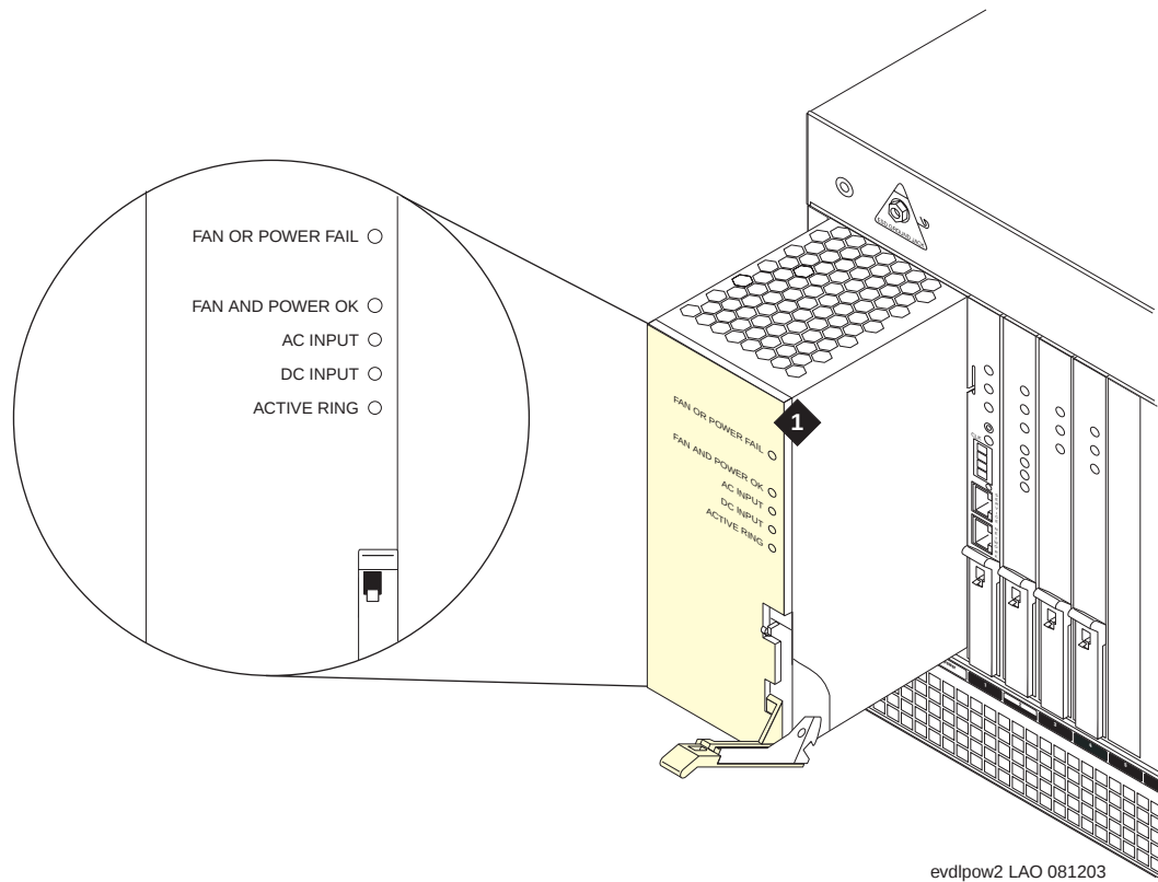
Figure 46: 655A faceplate LEDs
