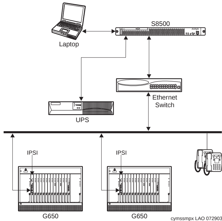
Figure 15: S8500 simplex configuration
