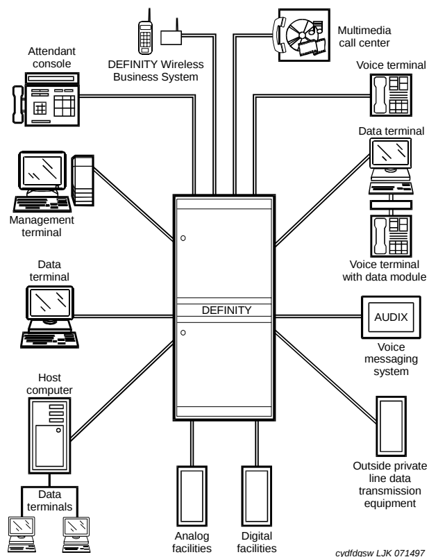
Figure 29: DEFINITY Server SI with Communication Manager
