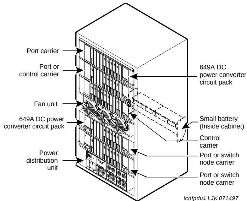
Figure 81: Power distribution in MCC1
