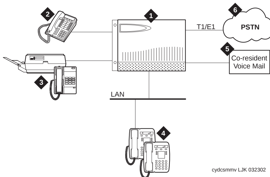
Figure 84: Small-business solution using the Avaya S8100 Media Server and the G600 Media Gateway
