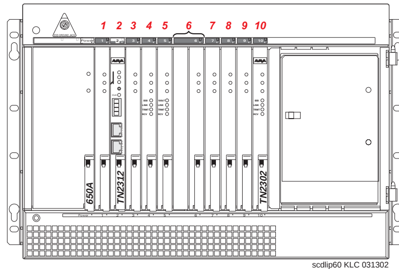
Figure 42: G600 Media Gateway
