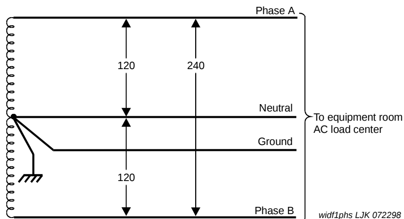
Figure 70: Single-phase, 120- to 240-VAC, 60-Hz source
