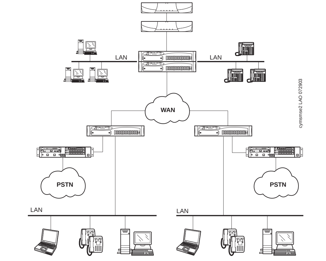
Figure 88: Multi-Site Configuration
