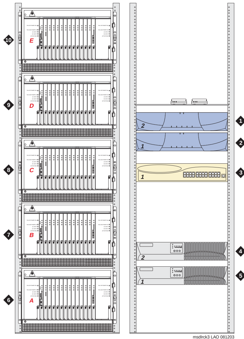
Figure 45: G650 stack
