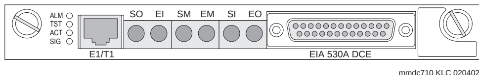
Figure 66: Avaya MM710 T1/E1 Media Module
