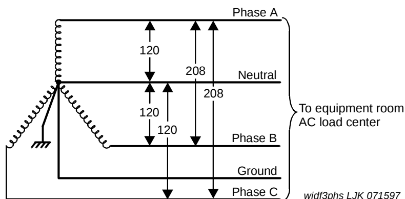
Figure 71: 3-phase, 120- to 208-VAC, 60-Hz source
