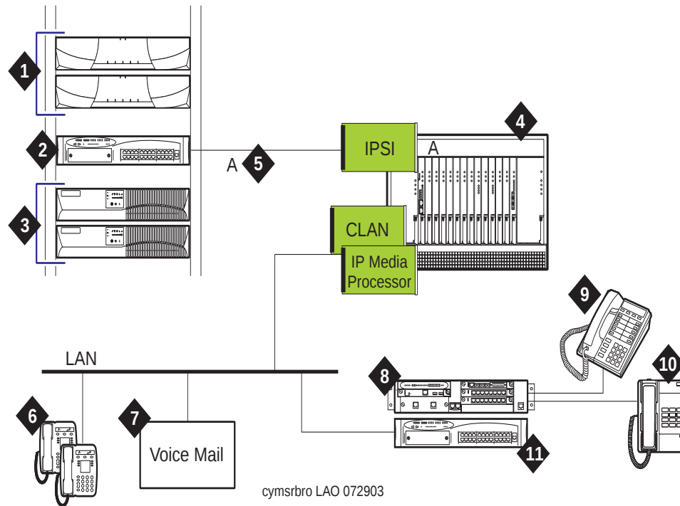
Figure 87: Branch Office Configuration
