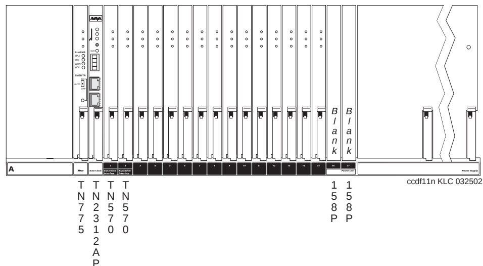
Figure 56: Expansion control cabinet
