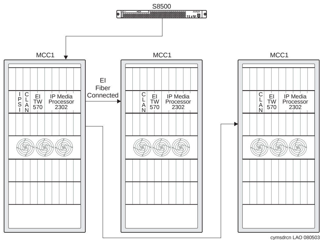
Figure 16: S8500 Media Server in a direct-connect configuration
