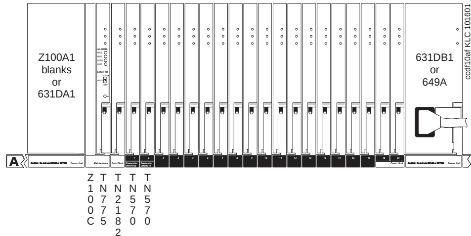
Figure 63: Expansion Control Carrier (Front)
