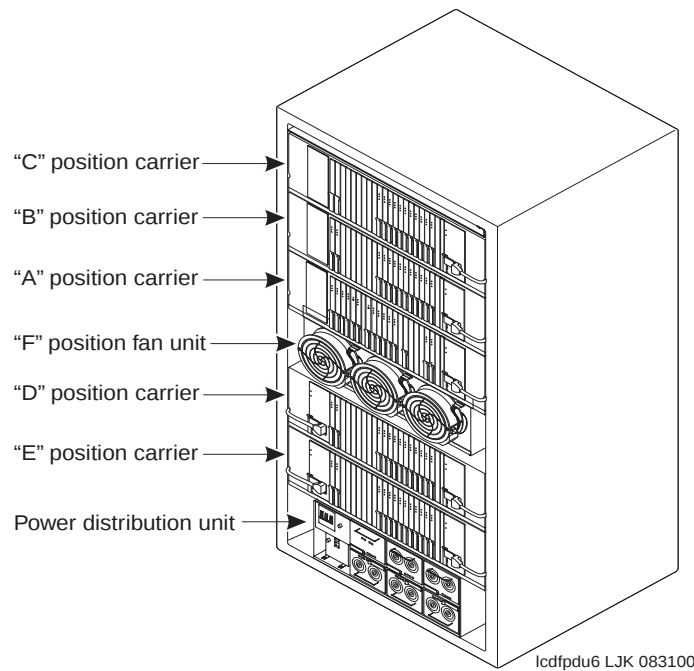
Figure 37: Typical multicarrier cabinet (MCC1)
