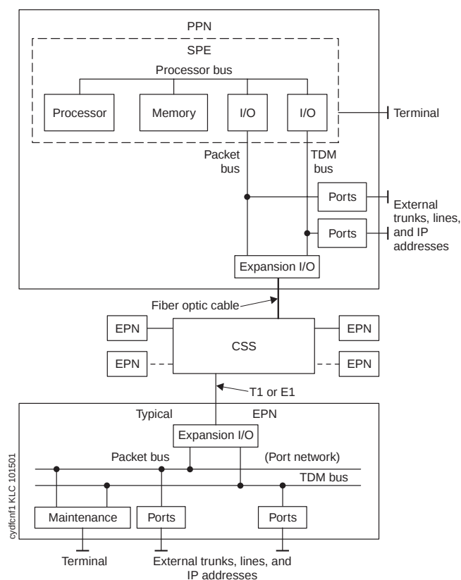
Figure 39: Components of a CSS-connected system
