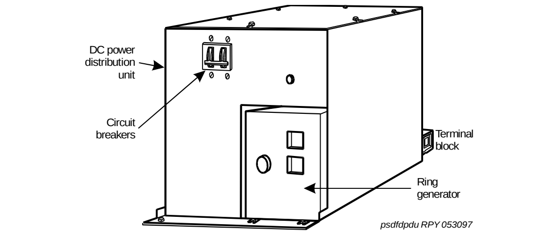
Figure 80: DC power-distribution unit (J58890CF-2) (front view))
