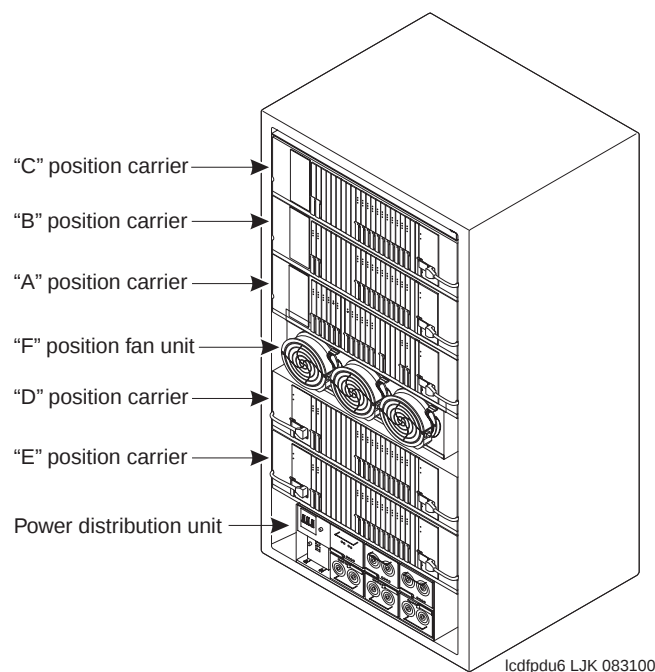
Figure 32: Typical multicarrier cabinet (MCC1)
