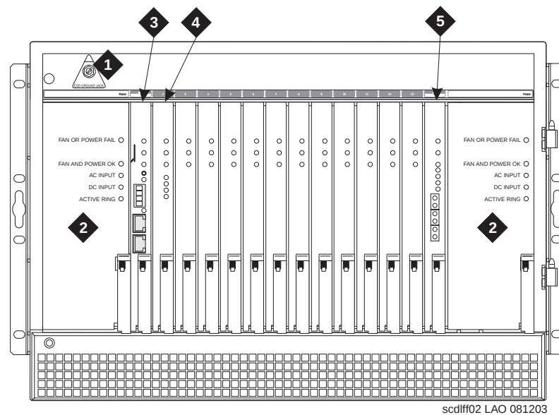
Figure 12: G650 Media Gateway
