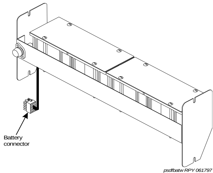
Figure 78: Small Battery Assembly
