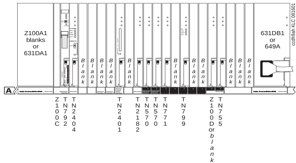
Figure 61: Control carrier (front)
