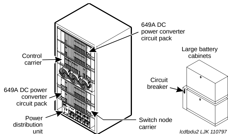
Figure 82: DC power distribution in MCC1s
