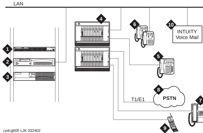
Figure 85: Medium-sized business solution using the Avaya S8500 Media Server and the G650 Media Gateway
