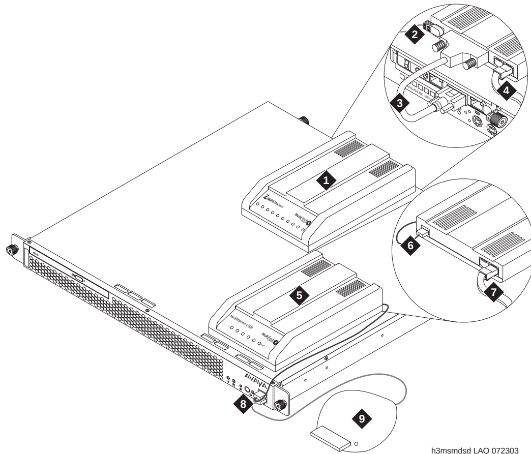
Figure 14: Modem connectivity to the S8500
