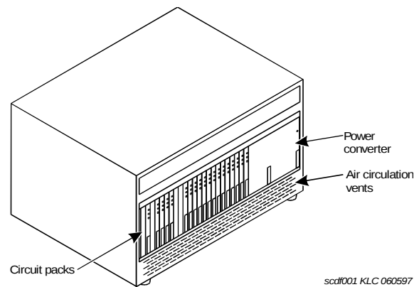
Figure 31: Typical single-carrier cabinet (SCC1)
