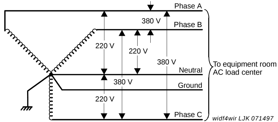
Figure 72: International, 3-phase, 220- to 380-VAC, 50-Hz source
