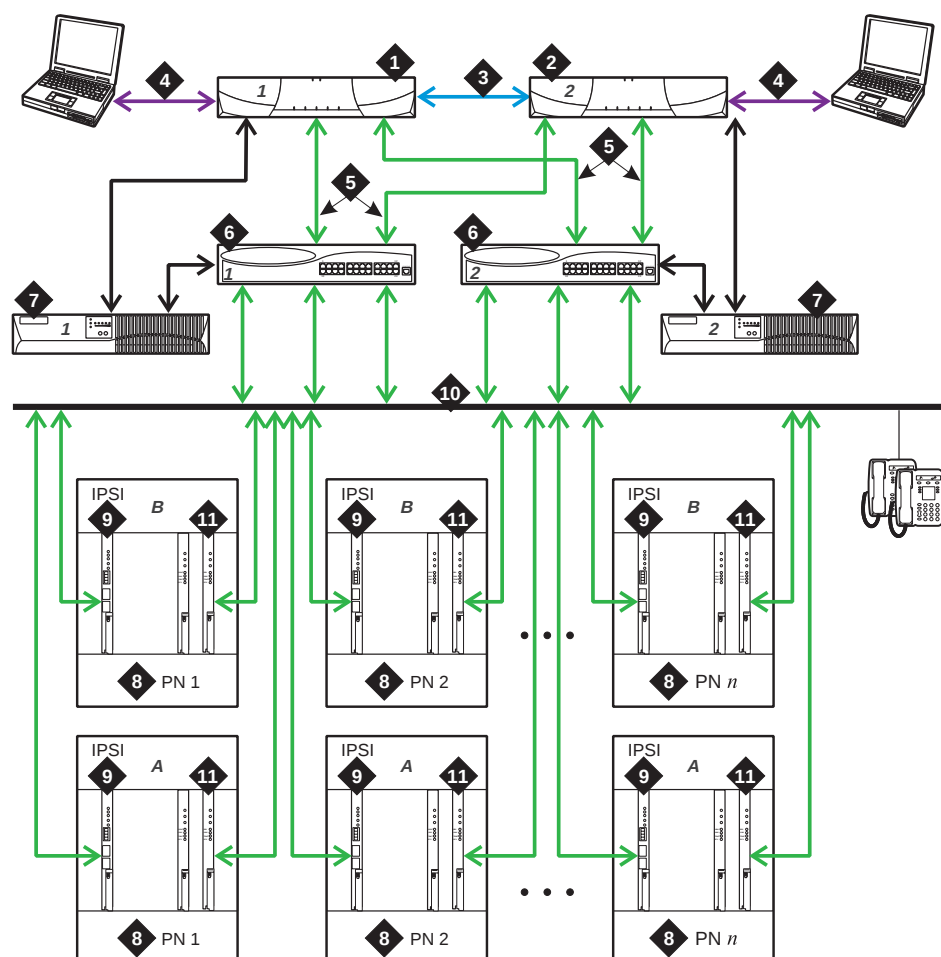
Figure 25: Duplex-reliability configuration when sending voice bearer over IP
