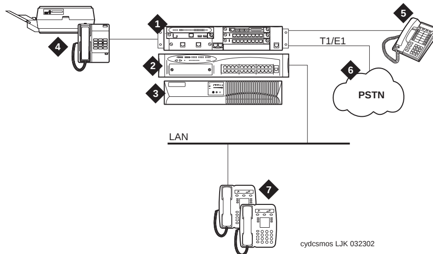
Figure 83: Small-business solution using the Avaya S8300 Media Server in the G700 Media Gateway
