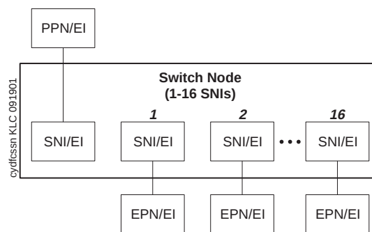
Figure 40: CSS with Switch Nodes (SNs)
