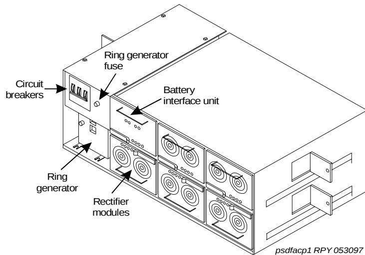
Figure 77: AC power-distribution unit (J58890CH-1) (front)
