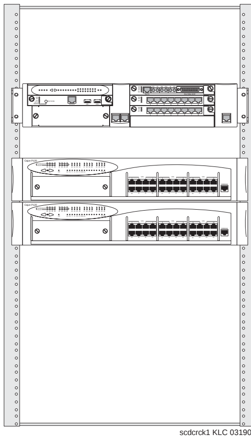
Figure 47: G700 Media Gateway with two Avaya P330 switches
