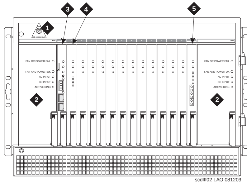
Figure 43: G650 Media Gateway
