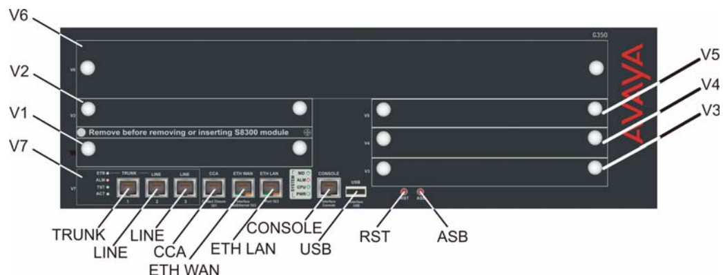
Figure 41: G350 chassis
