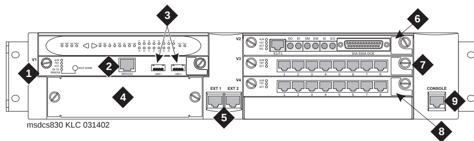
Figure 2: S8300 Media Server in a G700 Media Gateway
