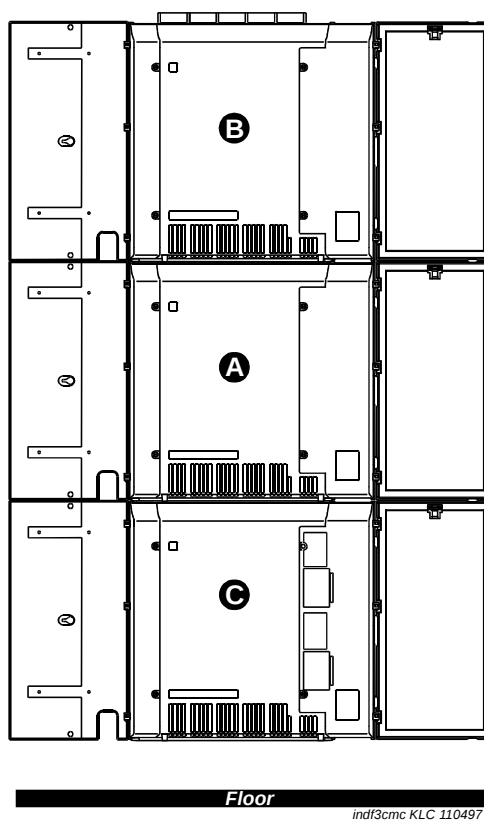
Figure 51: Typical vertical installation, front view of the CMC1 Media Gateway
