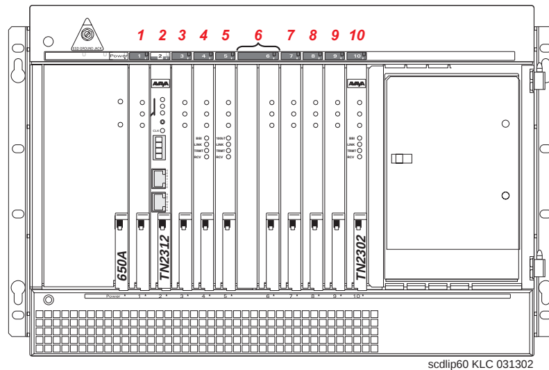
Figure 24: G600 Media Gateway
