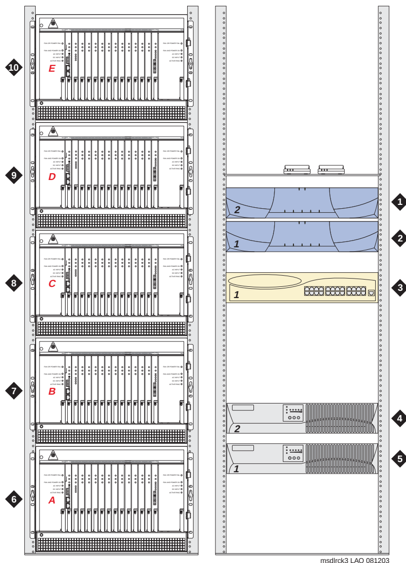
Figure 20: G650 Media Gateway
