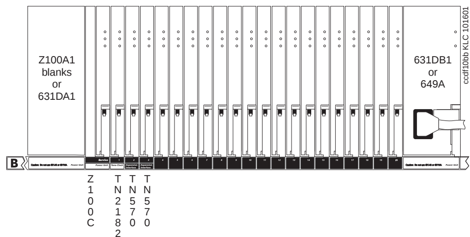
Figure 64: Port carrier (front)
