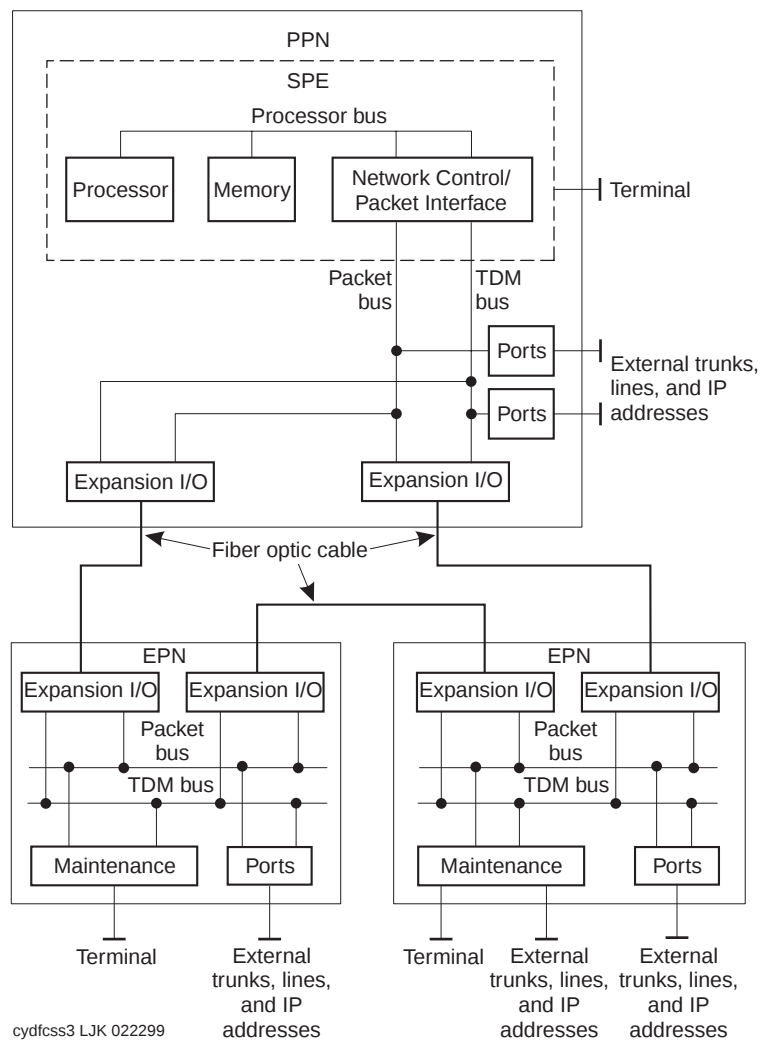
Figure 30: Components of a DEFINITY Server SI Configuration
