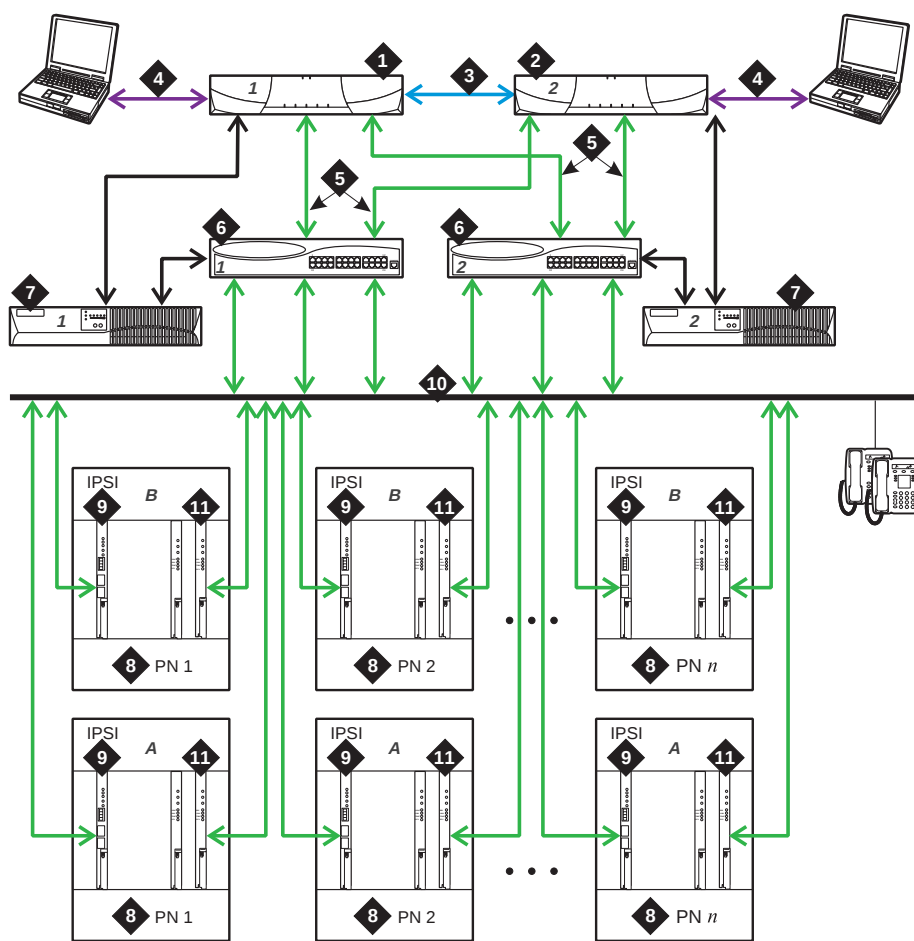
Figure 26: High-reliability when sending voice bearer over IP
