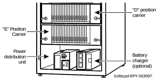
Figure 76: AC power distribution in MCC1 cabinets
