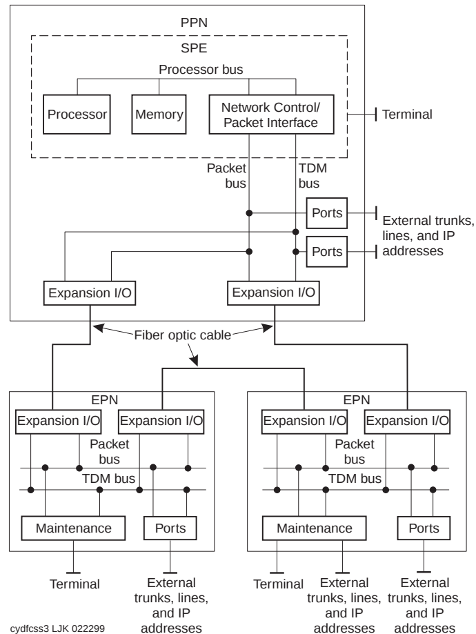
Figure 35: Components of a DEFINITY Server R
