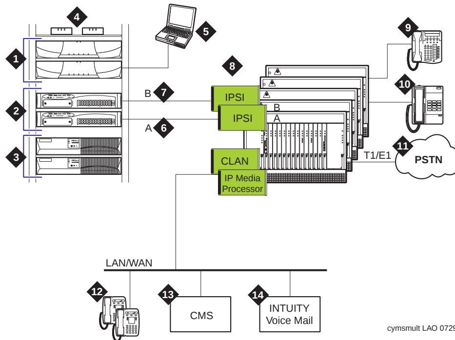
Figure 86: Large-business solution using the Avaya S8700 Media Server and the MCC1 Media Gateway
