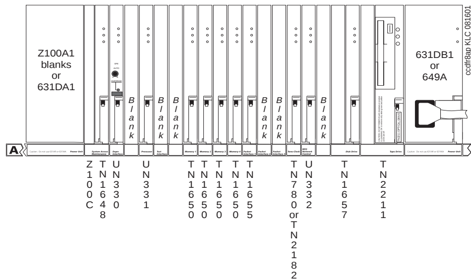
Figure 62: Processor Carrier
