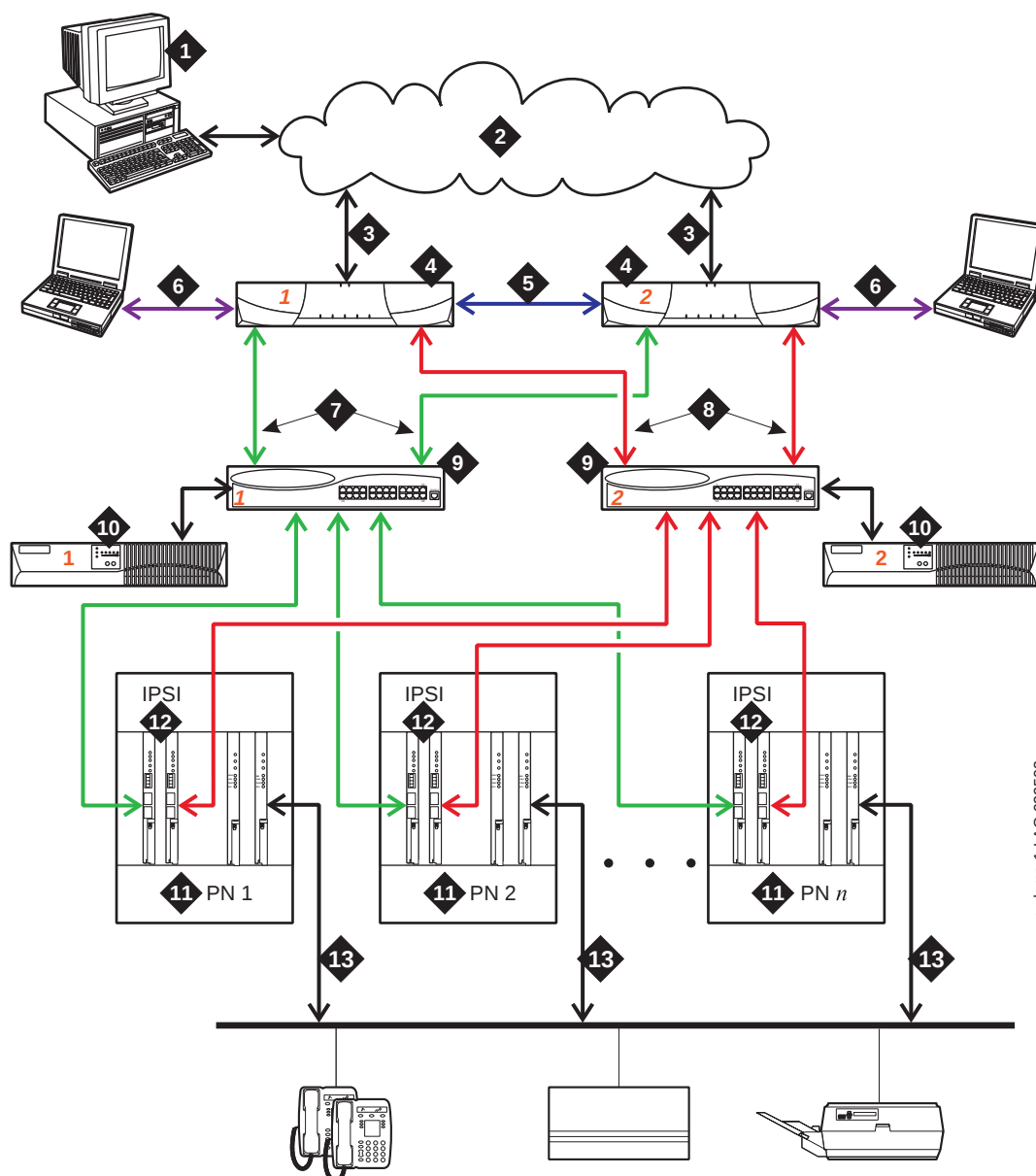
Figure 28: High-reliability configuration when sending voice bearer over CSS or ATM
