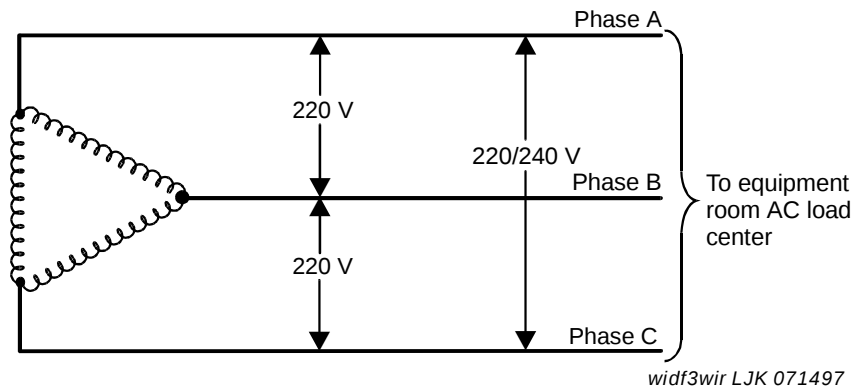
Figure 73: International delta, 220- or 240-VAC, 50-Hz source
