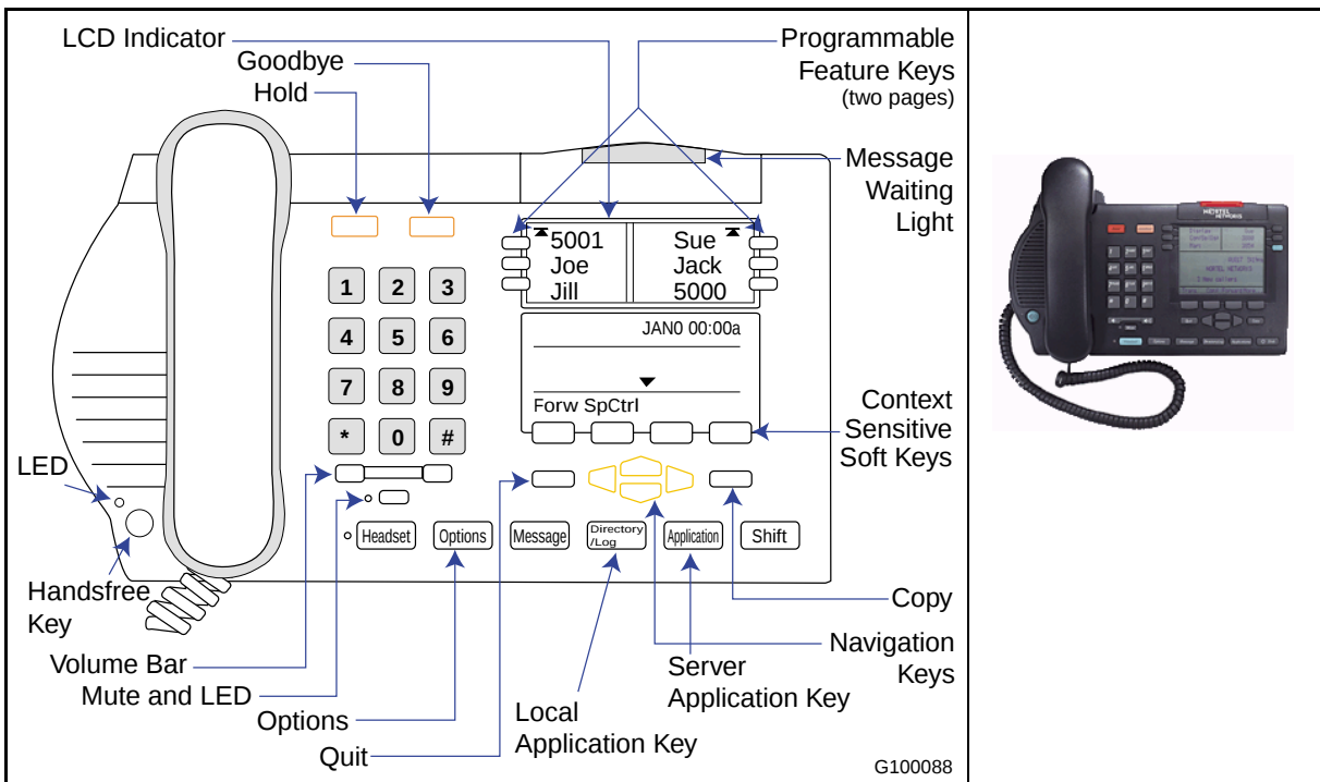
Figure 5 M3904 telephone set
