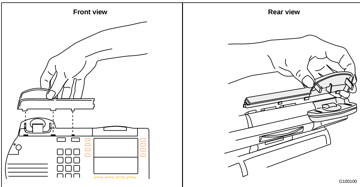
Figure 20 Removal of the hook switch cover
