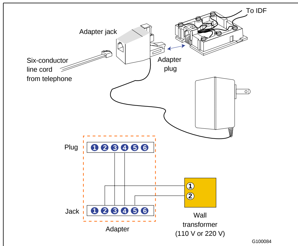
Figure 11 ATA connections
