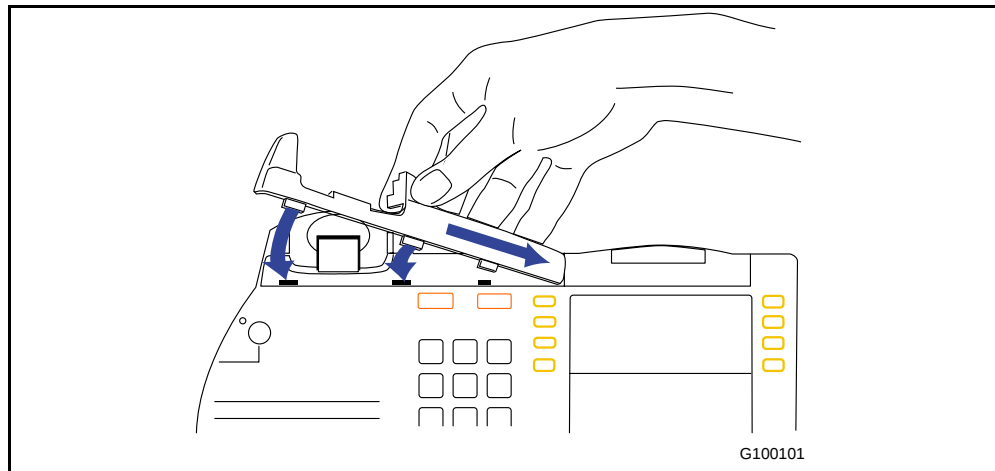
Figure 21 How to install the cradle
