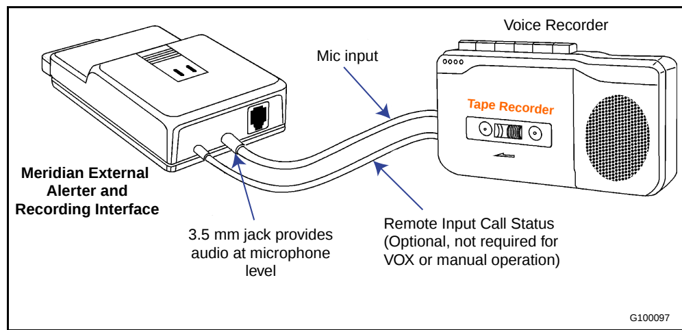
Figure 14 MEARI desktop voice recording device
