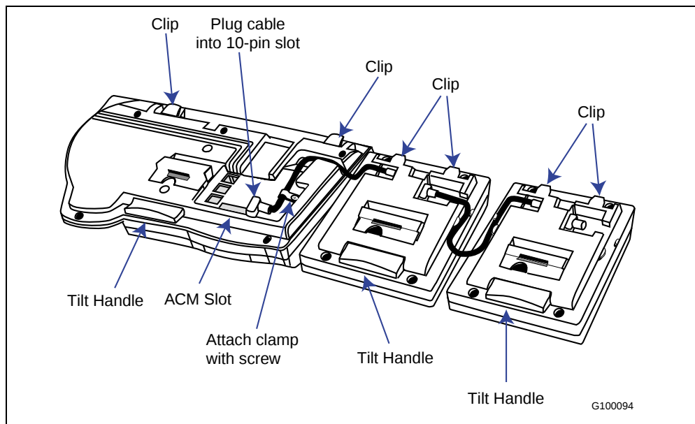
Figure 17 Key-based Expansion Module
