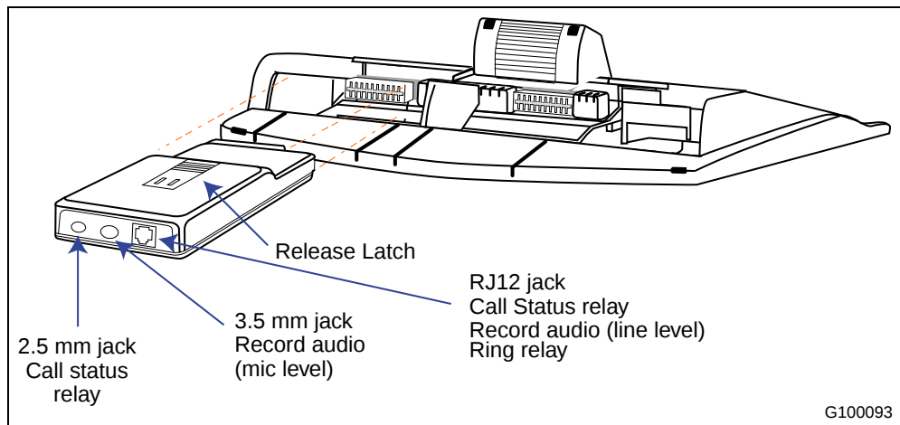
Figure 12 MEARI output connectors
