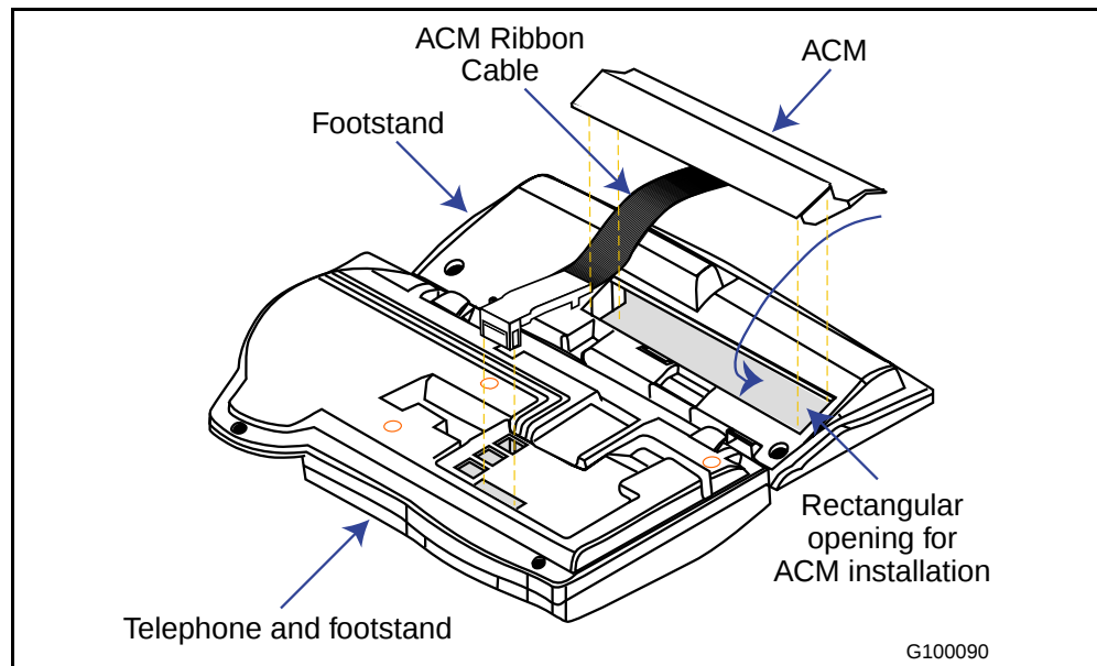
Figure 10 ACM Module
