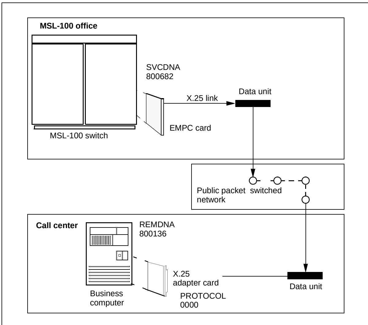
Figure 115 Packet switched network configuration
