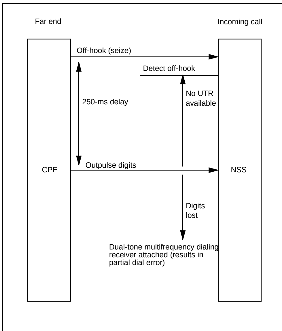
Figure 42 Trunk seizure and outputting of digits without UTR
