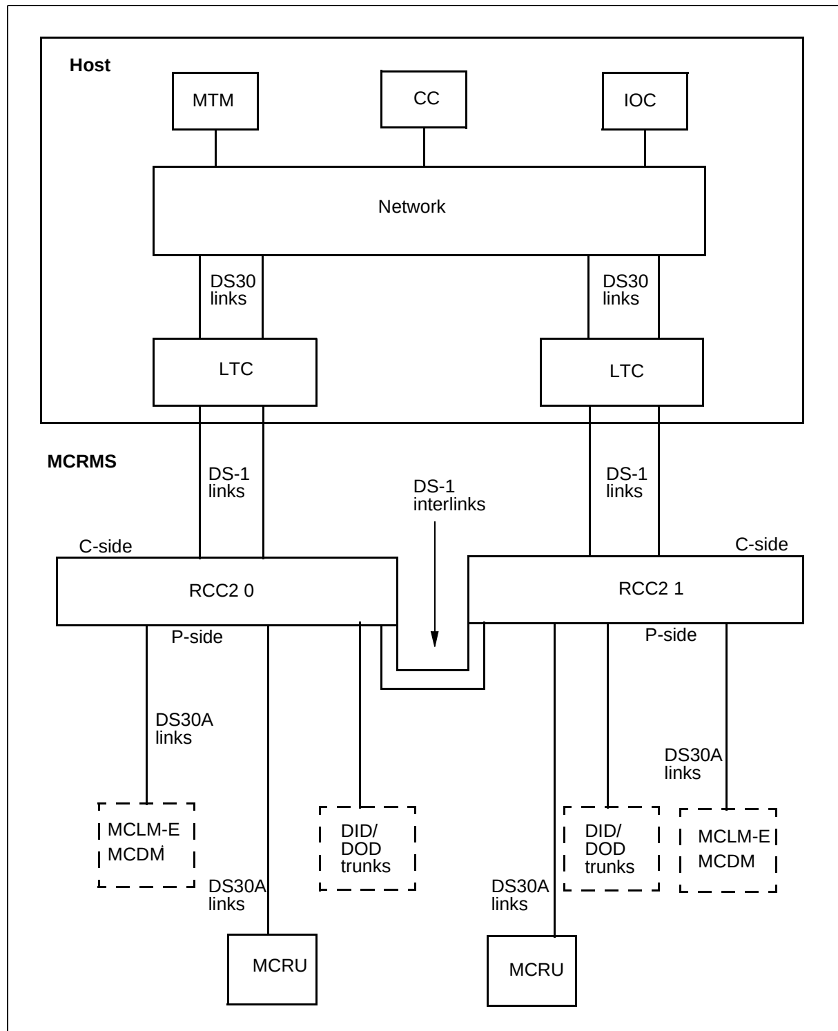
Figure 186 Dual MCRM-S
