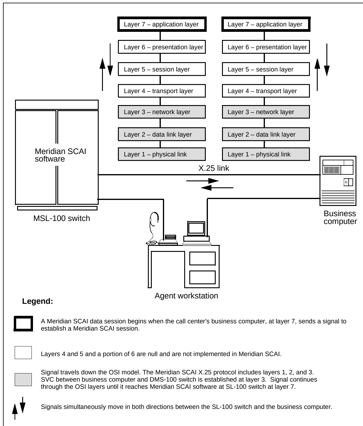
Figure 192 Meridian SCAI signaling and the OSI model
