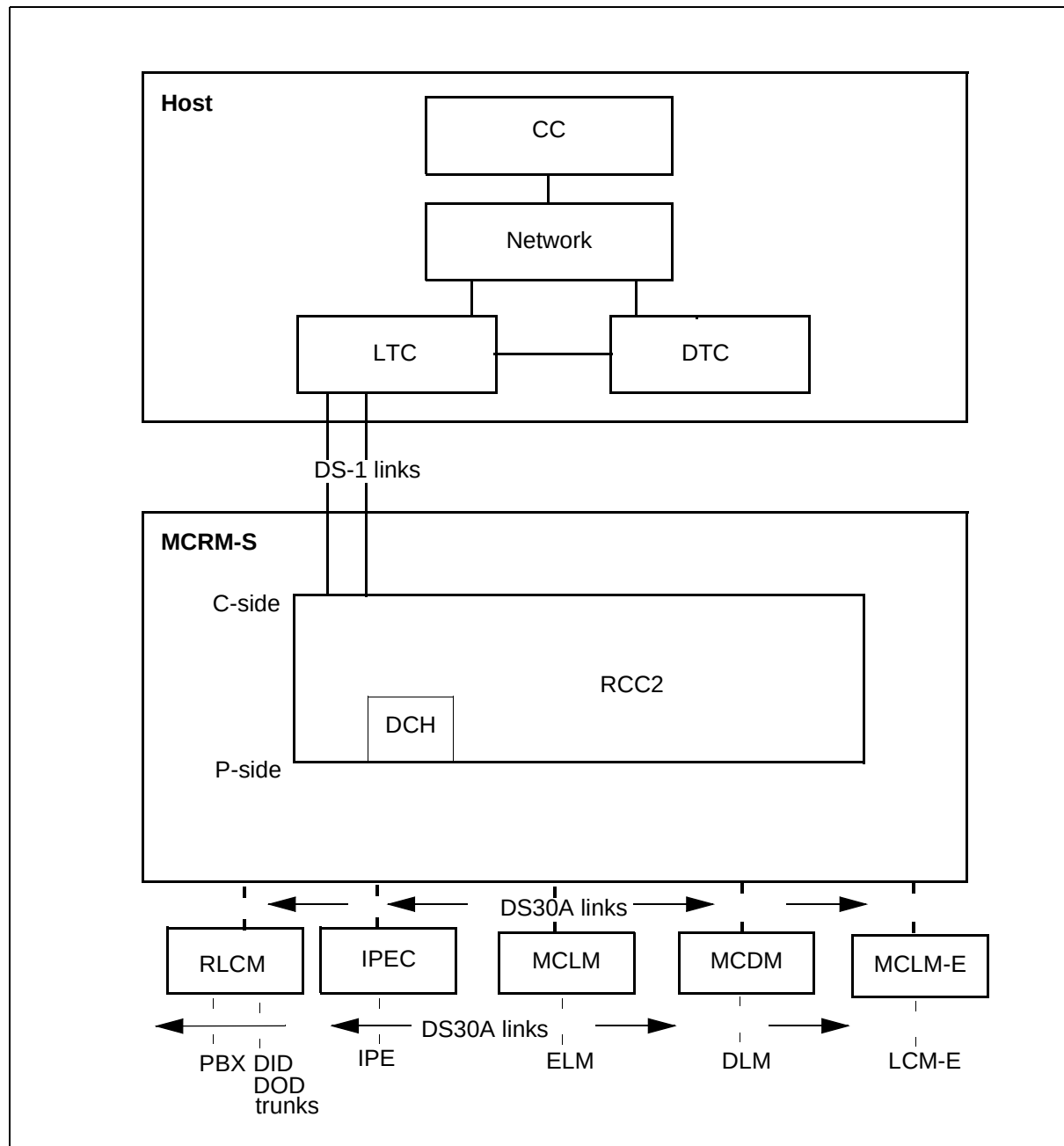
Figure 187 Single-cabinet ISDN-capable MCRM-S configuration
