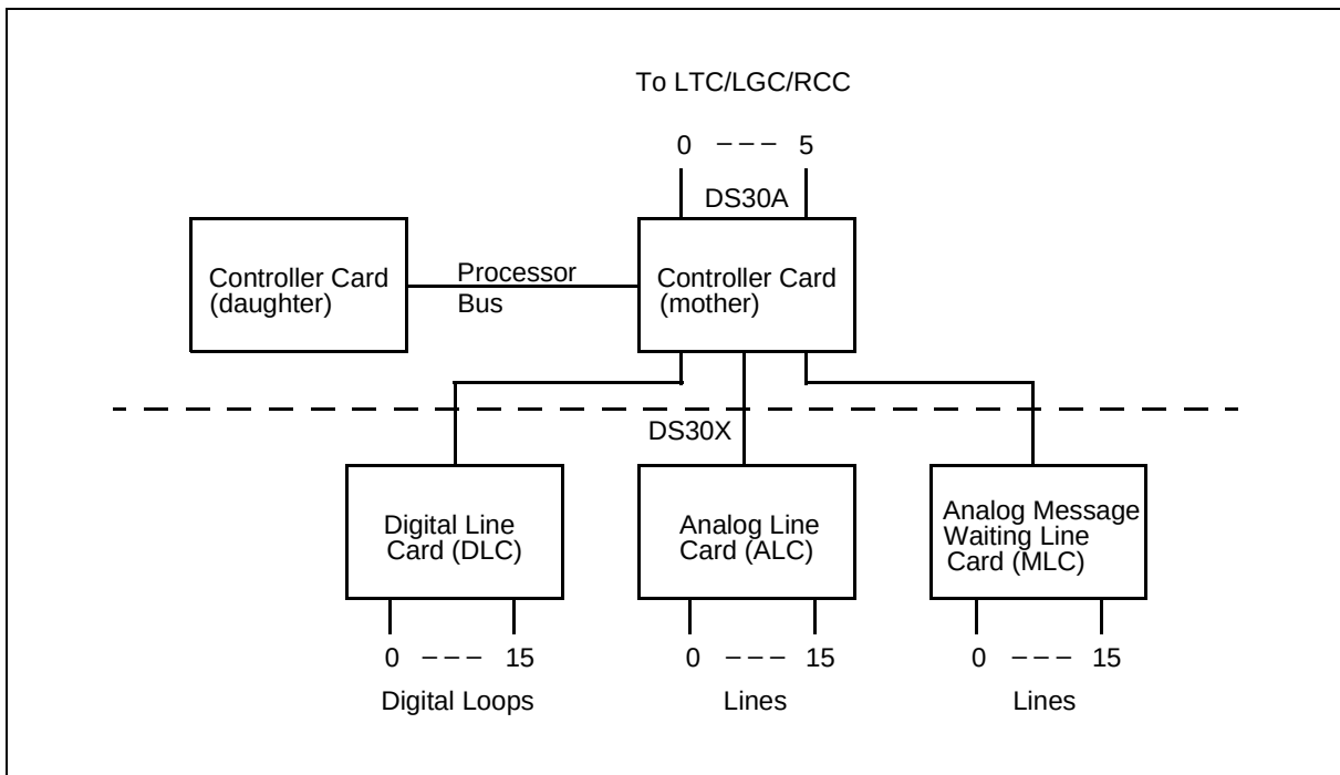
Figure 179 IPE schematic
