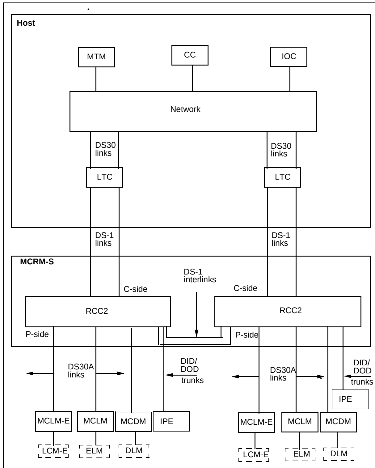
Figure 185 Multicabinet MCRM-S in the DMS network
