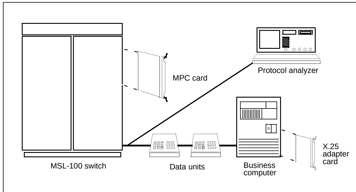
Figure 191 Meridian SCAI hardware components
