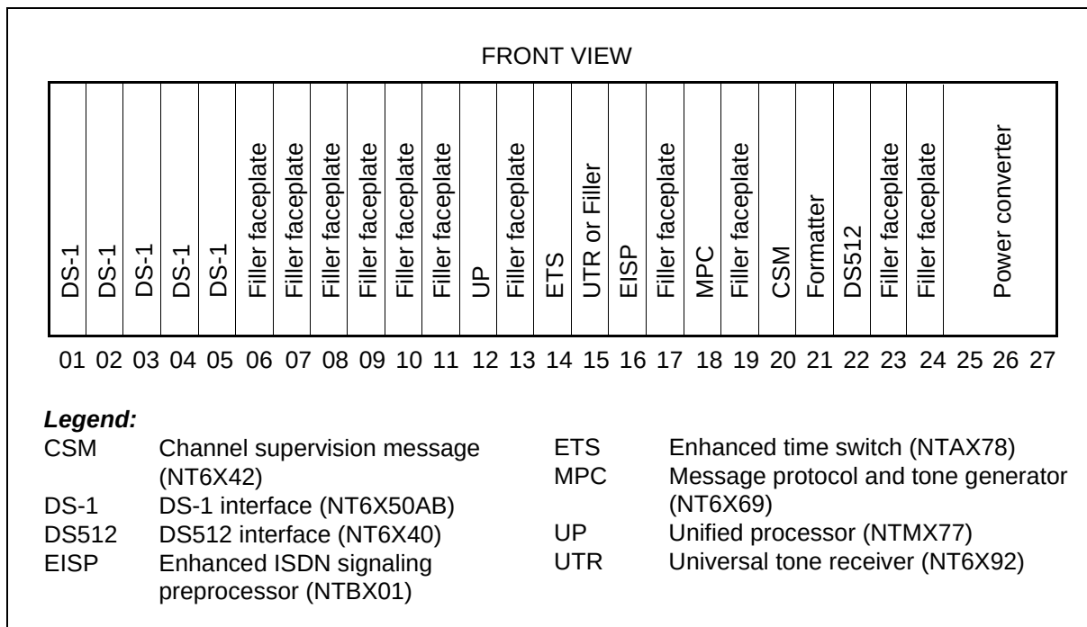
Figure 175 DTCI shelf layout for DWS in an XPM PLUS configuration
