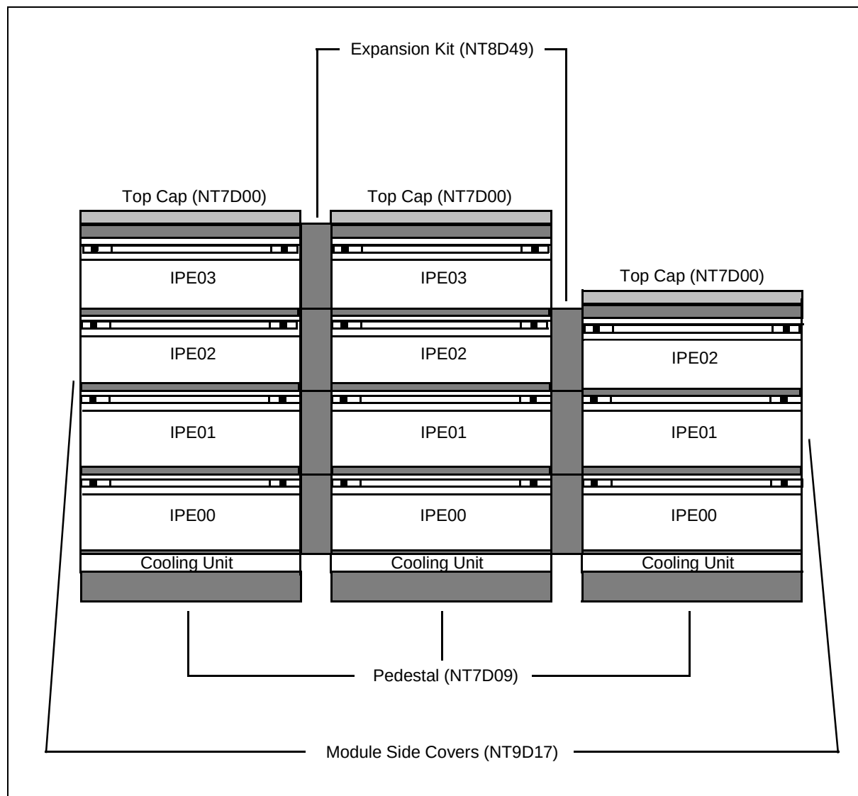
Figure 180 Standard growth configuration
