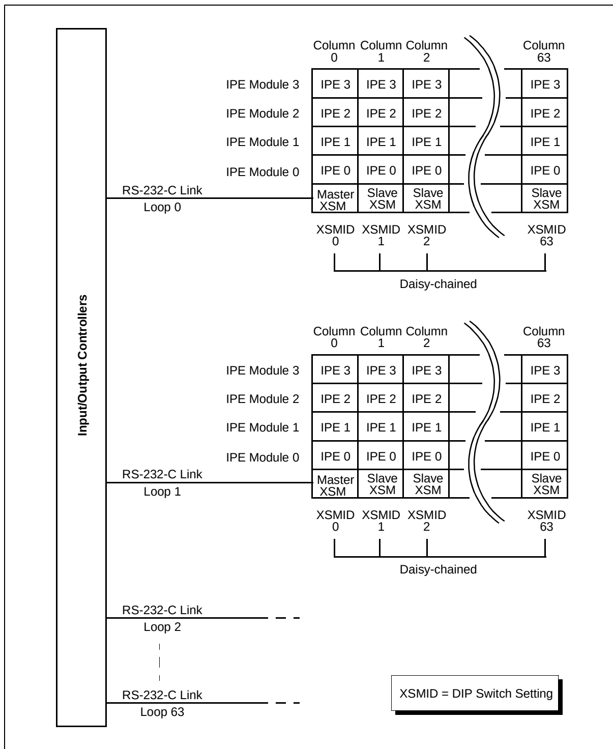
Figure 183 Relationship of XSM loop to XSMID and modules
