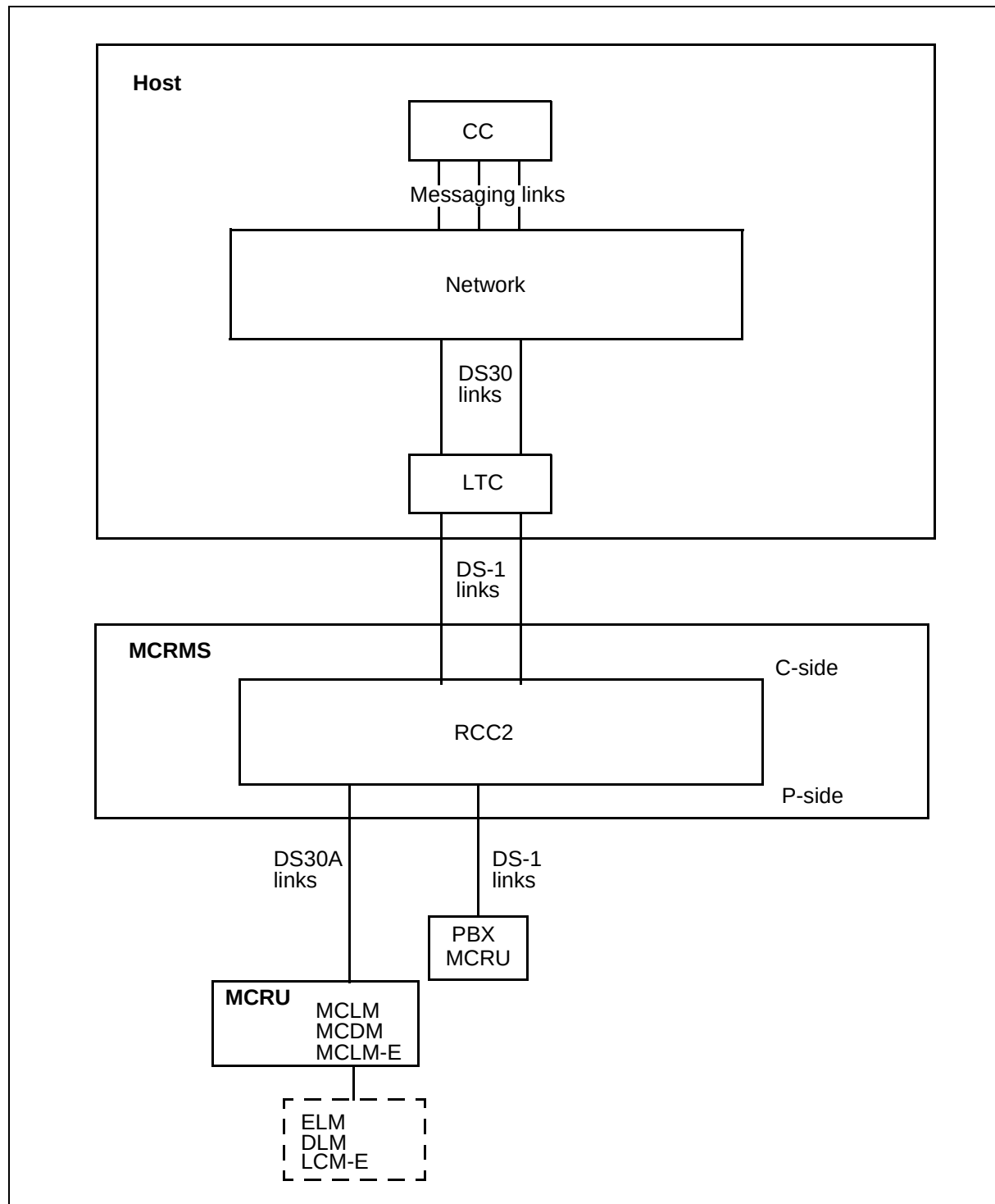
Figure 184 Single RCC2 MCRM-S in the DMS network
