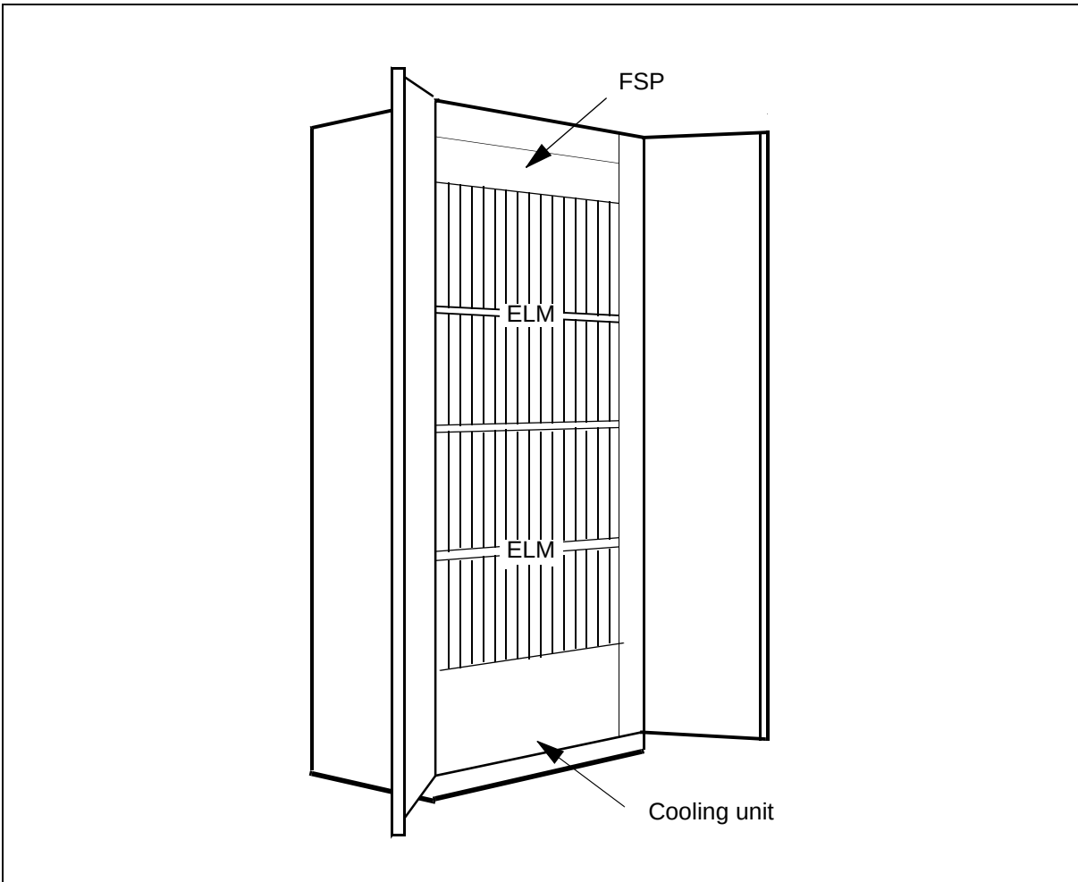
Figure 189 MCLM cabinet
