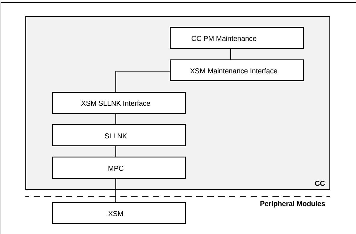
Figure 182 XSM-to-SLLNK interface
