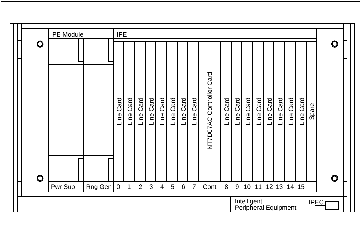
Figure 178 IPE shelf card slots
