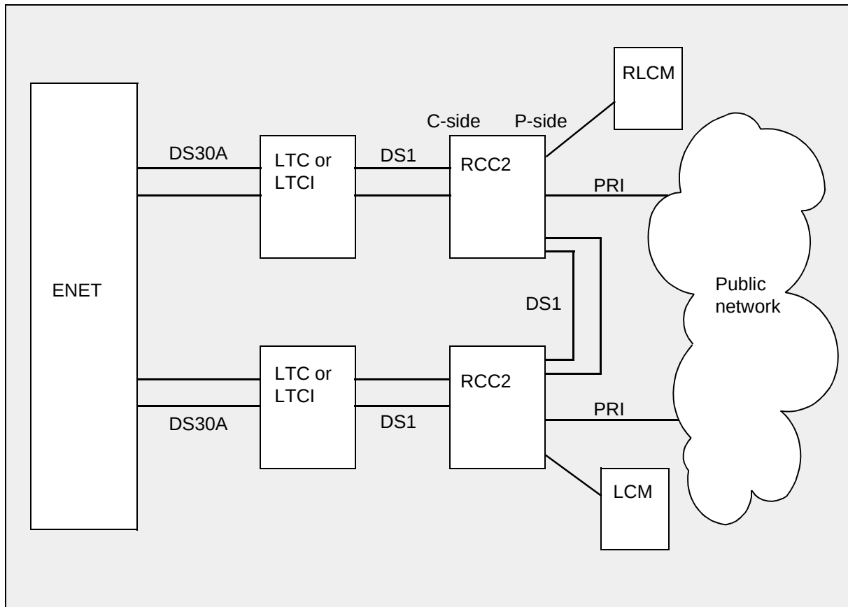
Figure 149 Dual RCC2 configuration
