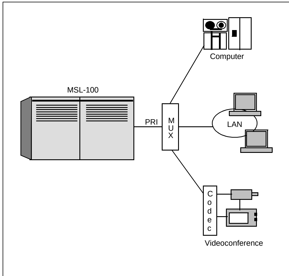
Figure 171 DWS shared access
