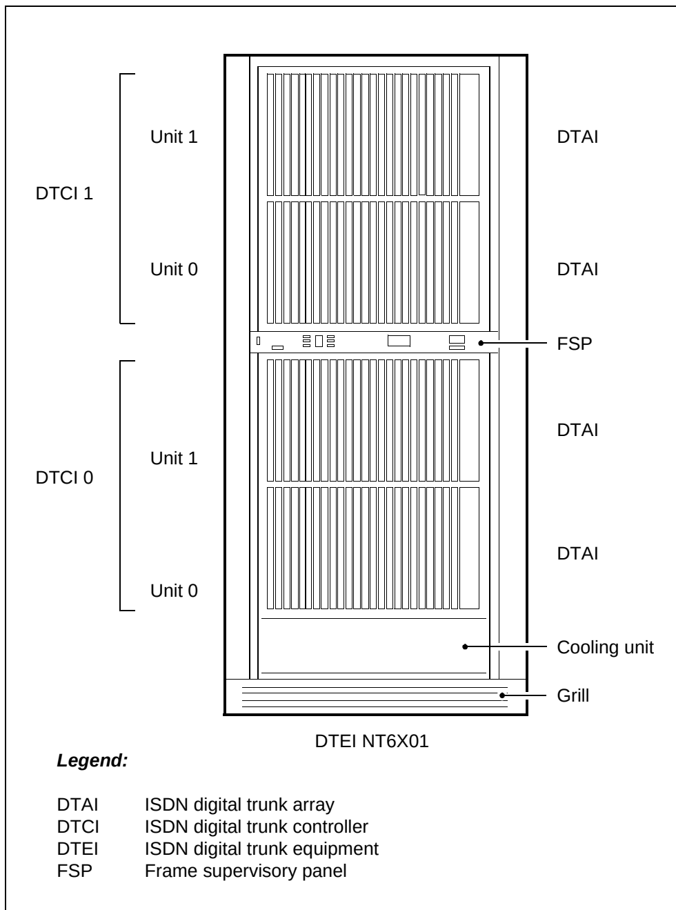
Figure 174 ISDN digital trunk controller equipment (DTEI) frame NT6X01
