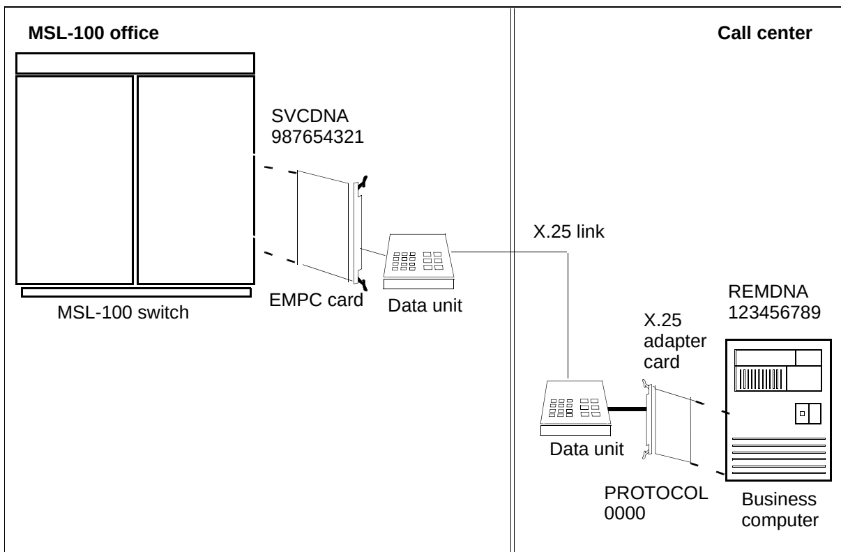
Figure 114 Point-to-point configuration
