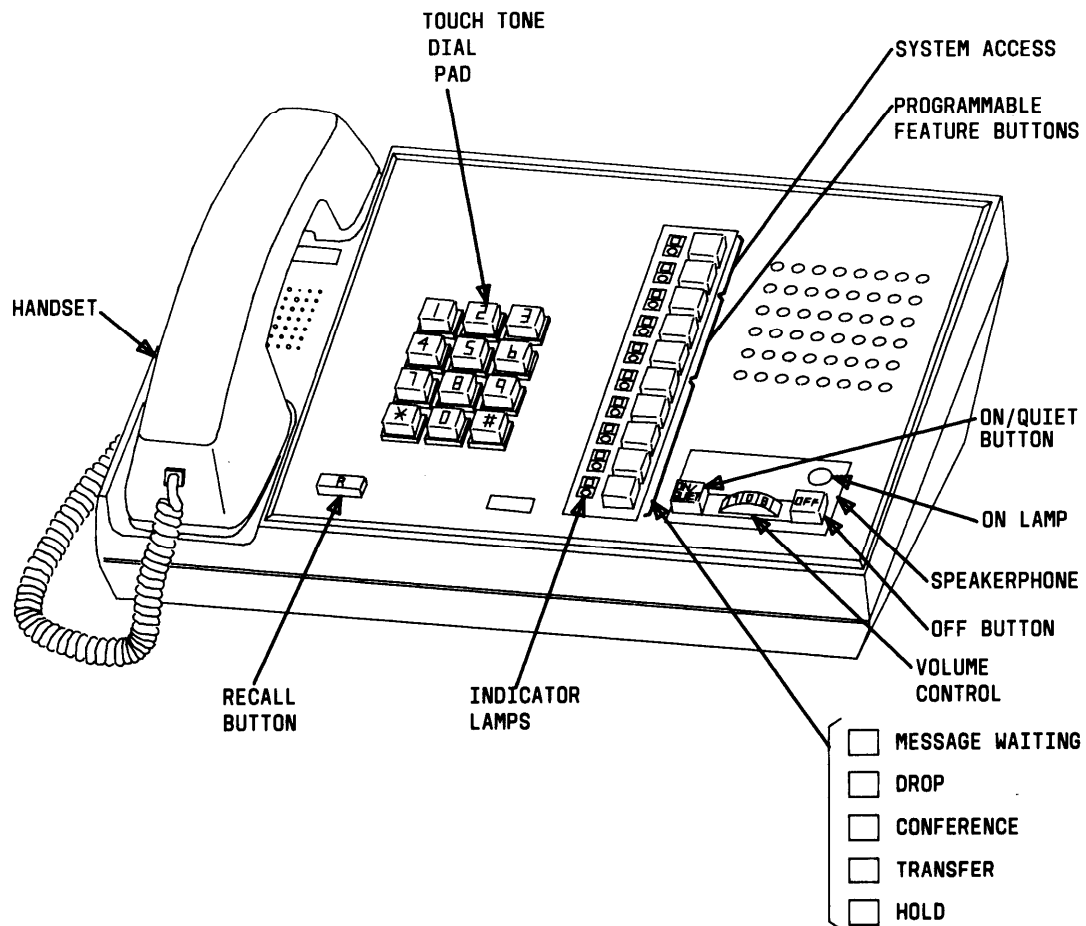
Figure 4-20. 10-Button MET With Built-In Speakerphone (2993C04)
