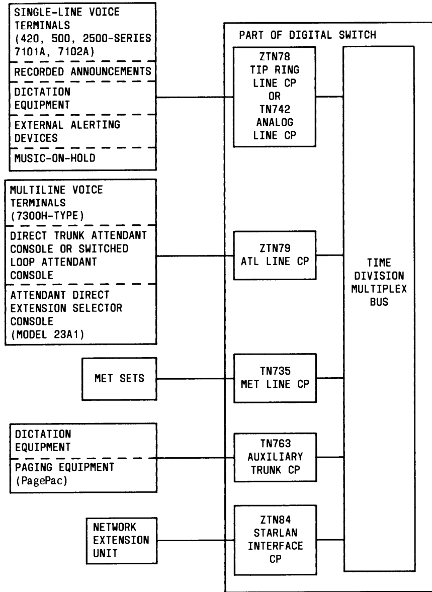
Figure 3-5. Equipment Connections Via Circuit Pack Ports (Sheet 3 of 3)
