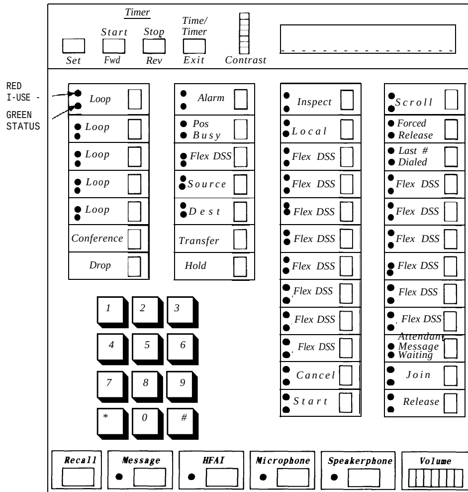
Figure 2-4. Buttons and Display of BIS-34D
