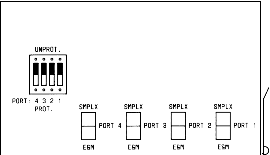
Figure 3-16. Tie Trunk (TN760B) Circuit Pack Option Switches
