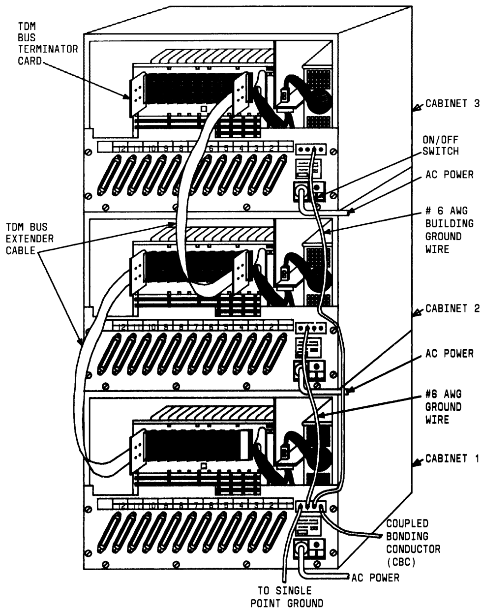
Figure 3-4. TDM Bus-Three Cabinet System
