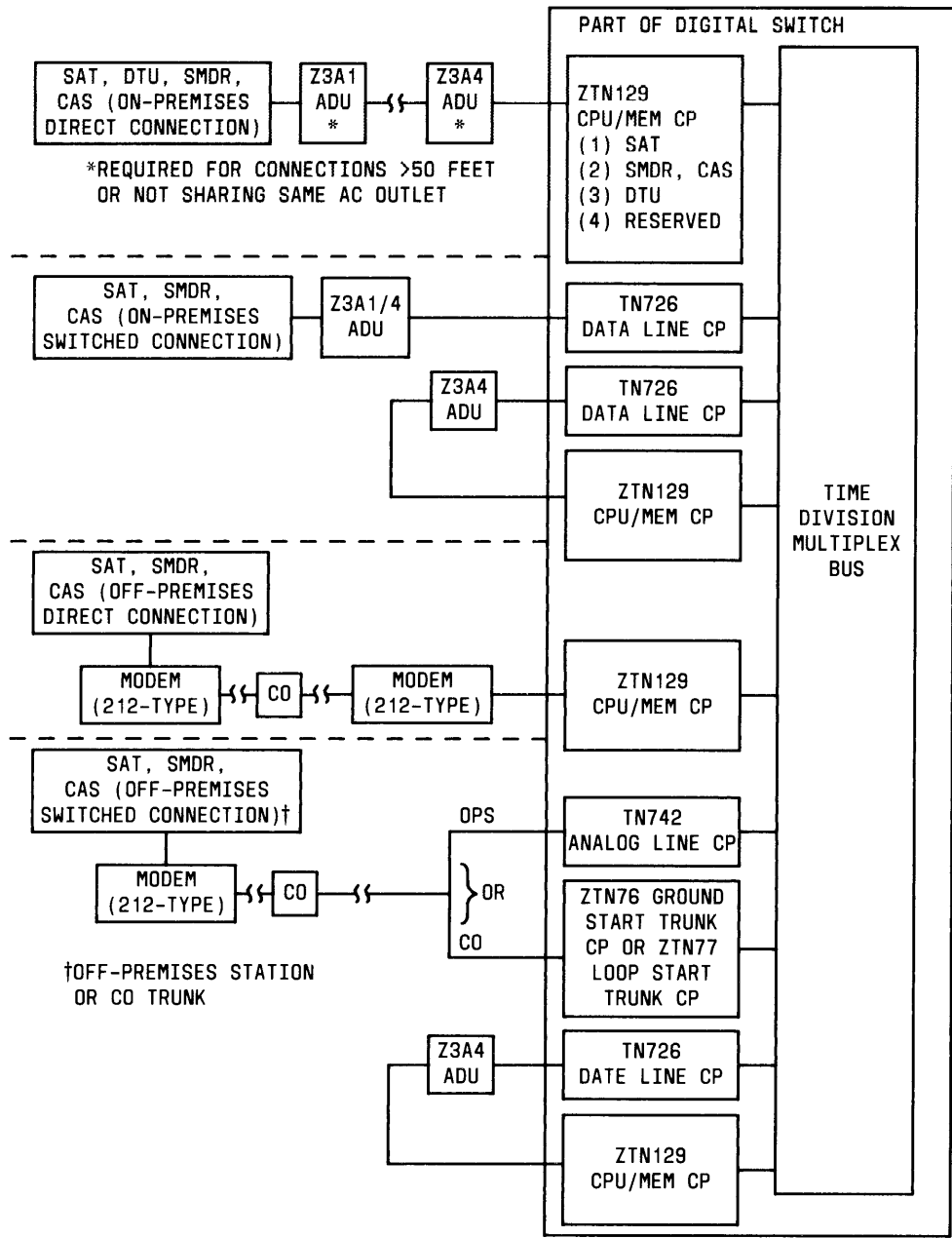
Figure 3-5. Equipment Connections Via Circuit Pack Ports (Sheet 2 of 3)
