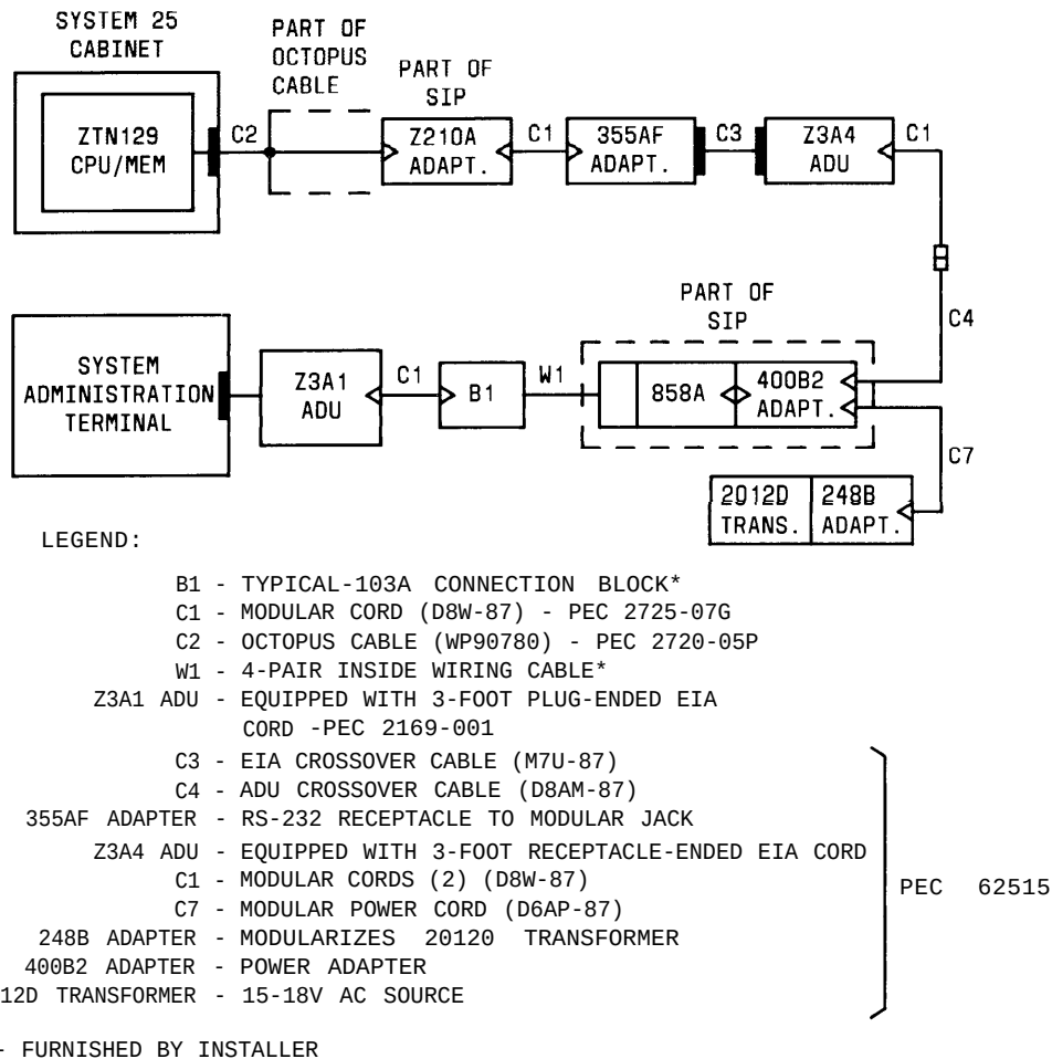
Figure 2-51. SAT On-Premises Direct Connections (Greater Than 50 Feet From System Cabinet or Nonsharing Same AC Outlet)
