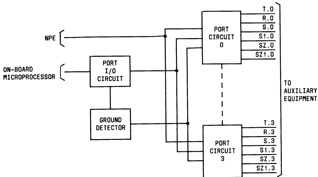
Figure 3-9. Auxiliary Trunk (TN763) Unique Circuitry
