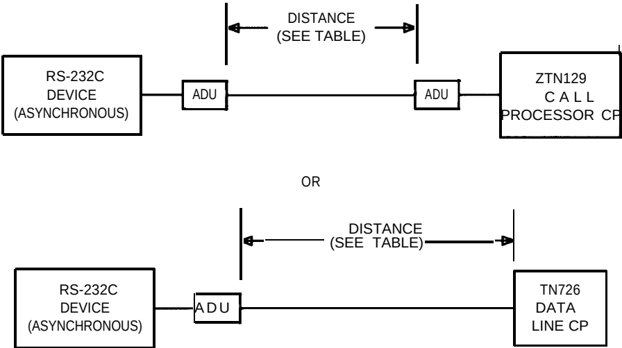
Figure 5-3. Asynchronous Data Unit Allowable Cable Distances (in-Building Only)
