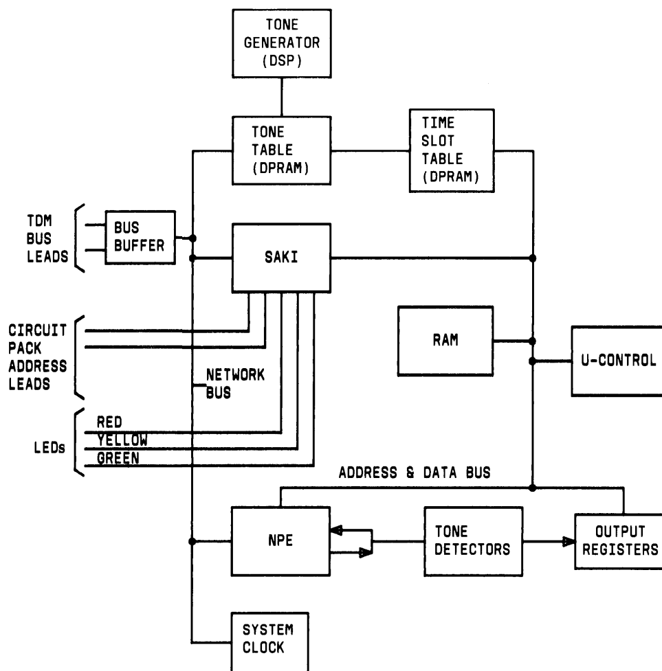
Figure 3-18. Service Circuit (ZTN85)
