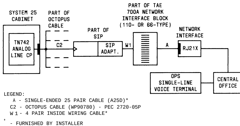
Figure 4-28. Off-Premises Station Single-Line Voice Terminal Connections
