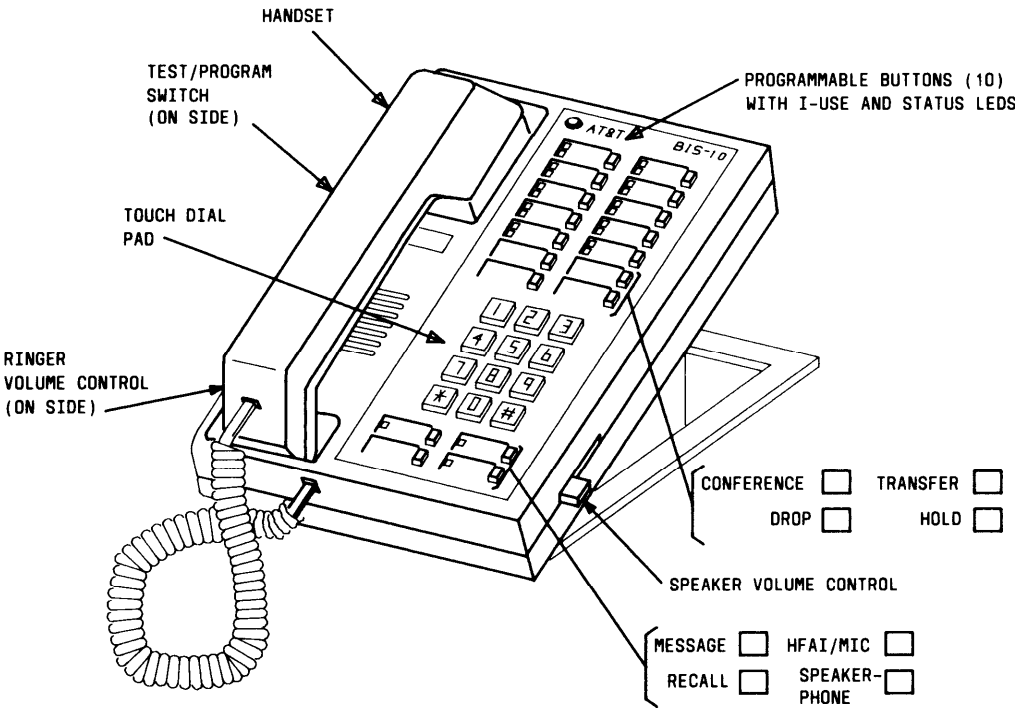
Figure 4-15. 7313H01A Voice Terminal (BIS-10)
