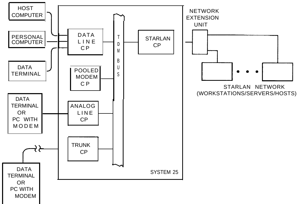
Figure 2-38. STARLAN NETWORK and System 25 Configuration
