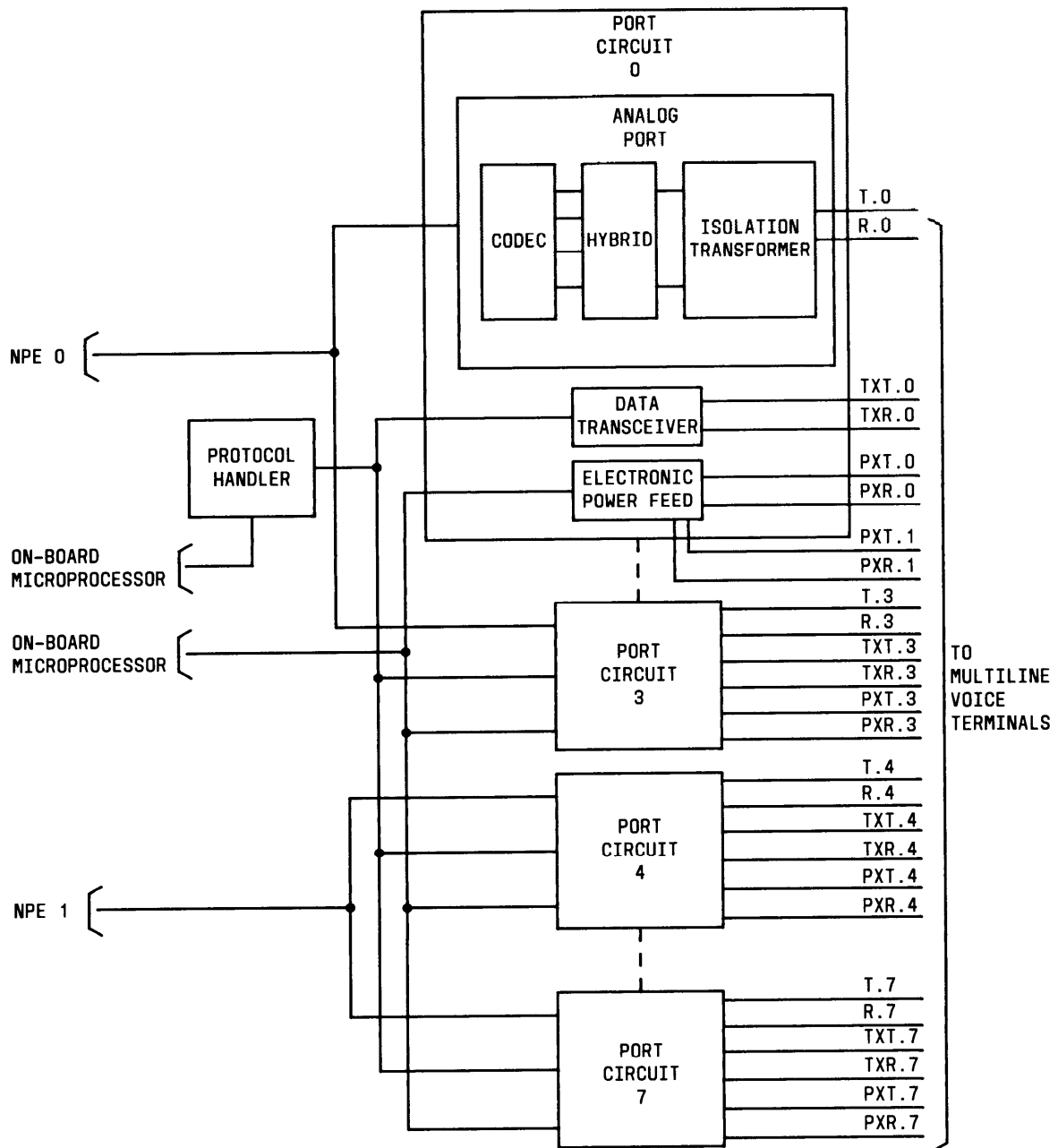
Figure 3-8. ATL Line (ZTN79) Unique Circuitry
