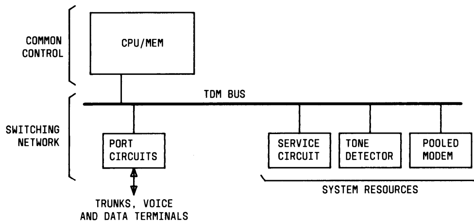
Figure 3-1. System 25 Digital Switch
