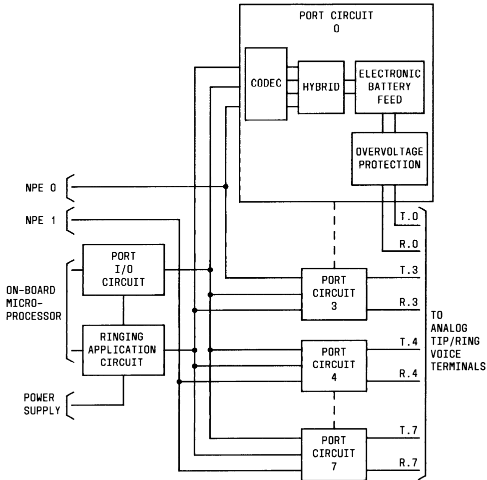
Figure 3-7. Analog Line (TN742) Unique Circuitry
