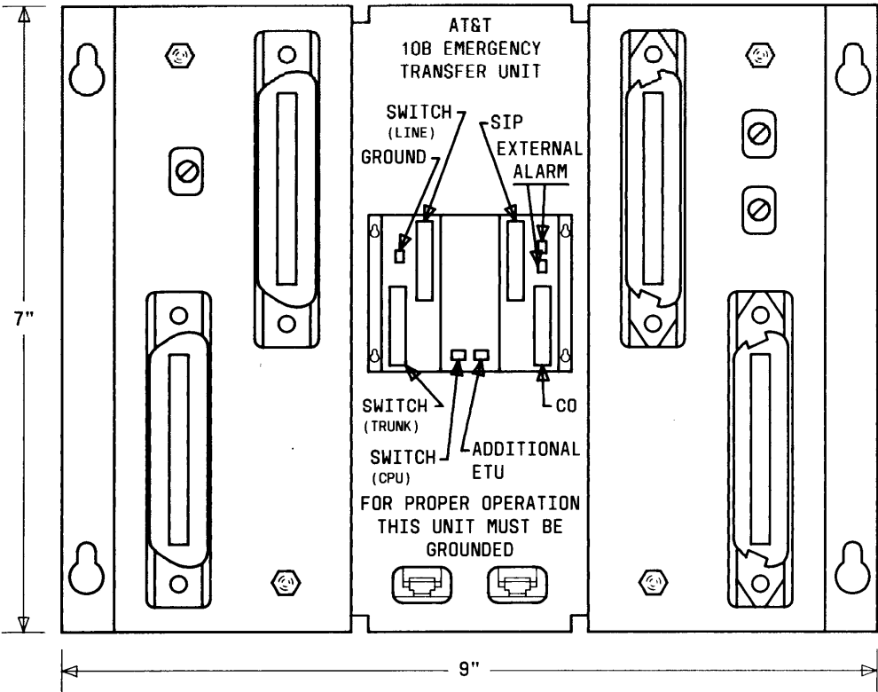
Figure 2-31. 10B Emergency Transfer Unit (ETU)
