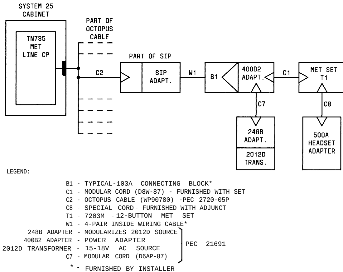
Figure 2-25. Typical Headset Adapter Connections For 12-Button MET Sets
