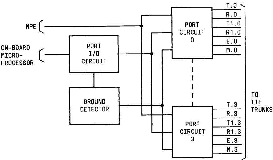
Figure 3-15. Tie Trunk (TN760B) Unique Circuitry
