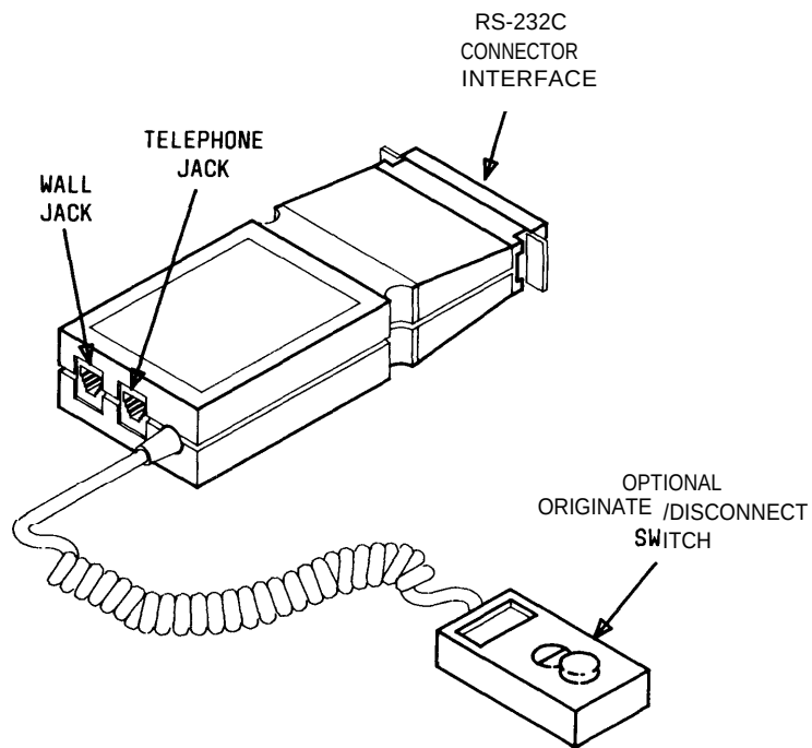
Figure 4-22. Asynchronous Data Unit (ADU)
