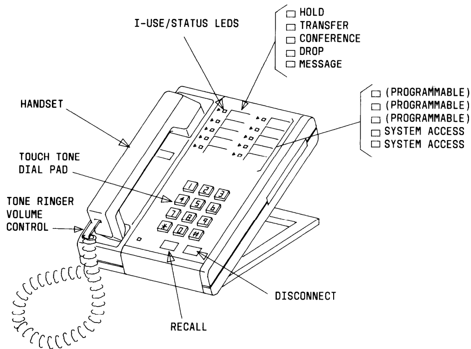
Figure 4-21. 12-Button MET Set (7203M)
