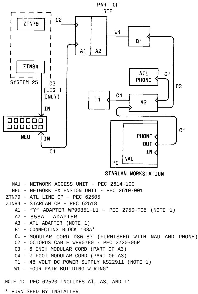
Figure 2-40. STARLAN NETWORK Connection to System 25 (With ATL-Type Telephone)
