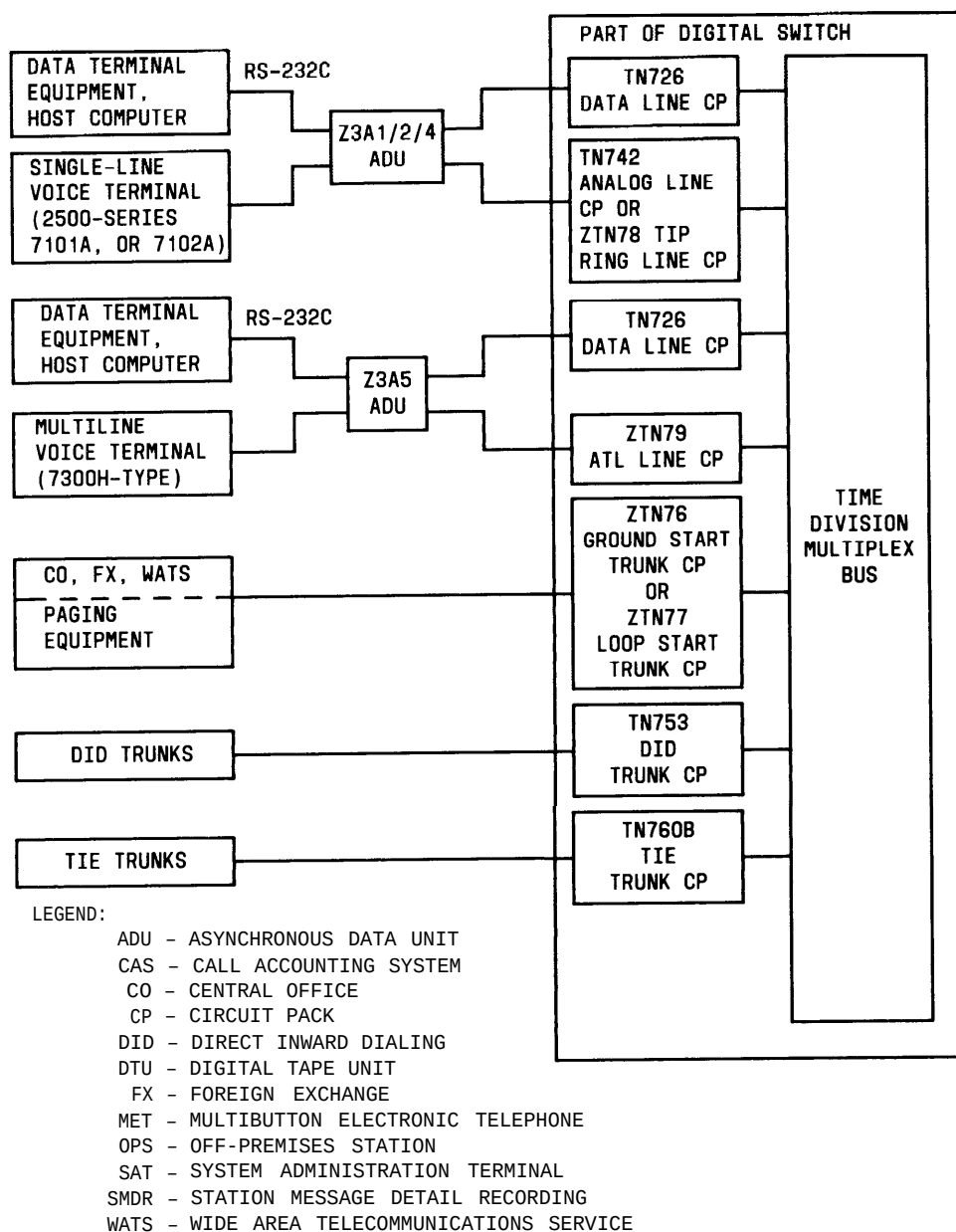
Figure 3-5. Equipment Connections Via Circuit Pack Ports (Sheet 1 of 3)
