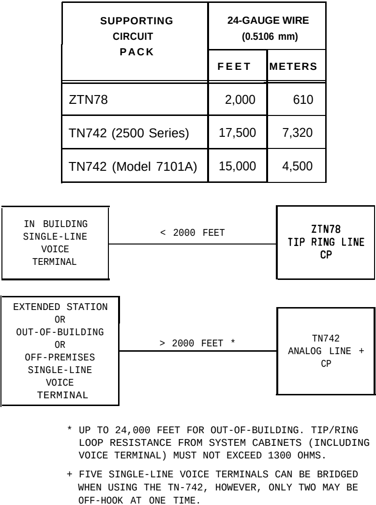
Figure 5-1. Single-Line Voice Terminal Allowable Cable Distances
