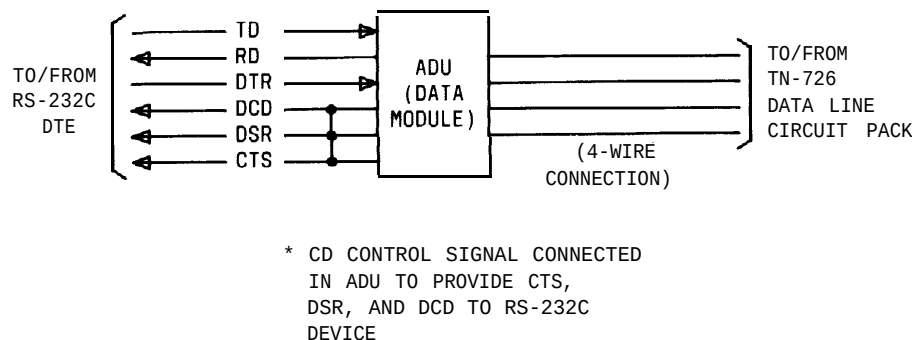
Figure 2-14. Asynchronous Data Unit Interface Signals
