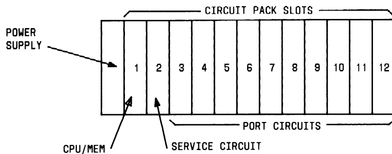
a) CABINET 1 - (MOUNTING FOR CONTROL &amp; PORT CIRCUIT PACKS)
