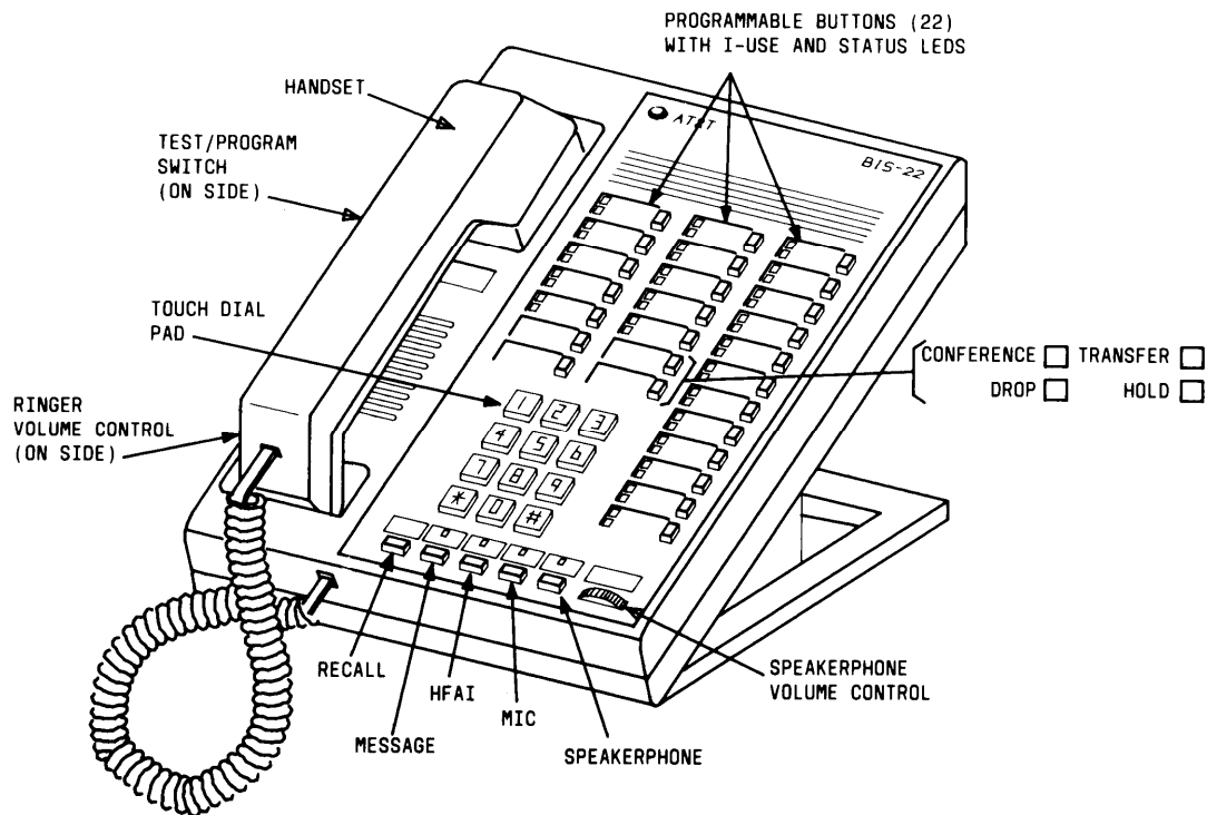
Figure 4-16. 7314H01A Voice Terminal (BIS-22)
