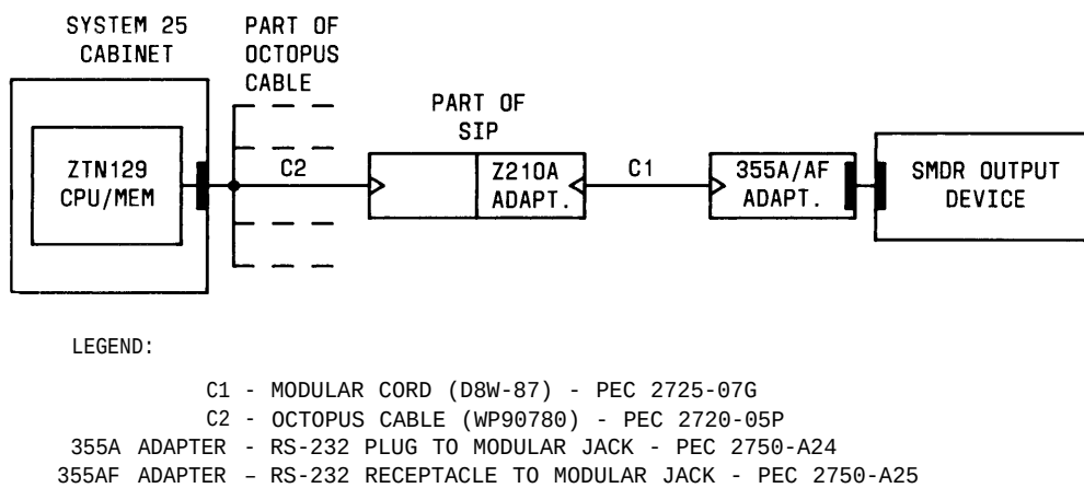
Figure 2-44. SMDR Output Equipment—On-Premises Direct Connections (Sharing Same AC Outlet)
