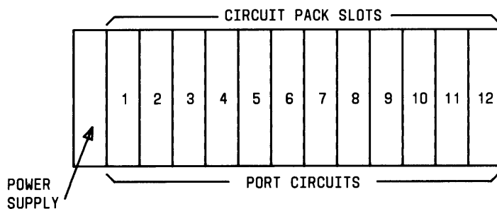
(b) CABINET 2 OR 3 - (MOUNTING FOR PORT CIRCUIT PACKS)
