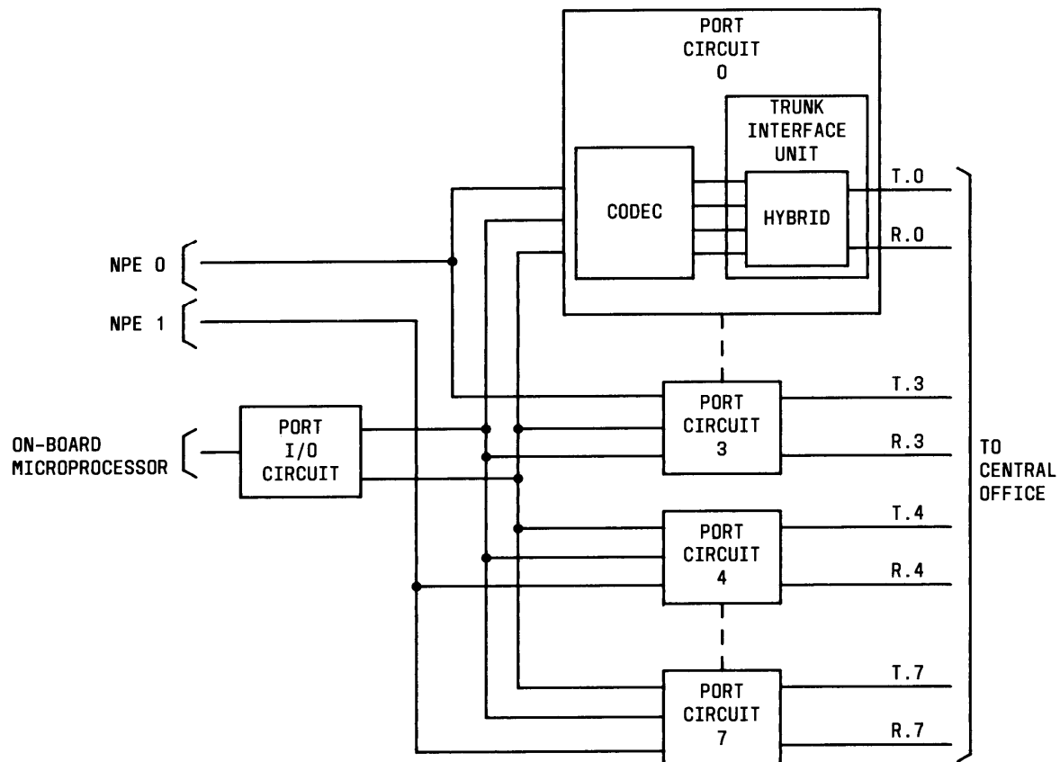
Figure 3-11. DID Trunk (TN753) Unique Circuitry
