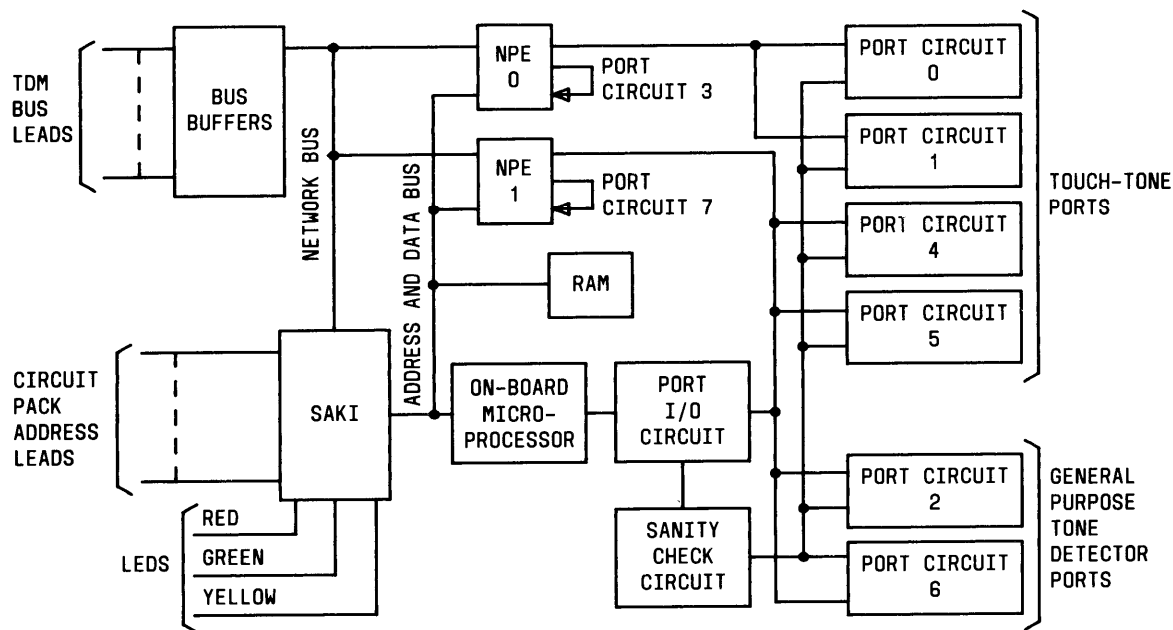
Figure 3-19. Tone Detector (TN748B)
