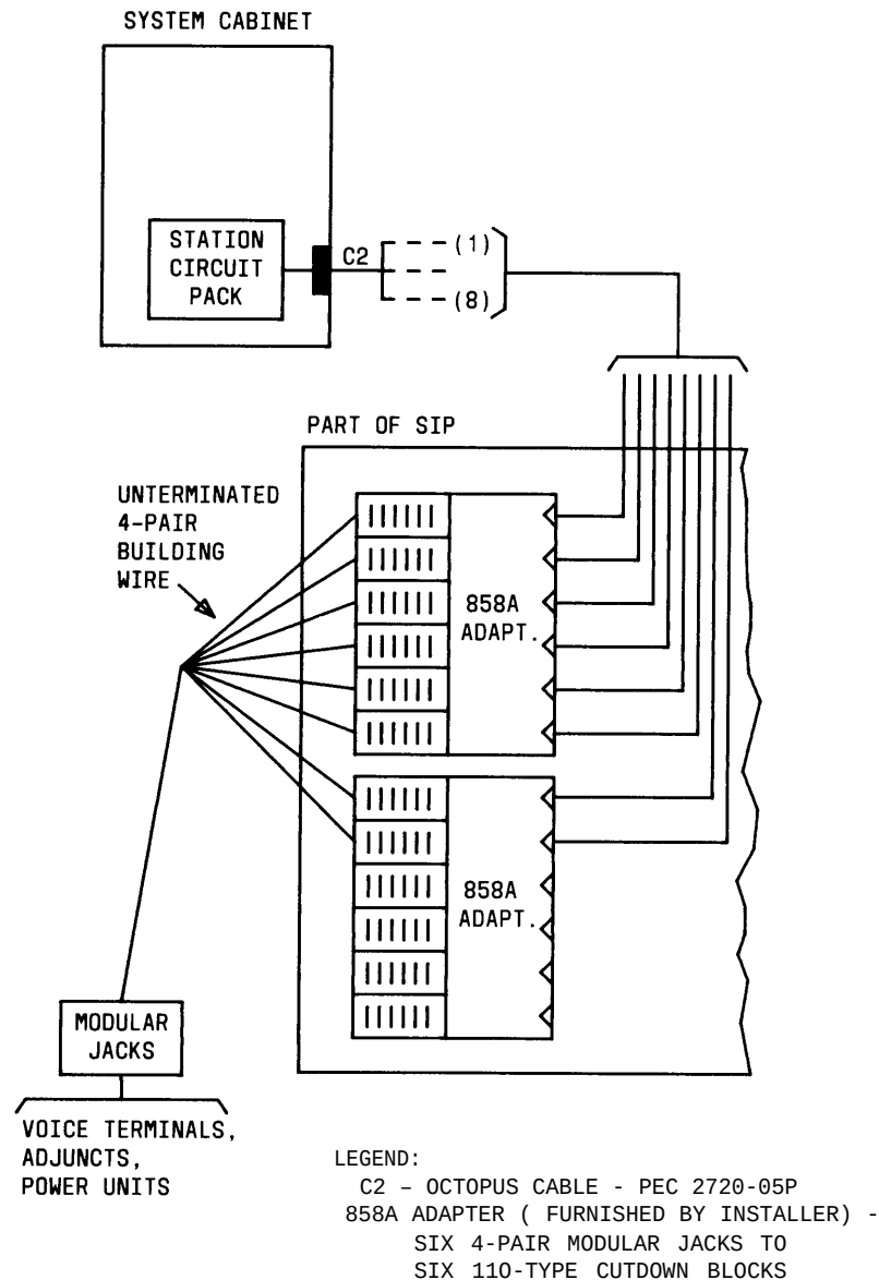
Figure 4-25. Typical SIP Connections
