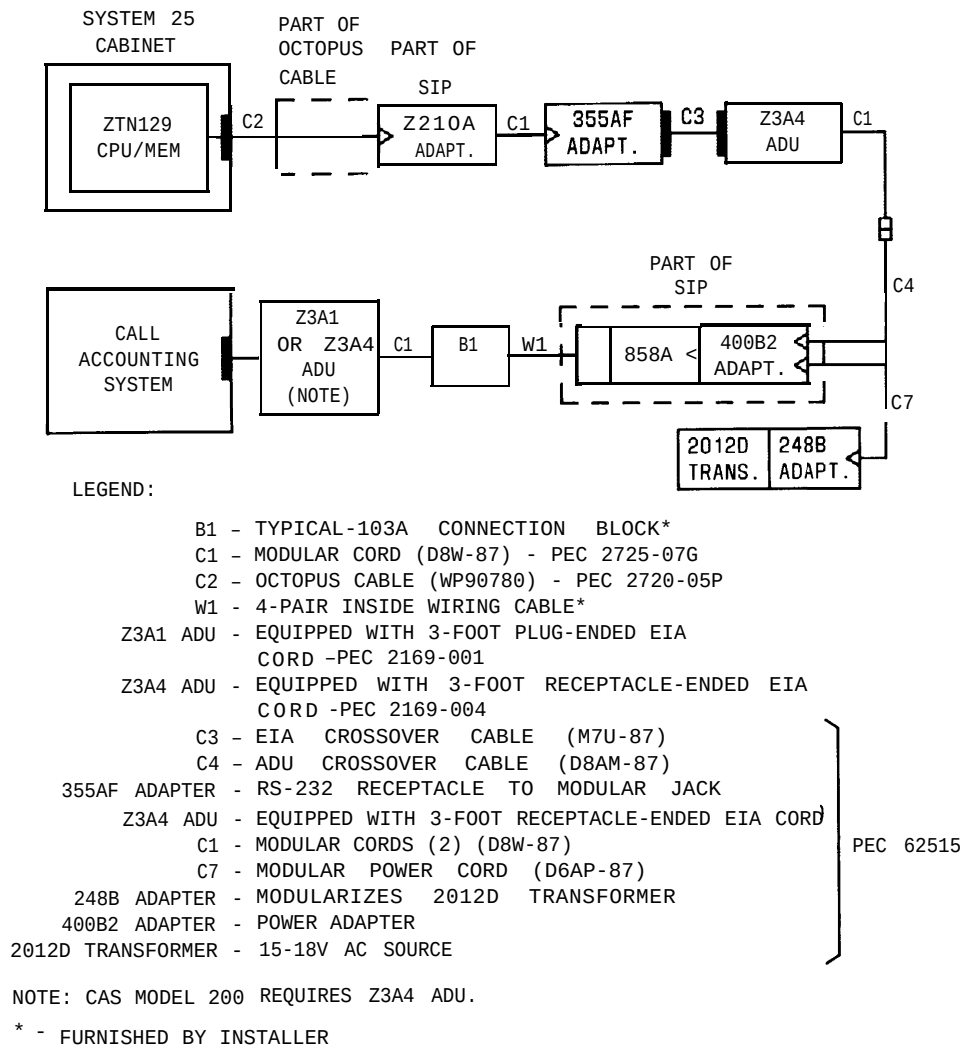
Figure 2-12. Call Accounting System—On-Premises Direct Connections (Greater Than 50 Feet From System Cabinet or Nonsharing Same AC Outlet)
