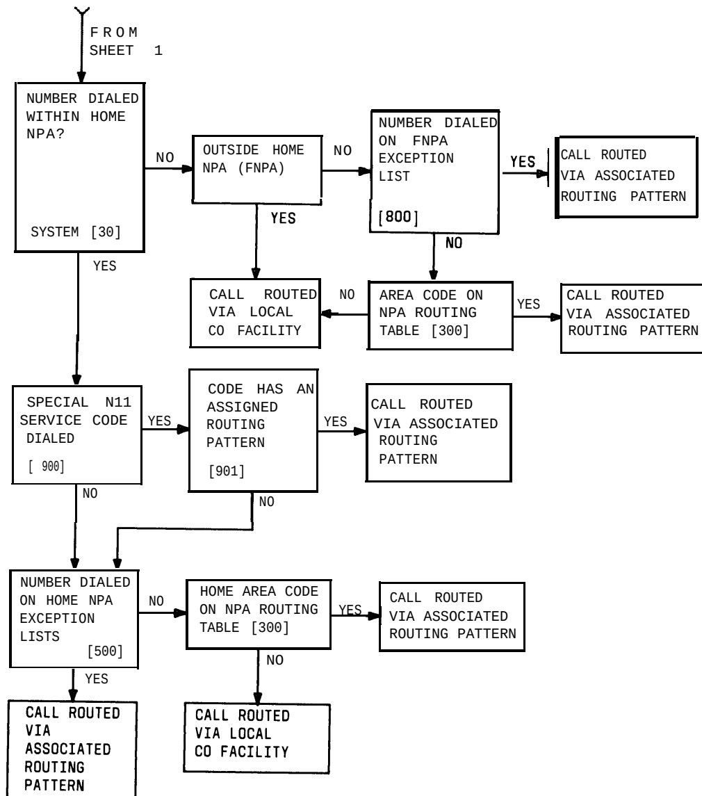
Figure 2-8. Automatic Route Selection Flow Chart (Sheet 2 of 2)
