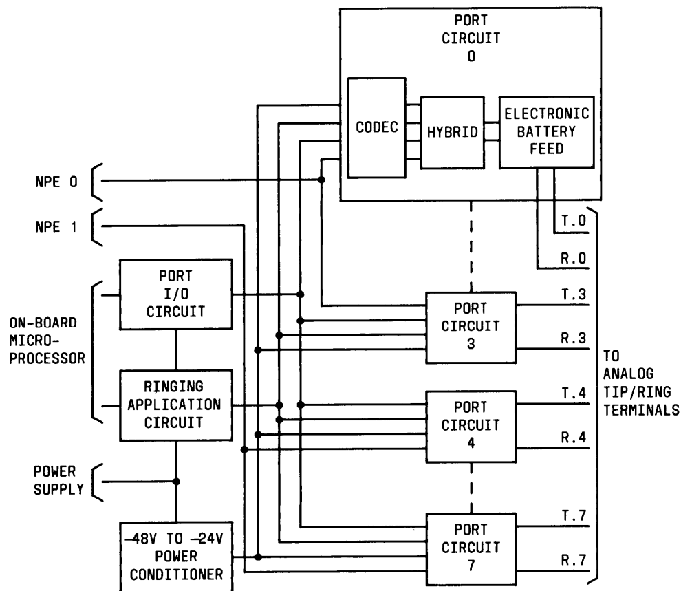
Figure 3-17. Tip Ring Line (ZTN78) Unique Circuitry
