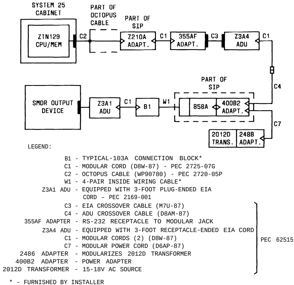
Figure 2-45. SMDR Output Equipment—On-Premises Direct Connections (Greater Than 50 Feet From System Cabinet or Nonsharing Same AC Outlet)
