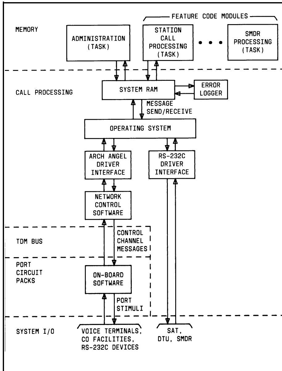
Figure 3-21. System Software Partitioning
