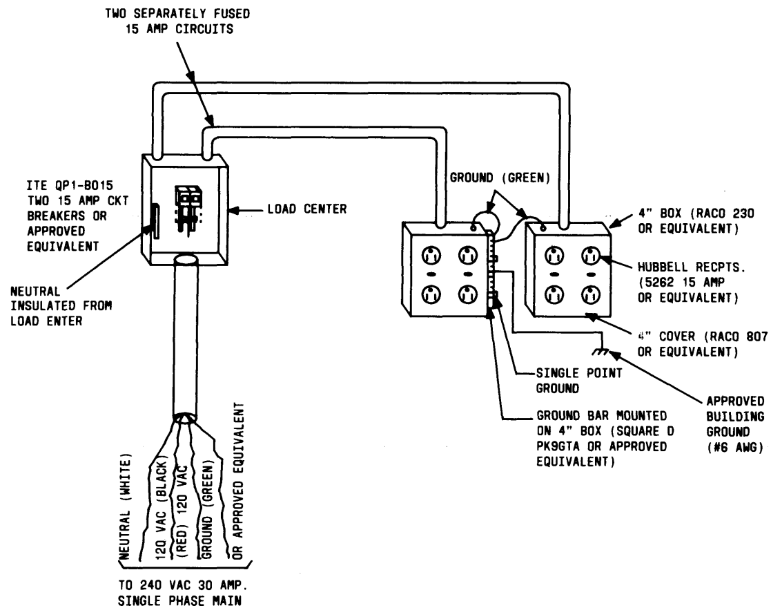
Figure 6-3. AC Power Distribution - Multiple Cabinet System
