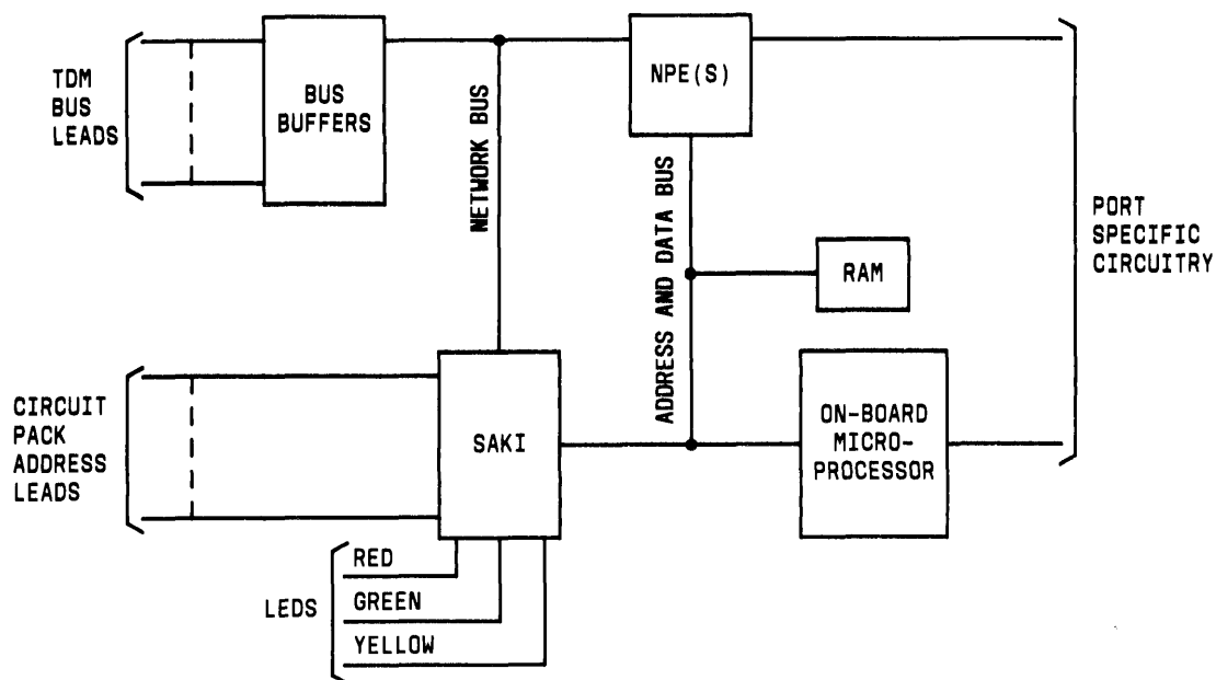
Figure 3-6. Port Circuit Pack Common Circuitry
