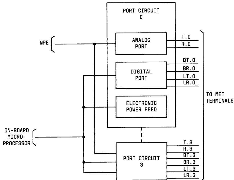
Figure 3-14. MET Line (TN735) Unique Circuitry
