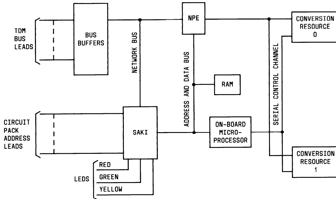
Figure 3-20. Pooled Modem (TN758)
