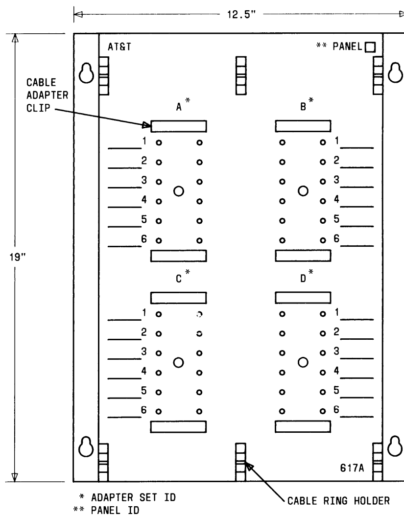
Figure 4-24. 617A Panel
