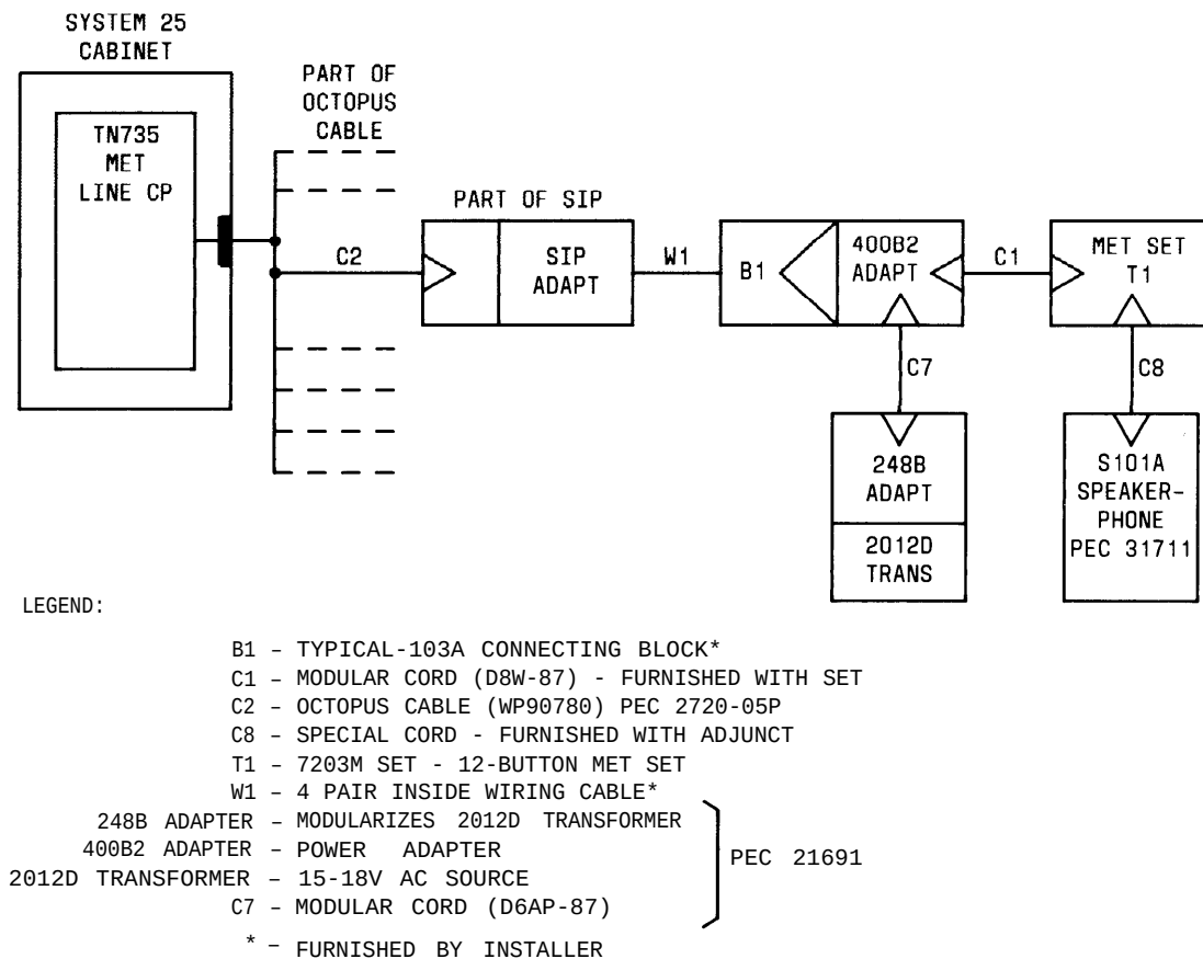
Figure 2-37. Speakerphone Connections For 12-Button MET Sets
