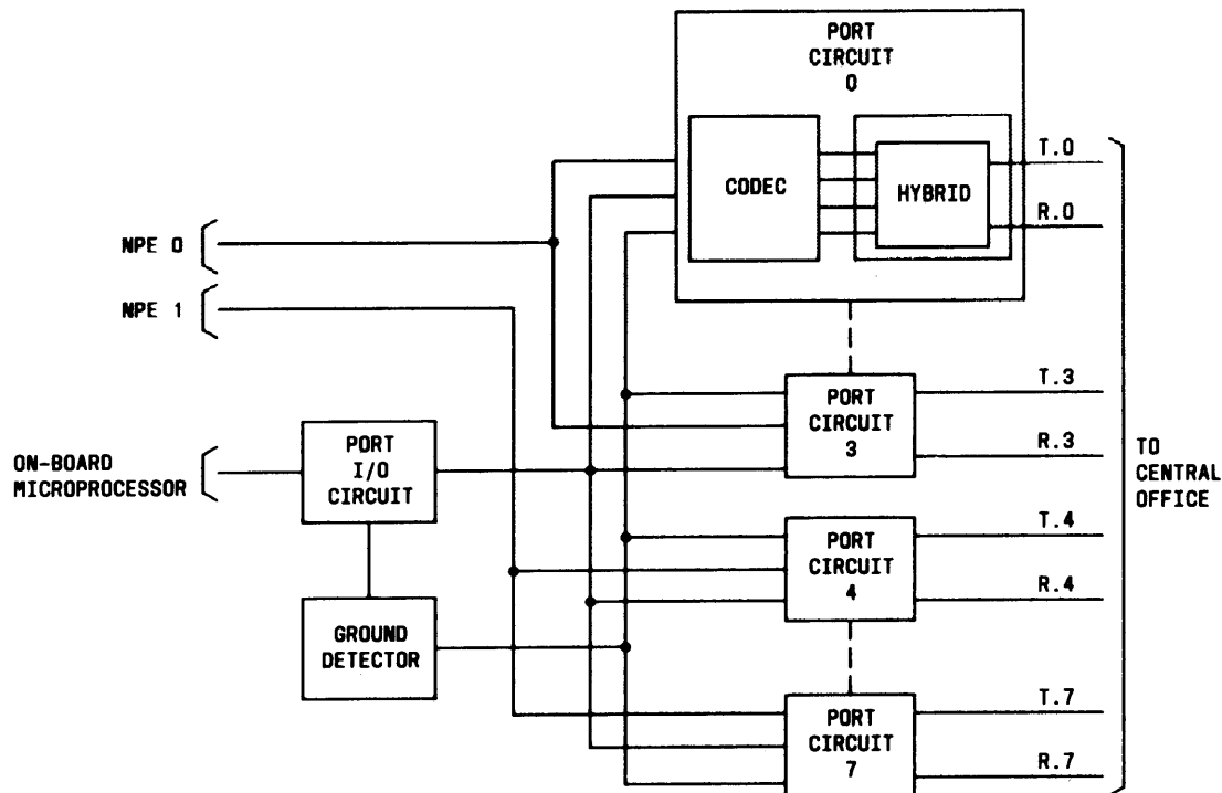
Figure 3-12. Ground Start Trunk (ZTN76) Unique Circuitry
