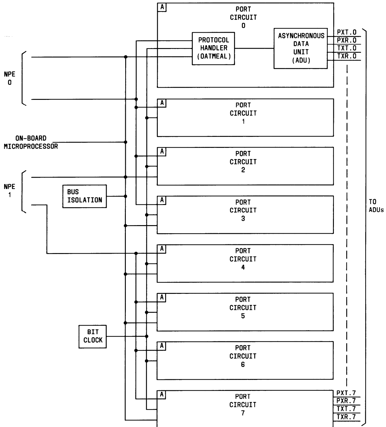
Figure 3-10. Data Line (TN726) Unique Circuitry
