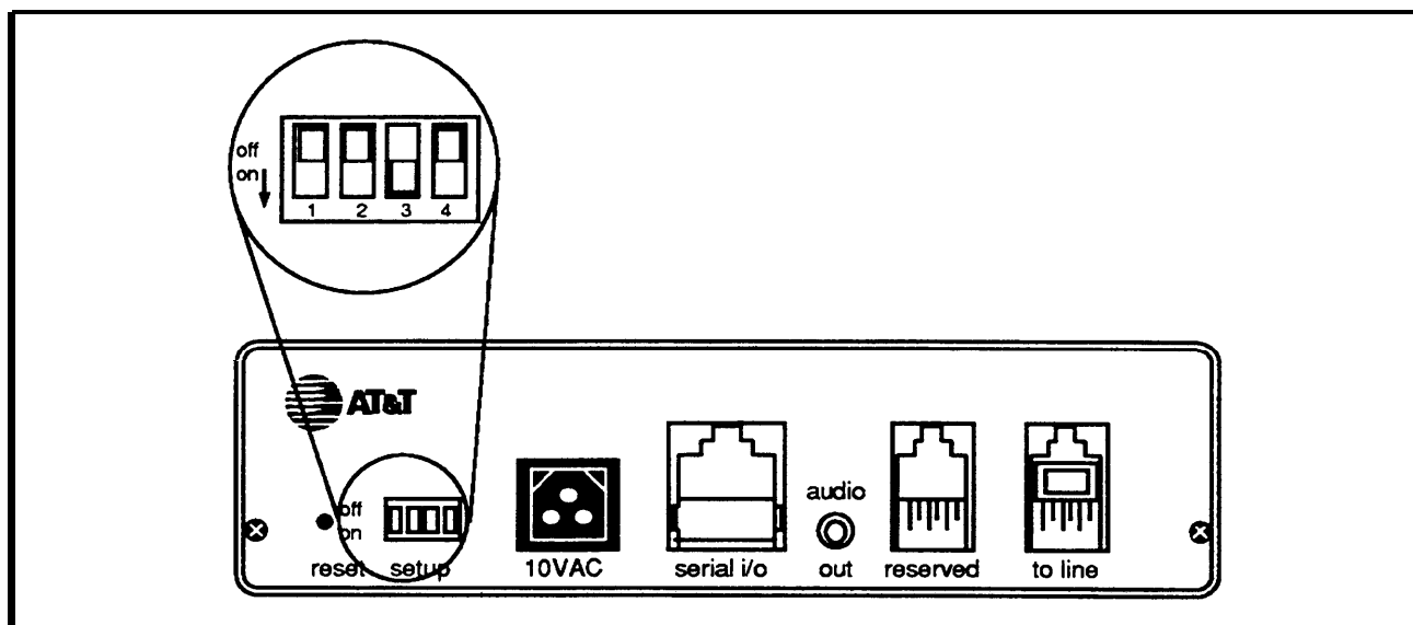
Figure 1-3 Setup Switch Positions for Installing Unit
