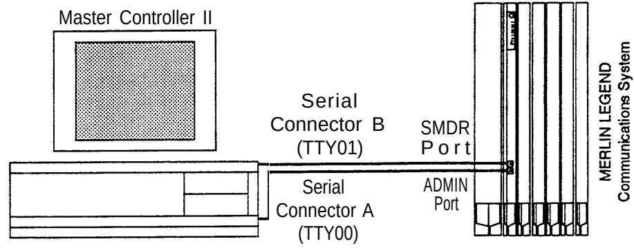
Figure 2-6. IS-II Hardware Connection
