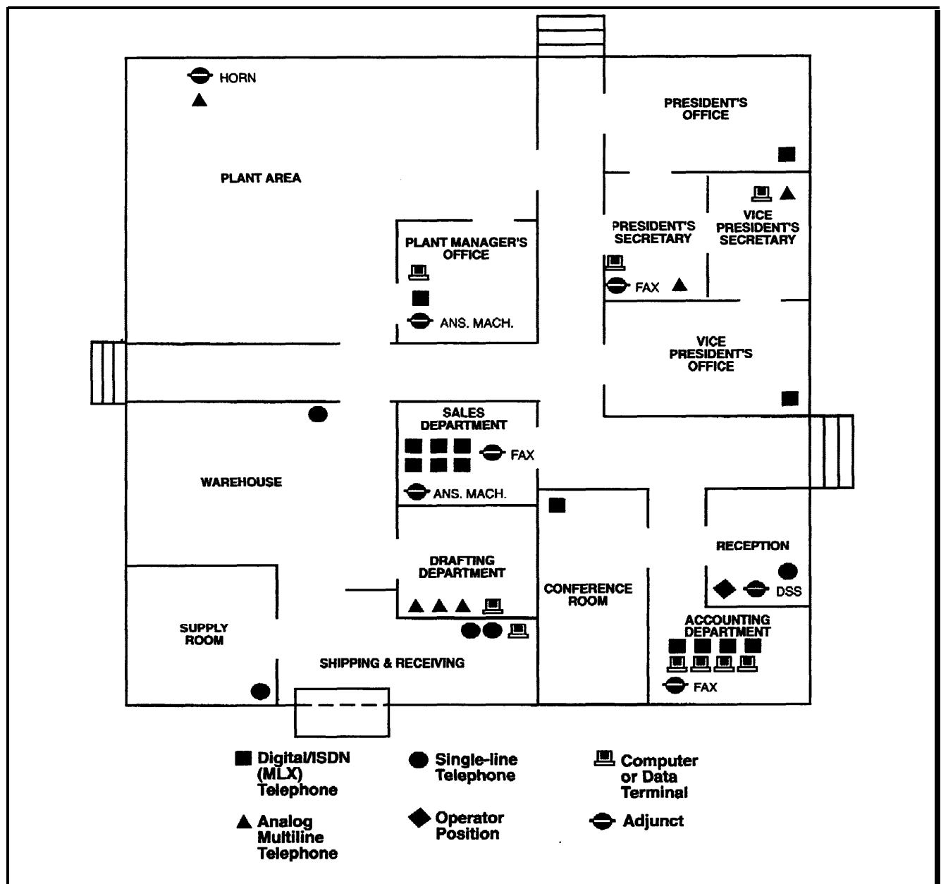
Figure 1-3 Floor Plan
