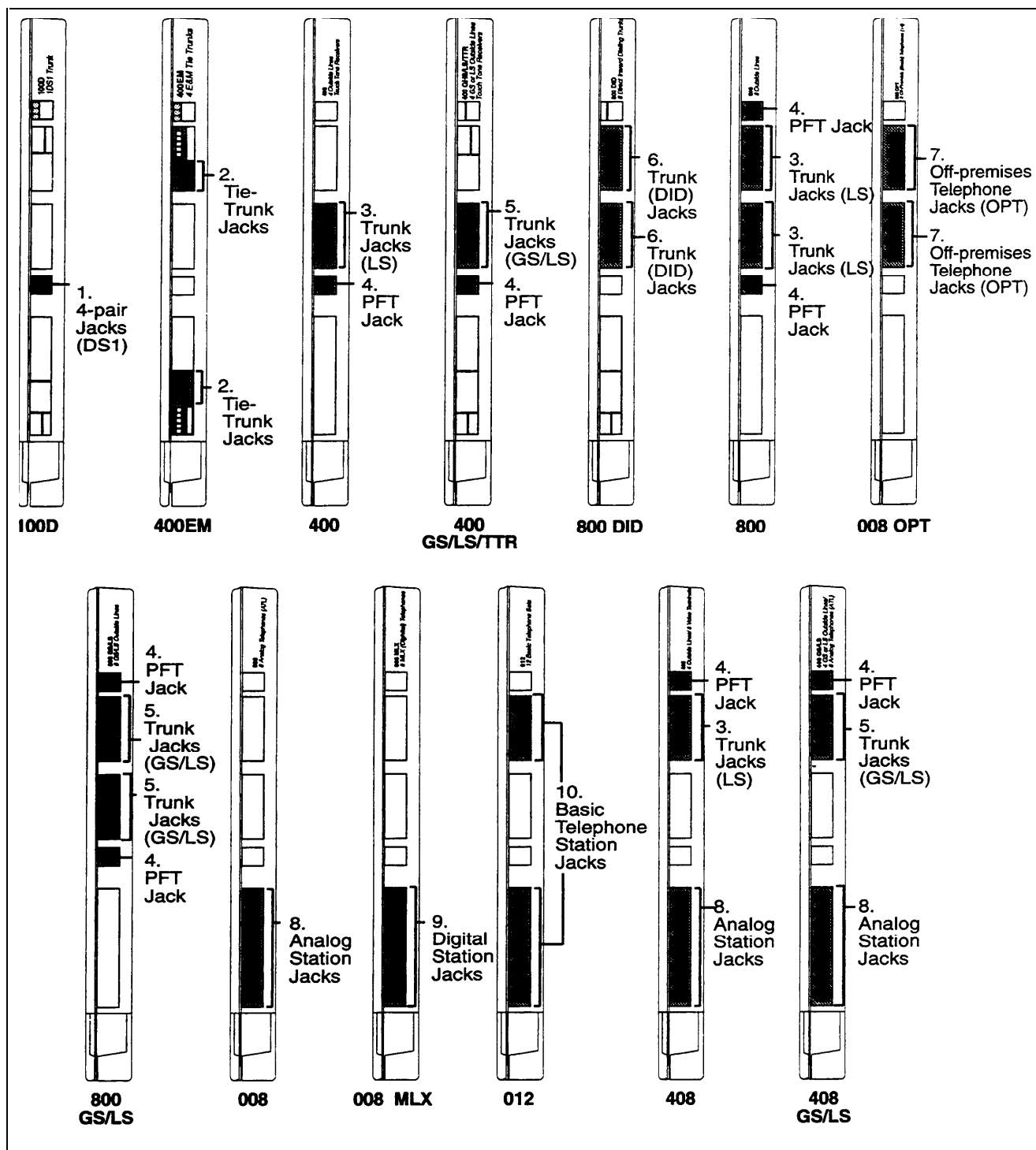
Figure 2-1 Trunk and Station Modules
