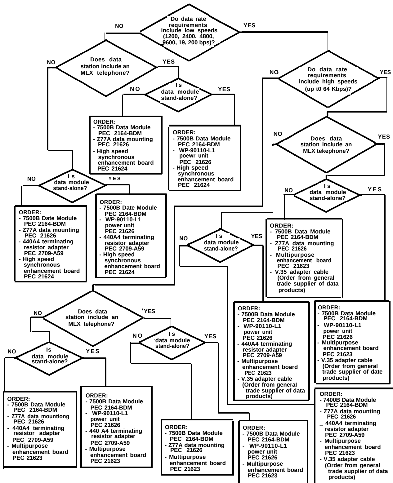
Figure 2-4 Synchronous Hardware Decision Flowchart
