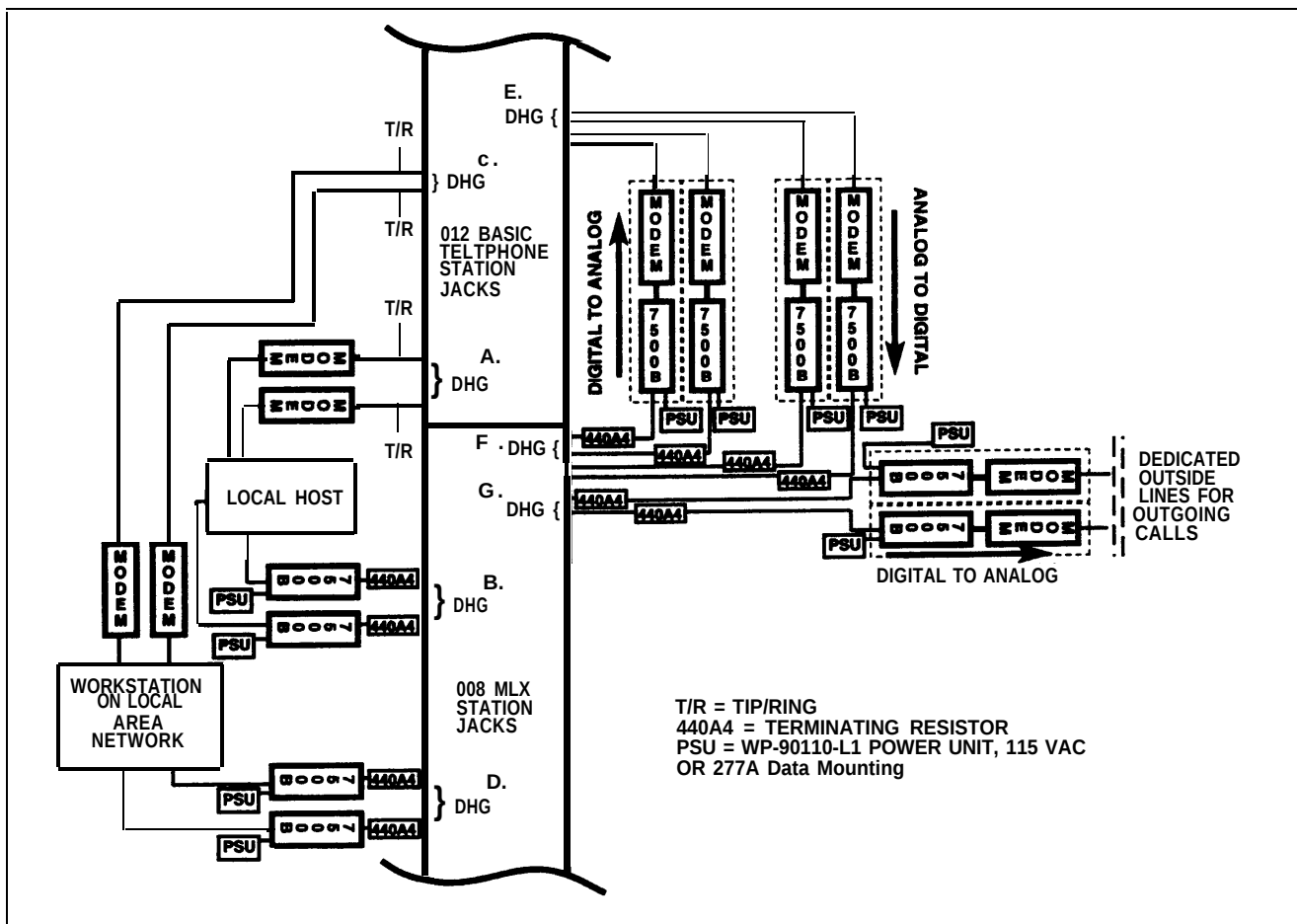
Figure 3-3 Data Hunt Groups
