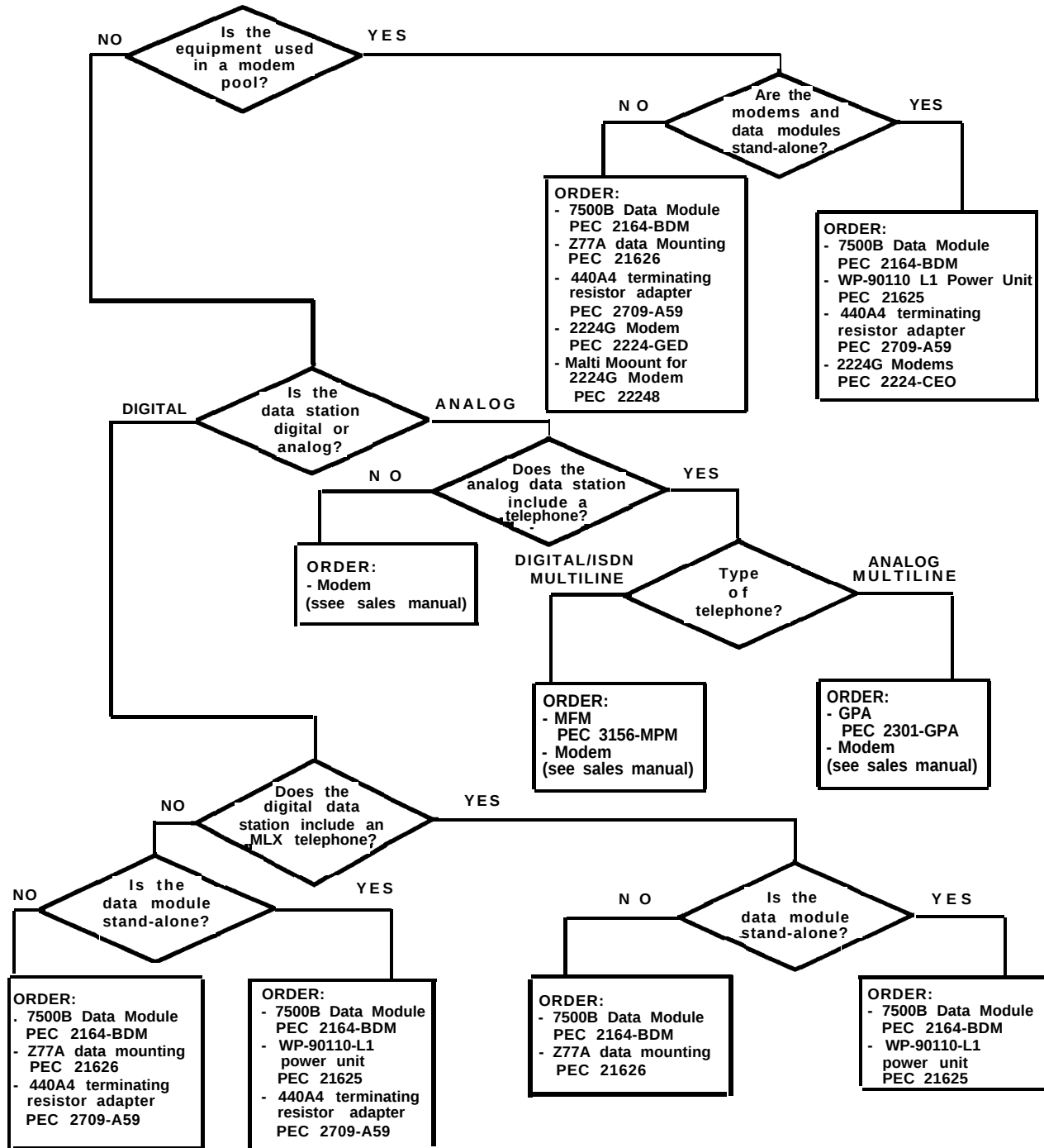
Figure 2-3 Asynchronous Hardware Decision Flowchart
