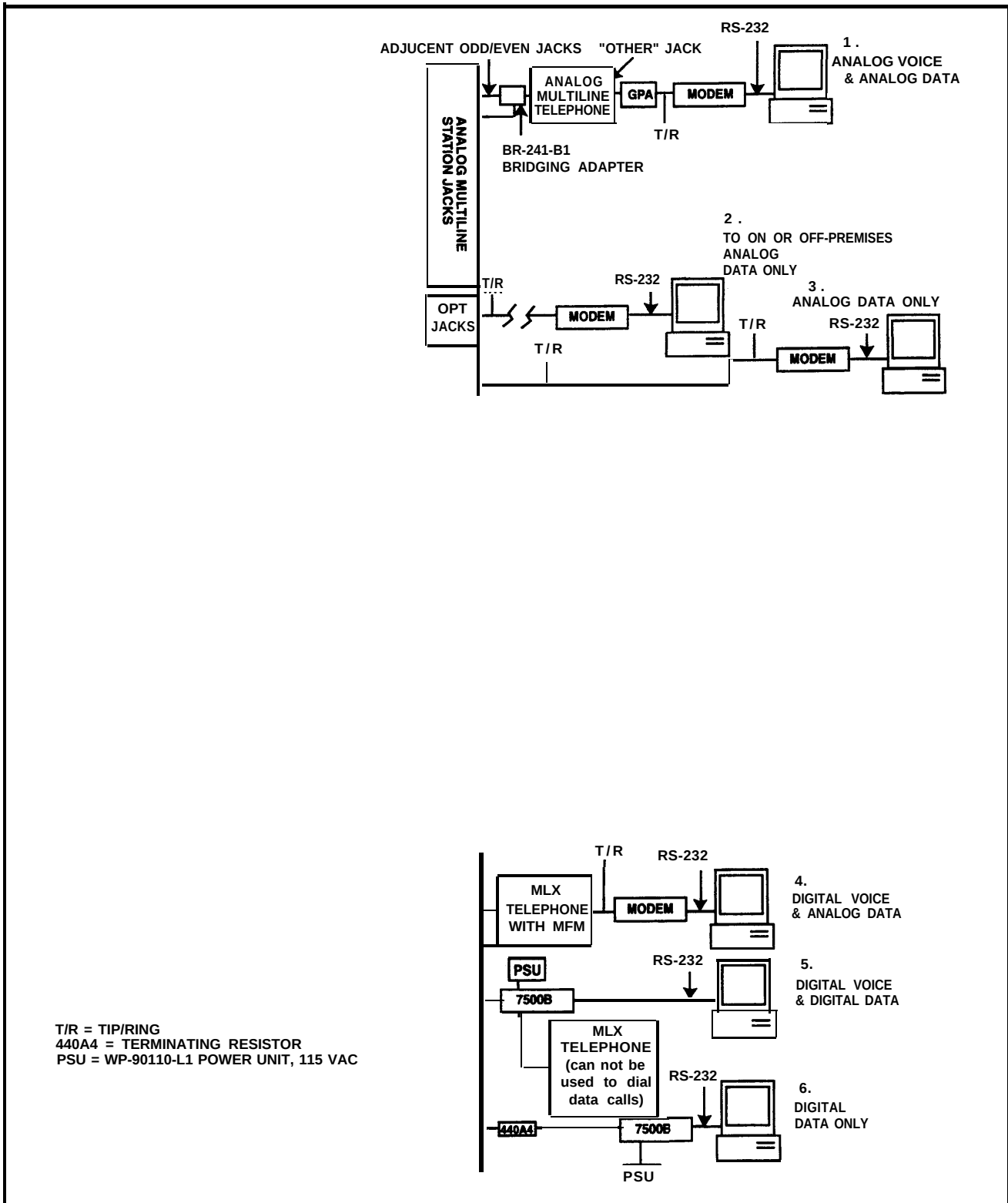
Figure 1-1 Individual Use Data Station Configurations
