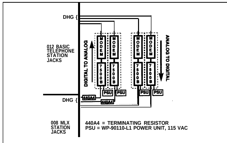
Figure 3-1 Modem Pools Using System Lines
