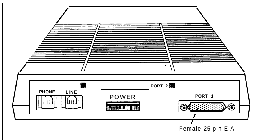
Figure 2-2 ISDN 7500B Data Module Back Panel
