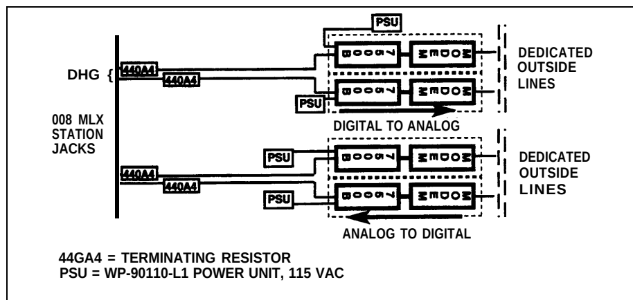
Figure 3-2 Modem Pools on Dedicated Outside Lines
