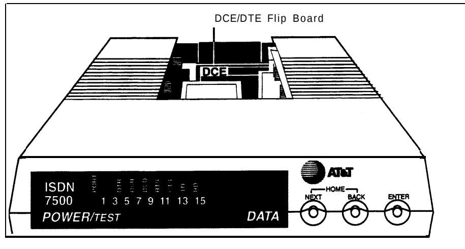
Figure 2-1 ISDN 7500B Data Module Front Panel
