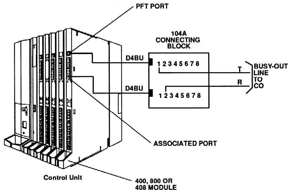
Figure 2-25. Power Failure DID Busy-Out Connections
