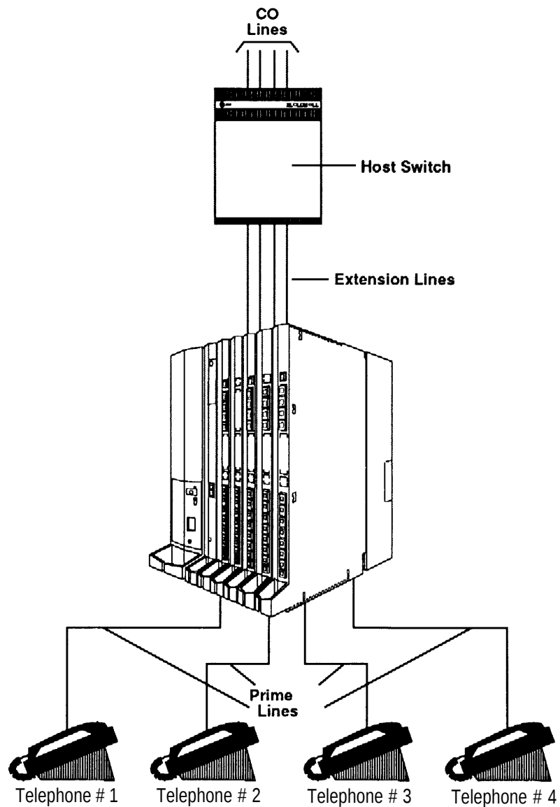
Figure 1-6. Behind Switch Mode
