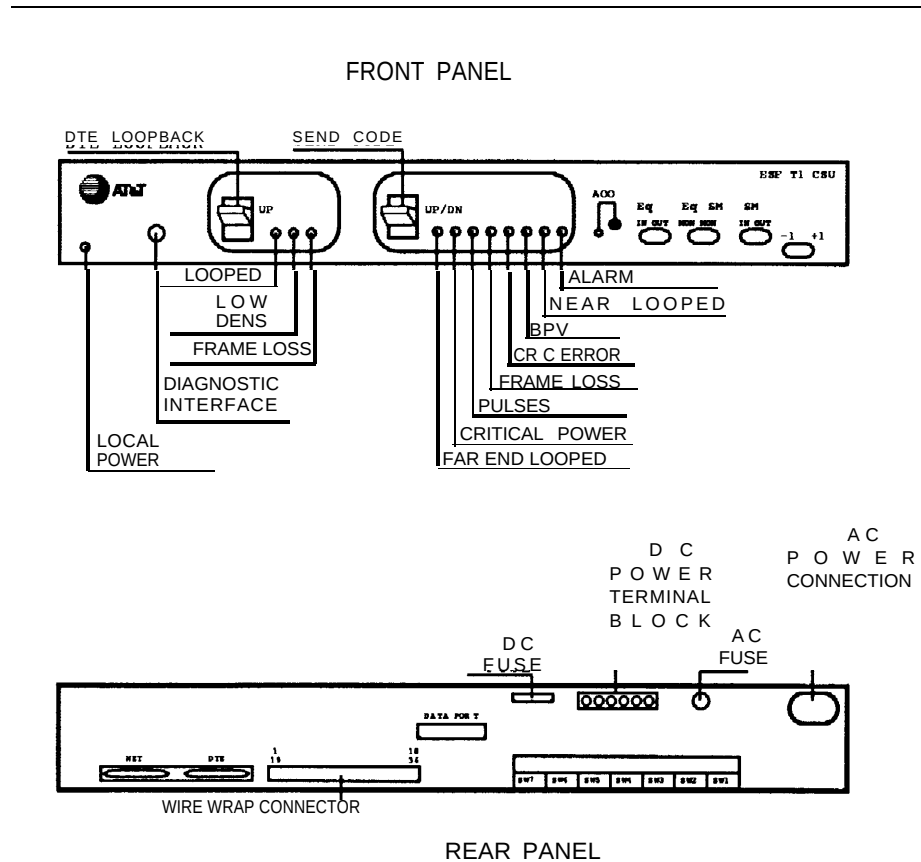
Figure 2-12. ESF T1 Channel Service Unit Connections
