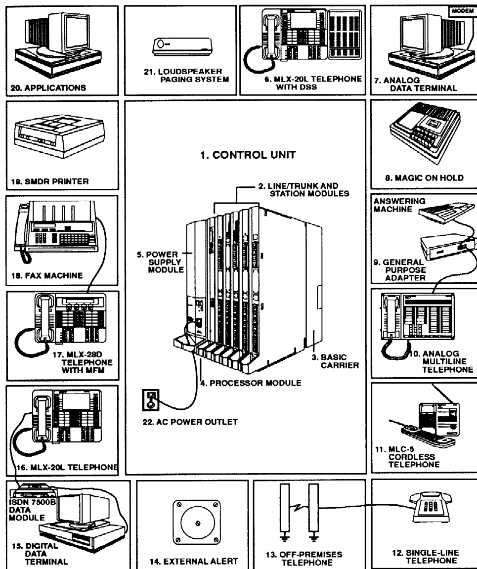
Figure 1-1. System Components
