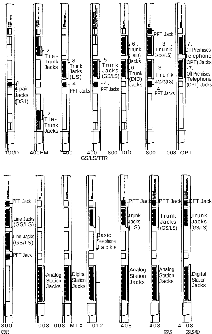
Figure 2-4. Line/Trunk and Station Modules
