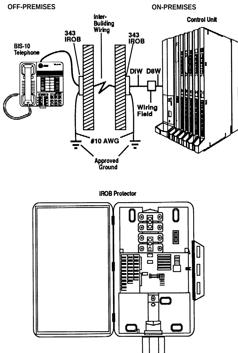
Figure 2-20. Analog IROB Connection
