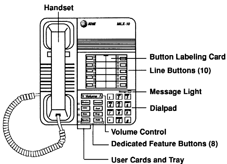
Figure 2-9. MLX-10 Telephone
