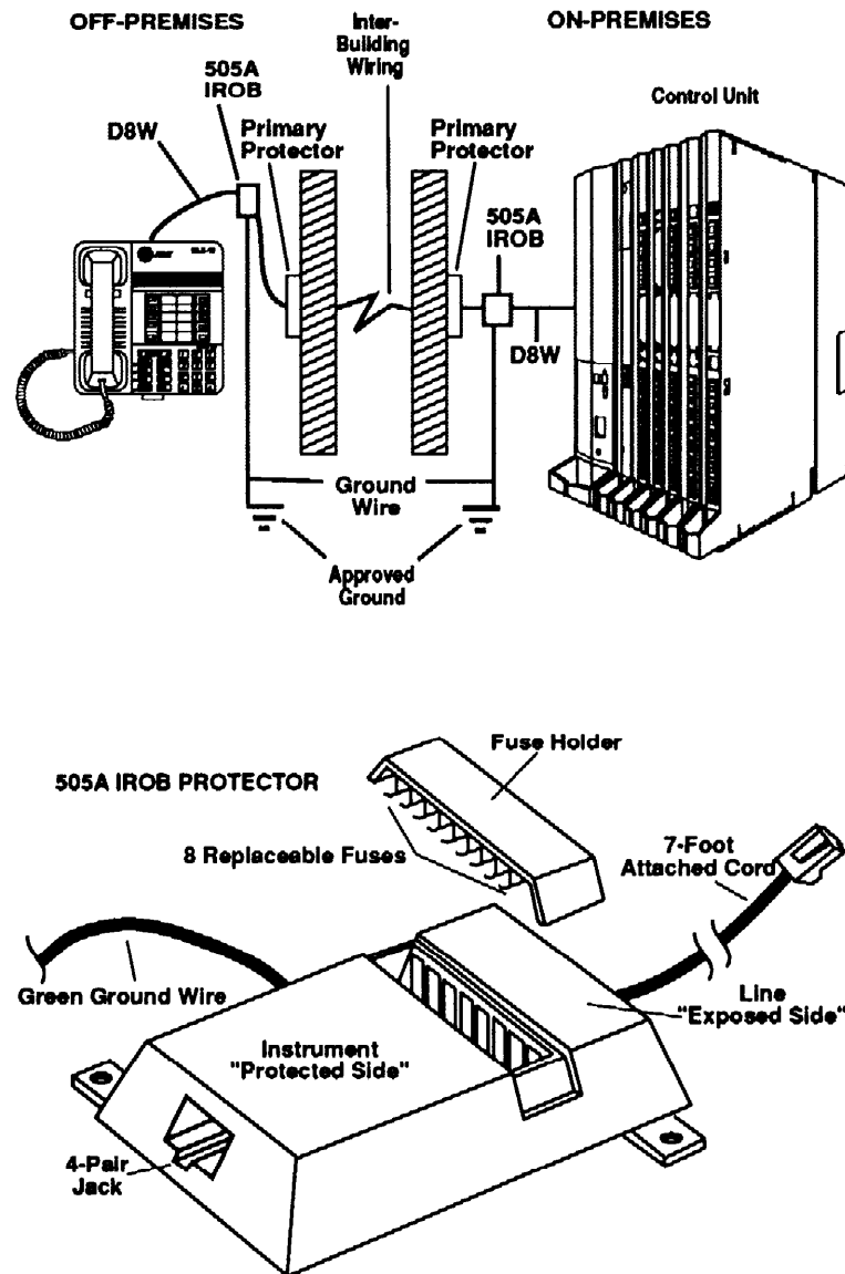
Figure 2-21. MLX IROB Connection
