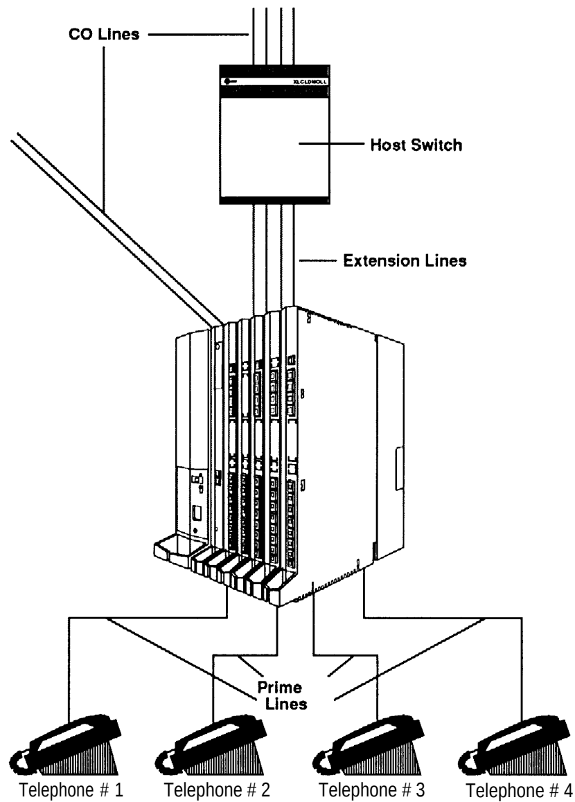
Figure 1-7. Behind Switch Mode with Direct Outside Trunks
