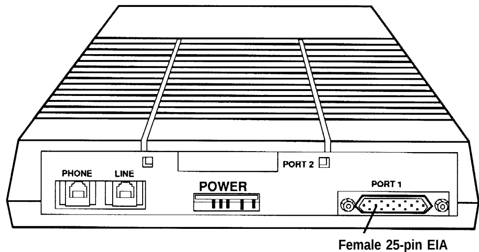
Figure 2-16. 7500B Data Module Back Panel
