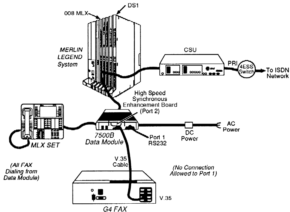
Figure 5-4. Direct V.35 Interface
