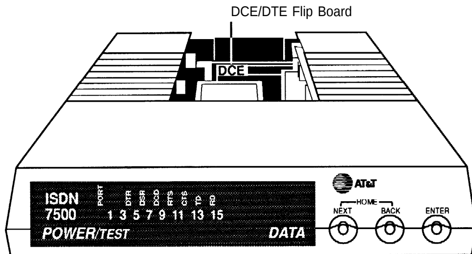
Figure 2-15. 7500B Data Module Front Panel
