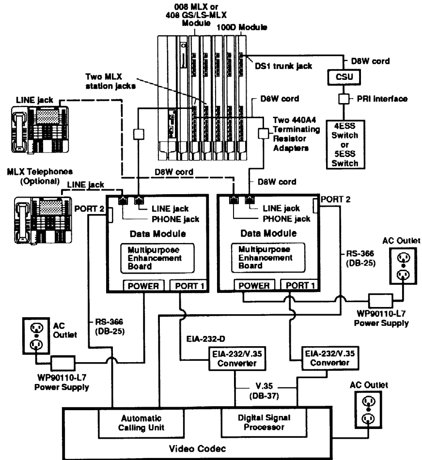
Figure 5-5. Video Conferencing Connections
