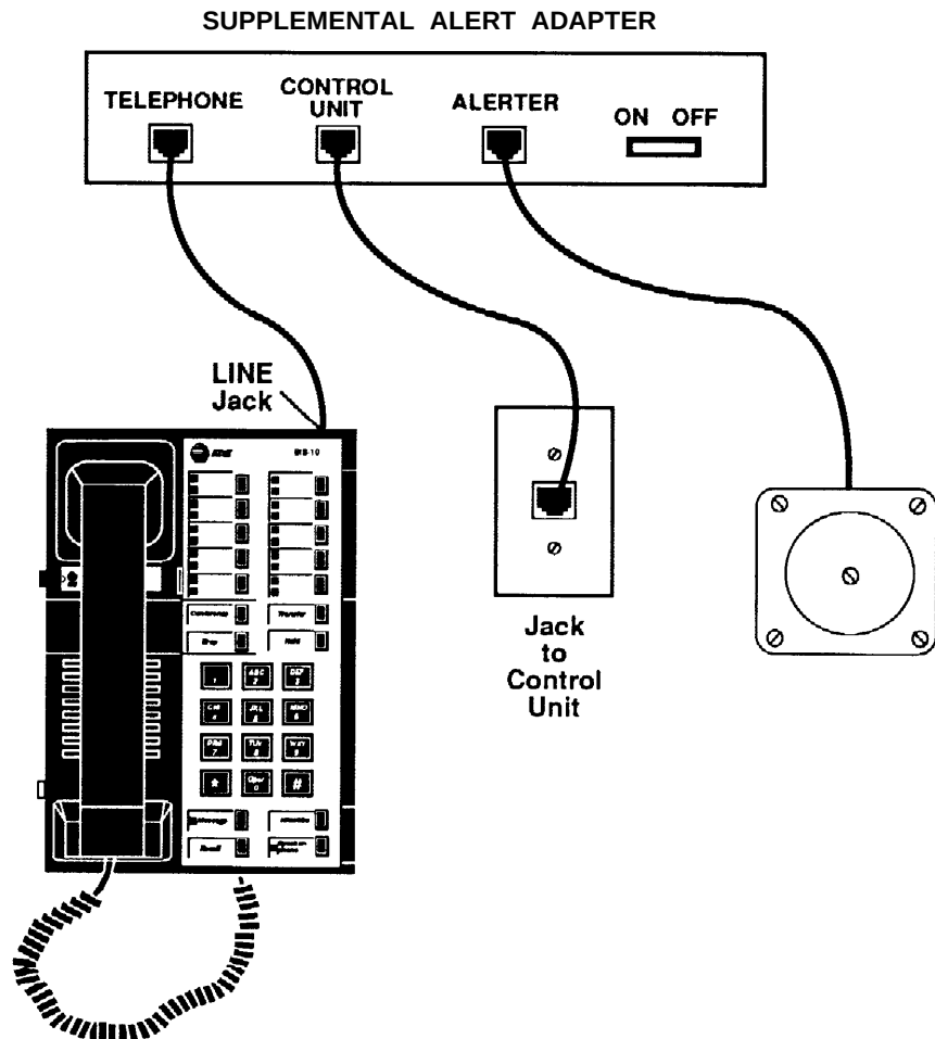
Figure 2-17, SAA Connections
