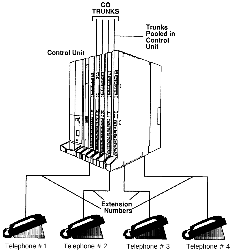
Figure 1-5. Hybrid/PBX Mode
