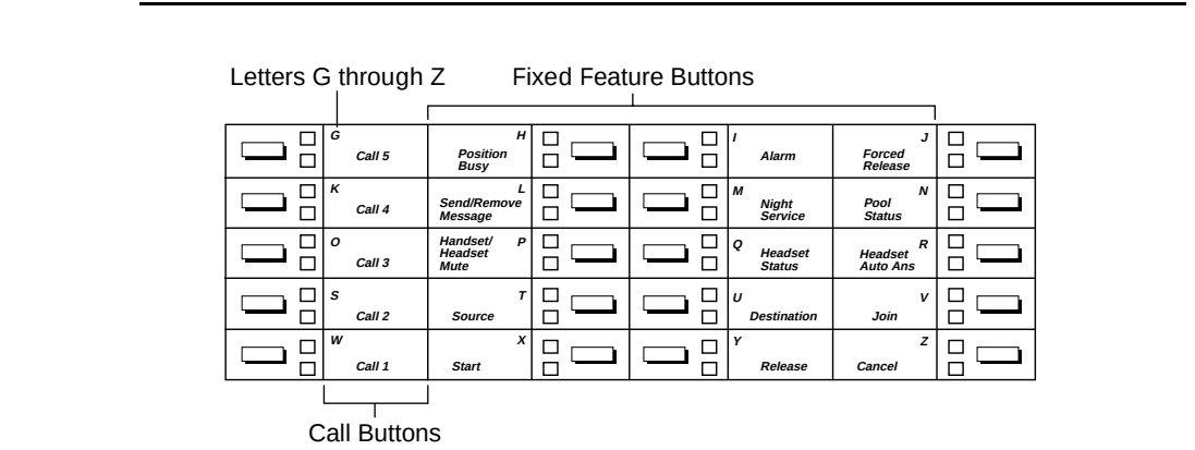
Figure 41. QCC Button Assignments
