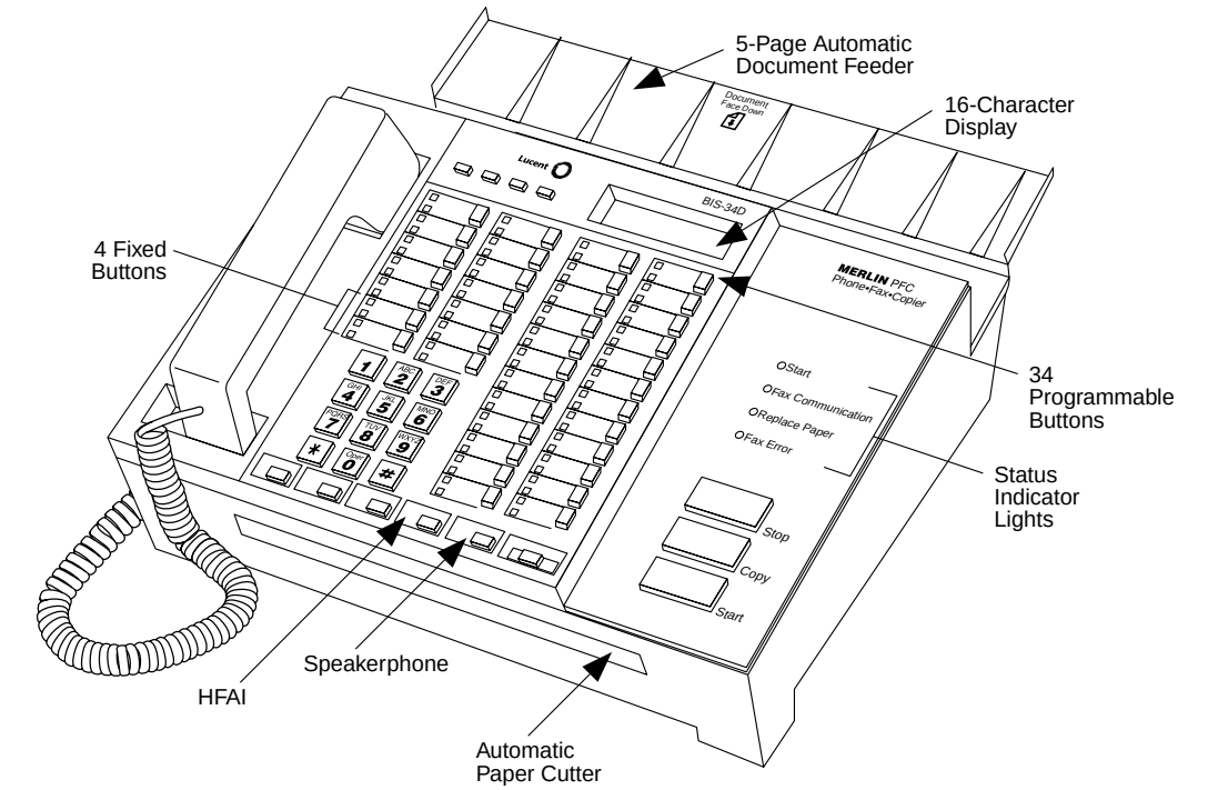
Figure I-3. MERLIN PFC Telephone
