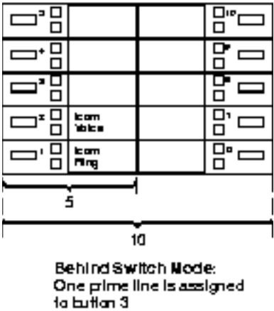
Figure G-7. MLX 5- and 10-Button Telephone Button Diagram (Key and Behind Switch Modes)
