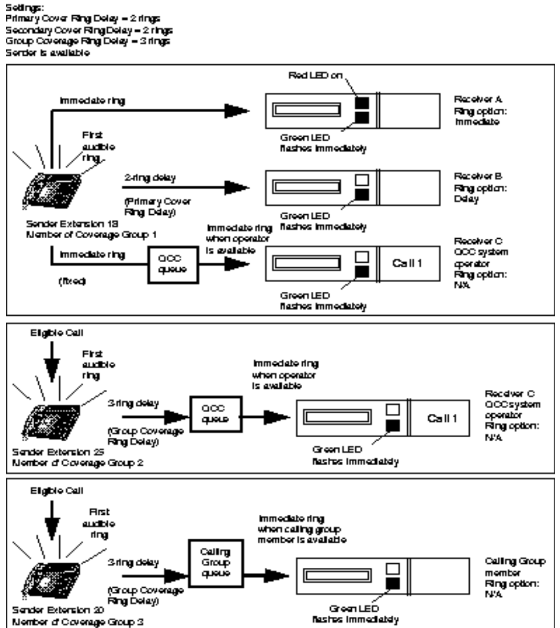
Figure 7. Group Coverage Only or All Individual Coverage Receivers Unavailable (Release 4.1 and Later Systems Only)
