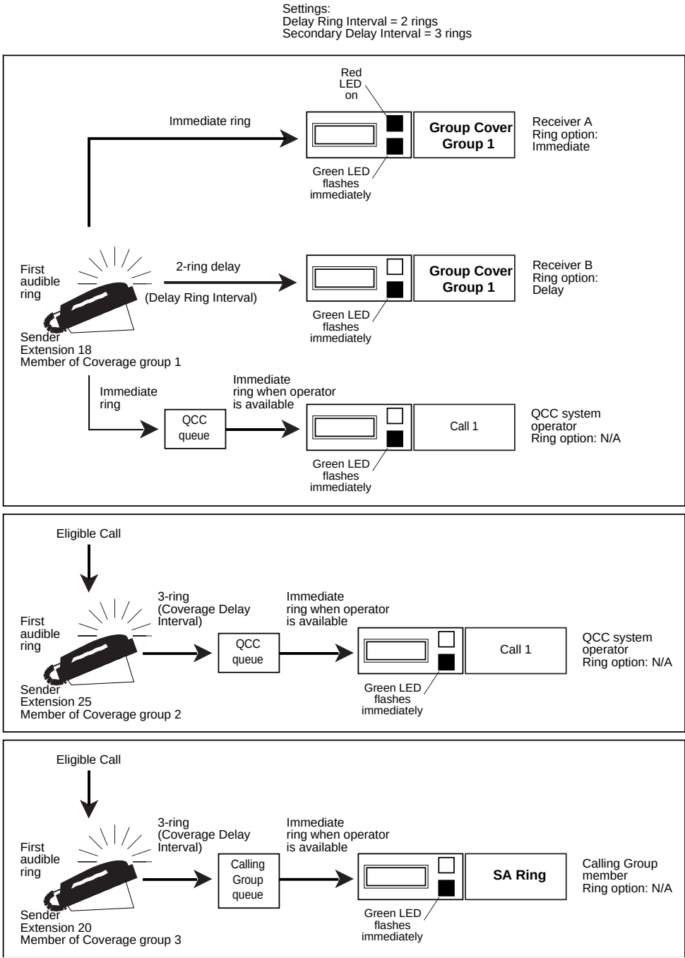
Figure 7. Group Coverage Only or All Individual Coverage Receivers Unavailable (Release 4.0 and Prior Systems)
