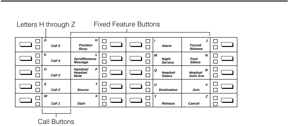
Figure 42. QCC Button Assignments
