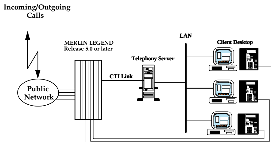
Figure 1-1. System Configuration for Support of CTI Applications
