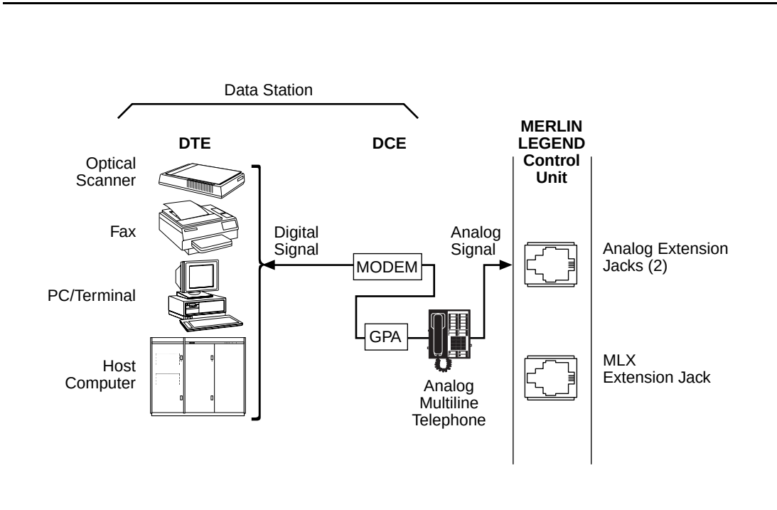
Figure 5-1. Analog Voice and Modem Data
