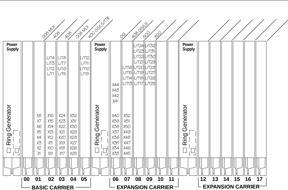
Figure 2-1. Sample Control Unit Diagram
