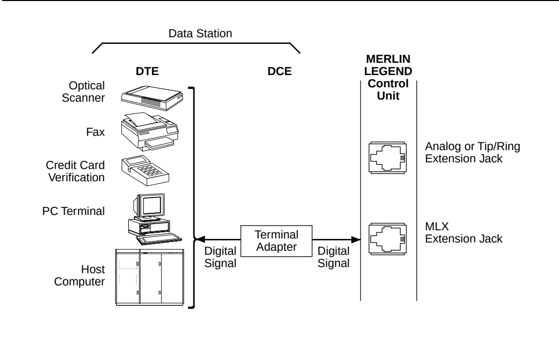
Figure 5-5. ISDN Terminal Adapter Data-Only
