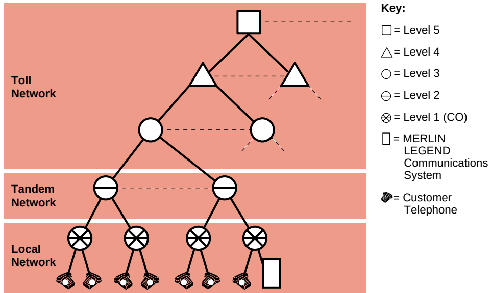
Figure 2-4. The Switching Office Hierarchy
