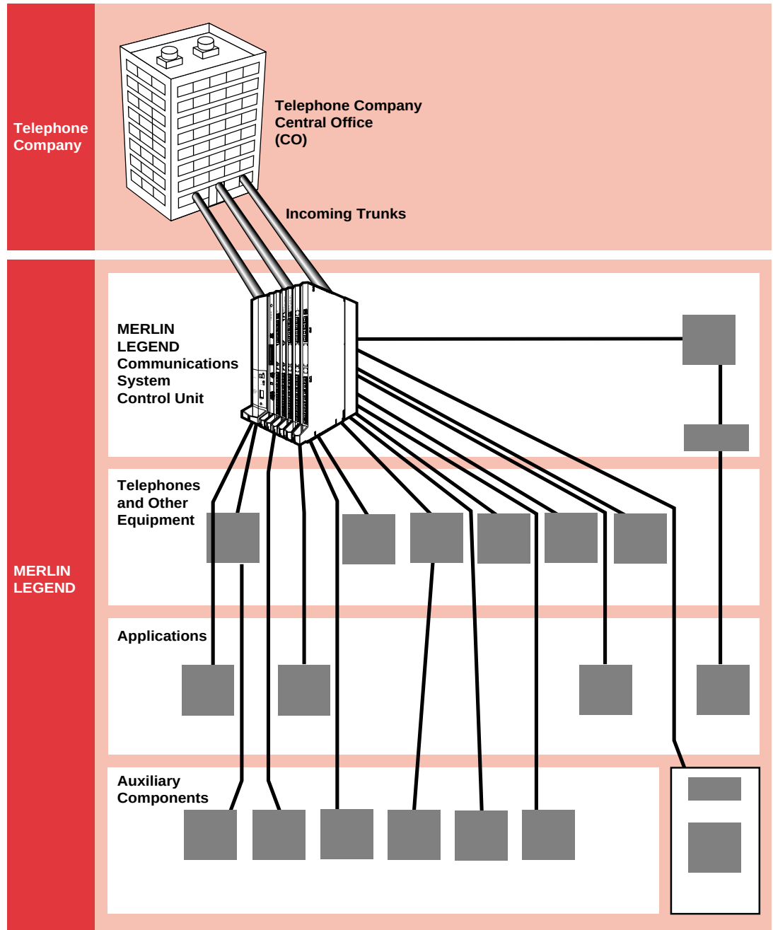
Figure 2-5. System Overview
