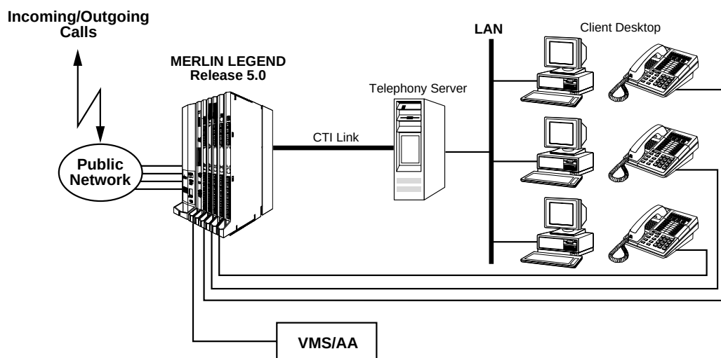
Figure 5-5. CTI Link Overview
