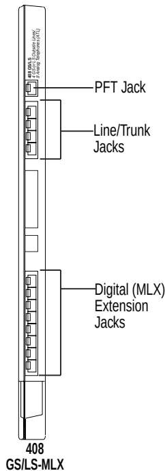
Figure 2-8. 408 GS/LS-MLX Module
