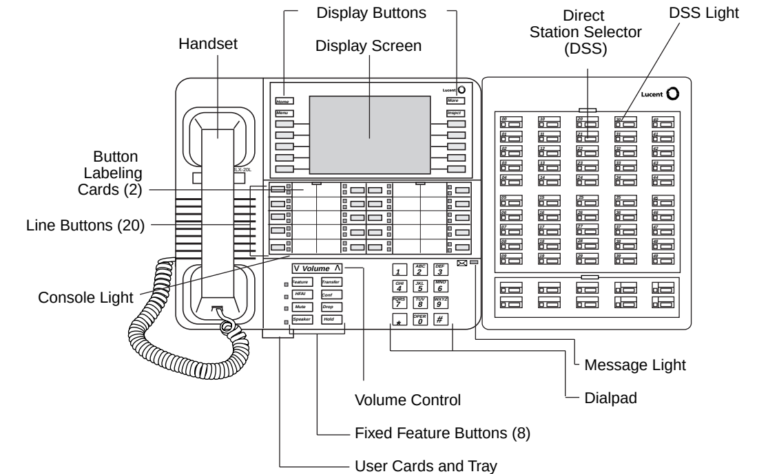
Figure 6-7. MLX-20L Telephone with Direct Station Selector (DSS)
