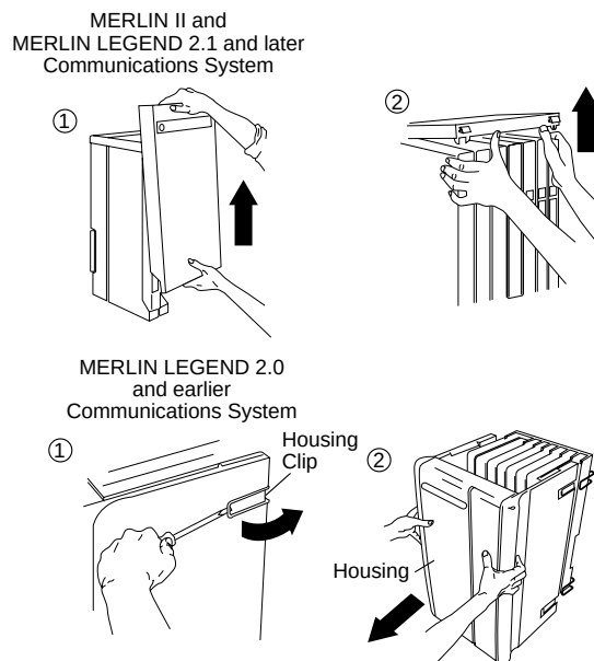
Figure E-1. Removing the Control Unit Housing
