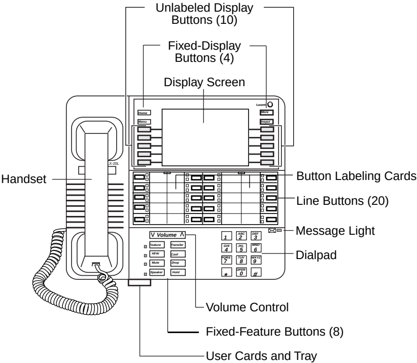
Figure 3-5. MLX-20L Telephone
