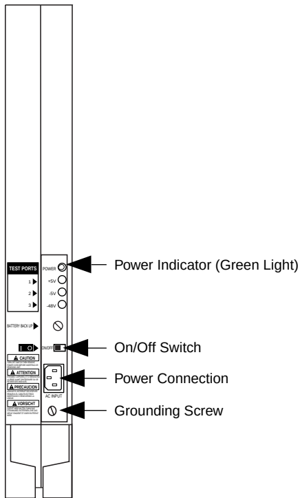
Figure 3-2. Power Supply Module
