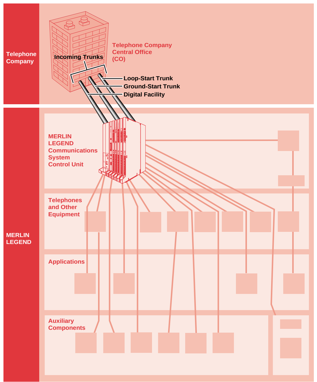
Figure 2-6. Incoming Trunks
