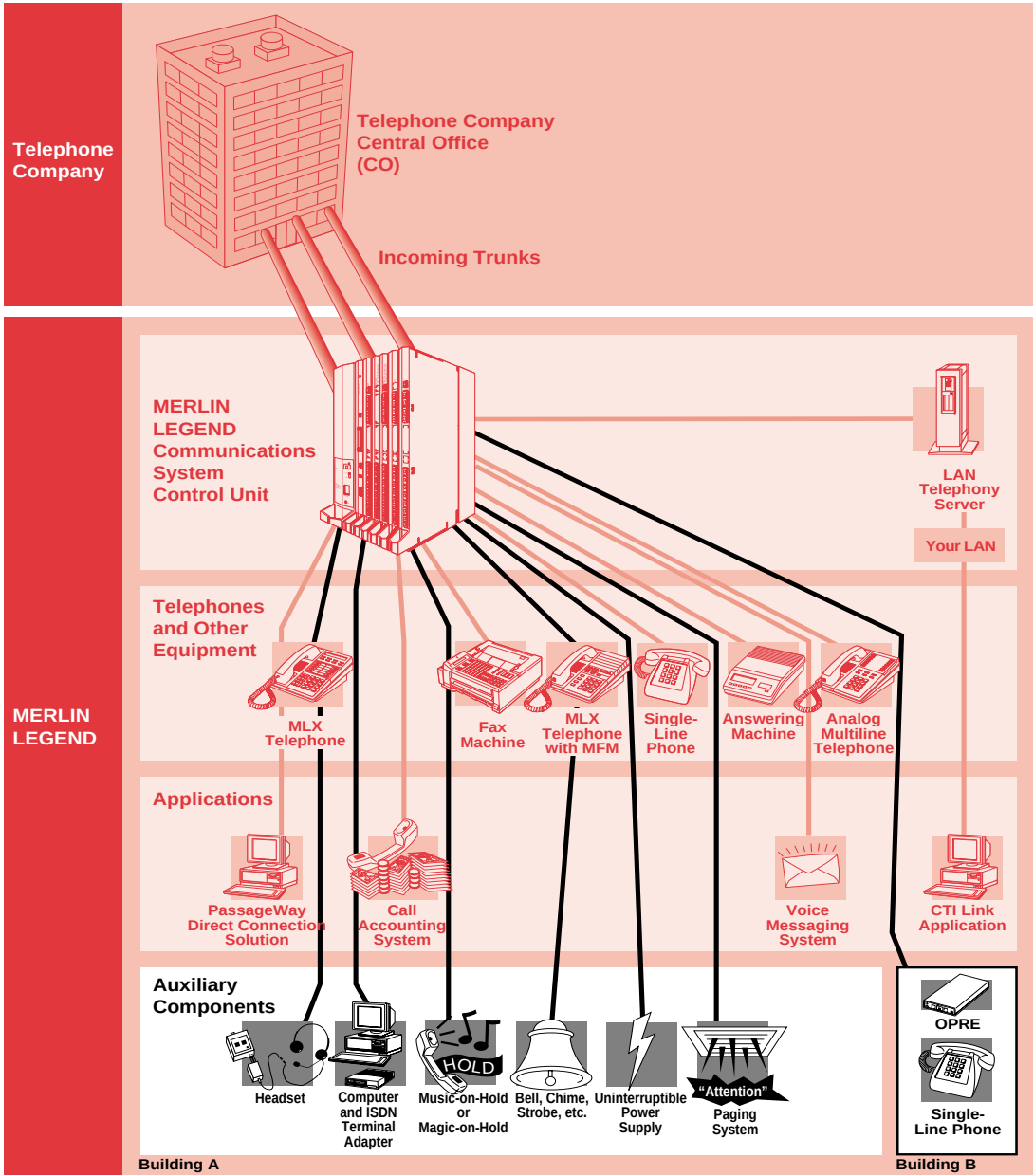
Figure 2-10. Auxiliary System Components
