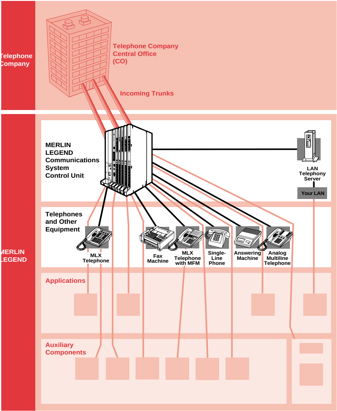
Figure 2-7. System Components
