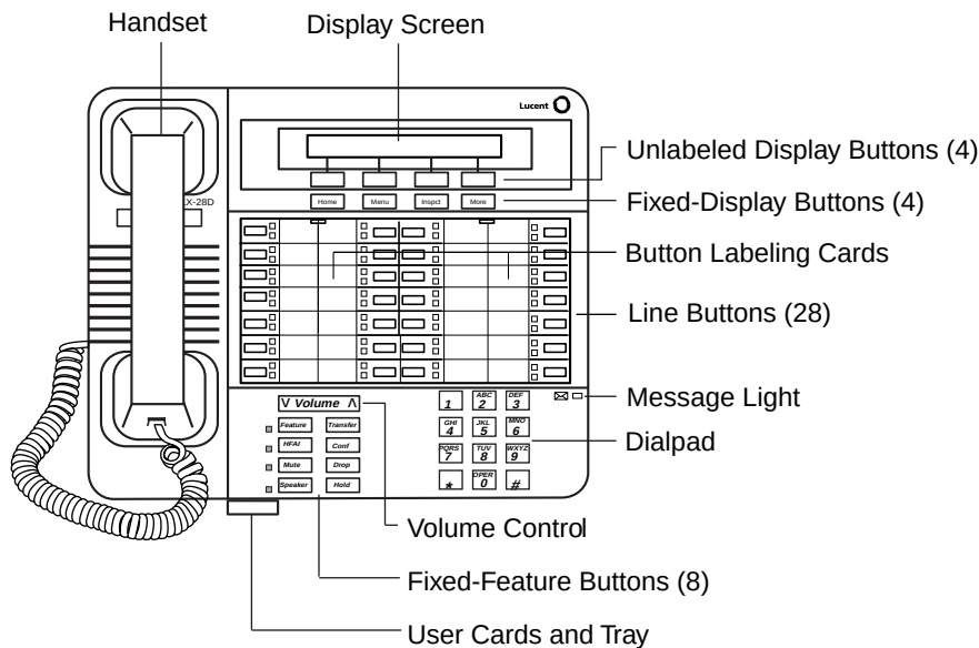
Figure 3-4. MLX-28D Telephone
