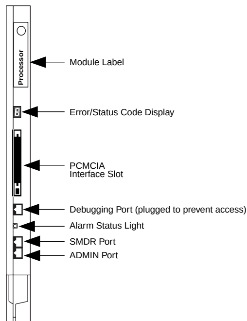
Figure 3-1. Processor Module
