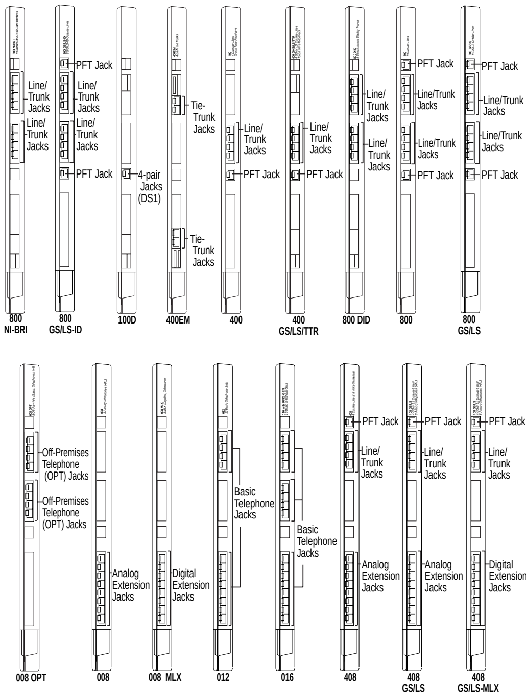
Figure 3-3. Line/Trunk and Extension Modules
