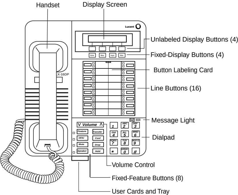
Figure 3–6. MLX-16DP Telephone
