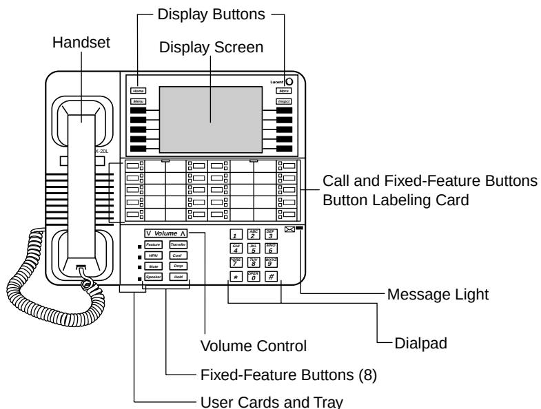
Figure 31. MLX-20L Telephone
