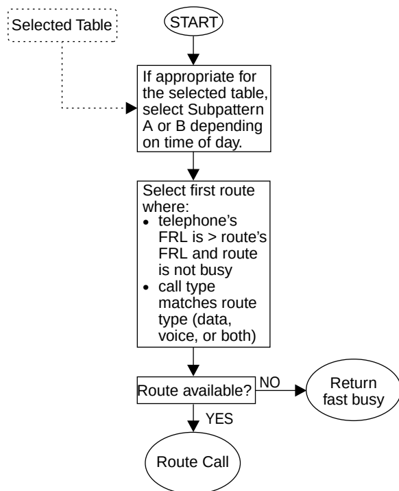
Figure 4. ARS Route Selection within a Table
