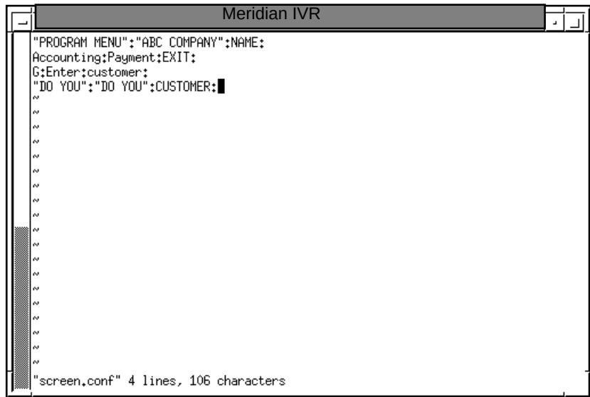
Figure 3-2 screen.conf file
