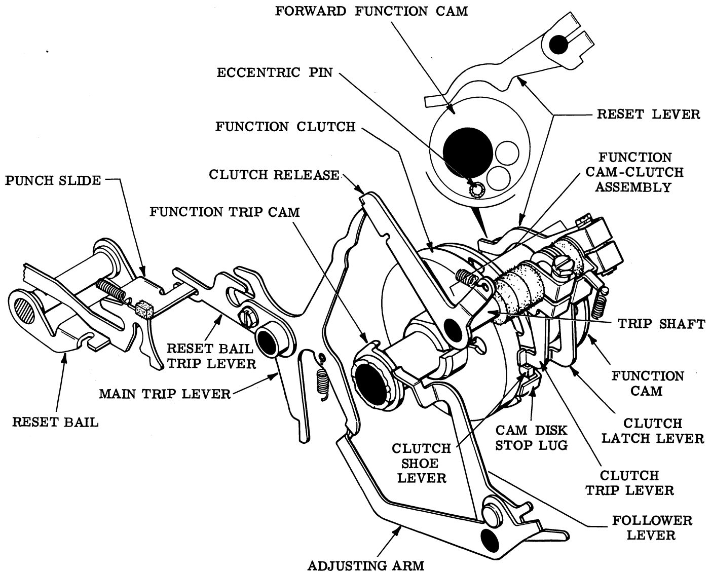
Figure 13 - Function Cam-Clutch and Clutch Trip Assembly
