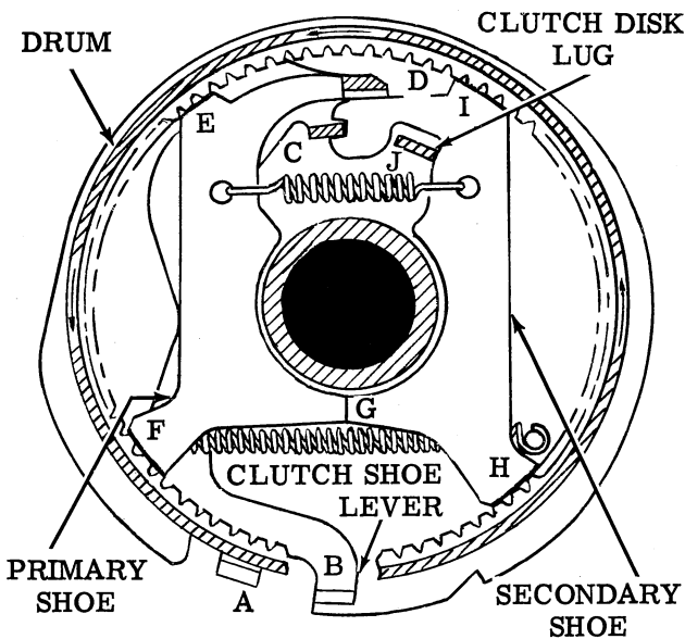
Figure 9 - Clutch, Engaged
