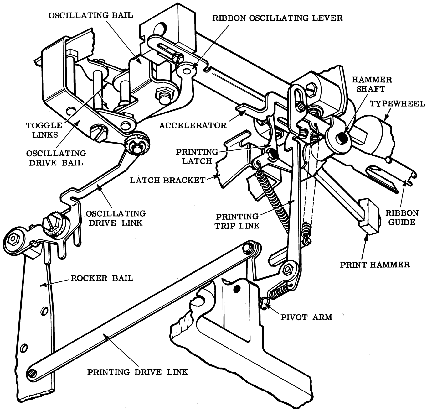
Figure 20 - Printing Mechanism
