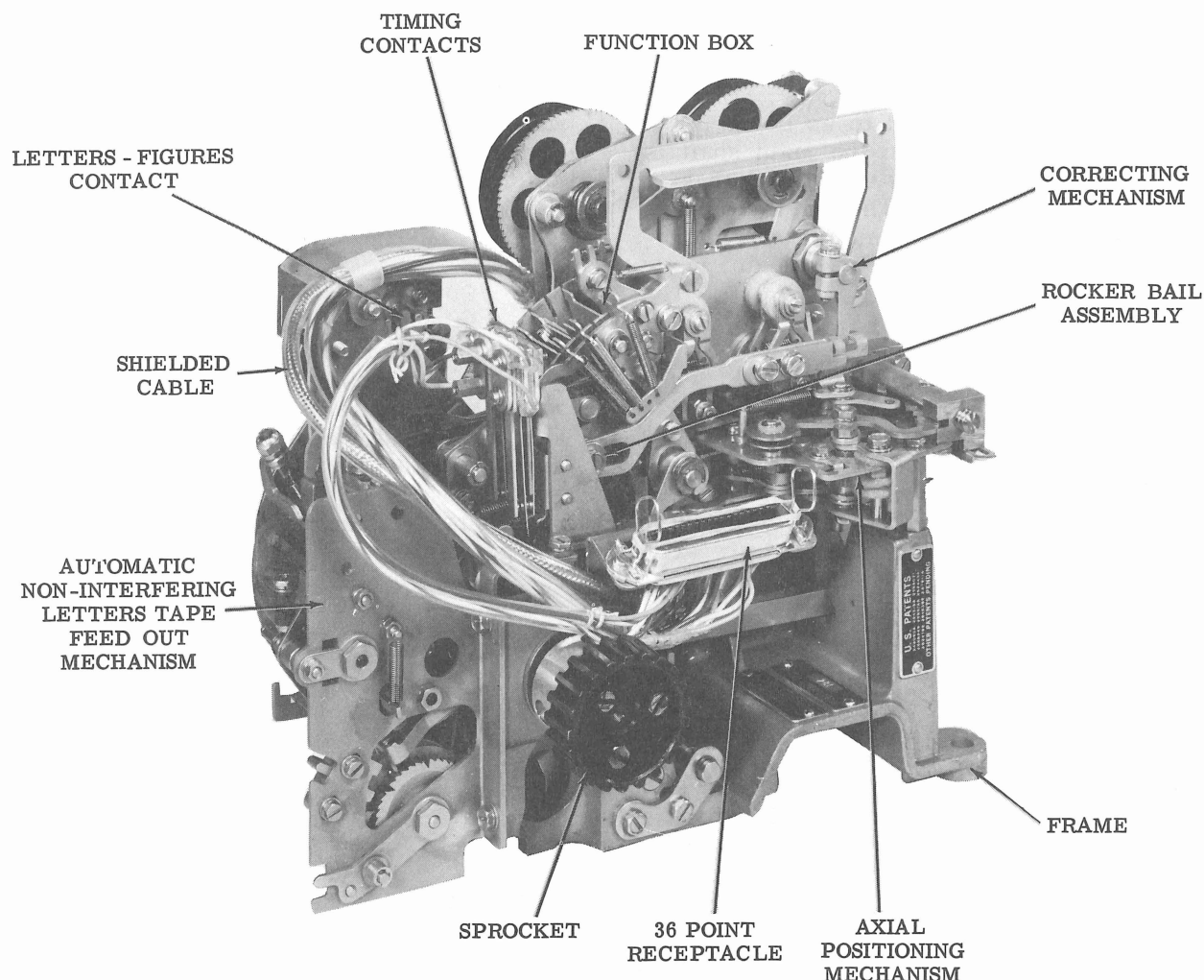
Figure 3 - 28 Typing Reperforator Unit - Fully Perforated Tape (Left Rear View)
