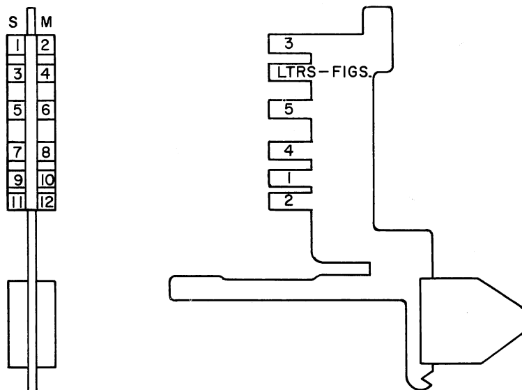
Figure 26 - Universal Function Blade
