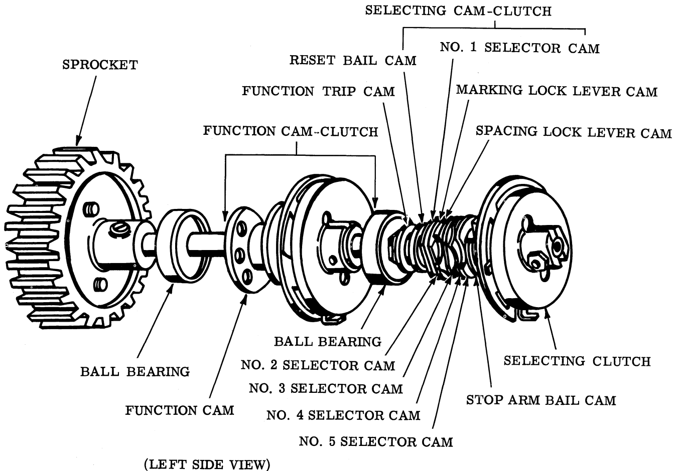
Figure 7 - Main Shaft
