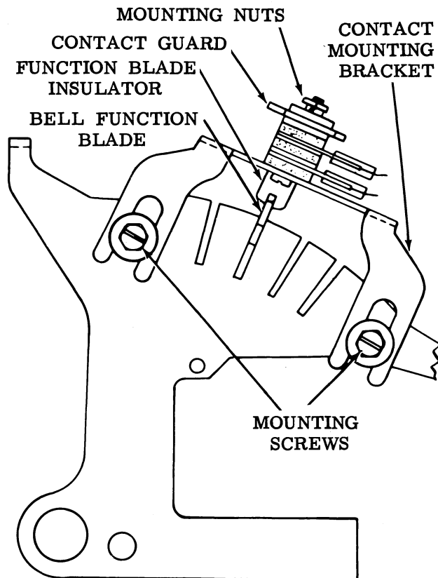
Figure 25 - Signal Bell Contacts
