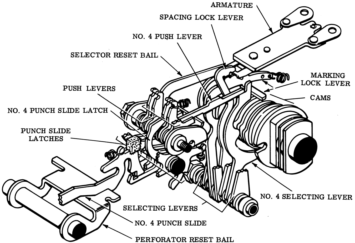
Figure 11 - Selector
