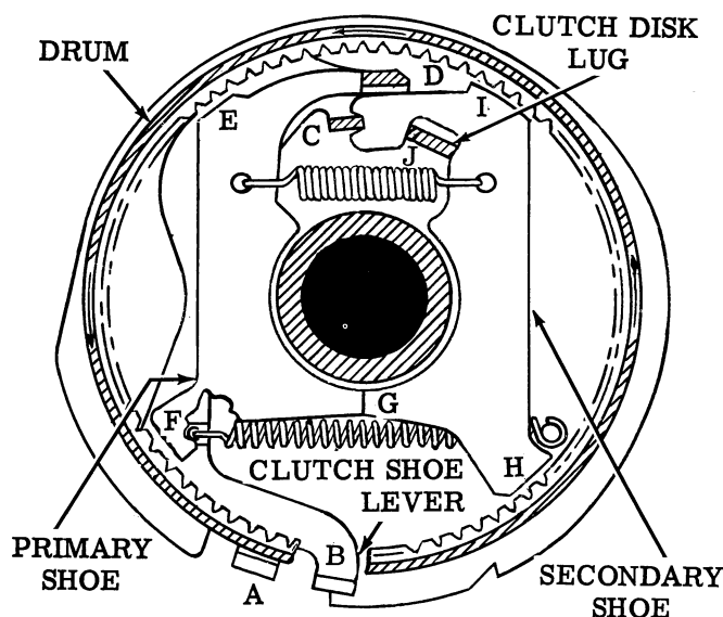
Figure 10 - Clutch, Disengaged
