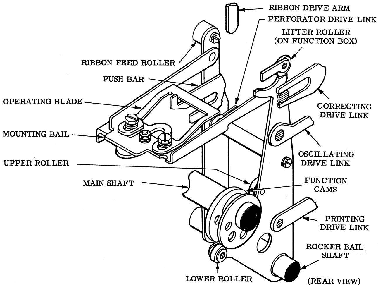
Figure 14 - Rocker Bail Assembly
