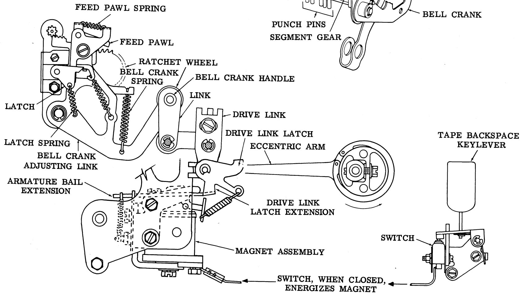
Figure 30 - Back Space Mechanisms
