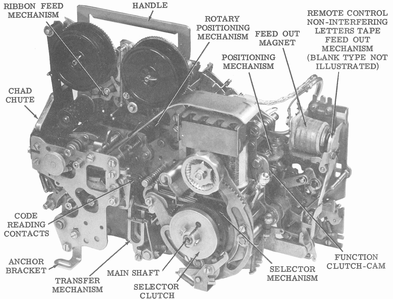
Figure 4 - 28 Typing Reperforator Unit (Front View) (Fully-Perforated Tape)
