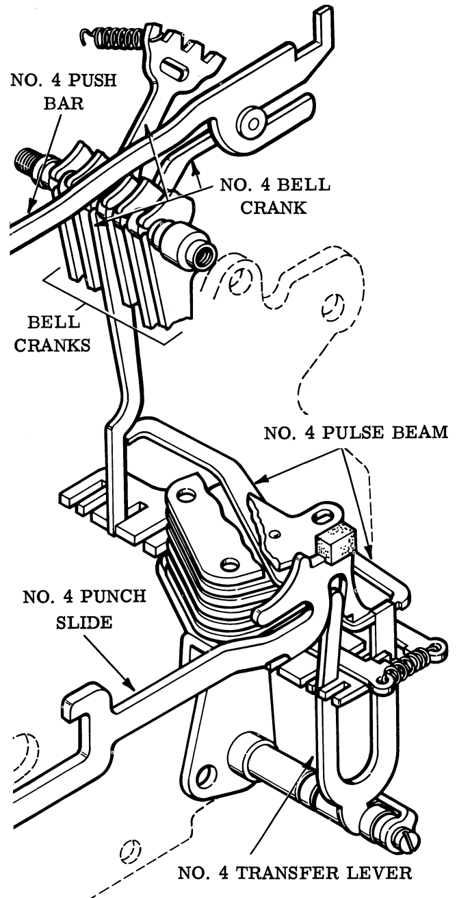
Figure 12 - Transfer Mechanism
