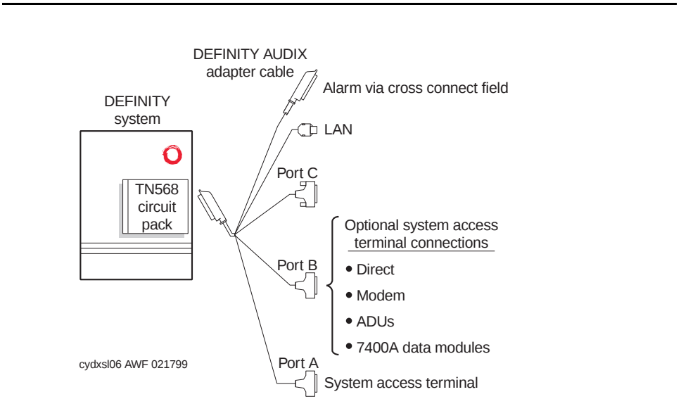
Figure 1-1. DEFINITY AUDIX System Connectivity Diagram - DS Integration
