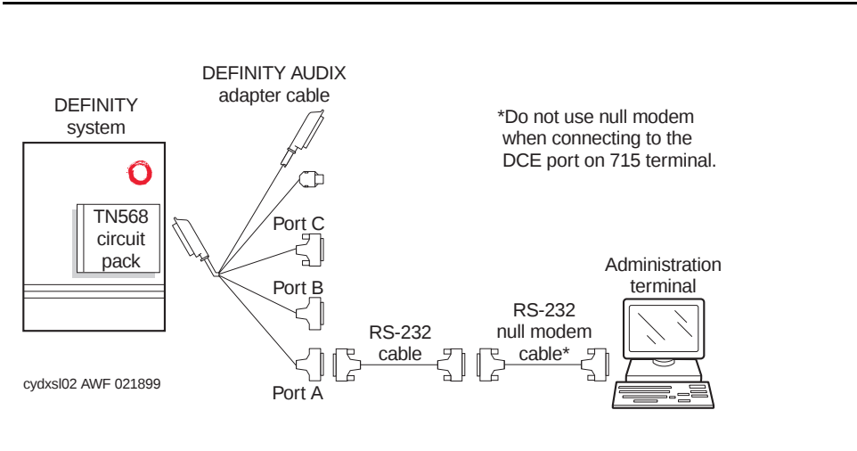
Figure 2-6. Installing a Terminal via Direct Connection (AC Switch only)
