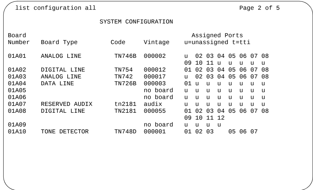
Figure I-4. Example List Configuration Screen — TN2181 Digital Port Emulation
