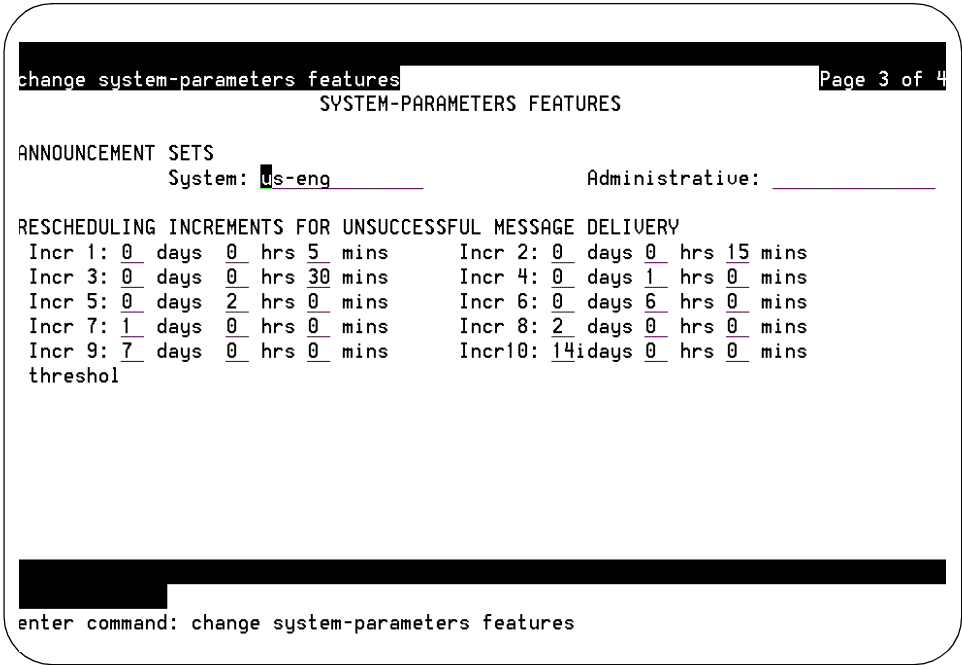
Figure 5-13. System-Parameters Features Screen (page 3)
