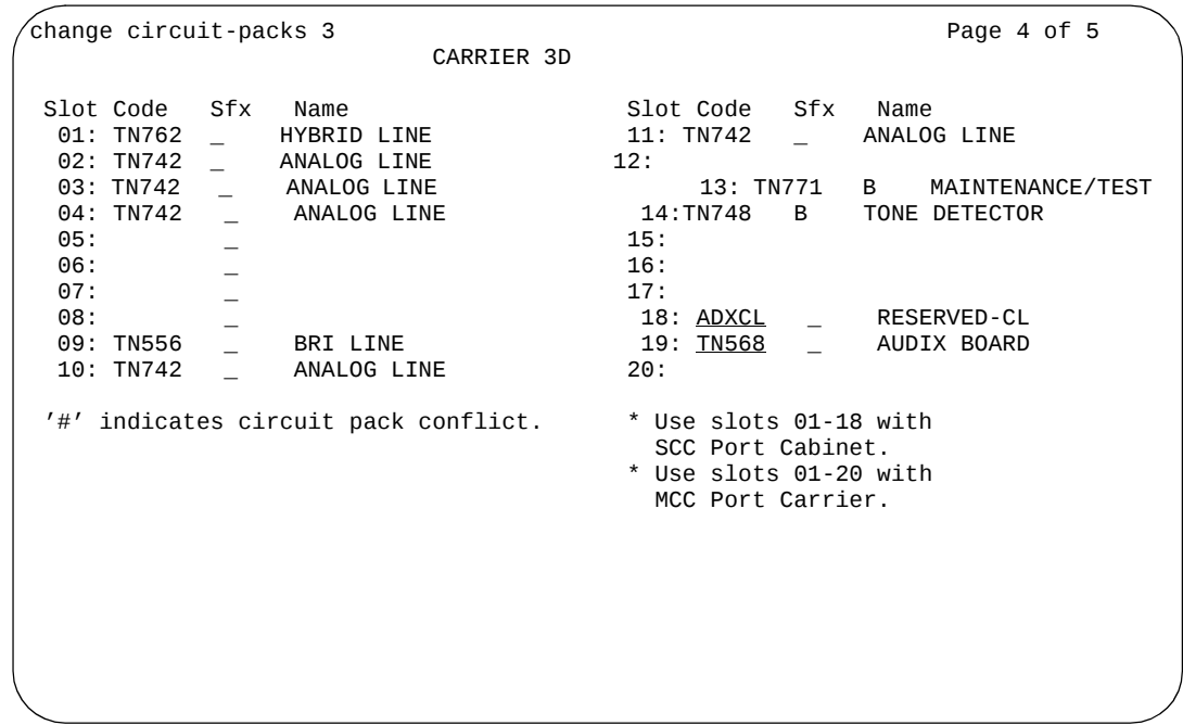
Figure J-1. Example of a Circuit Pack Screen G3V2/G3V3 (G3i)
