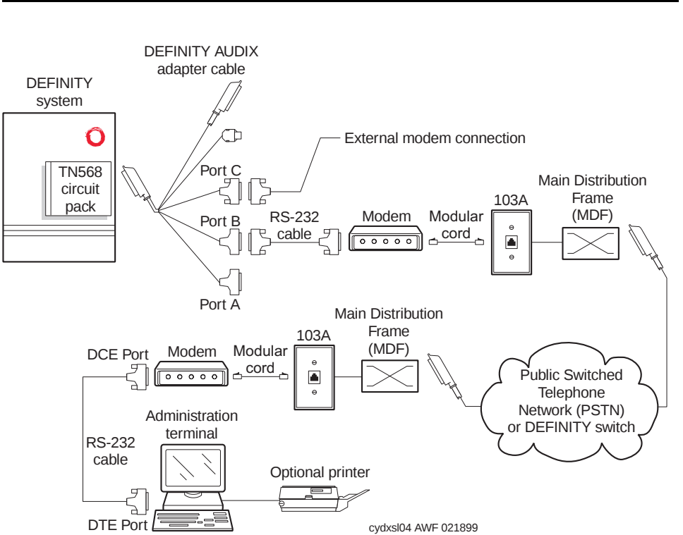
Figure 2-8. Installing an Additional Administration Terminal via Modem
