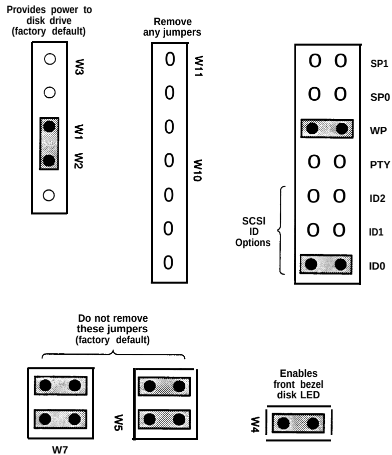
Figure B-17. Jumper Settings for SCSI Hard Disk Drive 1 (Second Drive)
