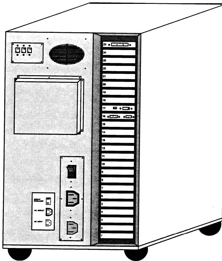
Figure 1-3. Map/100 Deskside Unit (Back)
