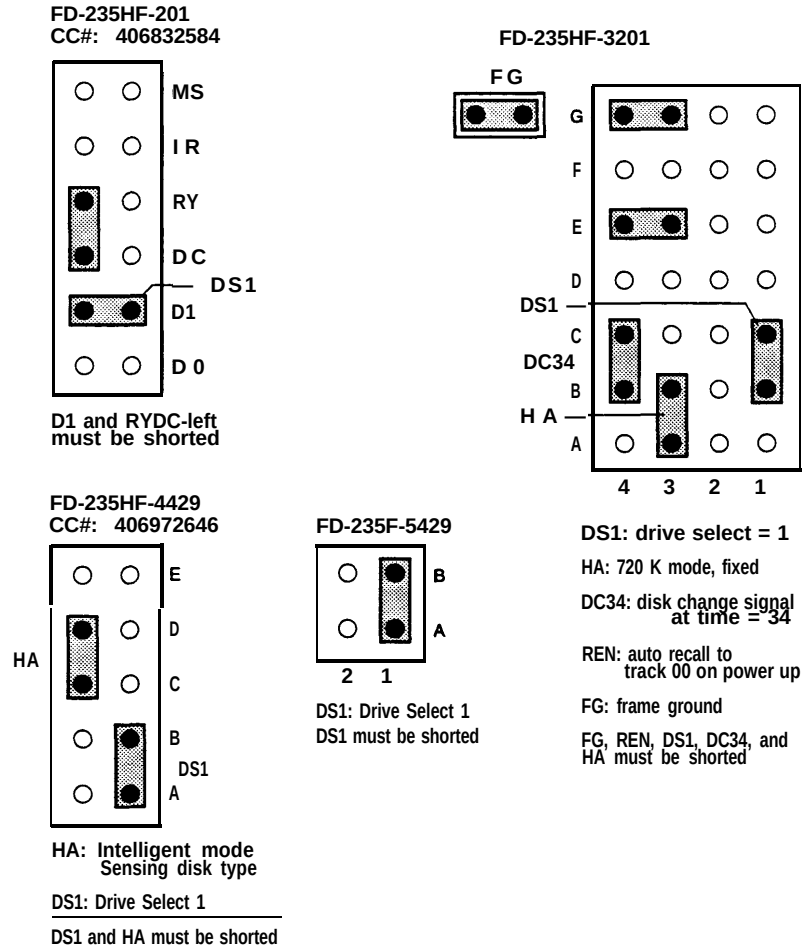
Figure B-10. Floppy Disk Drive Jumper Connections (201, 3201, 4429, 5429)
