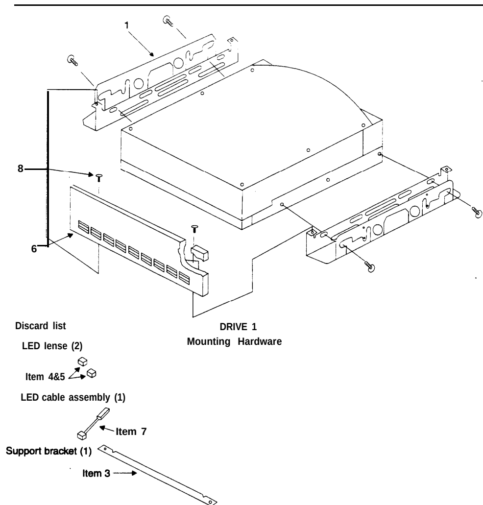
Figure B-19. Universal Installation Kit Assembly Instructions
