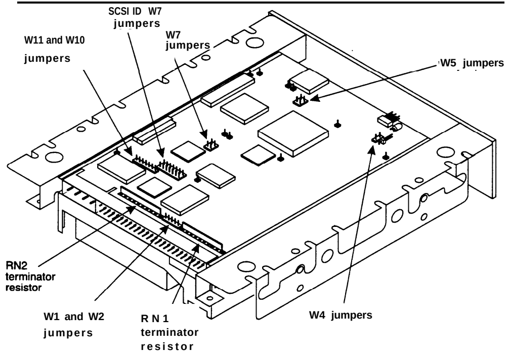
Figure A-4. SCSI Hard Disk Jumper Locations
