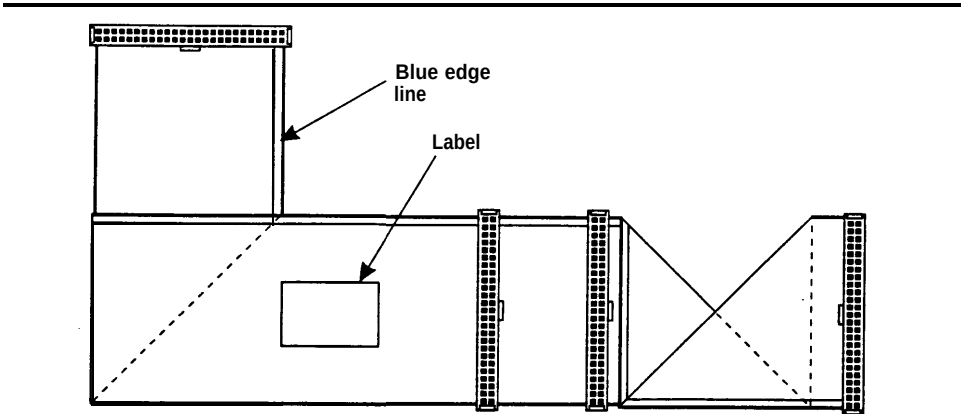
Figure B-20. SCSI Cable for SCSI Peripherals—Folded View
