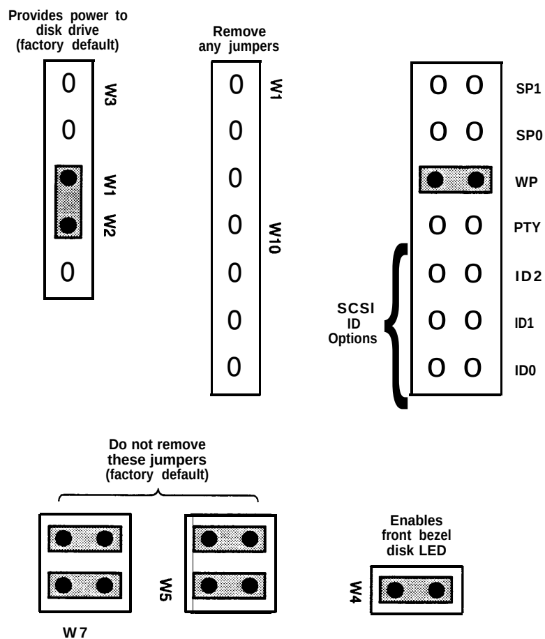
Figure A-5. Jumper Settings for First Disk Installed—Bay 1—SCSI ID=0
