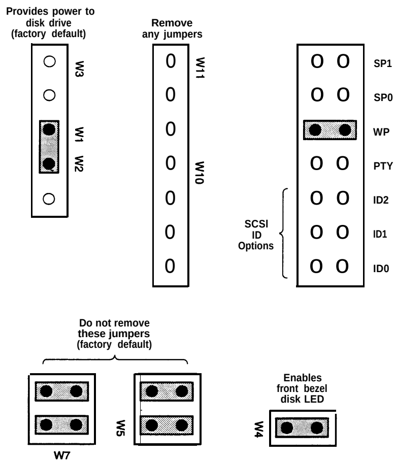
Figure B-16. Jumper Settings for SCSI Hard Disk Drive 0 (First Drive)
