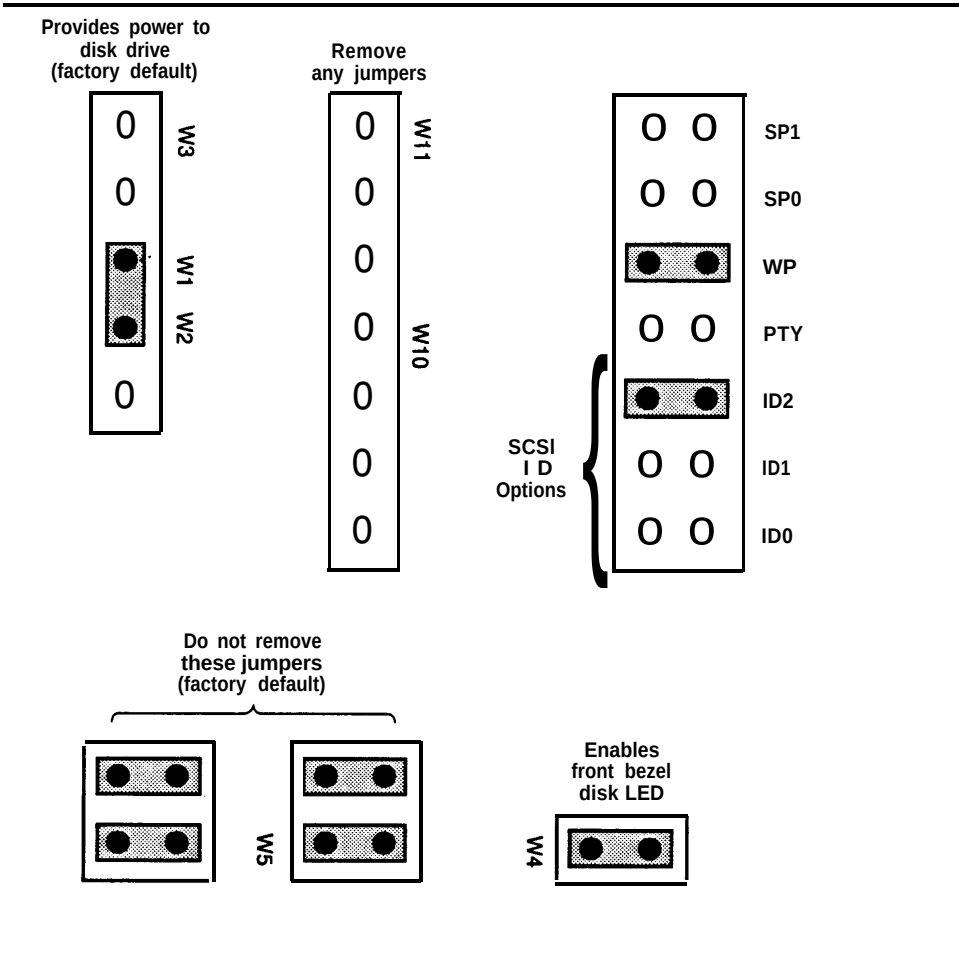
Figure A-8. Jumper Settings for Fourth Disk Installed—Bay 6—SCSI ID=4
