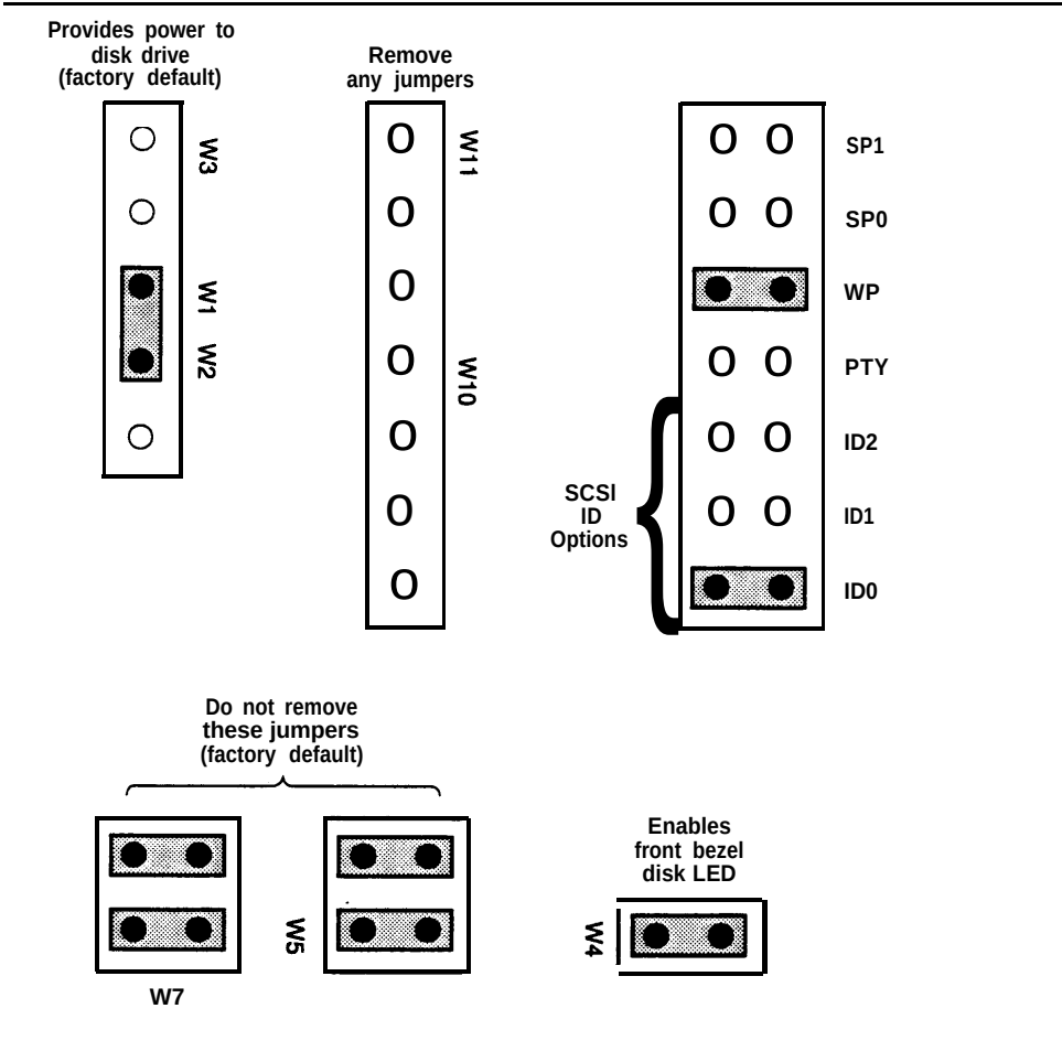
Figure A-6. Jumper Settings for Second Disk Installed—Bay 3—SCSI ID=2
