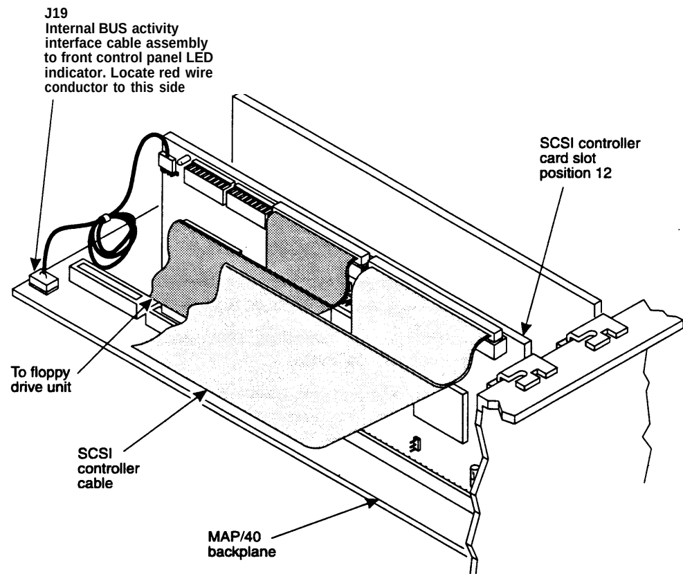
Figure B-13. MAP/40 Cable Assembly Placement
