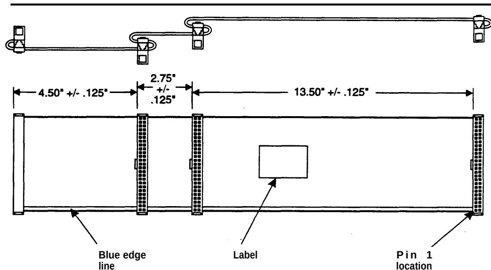
Figure A-12. SCSI Cable for SCSI Peripherals
