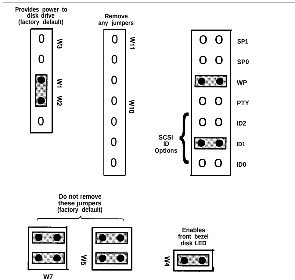
Figure A-7. Jumper Settings for Third Disk Installed—Bay 5—SCSI ID=3
