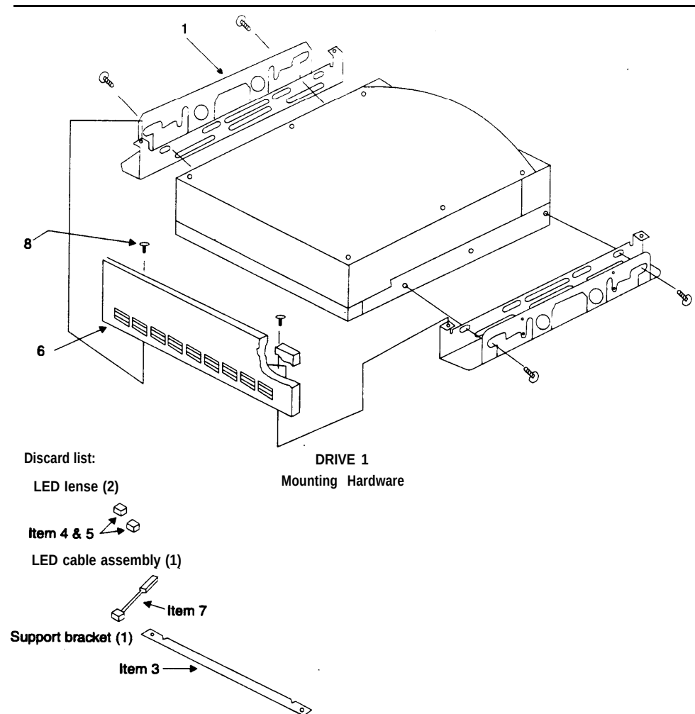
Figure A-11. Universal Installation Kit Assembly Instructions
