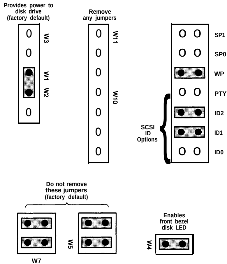
Figure A-10. Jumper Settings for Sixth Disk Installed—Bay 4—SCSI ID=6
