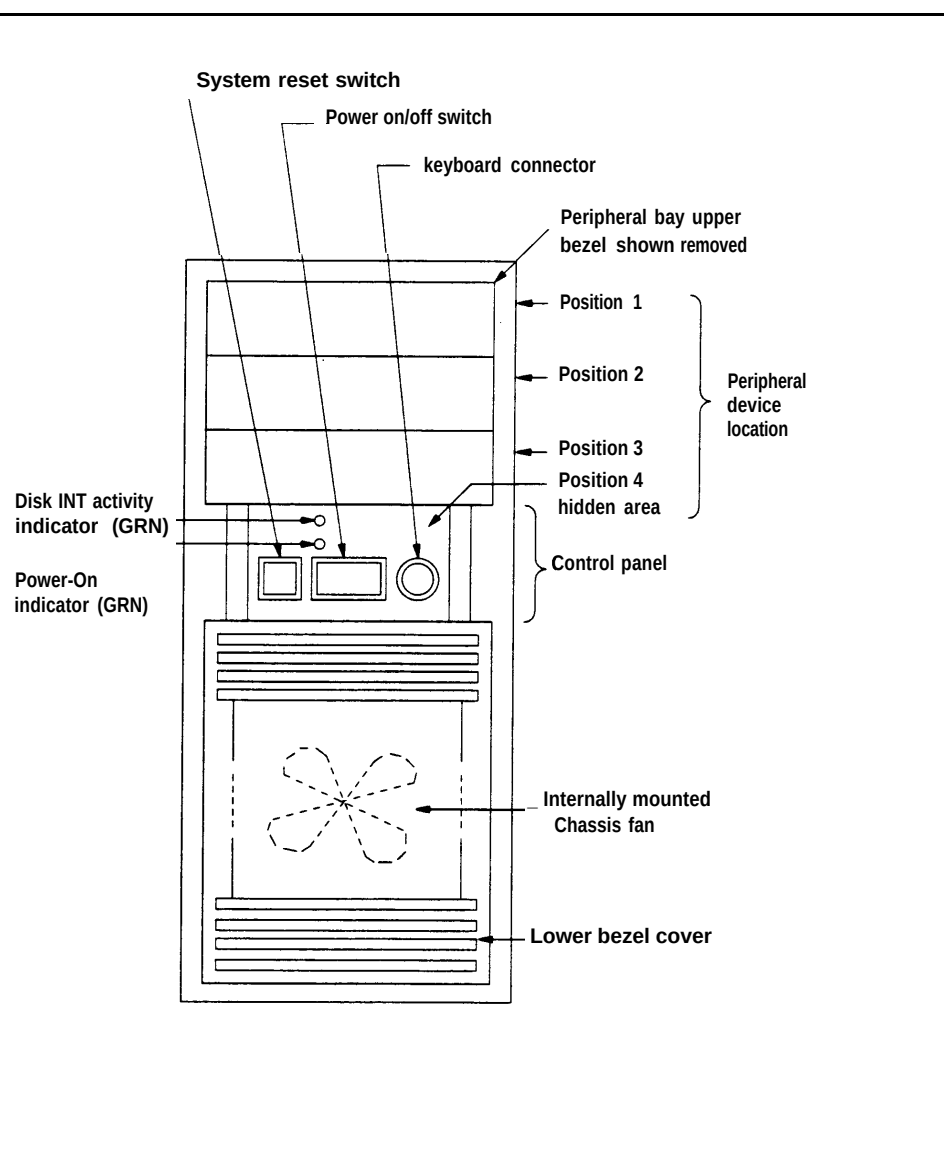
Figure B-1. Front View of MAP/40-Components
