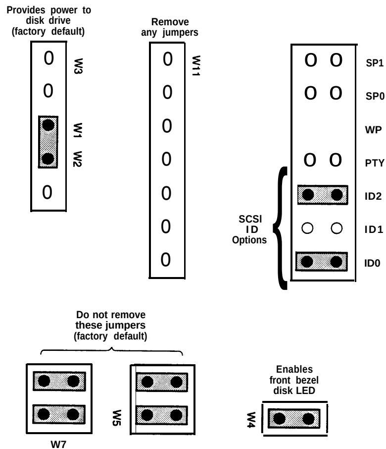
Figure A-9. Jumper Settings for Fifth Disk Installed—Bay 2—SCSI ID=5
