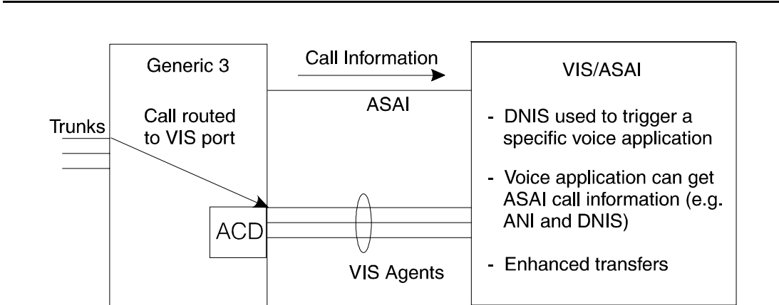
Figure 3-3. ASAI Voice Response Applications
