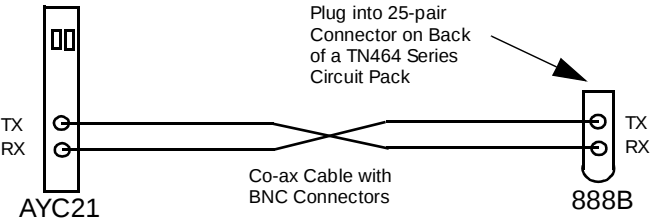
Figure 2-1. Example of AYC21 Coaxial Connections to a DEFINITY G3 Switch
