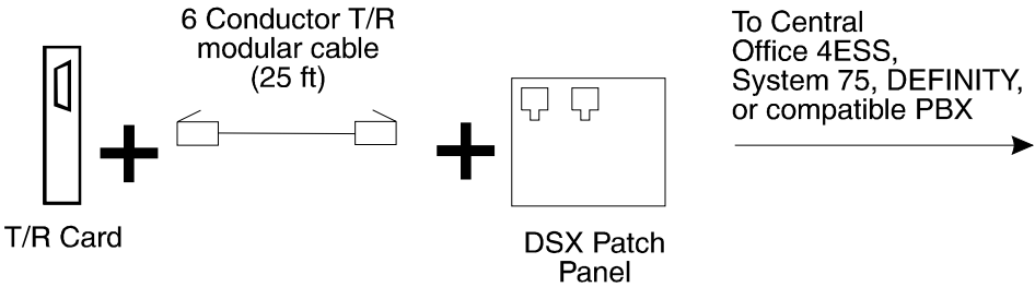
Figure 1-1. Analog Tip/Ring Interface Connection to a DSX Patch Panel
