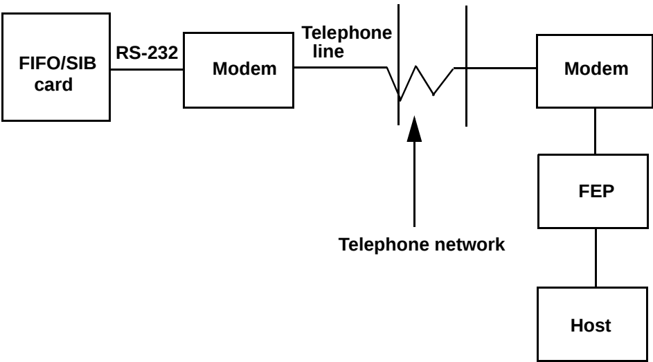
Figure 6-1. Sample Host Connection Using a Modem
