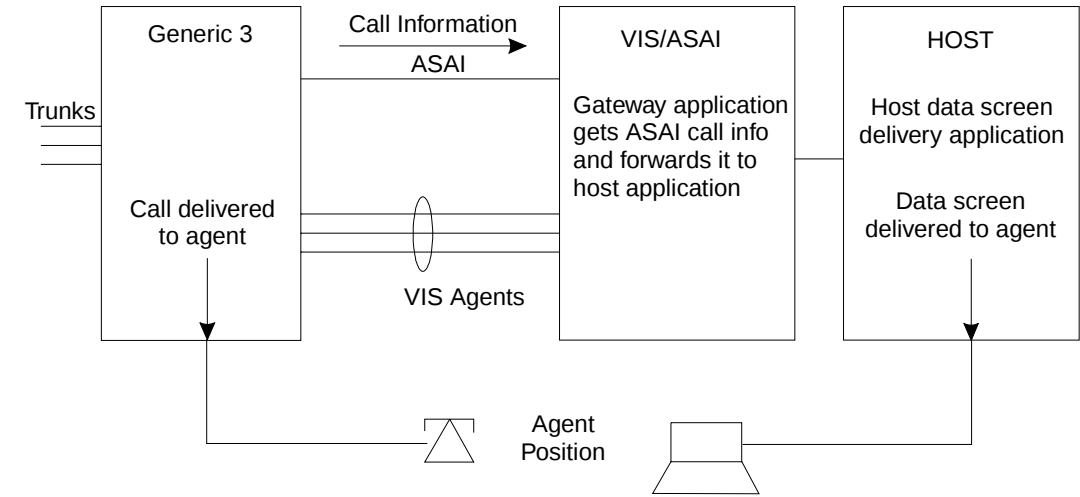
Figure 3-5. Data Screen Delivery Applications
