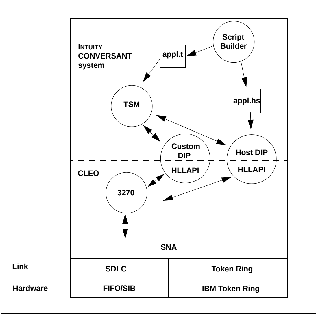
Figure 6-4. Host Interface Protocol
