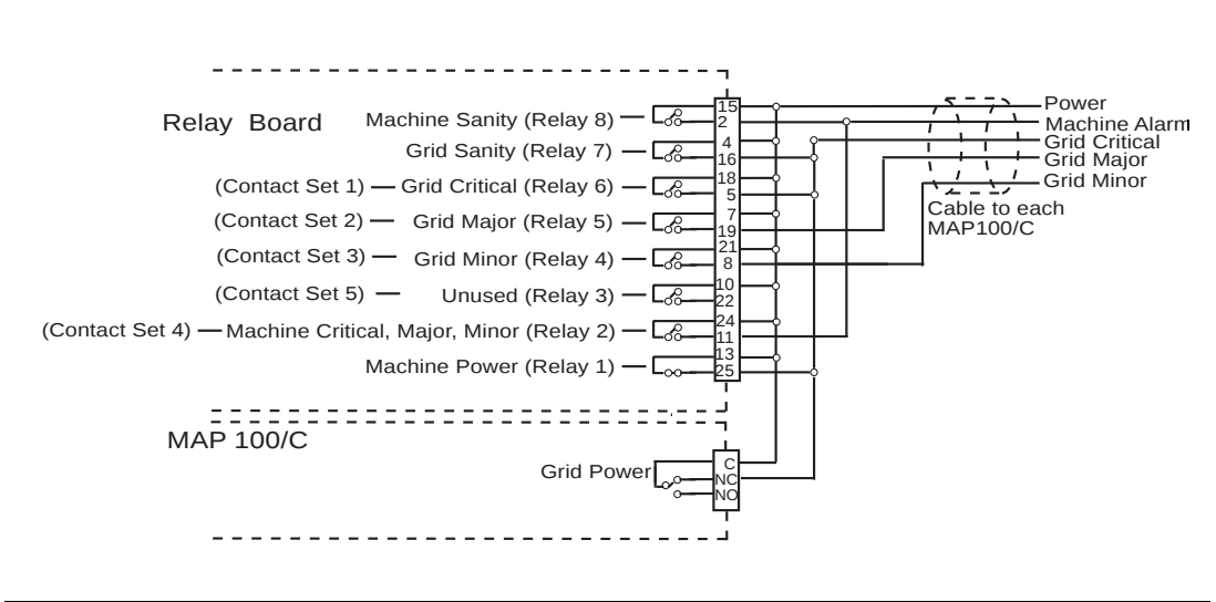
Figure 7-3. Alarm Relay Card Configured for a Central Office Application
