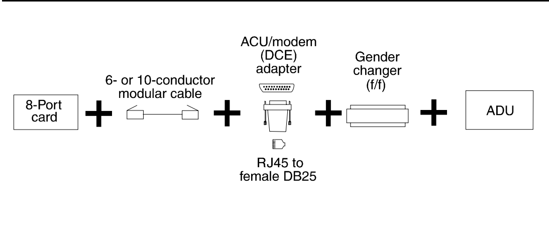
Figure 6-14. 8-port Asynchronous ADU Connection
