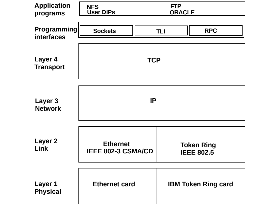
Figure 6-7. Network Layering
