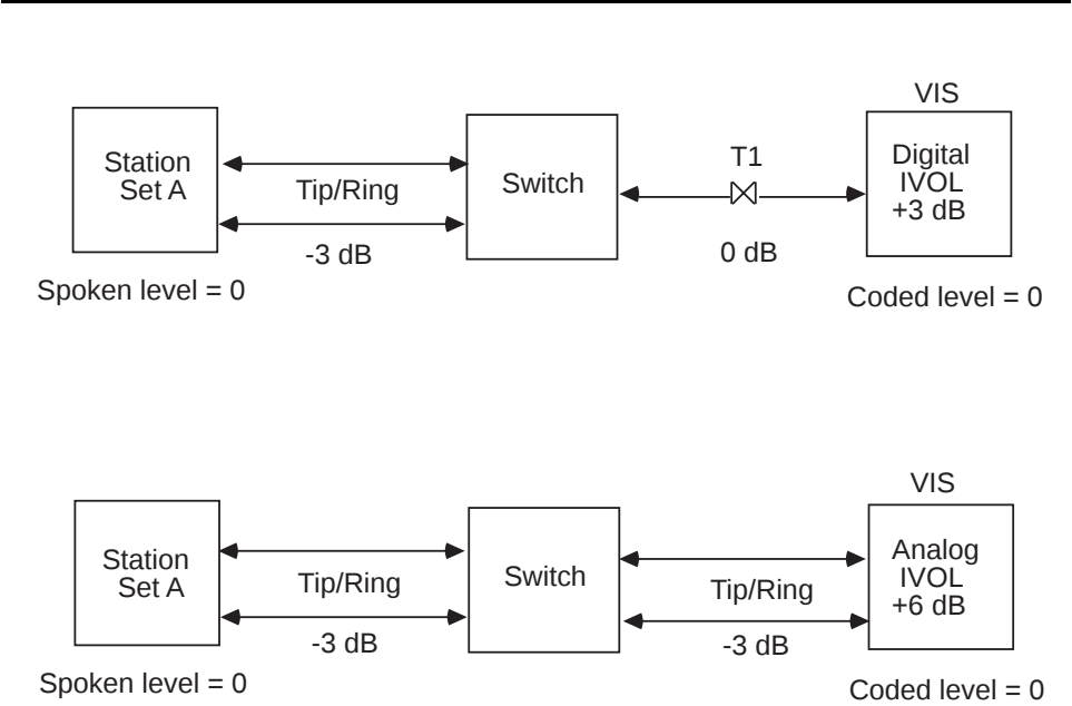
Figure A-1. Effect of IVOL Parameters on Voice Coding
