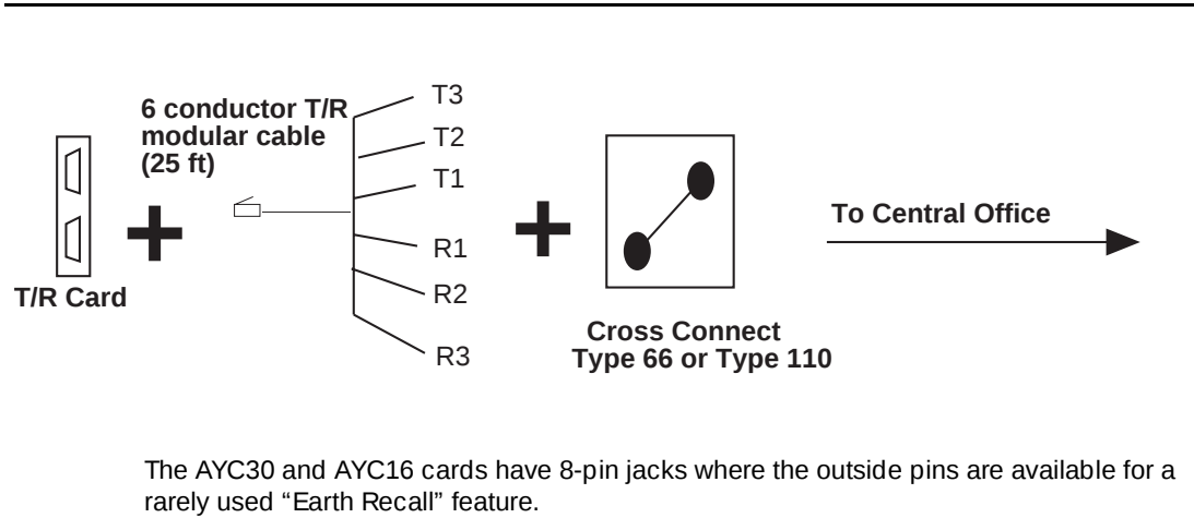
Figure 1-2. Analog Tip/Ring Interface Connection to a Type 66 or 110 Cross-Connect
