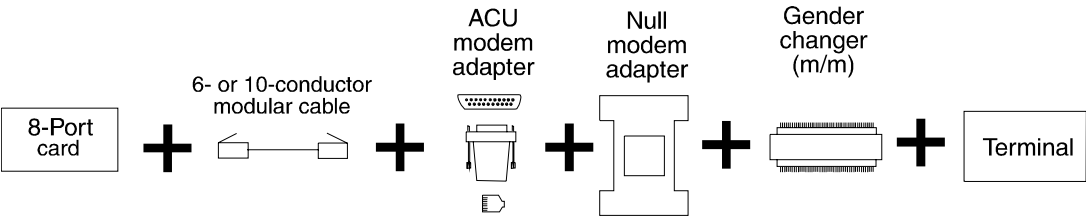
Figure 6-9. 8-port Asynchronous Terminal Connection Using 6- or 10-Conductor Modular Cable and a Null Modem
