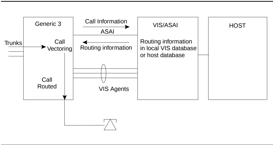
Figure 3-4. ASAI Routing Applications
