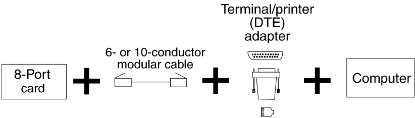
Figure 6-10. 8-port Asynchronous Computer Connection Using 6- or 10-Conductor Modular Cable
