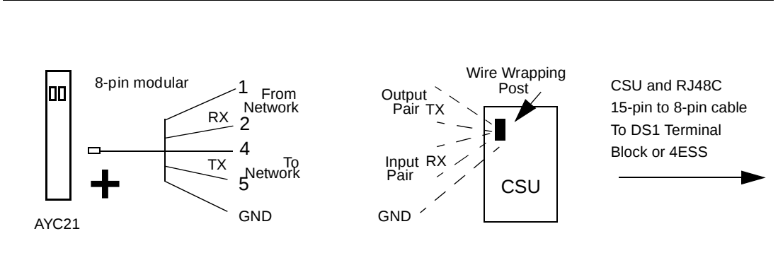
Figure 2-4. Example of AYC21 Connection to a CSU with Wire Wrapping Posts
