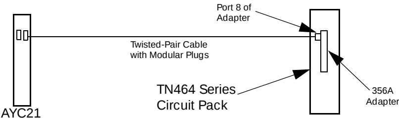
Figure 2-2. Example of AYC21 Twisted-Pair Connections to a DEFINITY G3 Switch
