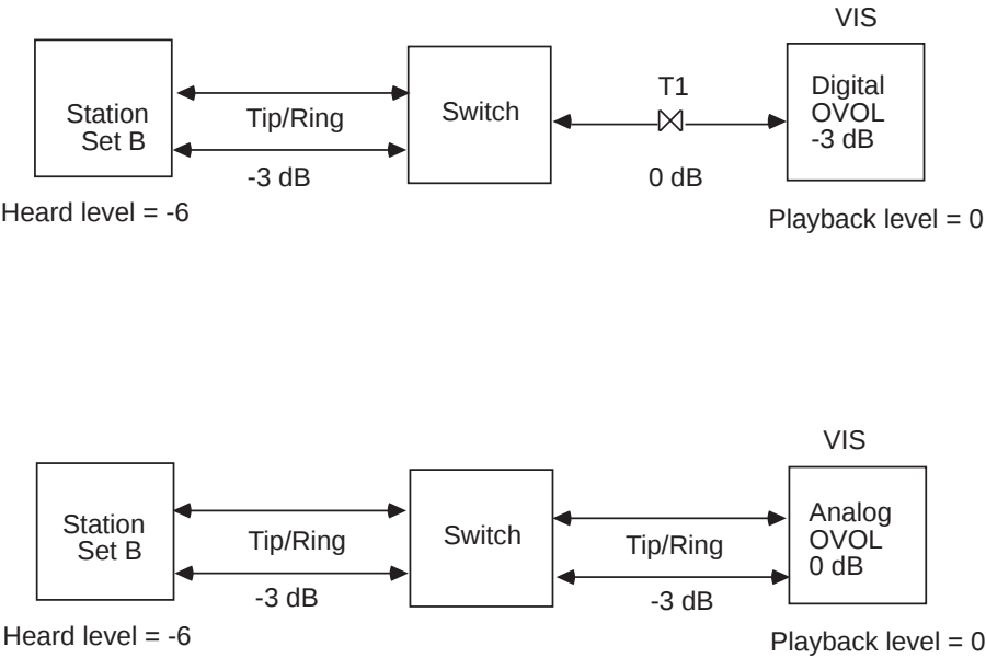
Figure A-2. Effect of OVOL Parameters on Voice Play
