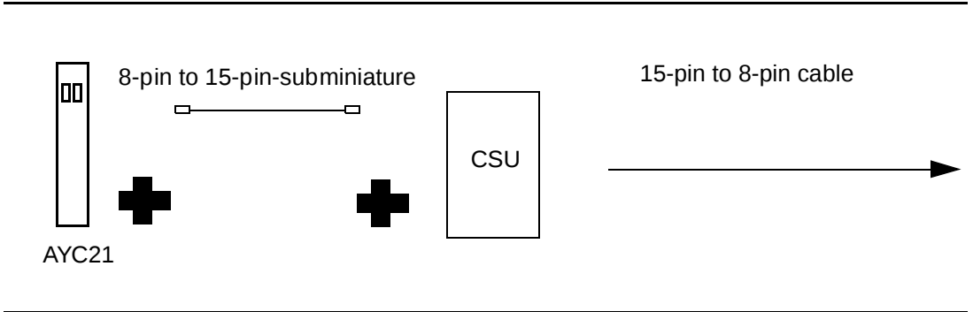
Figure 2-3. Example of T1 Interface Connection to a CSU (From an AYC21 Circuit Card)
