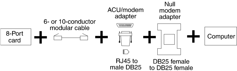
Figure 6-11. 8-port Asynchronous Computer Connection Using 6- or 10-Conductor Modular Cable and a Null Modem
