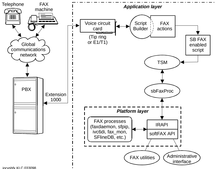
Figure 111. Script Builder FAX Actions Architecture
