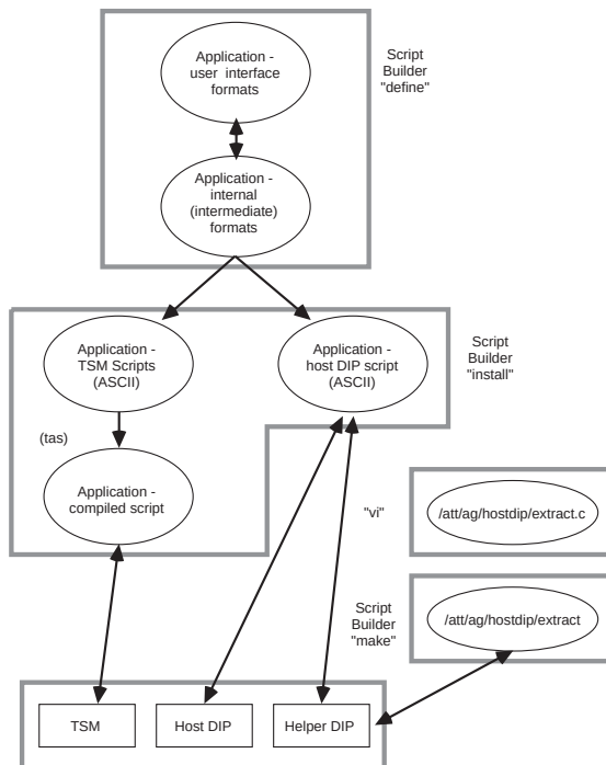
Figure 186. Script Builder Software Architecture
