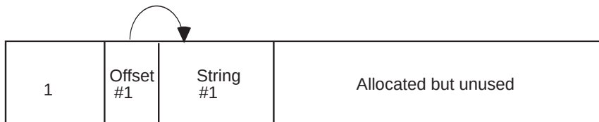
Figure 181. Execute (1 Argument)
