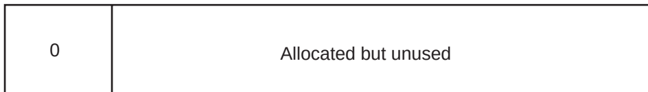
Figure 180. Execute (0 Arguments)
