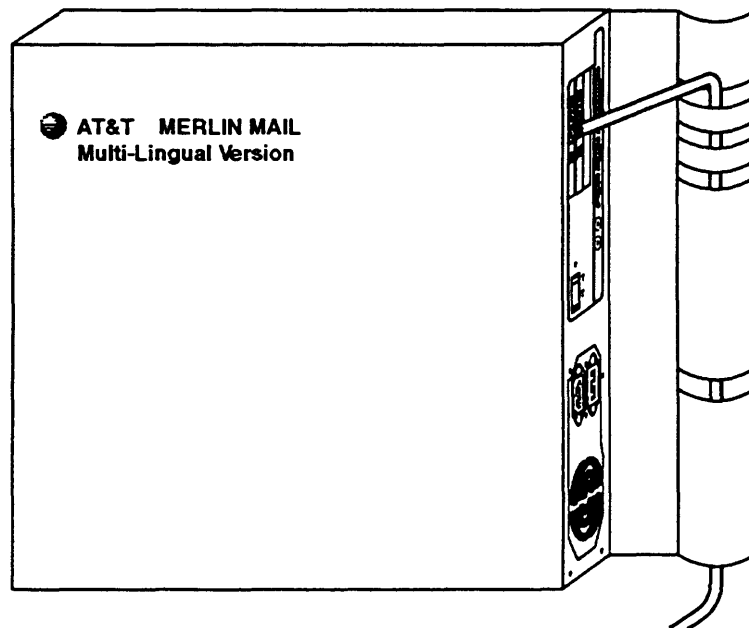
Figure 2-5. Threading Cords through the MERLIN MAIL—ML Wall Mount and Cable Manager Bracket
