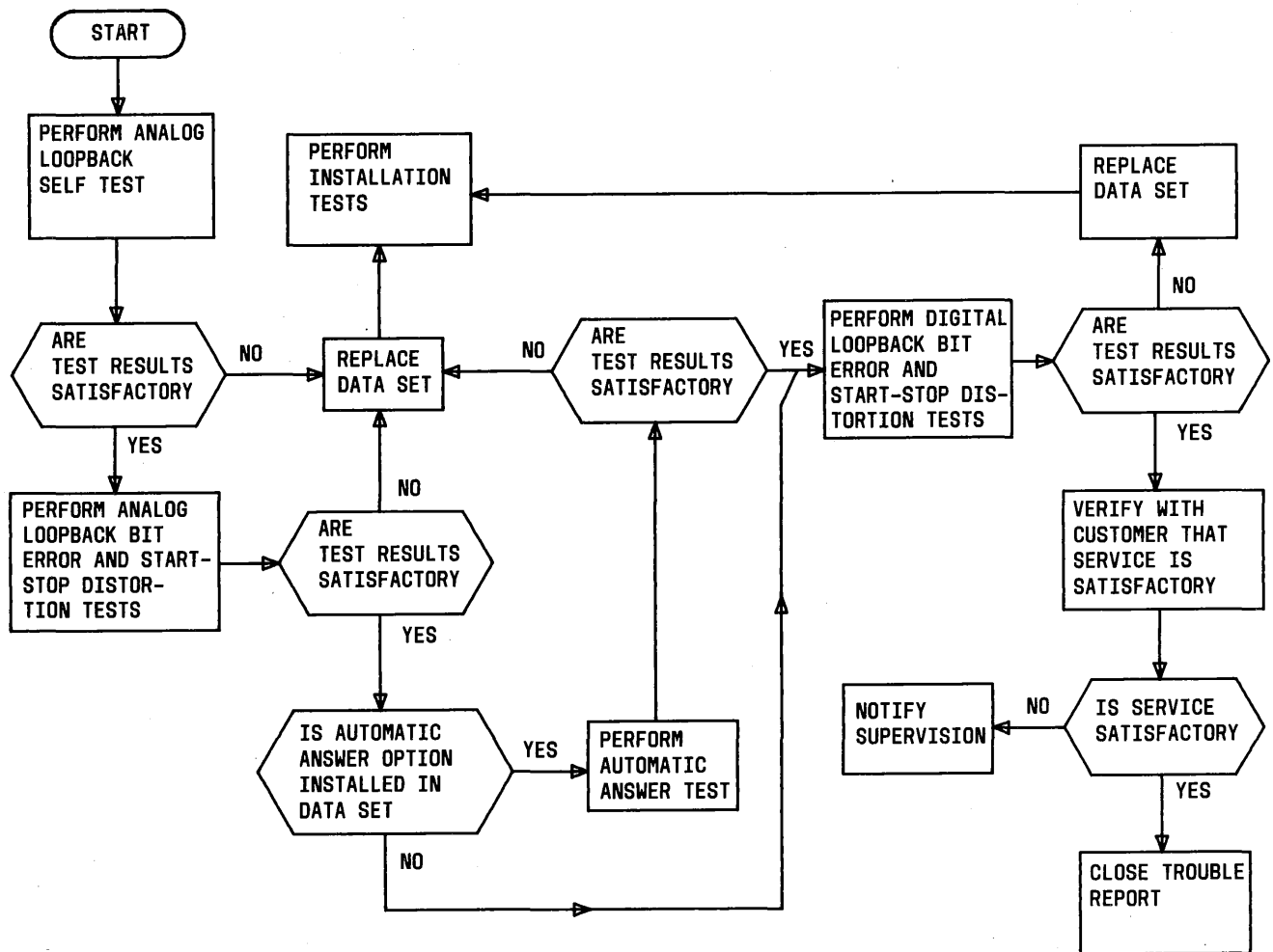
Fig. 4—Maintenance Test Sequence
