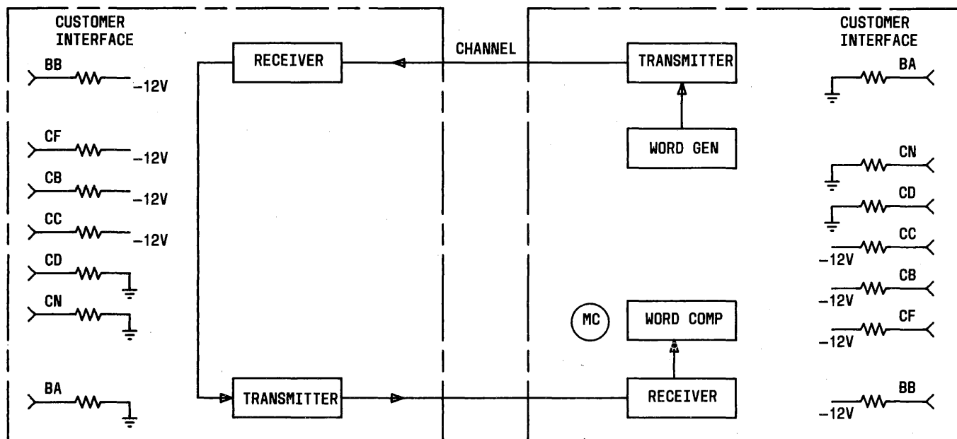
Fig. 6—Digital Loopback Self Test—Simplified Block Diagram
