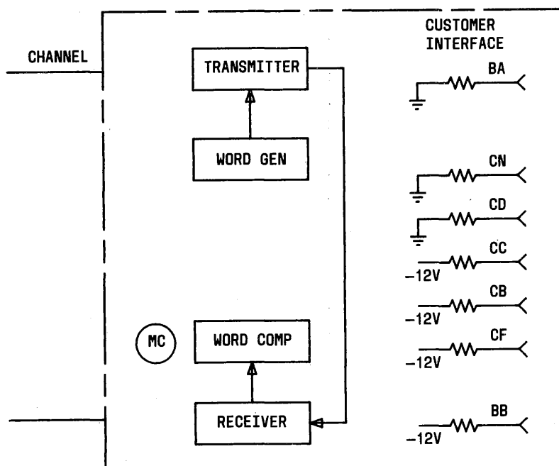
Fig. 5—Analog Loopback Self Test—Simplified Block Diagram
