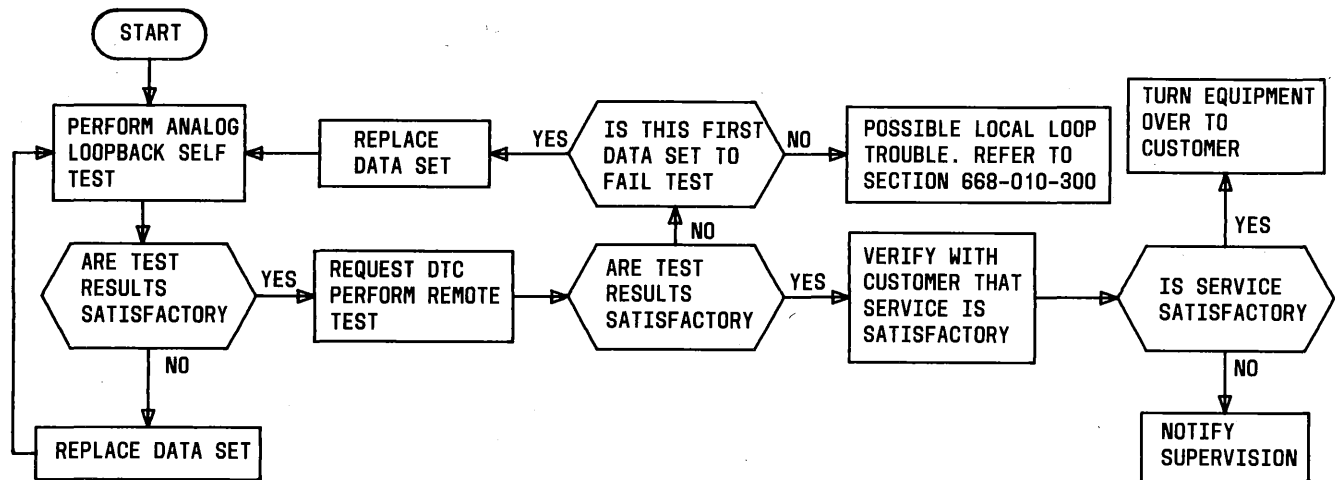
Fig. 2—Installation Test Sequence
