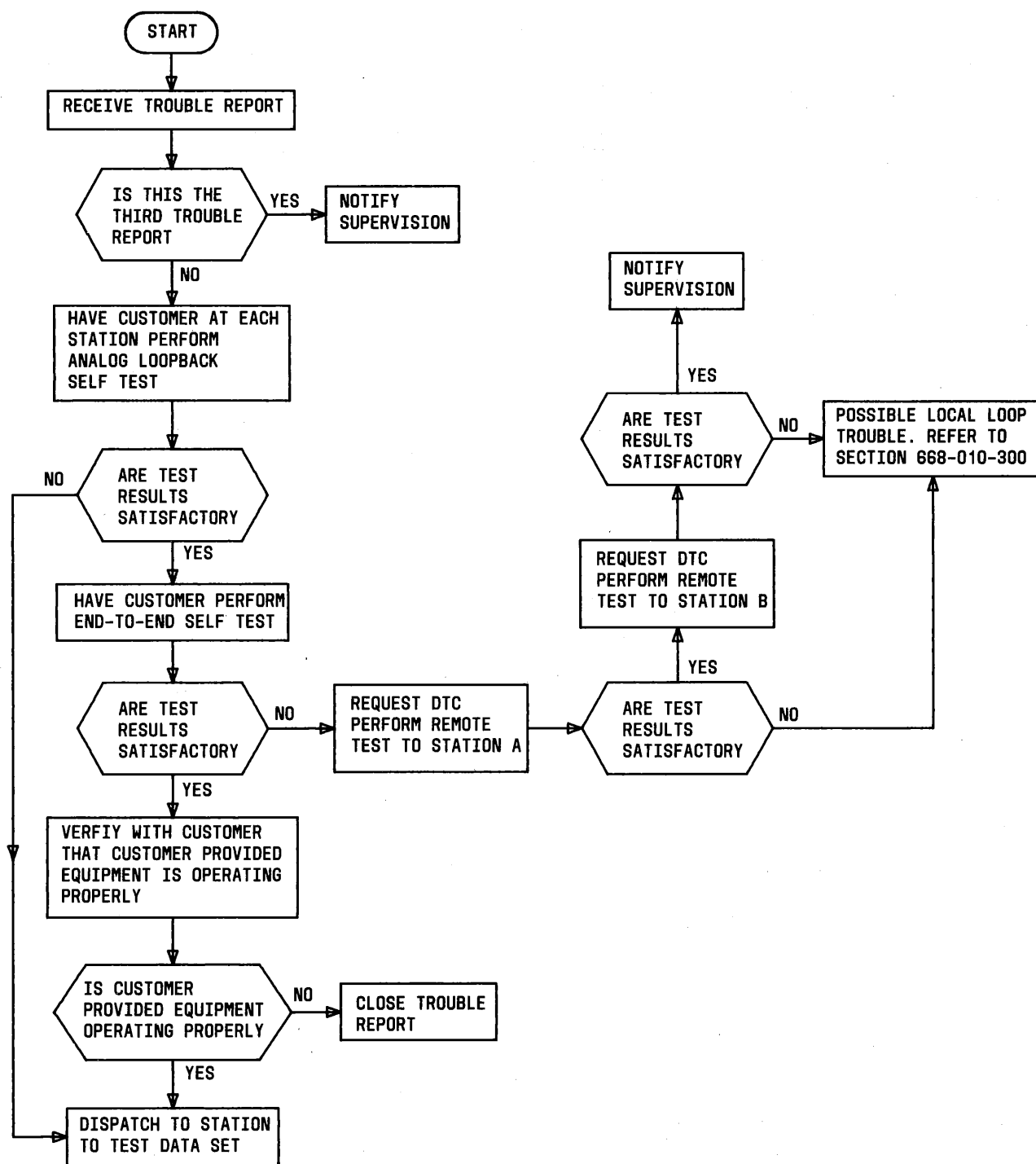
Fig. 3—Clearing Trouble Report
