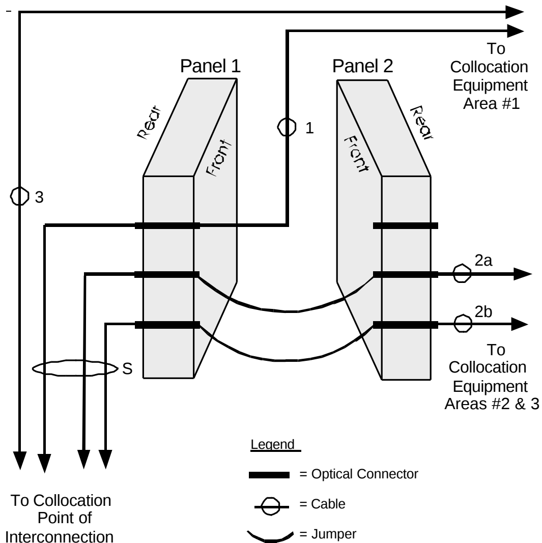
Figure 2-2 Fiber Distribution Frame Detail
