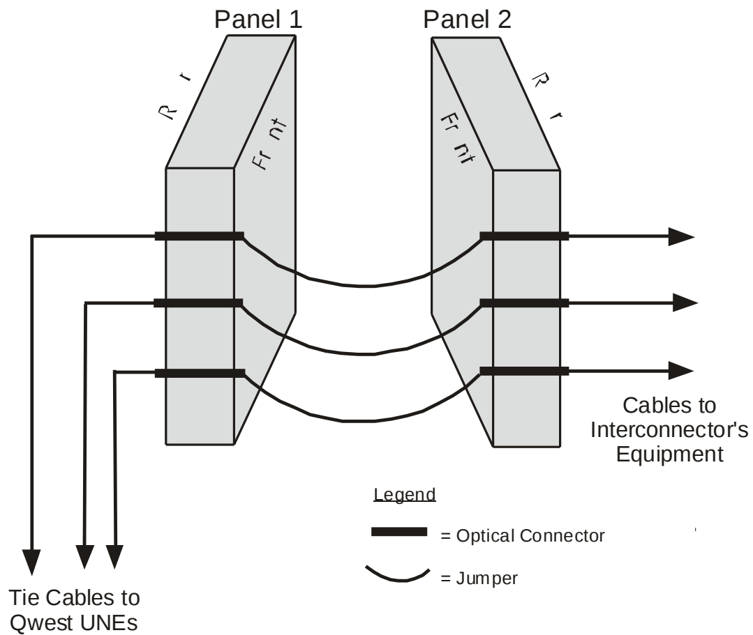
Figure 3-7: Fiber ICDF Arrangement
