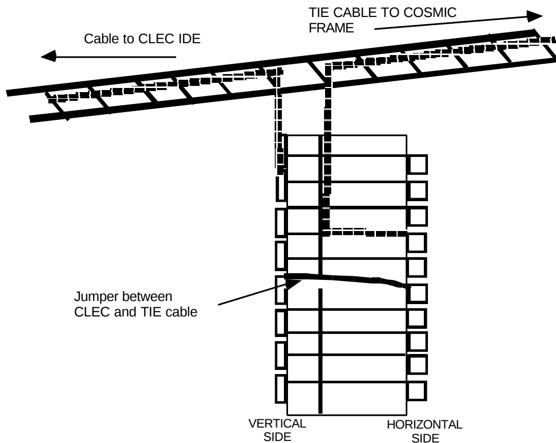
End view of InterConnection Distribution Frame (ICDF) showing typical CLEC cable termination, a jumper between the horizontal and vertical side, and a typical tie cable termination.
