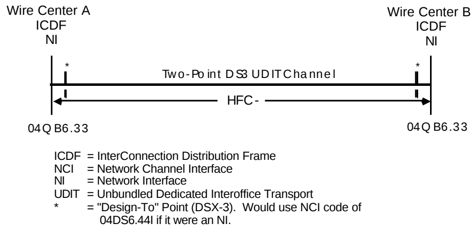
Figure B-2: Typical DS3 Two-Point UDIT UNE
