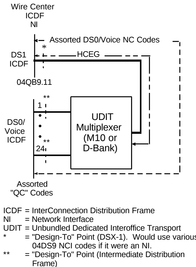
Figure B-5: Typical DS1 UDIT Multiplexer UNE.
