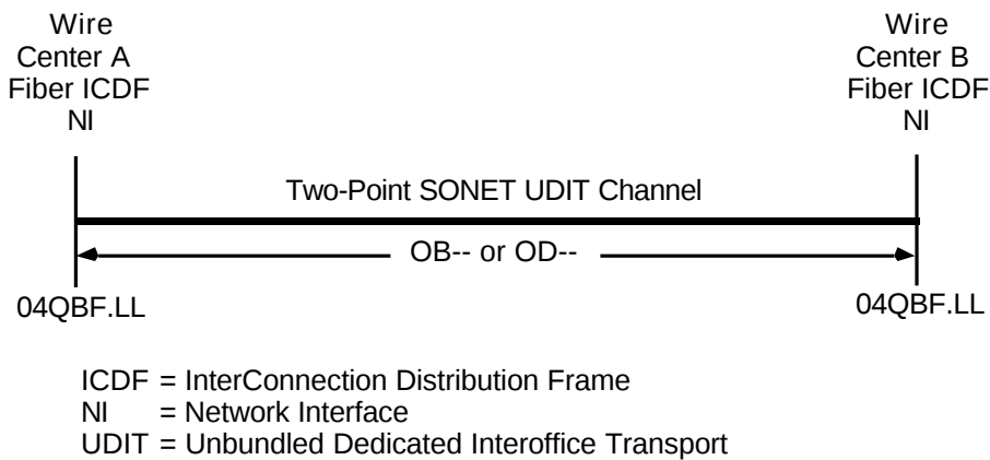
Figure B-6: Typical OC-n Two-Point UDIT Element
