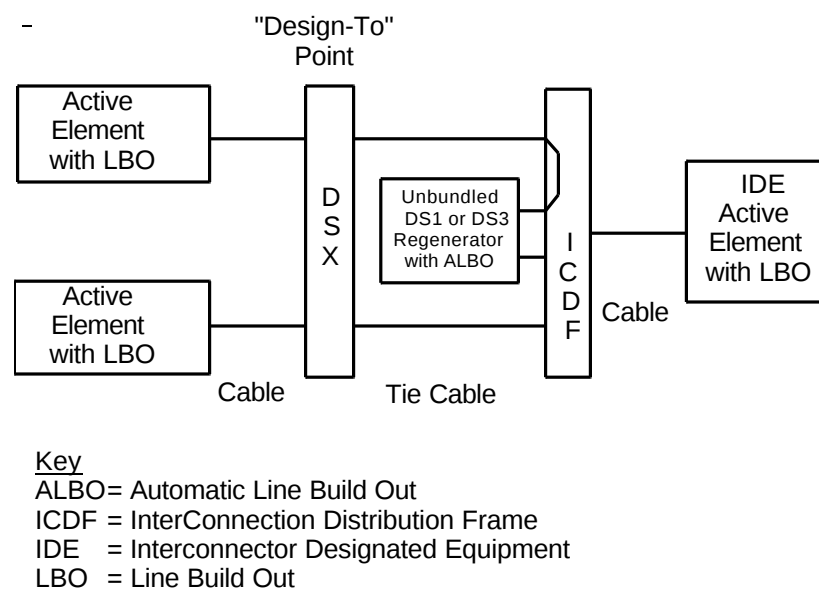
Figure 15-3: DS1 or DS3 Regenerator Option Arrangement
