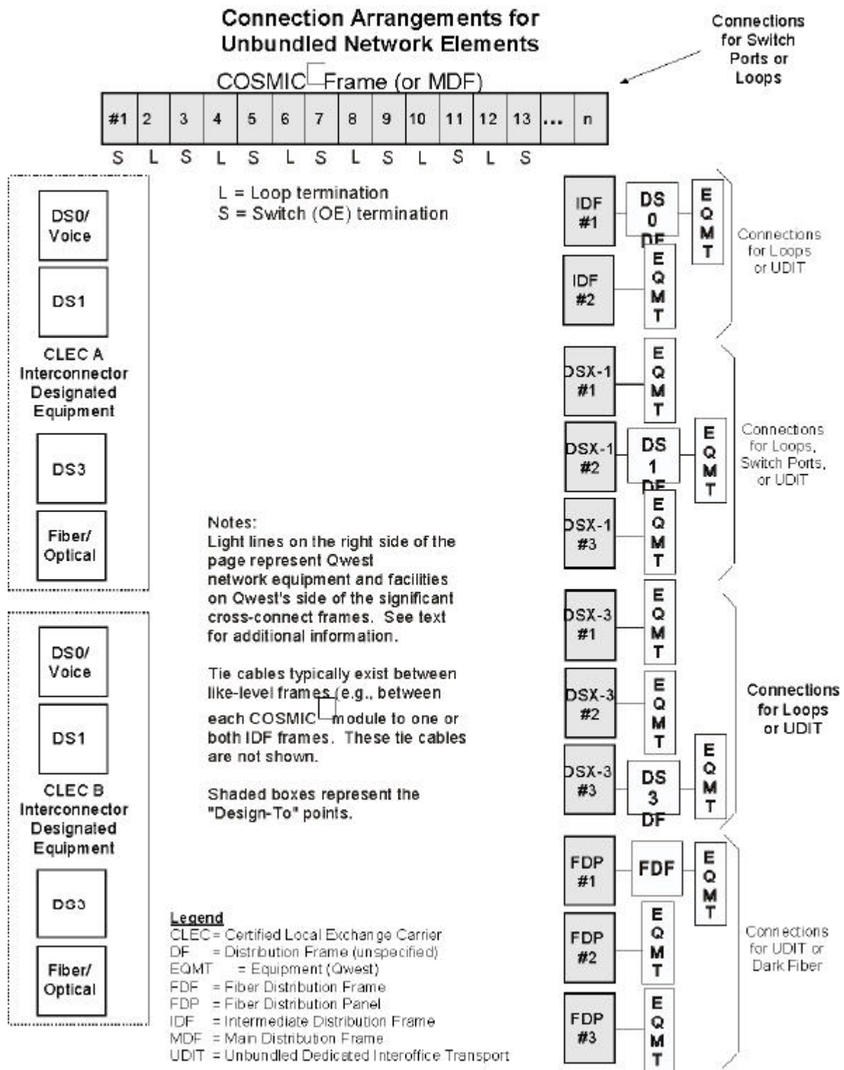
Figure 3-1 Typical Wire Center Arrangement
