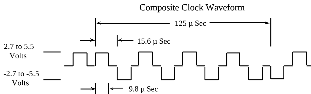
Figure 13-3: Composite Clock Waveform
