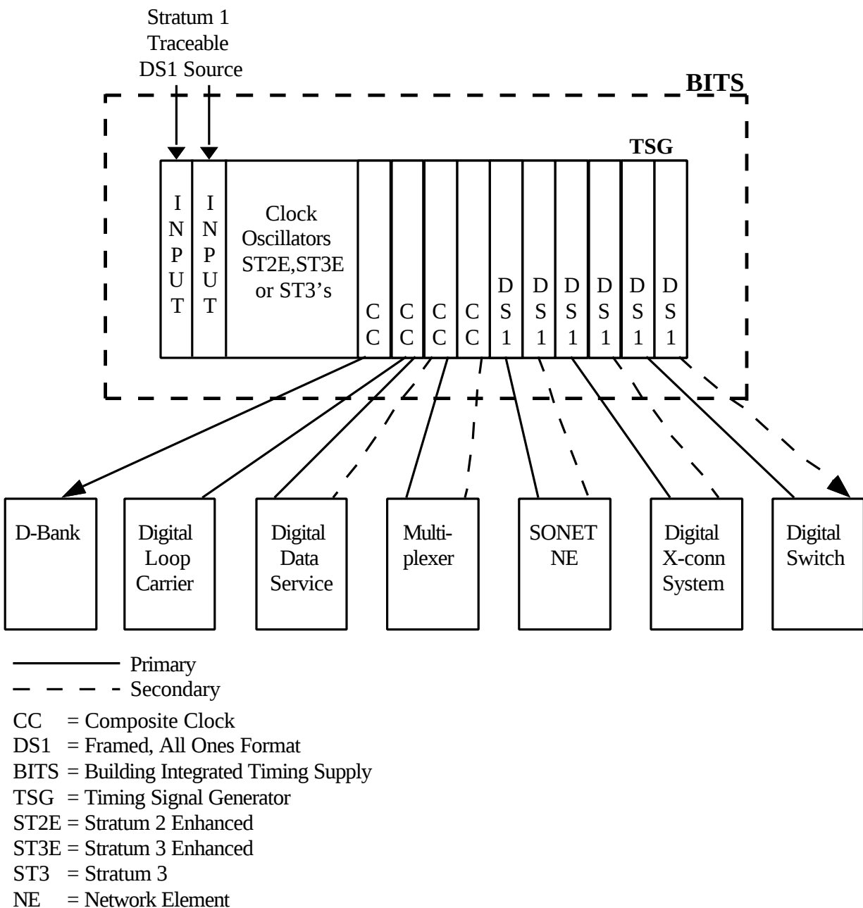
Figure 13-1: Typical QWEST BITS Arrangement
