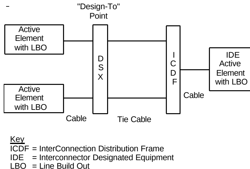
Figure 15-2: Interconnection Application
