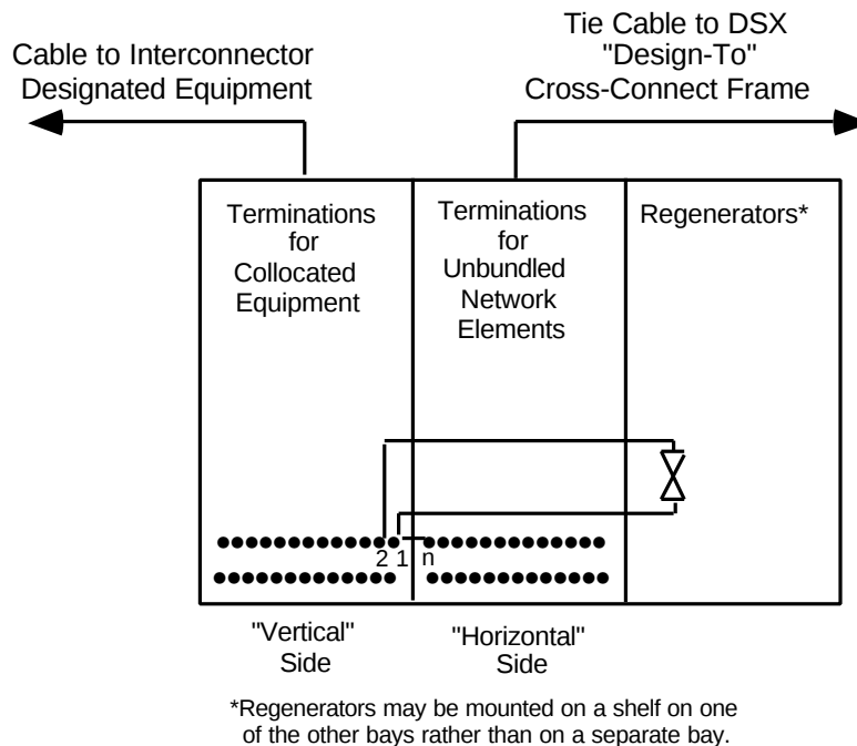
Figure 3-5 Typical DS1 or DS3 ICDF Arrangement
