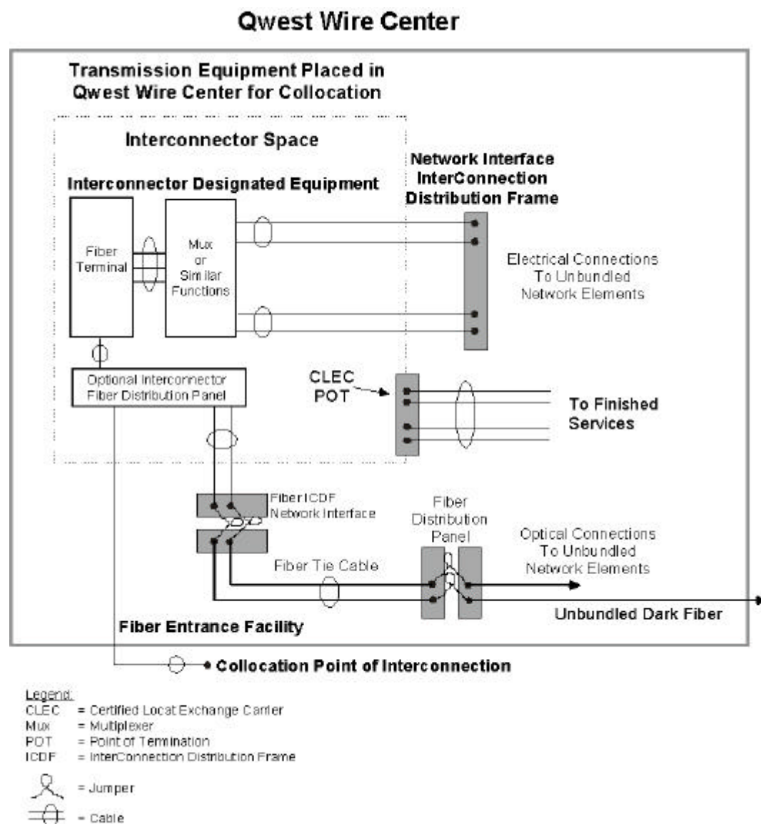
Figure 12-1: Fiber ICDF Arrangement
