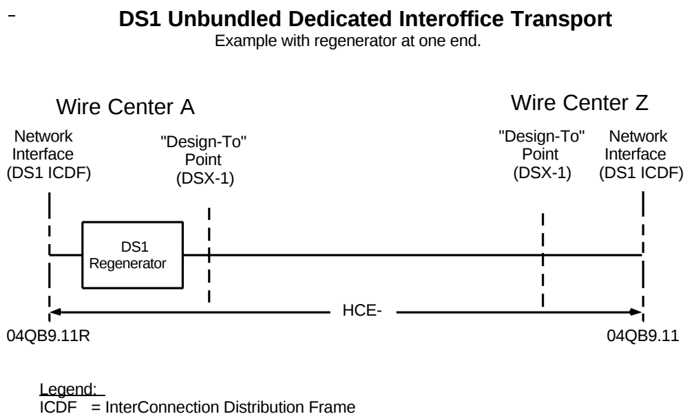
Figure 15-4: DS1 Regenerator Option Code Usage Example
