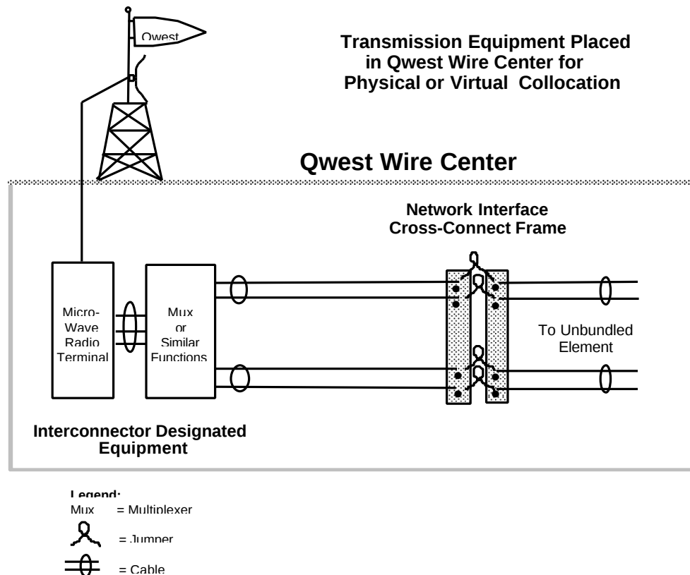
Figure 2-3 Microwave Entrance Facility Arrangement
