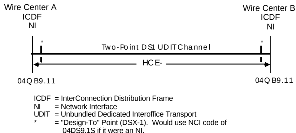
Figure B-4: Typical DS1 Two-Point UDIT UNE
