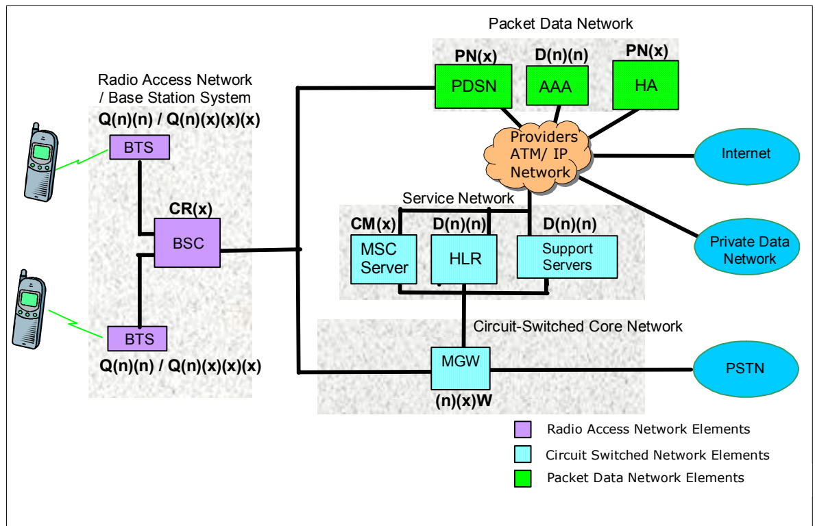
Figure 16-30 CDMA2000 3x Architecture
