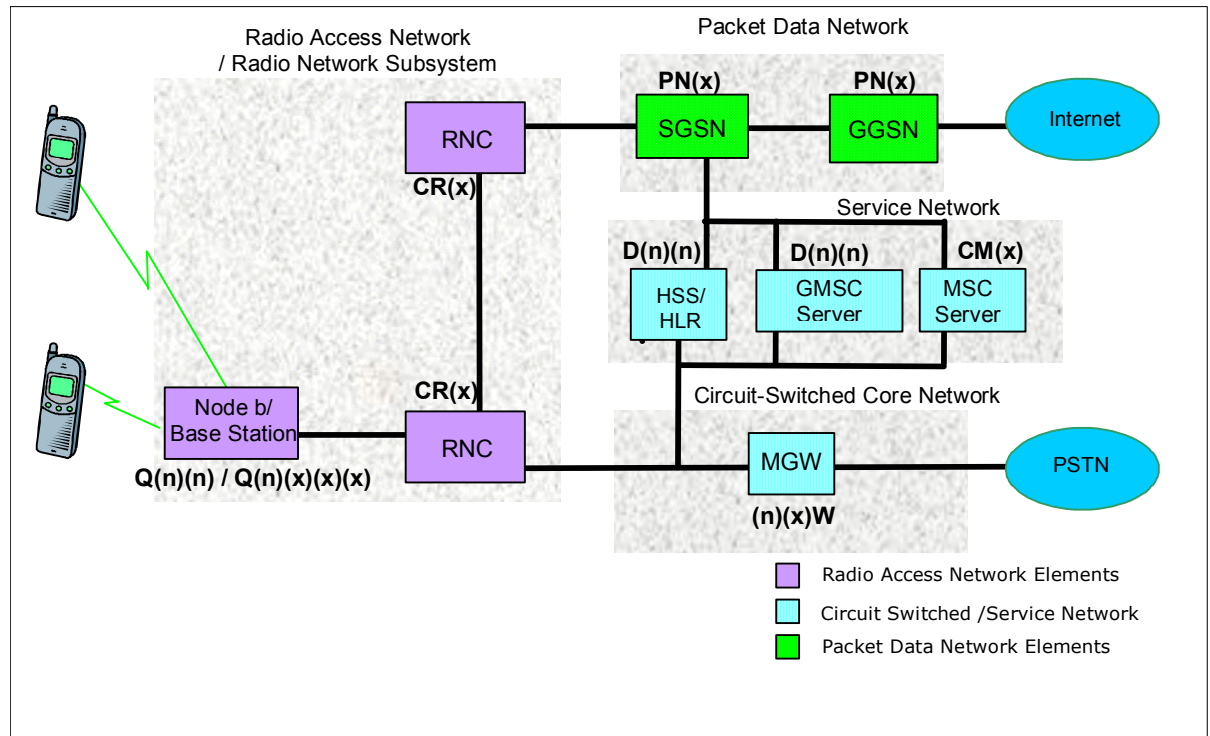
Figure 16-29 WCDMA Network Architecture 3GPP Release 4
