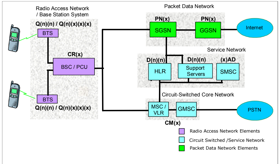
Figure 16-27 GPRS/EDGE Network
