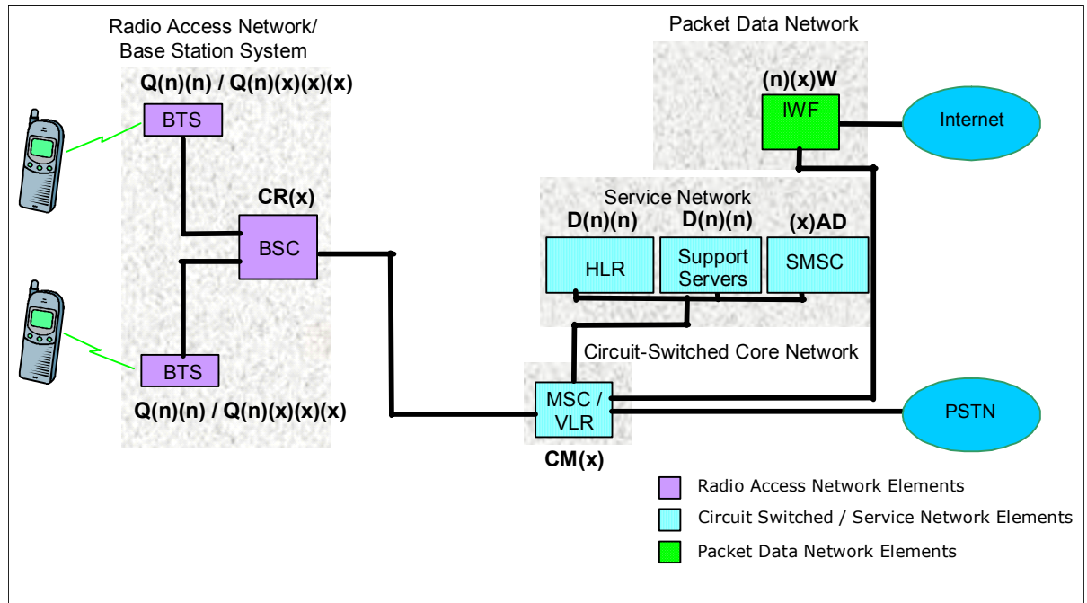
Figure 16-25 CDMAOne Network Architecture
