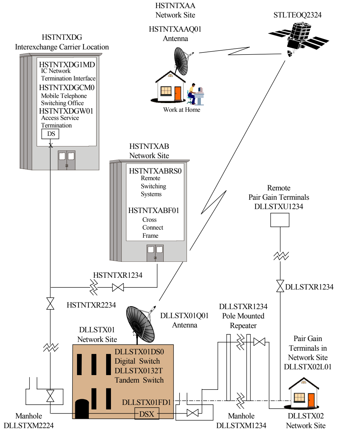
Figure 16-12 Typical Types of Network Locations Requiring CLLI Codes
