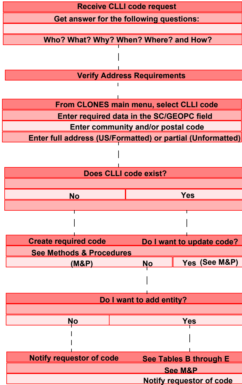
Figure 16-32 Location Coding Decision Flowchart
