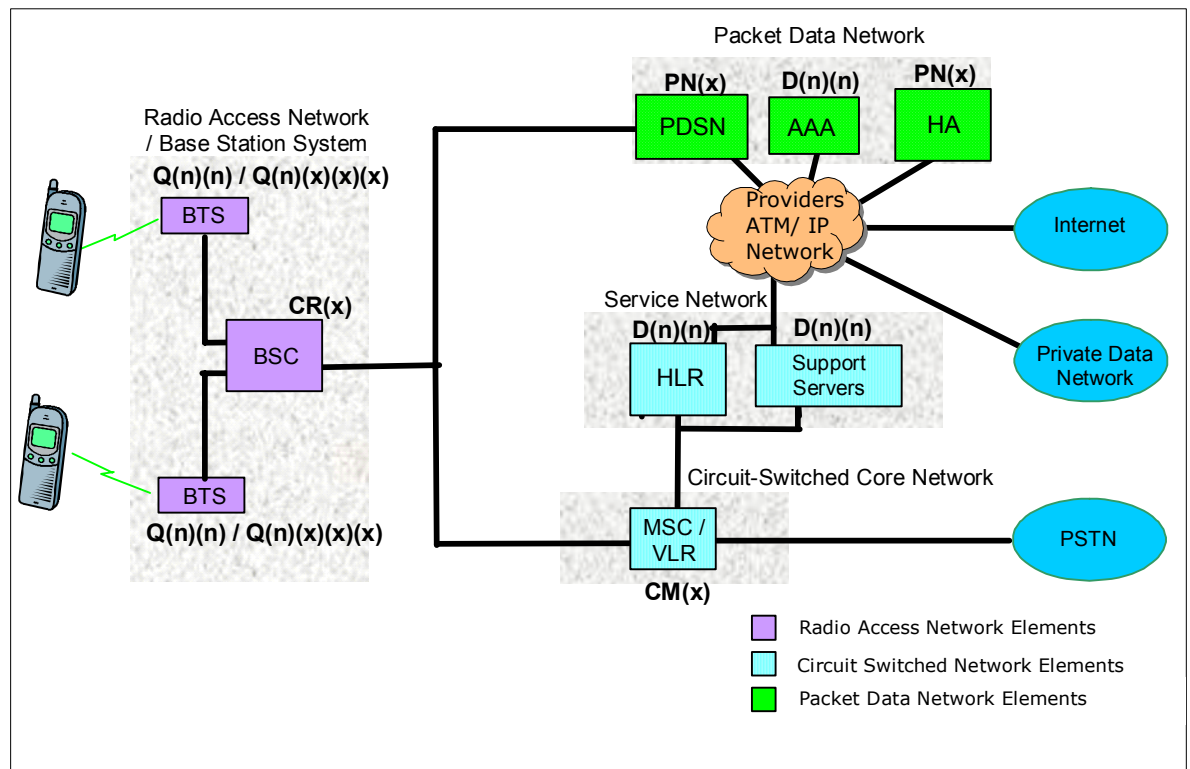
Figure 16-28 CDMA2000 1x Architecture
