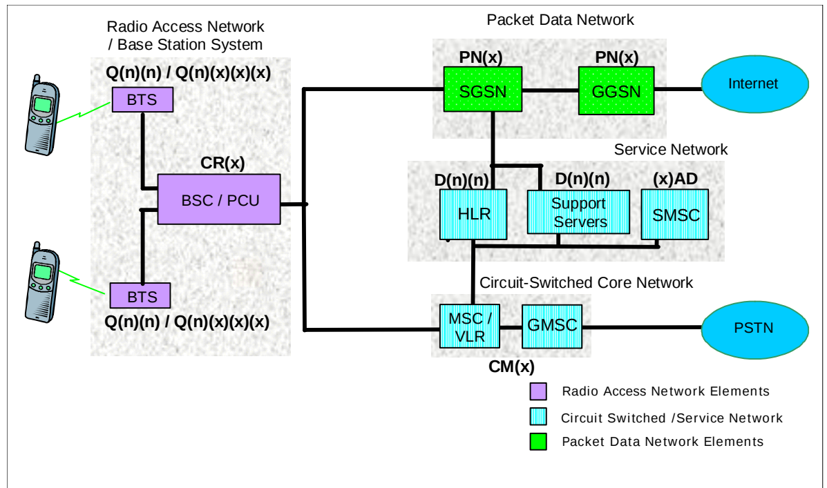
Figure 16-27 GPRS/EDGE Network
