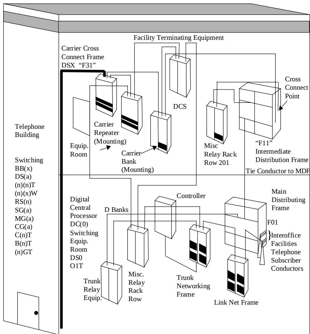
Figure 16-13 Central Office (CO) Network Entity Coding
