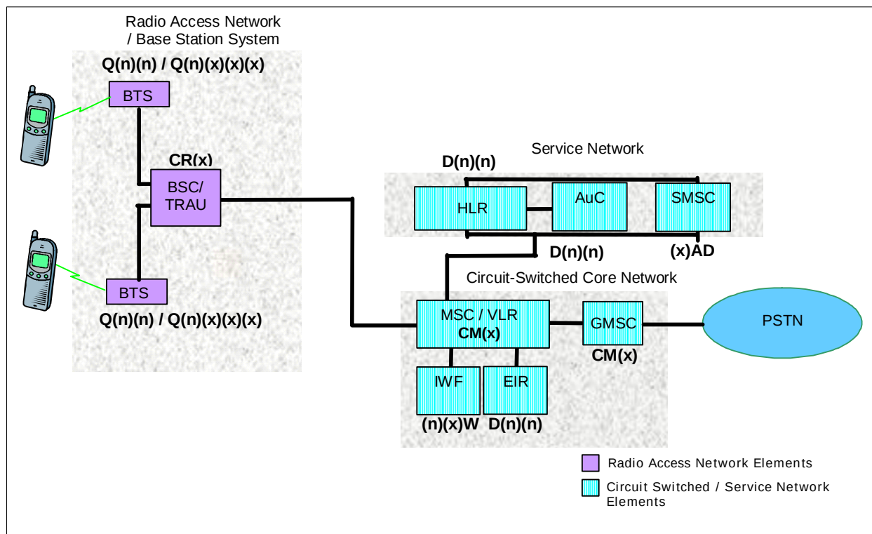
Figure 16-26 GSM Network
