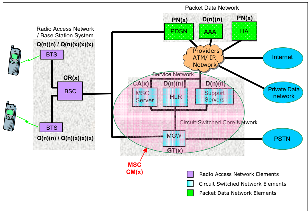
Figure 16-30 CDMA2000 3x Architecture - CM(x) Entity Code Identifies MSC Function of a Distributed MSC Architecture
