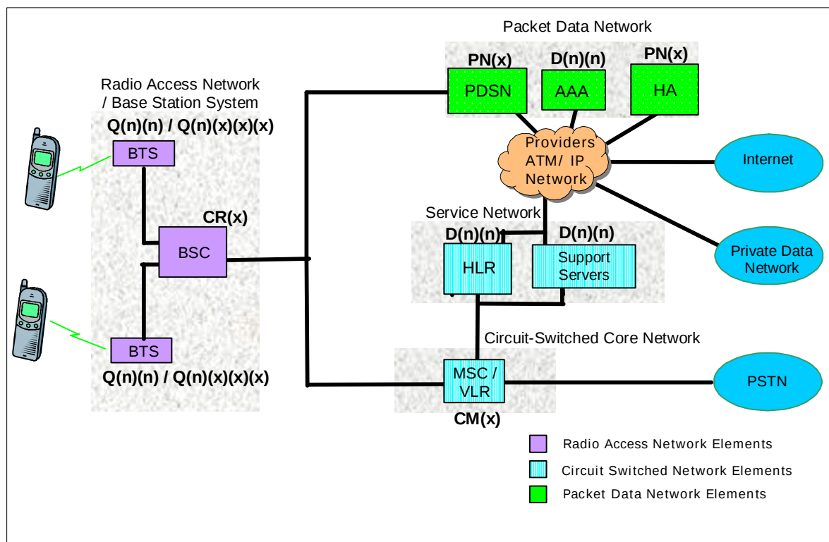
Figure 16-28 CDMA2000 1x Architecture
