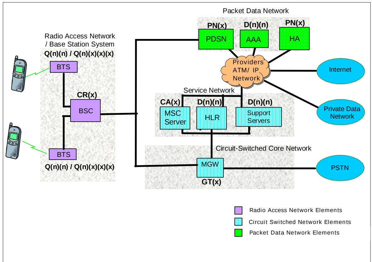
Figure 16-29 CDMA2000 3x Architecture
