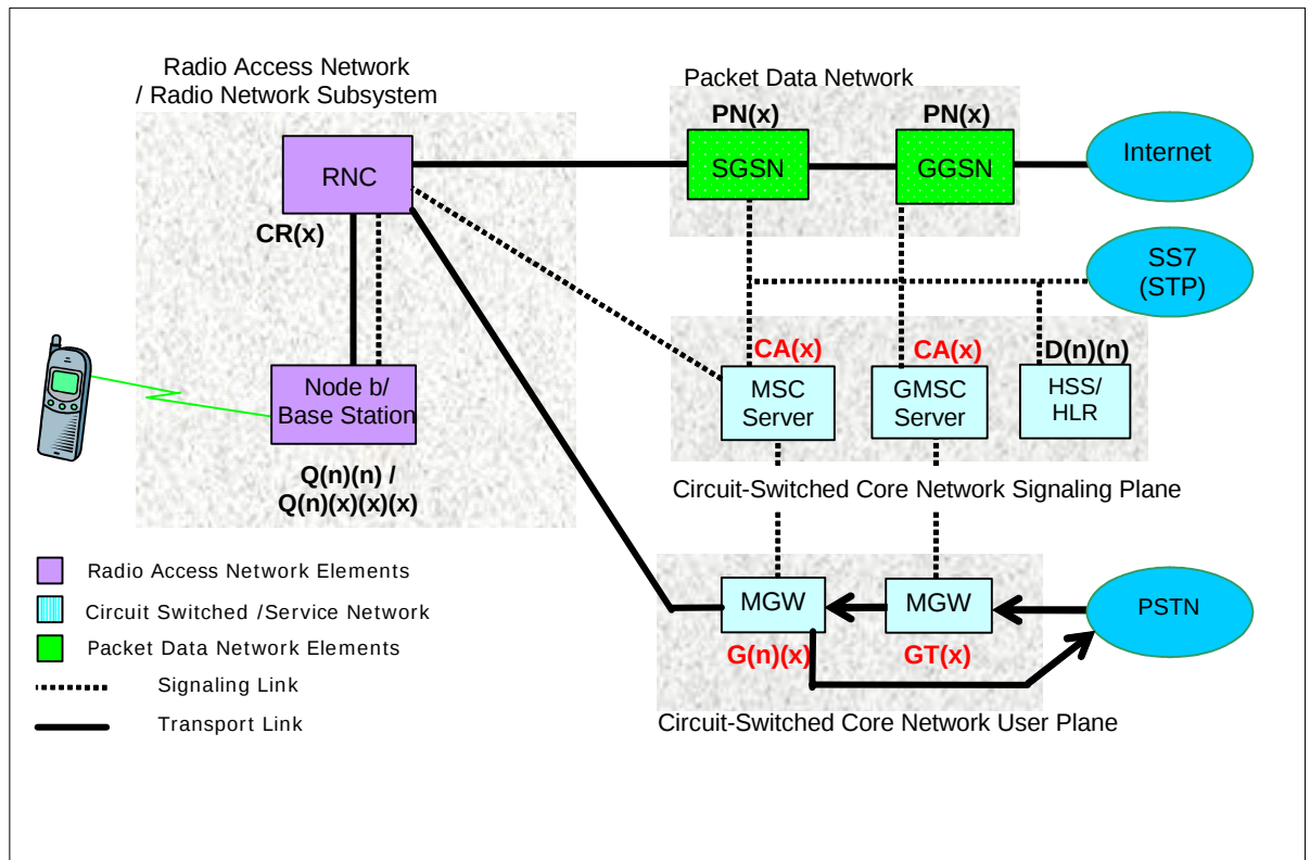
Figure 16-31 WCDMA Network Architecture 3GPP Release 4
