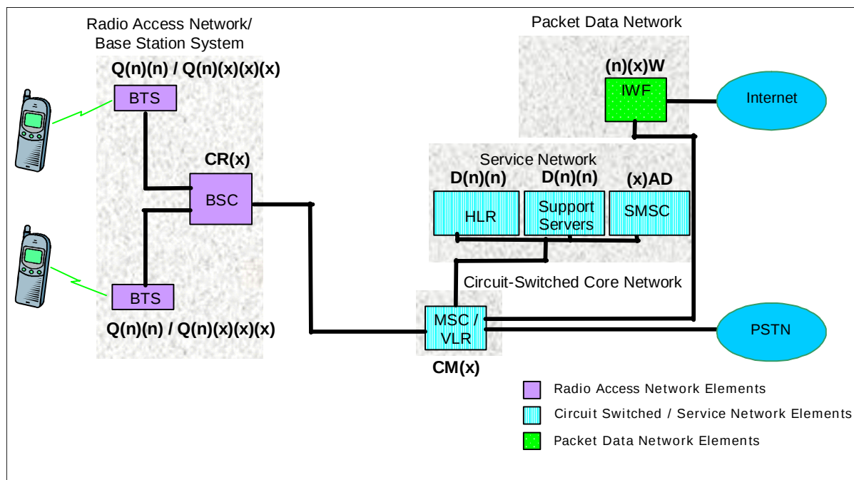
Figure 16-25 CDMAOne Network Architecture
