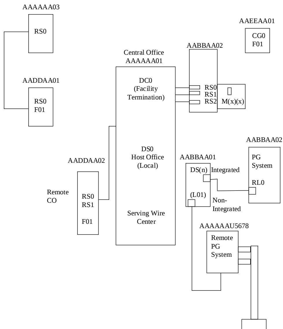
Figure 16-11 Host Office, Remote Switch, and Subscriber Line Carrier
