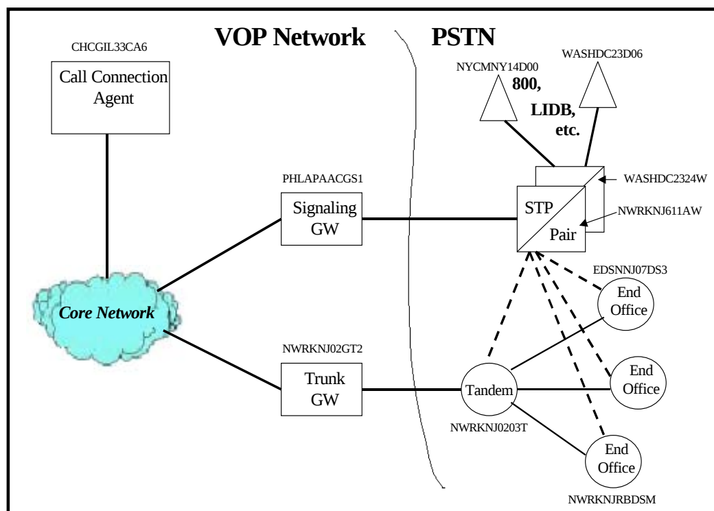
Figure 16-21 Interconnection to PSTN
