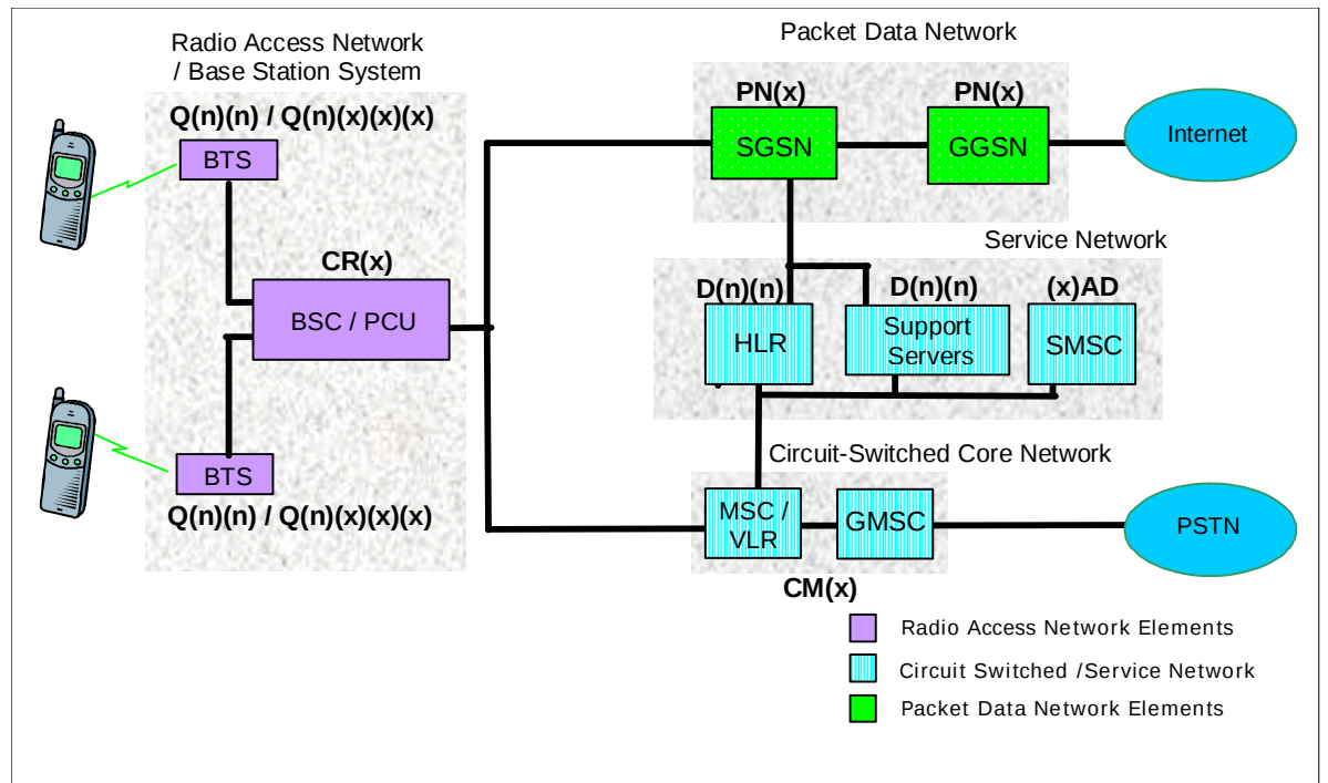
Figure 16-27 GPRS/EDGE Network
