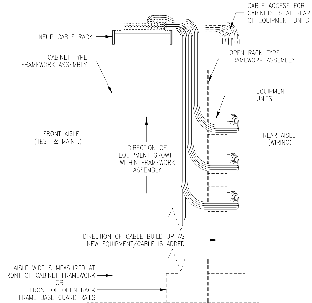
Figure 9-1 Generic Method Of Cabling Plan For Transport Equipment Frames And Cabinets
