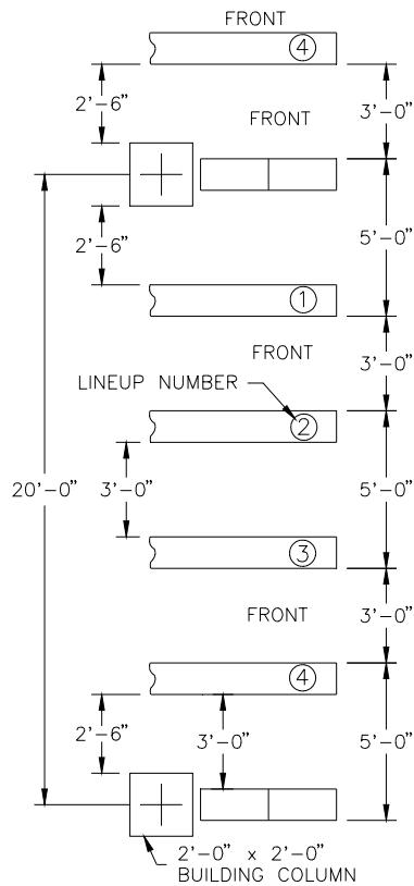
(Figure 9-2 C) Lightly Cabled Equipment And Limited Floor Space Applications
