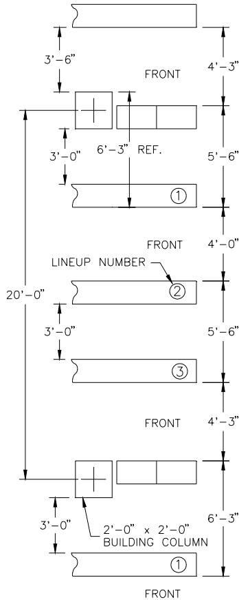
(Figure 9-3A) 1'-3" Deep Equipment Lineups
