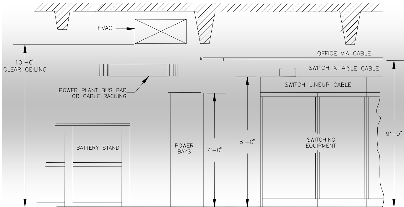
Figure 2-2a - Clear Ceiling - Power And Switching Areas
