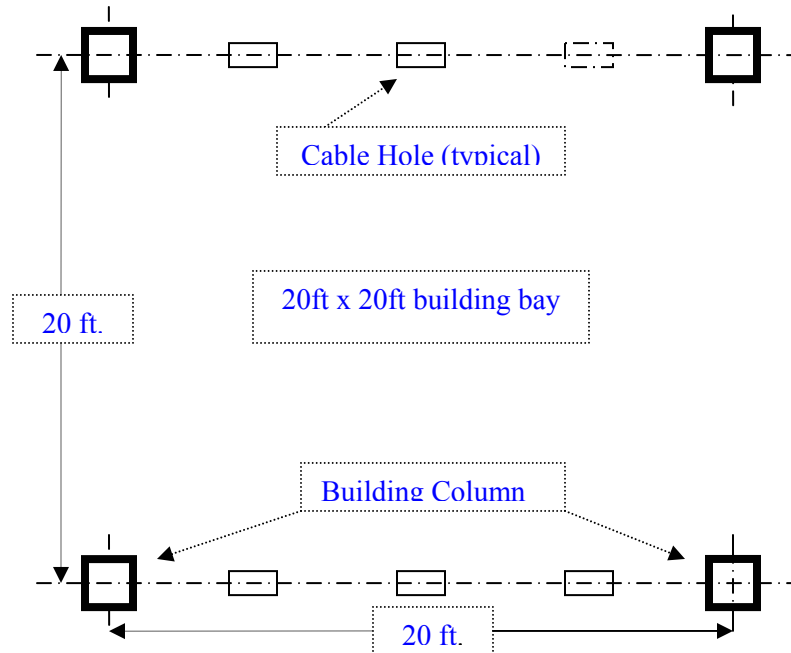
Figure 2-4 Column Spacing and Building Bay
