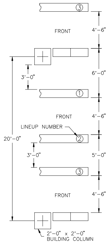
(Figure 9-2B) Preferred - Large Overhead Cable Capacity
