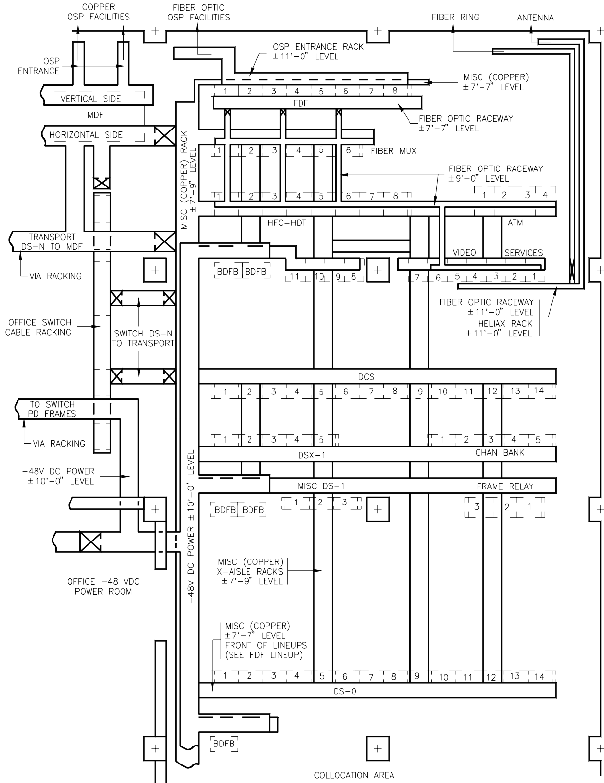
Figure 9-6 Typical Application Of Office Cable Racking To Figure 9-5 Floor Plan
