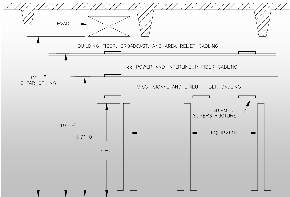
Figure 2-2b - Clear Ceiling - Transport And Collocation Areas
