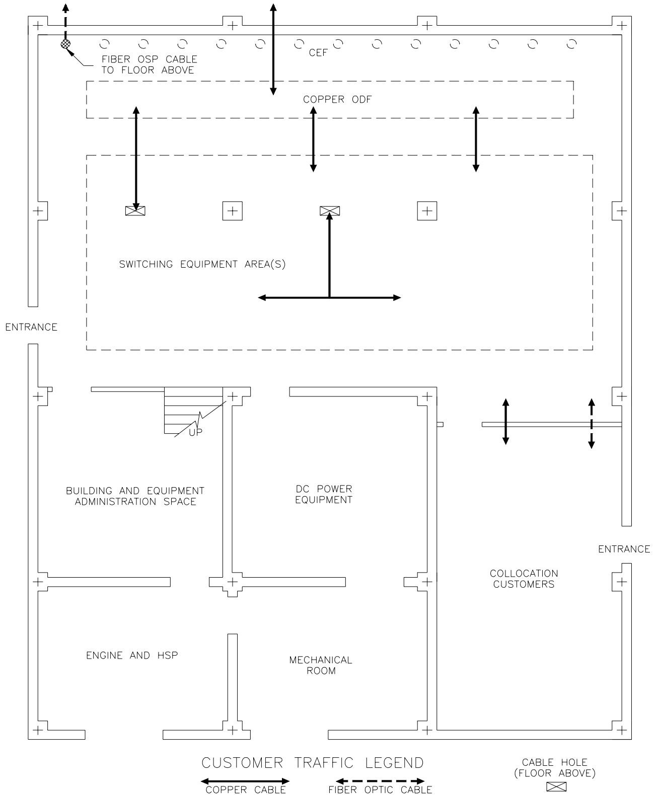
Figure 4-3 - Generic Model Of Multi-Story Network Equipment Building Switching Equipment Located On 1st Floor (see Fig. 4-4)
