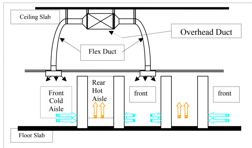
Figure 2-5 Conventional air Cooling
