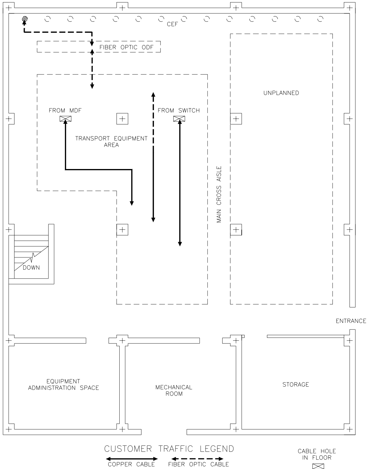
Figure 4-4- Generic Model Of Multi-Story Network Equipment Building Transport Equipment Located On 2nd Floor (see Fig. 4-3)
