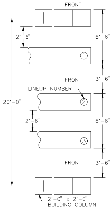
(Figure 9-3C) 2'-0" Deep Equipment Lineups
