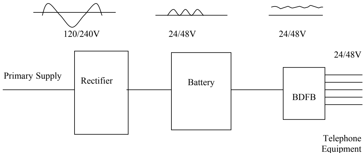
Figure 6-1 Basic Telephone Power Plant
