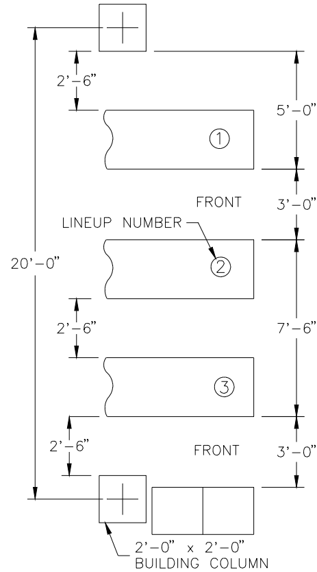
(Figure 9-4B) Limited Floor Space Applications
