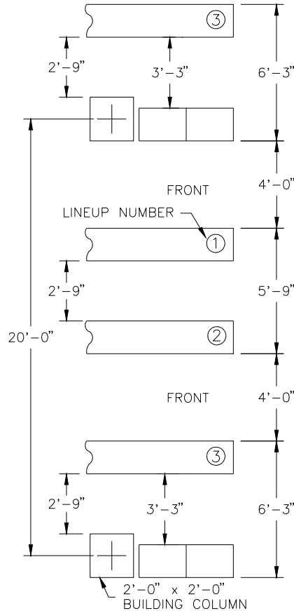
(Figure 9-3B) 1'-6" Deep Equipment Lineups
