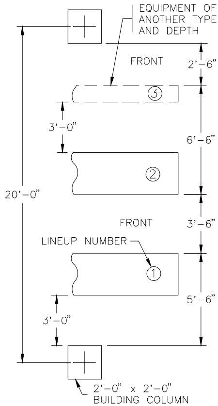
(Figure 9-4A) Preferred
