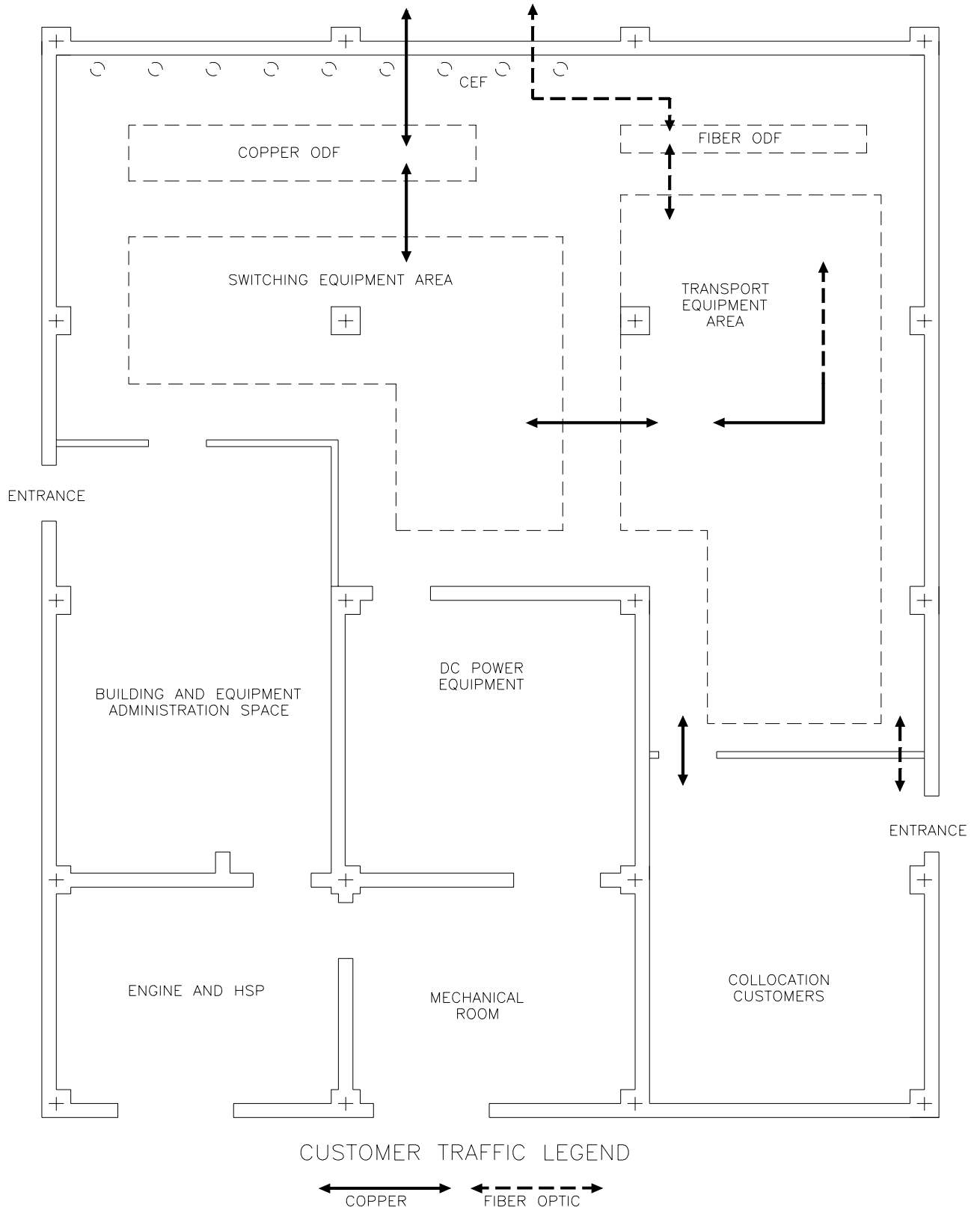
Figure 4-2- Generic Model Of Single Story Network Equipment Building
