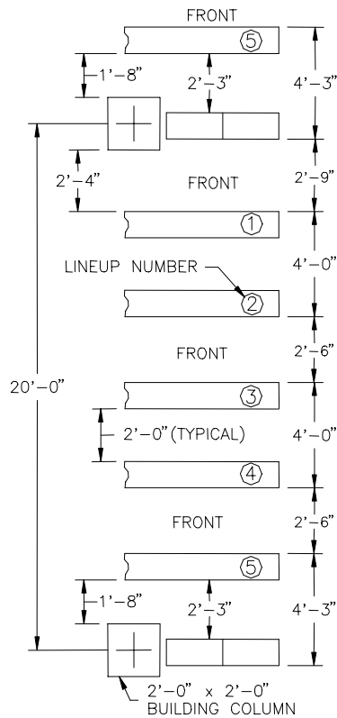
(Figure 9-2A) Traditional Telecom (Minimum) Aisle Spacing
