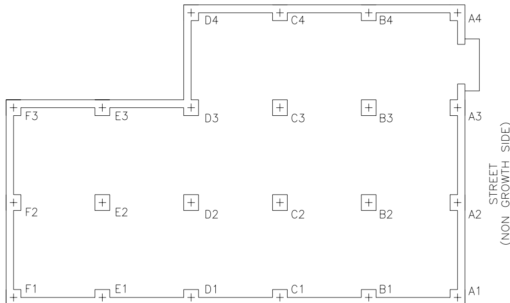
Fig 2-3 Column Designation Plan (not to scale)
