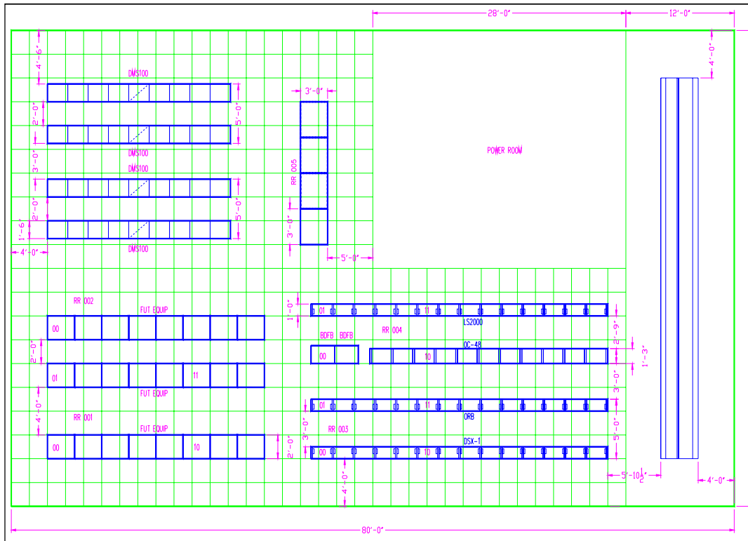
Figure 14-1 Generic Model of Equipment Layout on Raised Floors
