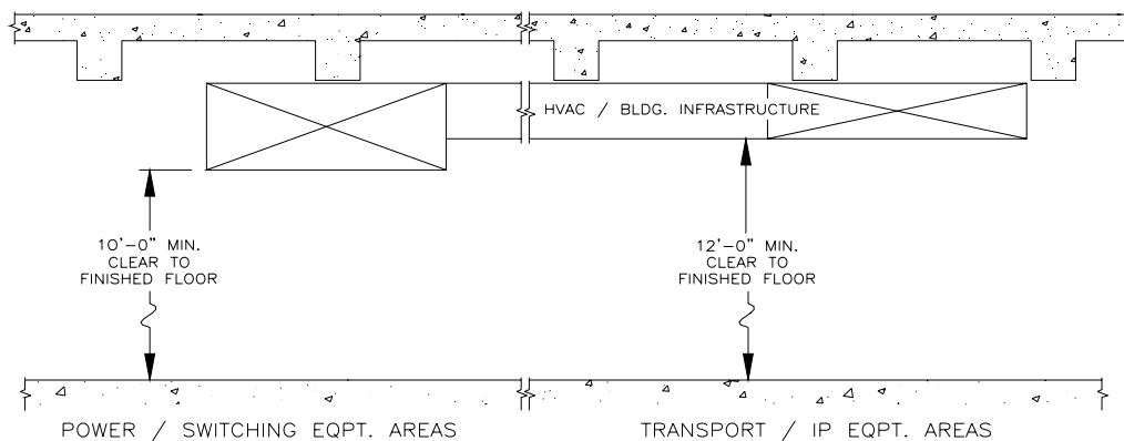
Figure 2-2 Minimum Clear Ceiling Height Requirements
