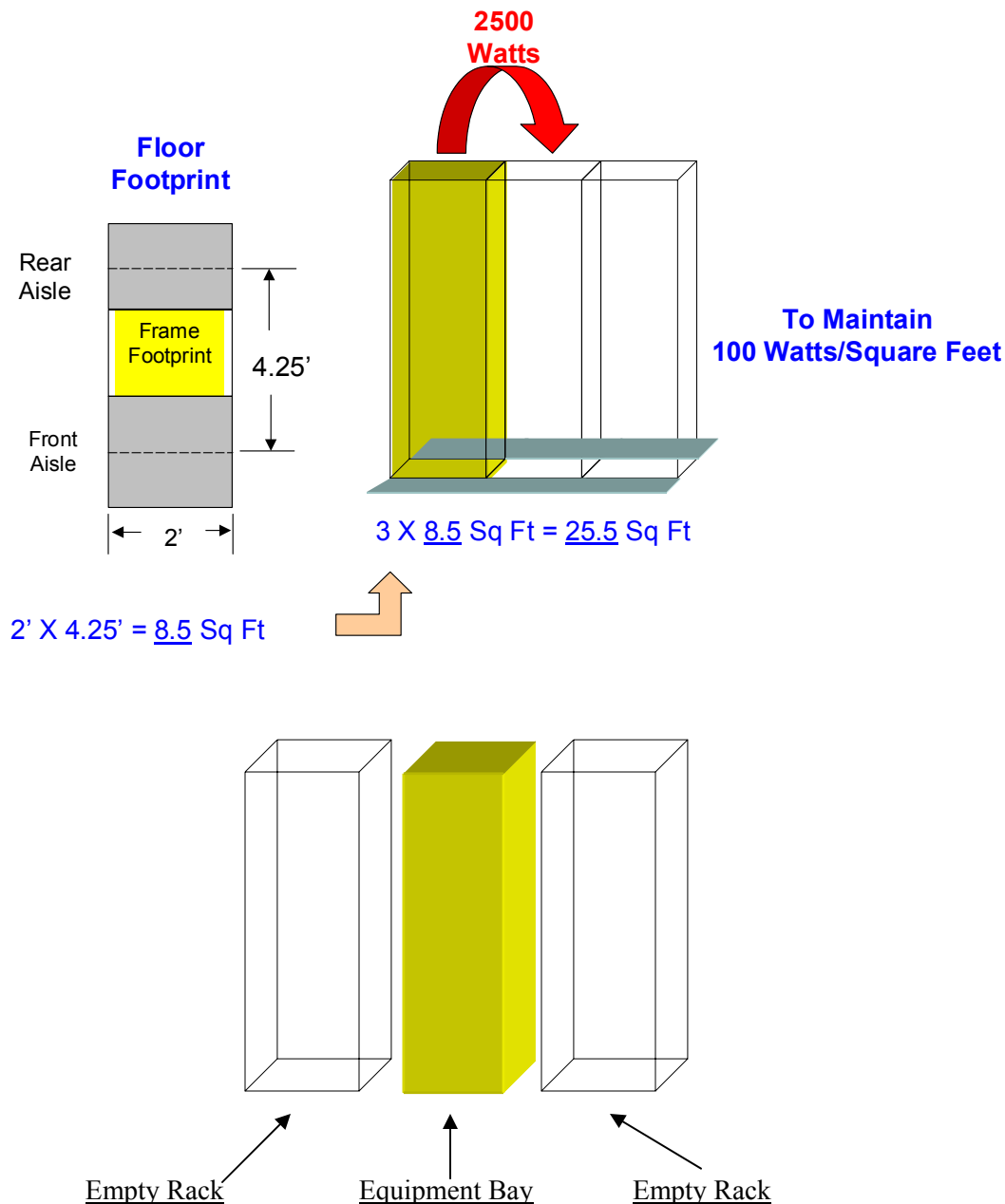
Fig 4-1 Examples of High Heat Dissipating Equipment Placement
