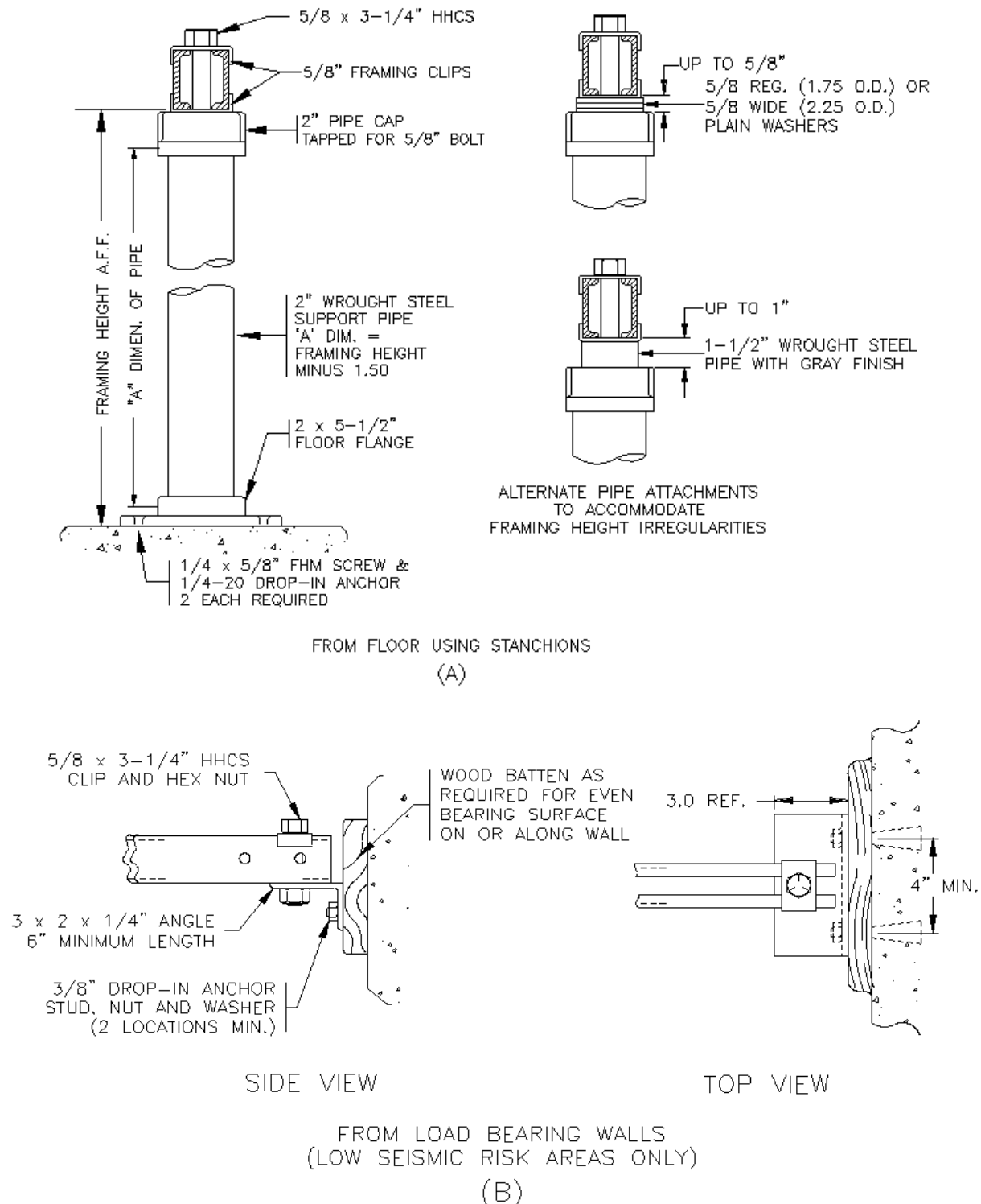
Figure 16. Alternative Auxiliary Framing Support Arrangements
