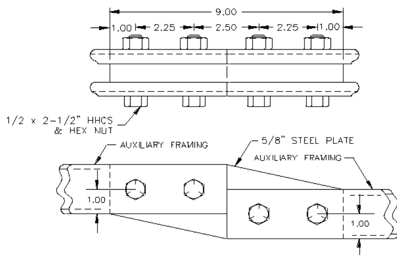
Figure 4. Auxiliary Framing Splice - 1 Inch Difference In Framing Levels
