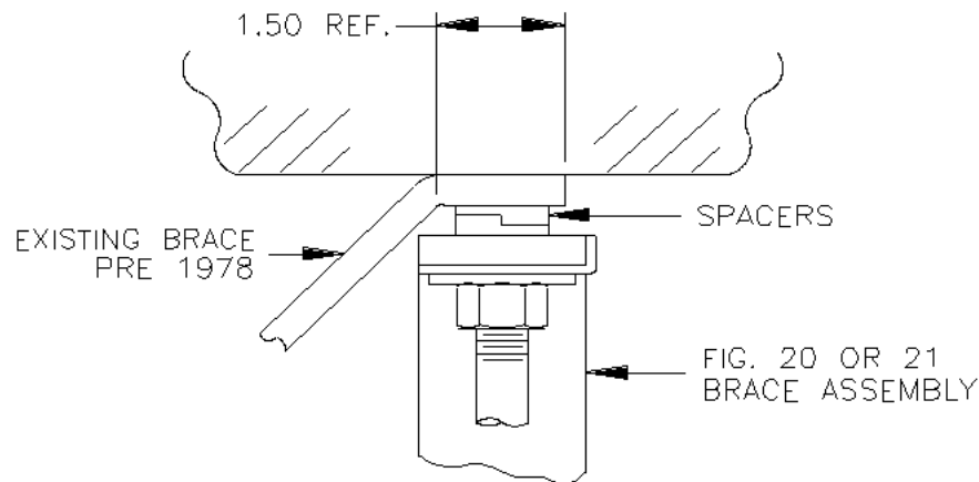
Figure 23. Auxiliary Framing Brace At Load Bearing Building Surfaces - High Seismic Risk Areas
