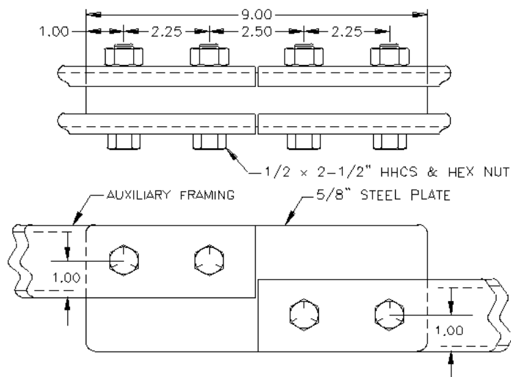
Figure 5. Auxiliary Framing Splice - 1-1/2 Inch Difference In Framing Levels
