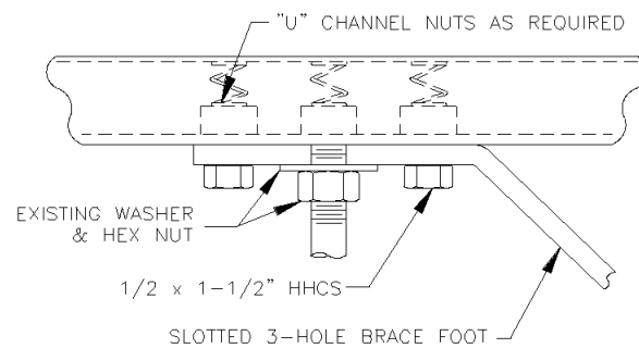
FROM PARALLEL CEILING "U" CHANNEL AT SUPPORT ROD (21B)
