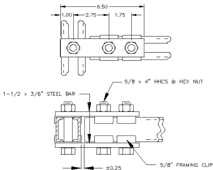
Figure 8. Auxiliary Framing Junction - Single Level Framing
