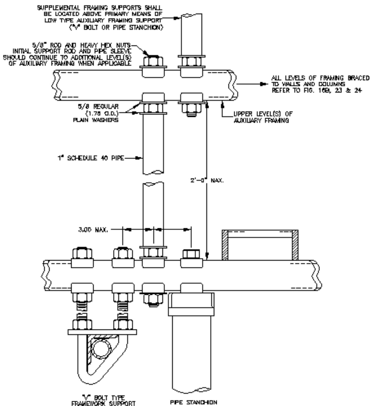
Figure 31. Supporting Upper Level Framing From Lower Level Framing
