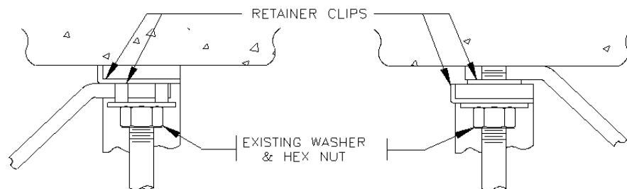
MULTIPLE BRACES AT CEILING INSERT SK-21A
