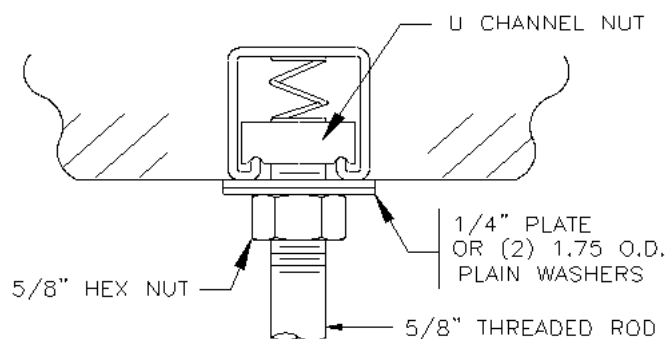
Figure 13. Hanger Rod Attachment At Ceiling Channel - Embedded Shown
