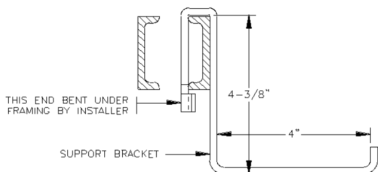
Figure 28. Miscellaneous Cable Supports For Auxiliary Framing
