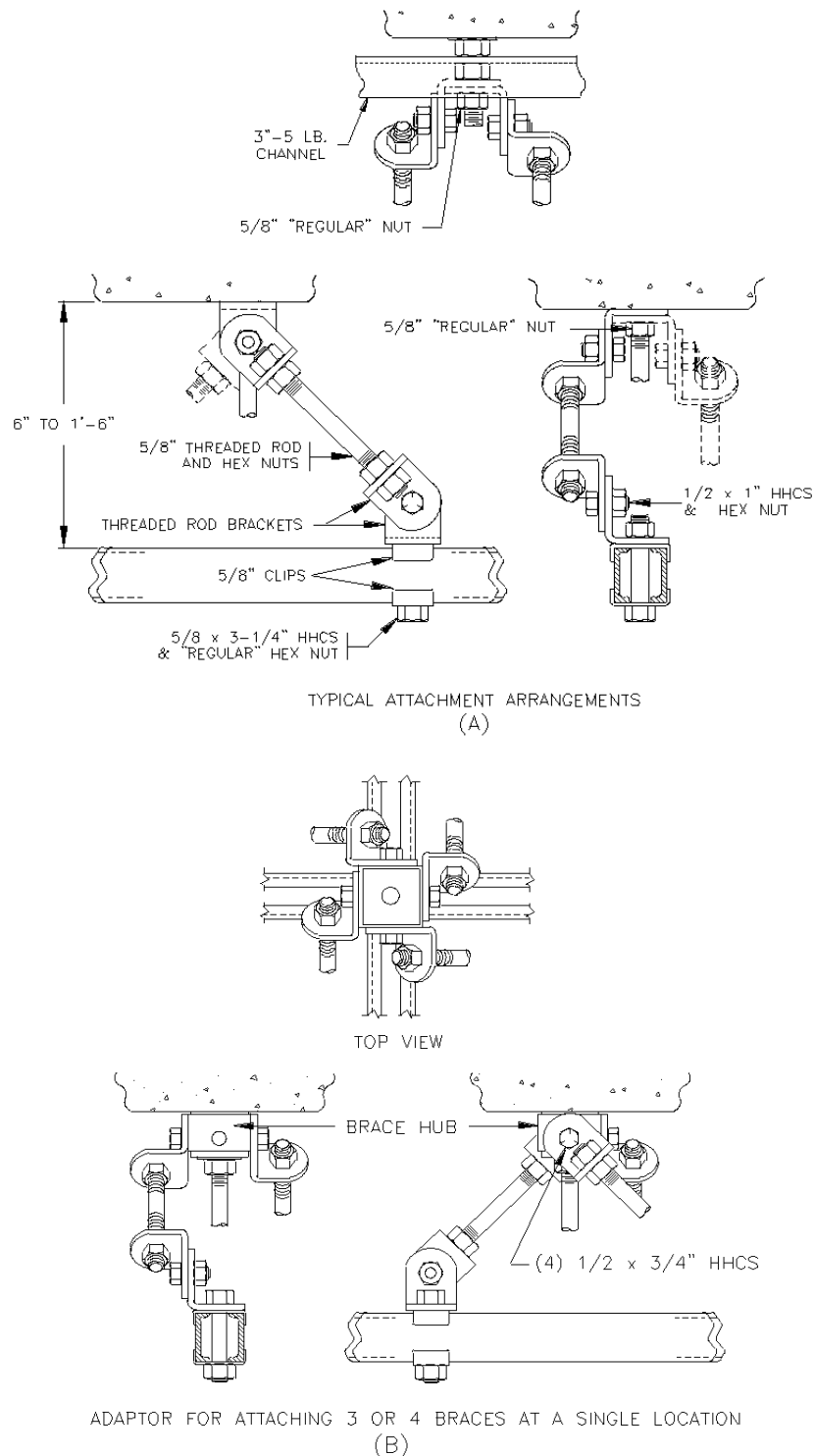
Figure 17. Threaded Rod Brace From Support Rod/Ceiling Insert
