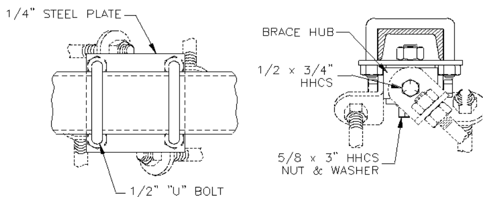
ATTACHING 3 OR 4 BRACES (B)
