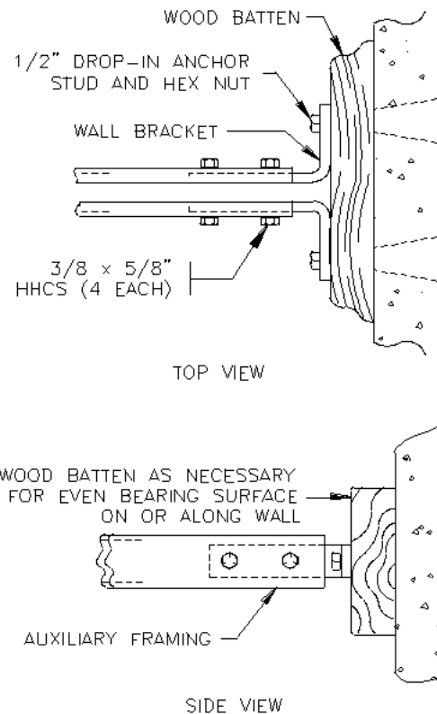
Figure 23. Auxiliary Framing Brace At Load Bearing Building Surfaces - High Seismic Risk Areas
