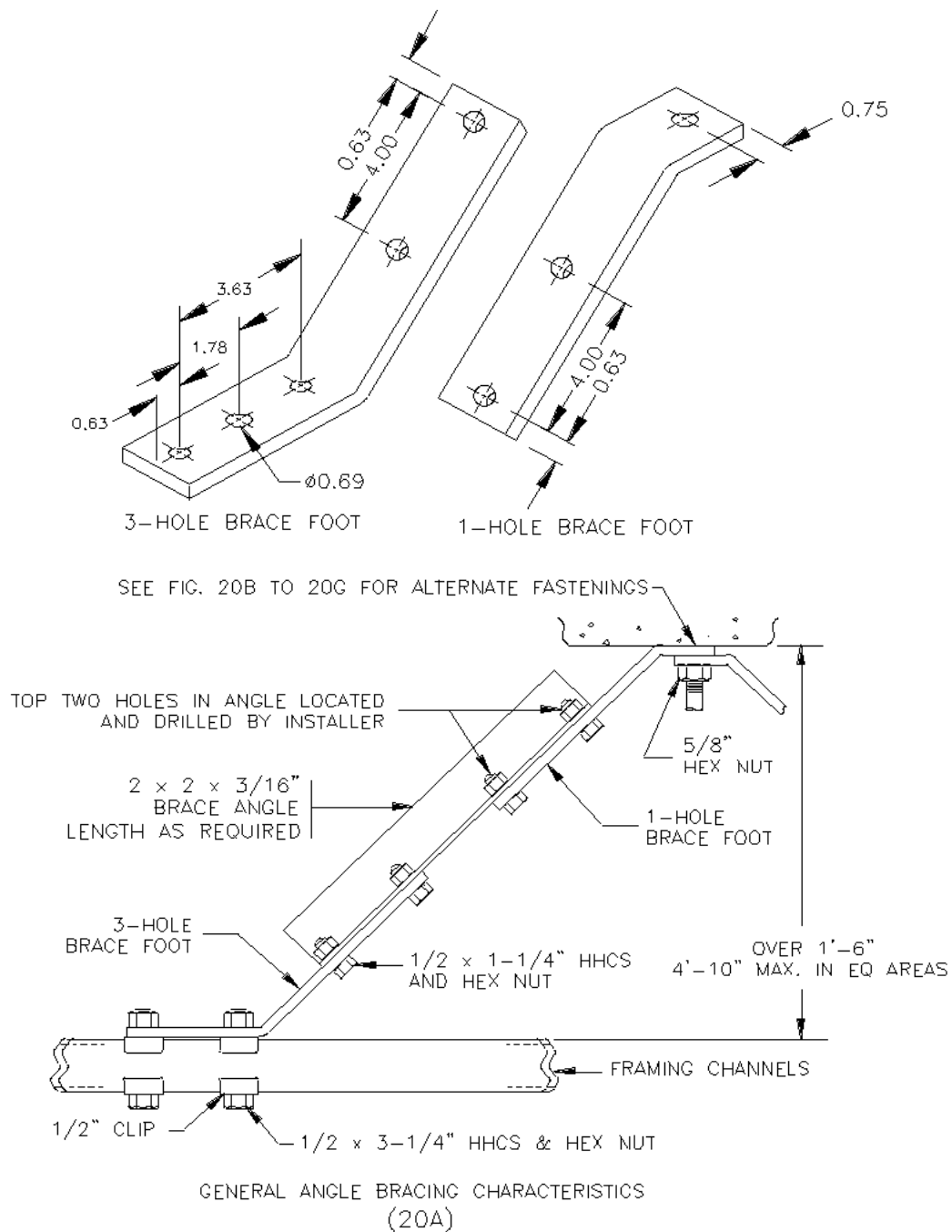
Figure 20. Angle Brace And Bracing Arrangements
