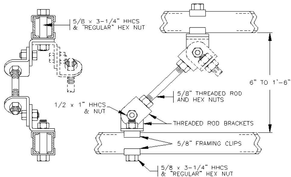
Figure 18. Threaded Rod Brace From Auxiliary Framing
