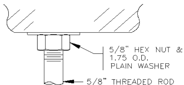
Figure 12. Hanger Rod Attachment At Ceiling Insert With 3'-5lb. Channel
