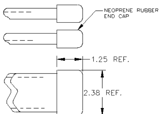
Figure 10. Auxiliary Framing Finishing Caps
