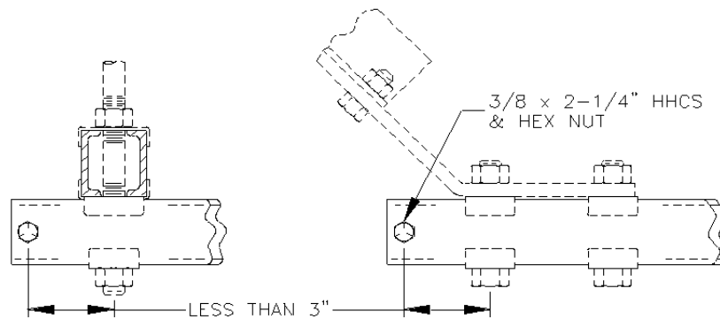
Figure 25. Arrangement Of Auxiliary Framing Stiffening Clips And Through Bolts
