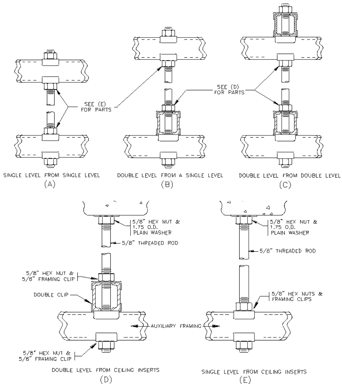
Figure 15. Typical Auxiliary Framing Support Arrangements
