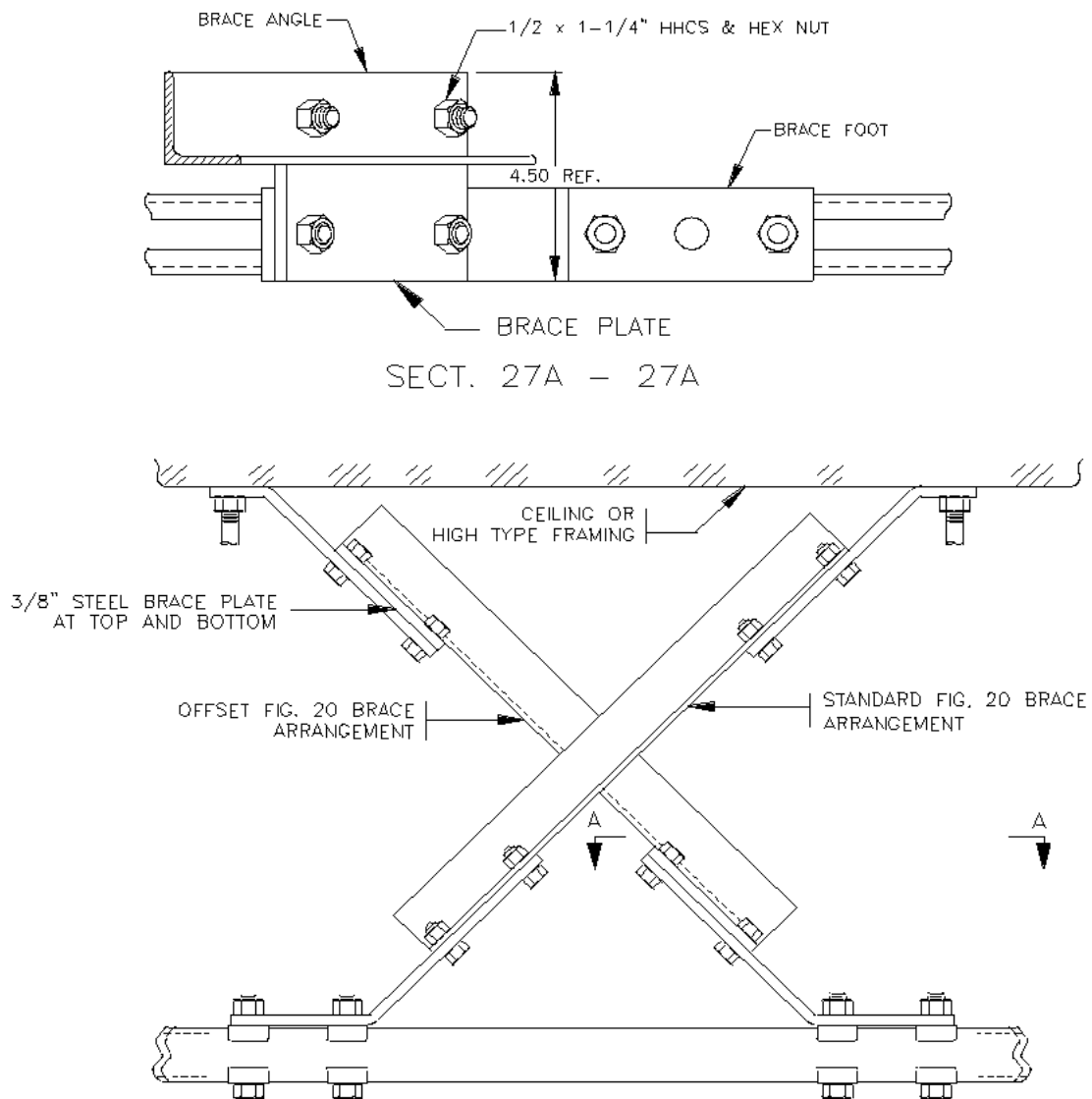
Figure 27. Method Of Installing Auxiliary Framing Braces At Same Location
