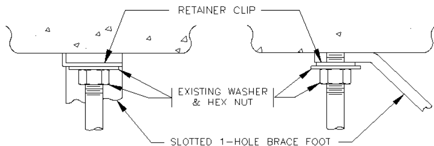
SINGLE BRACE ARRANGEMENT AT CEILING INSERT (21A)
