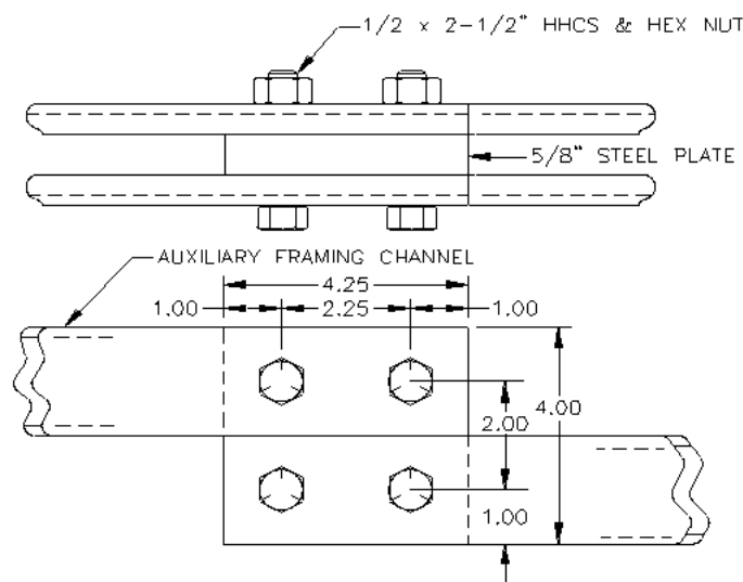
Figure 6. Auxiliary Framing Splice - 2 Inch Difference In Framing Levels
