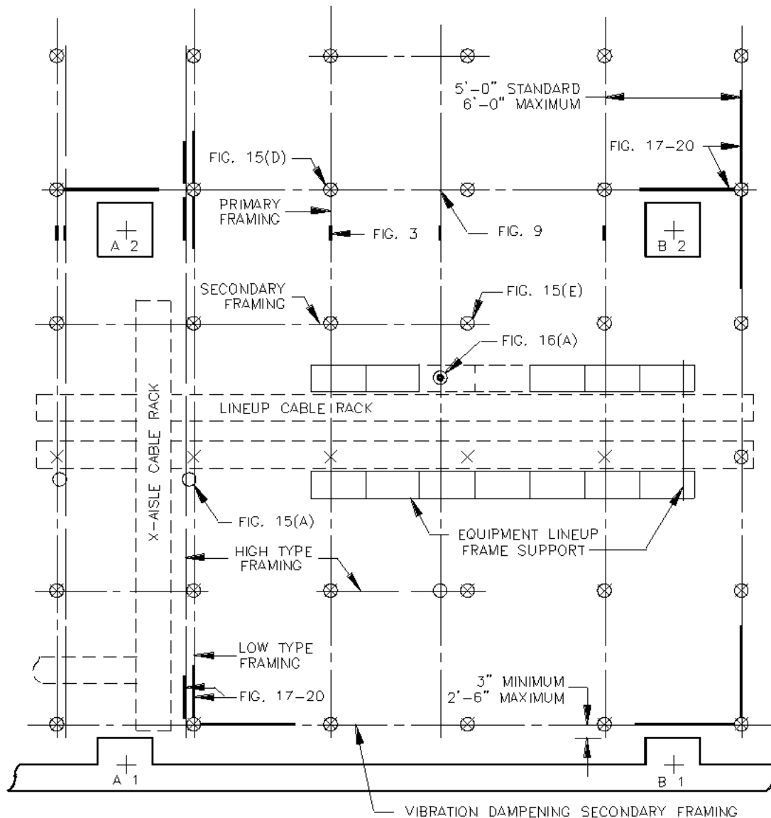
Figure 1. Typical Auxiliary Framing Arrangement - Low Seismic Risk Areas
