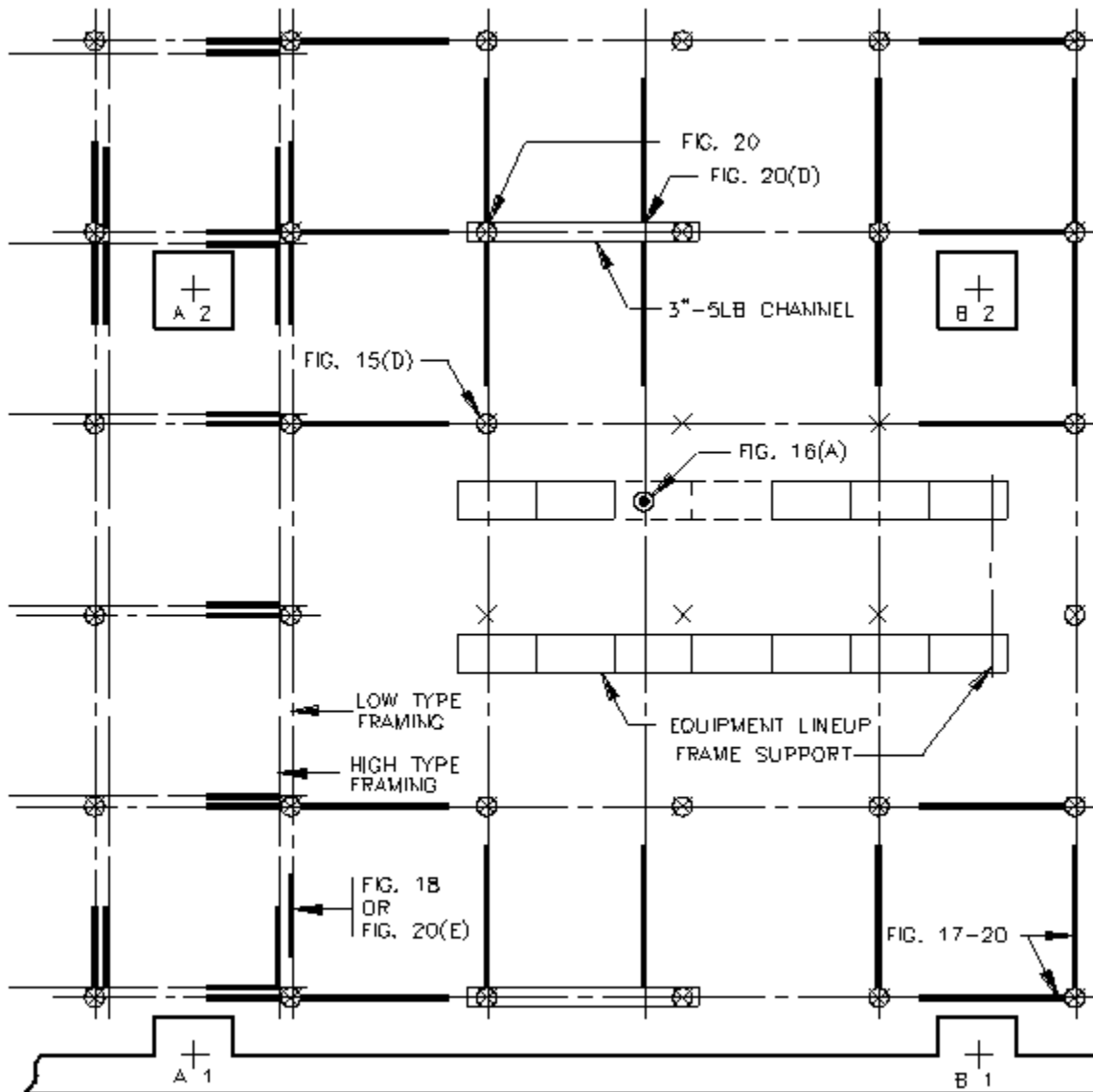
Figure 2. Typical Auxiliary Framing Arrangement - High Seismic Risk Areas
