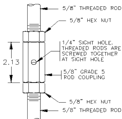
Figure 14. Hanger Rod Splice
