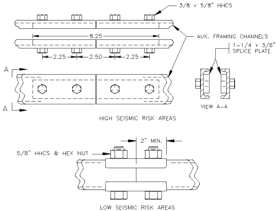
Figure 3. Auxiliary Framing Splices - Same Level
