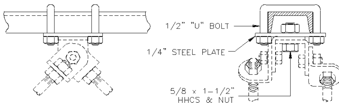
ATTACHING 1 OR 2 BRACES (A)
