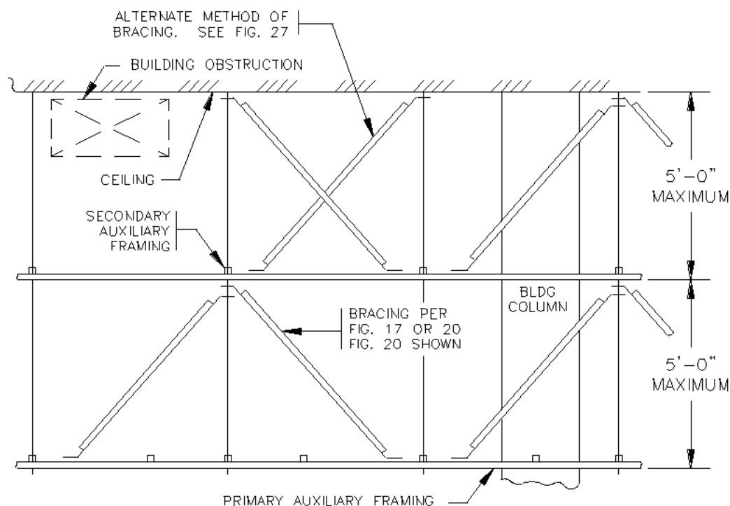
Figure 26. Typical Warren Truss Type Bracing Arrangement For Floor Supported Equipment Systems That Require Direct Attachment To Office Superstructure Via Framework Braces
