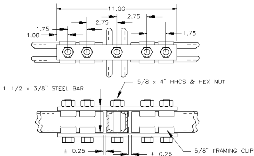
Figure 7. Auxiliary Framing Intersection - Single Level Framing
