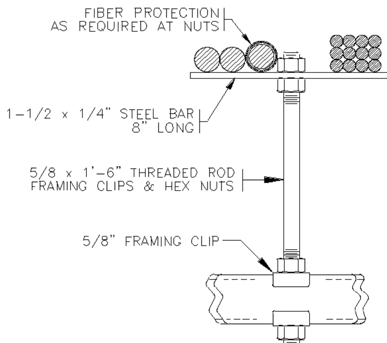
Figure 29. Auxiliary Cable Support From Auxiliary Framing
