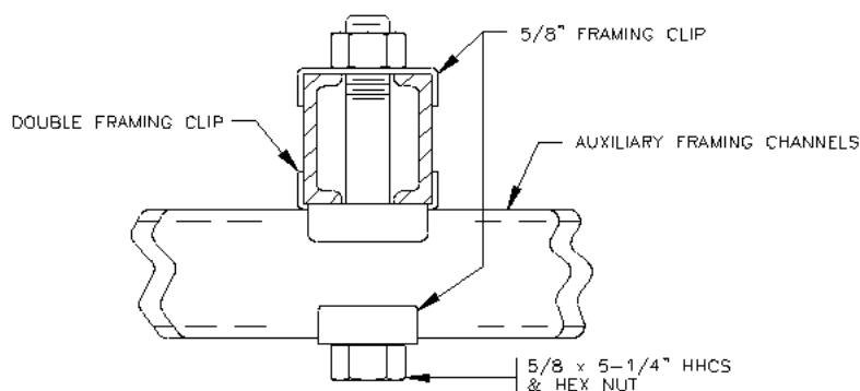
Figure 9. Auxiliary Framing Intersection - Double Level Framing
