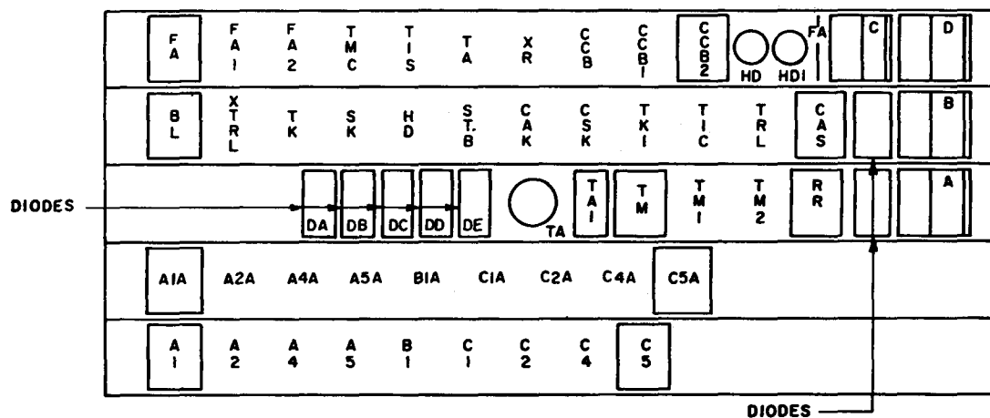
Fig. 6 - Code Compressor Unit - J95111K
