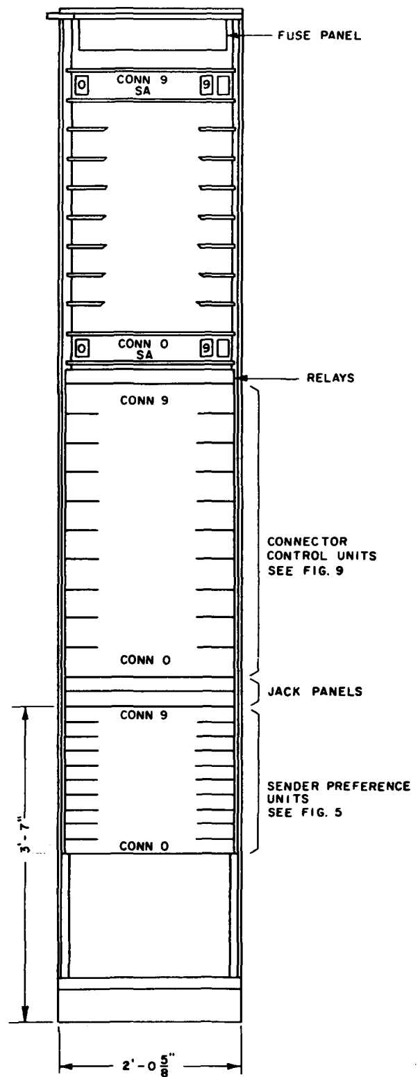
Fig. 2 - Code Compressor Connector Frame - J95111C
