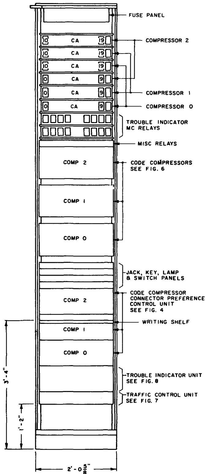
Fig. 1 - Code Compressor Frame - J95111A
