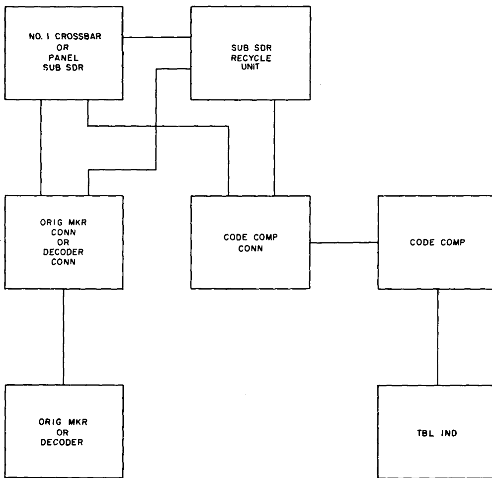
Fig. 11 - Six-digit Translation Arrangement
