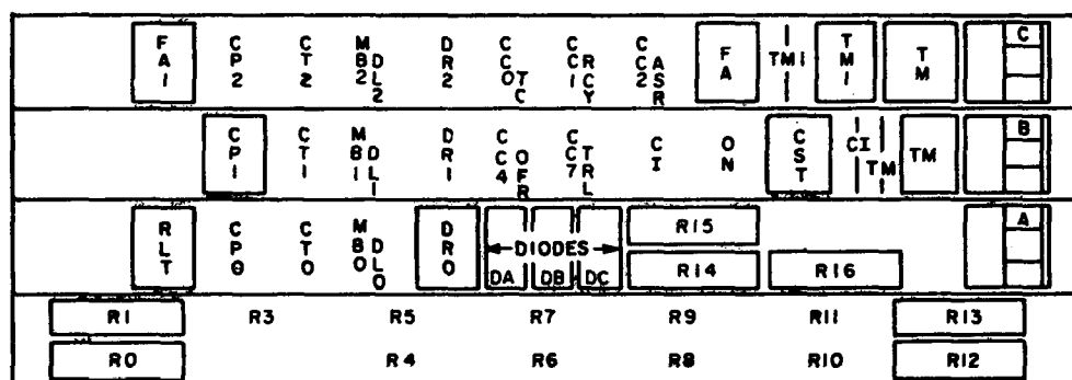
Fig. 8 - Trouble Indicator Unit - J95111M
