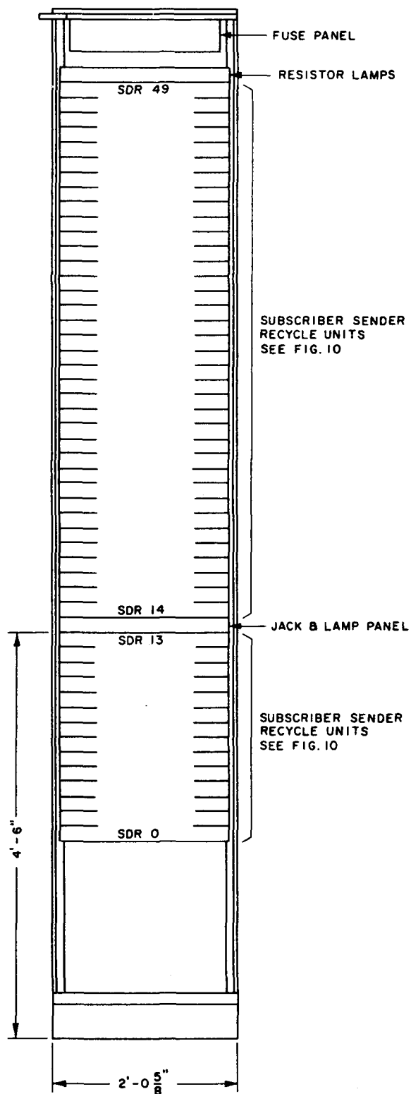
Fig. 3 - Subscriber Sender Recycle Frame - J95111E
