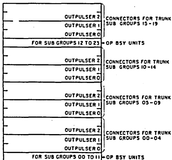
Fig 2—Typical Arrangement of Outputpulser Connectors on Relay Rack for 3 Outputpulsers (4 Ultimately) and 20 Trunk Subgroups
