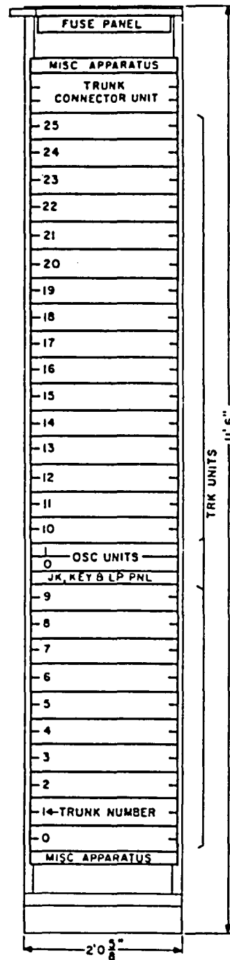
Fig 1—Typical ANIT Frame
