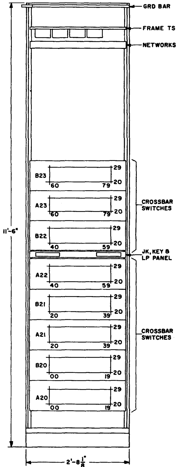
Fig. 3 - Second Supplementary Concentrating Frame
