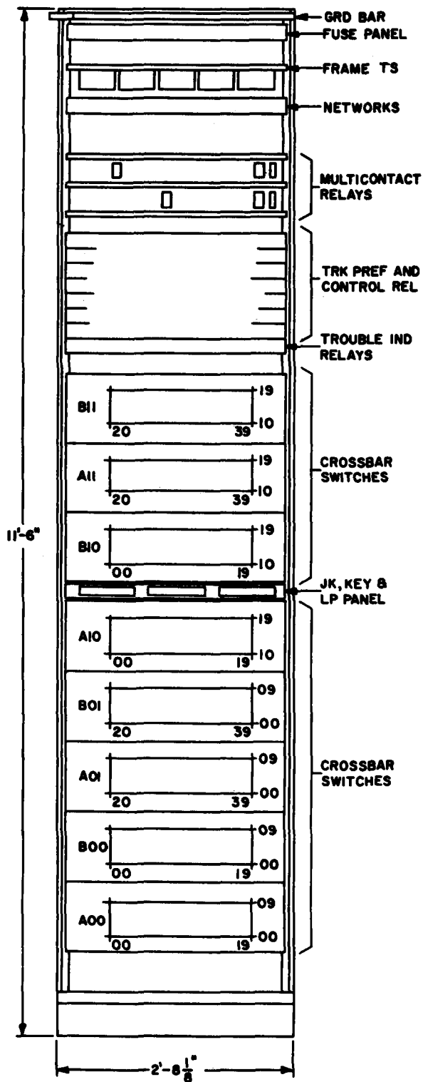
Fig. 1 - Concentrating Frame (Basic)
