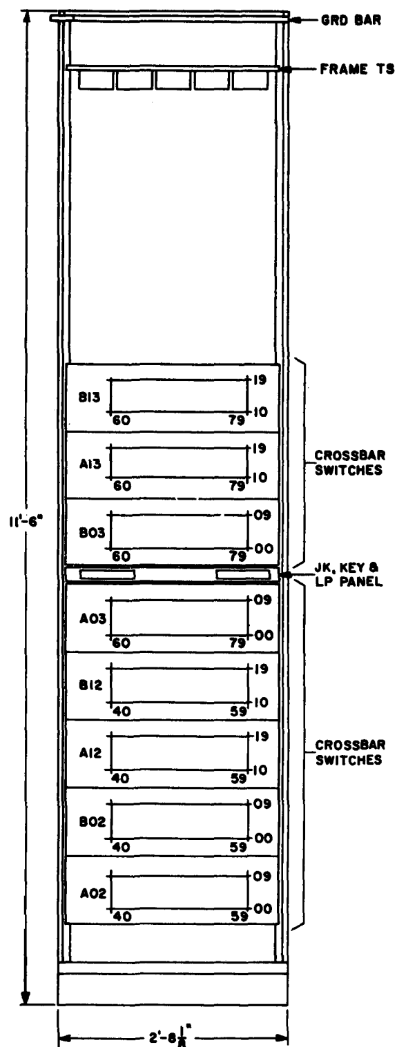
Fig. 2 - First Supplementary Concentrating Frame
