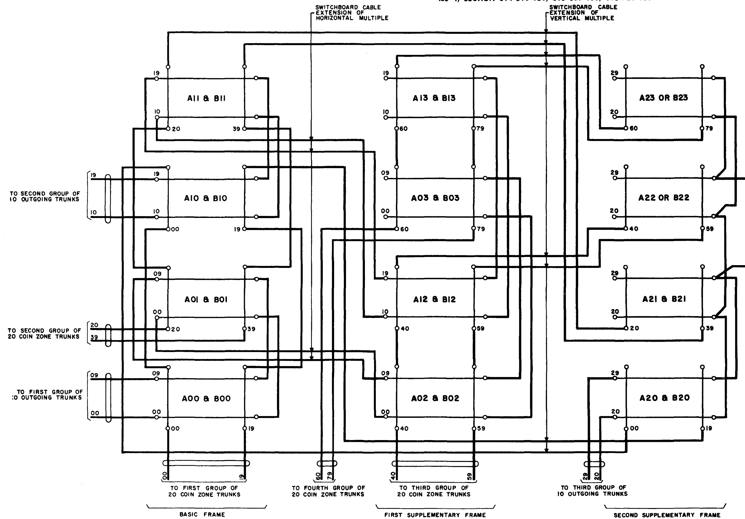
Fig. 4 - Arrangement of Interconnecting Switch Multiples
