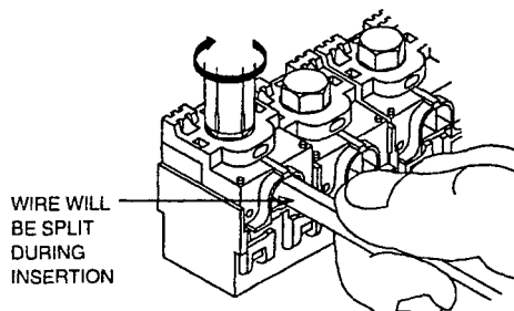
K-Series IDC Block With 18.5 Gauge (0.9 mm) Wire Inserted
