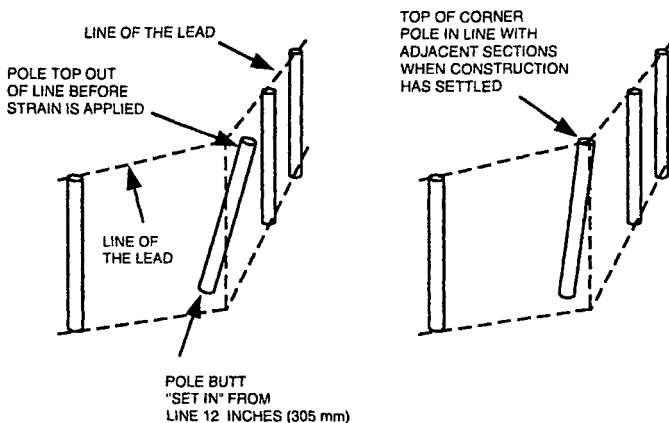
Unguyed Corner Pole Raked
