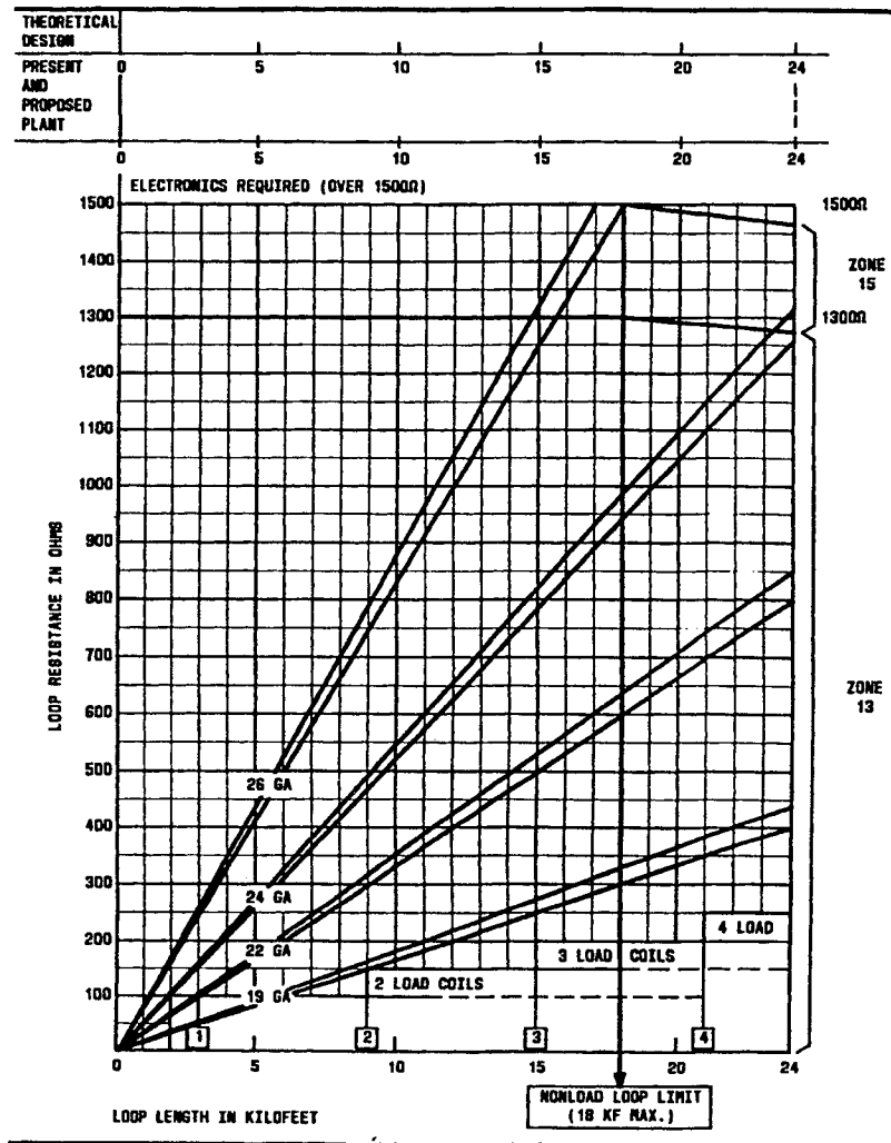
Resistance Design Chart 0 - 24,000 ft (7,315 m)
