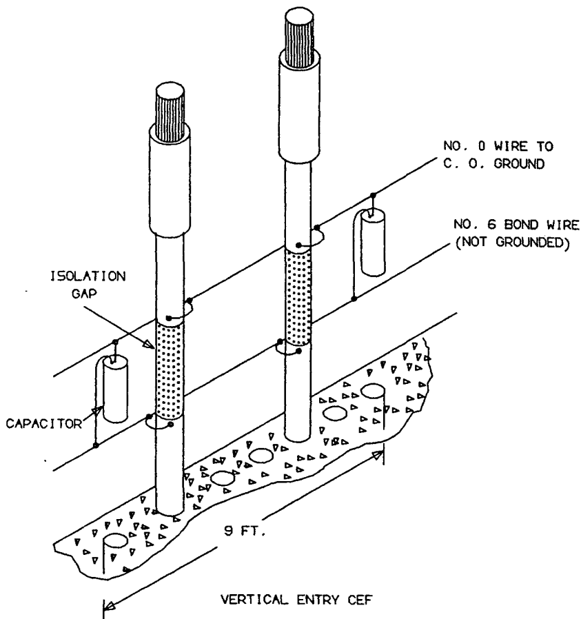
Bonding and Grounding Arrangements
