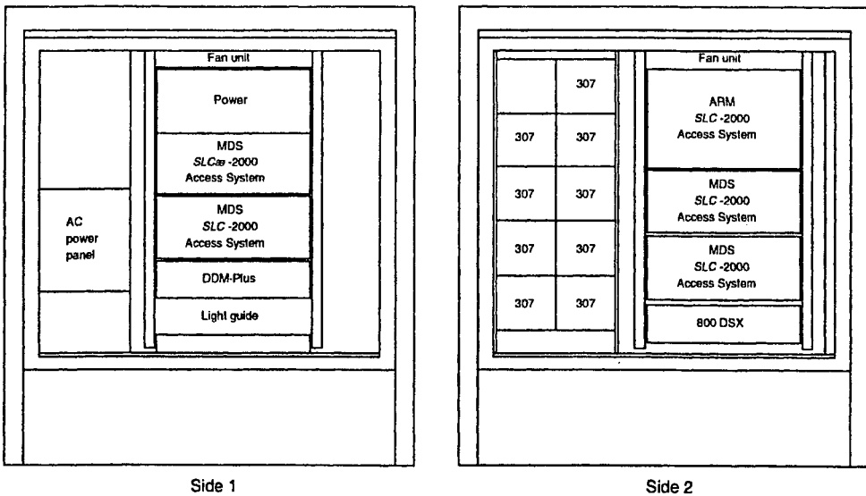
80A-HX Cabinet Configuration
