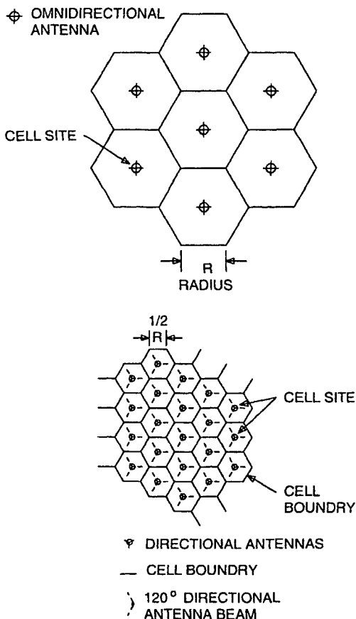
Cell Split (Startup-to-Growth Configurations)
