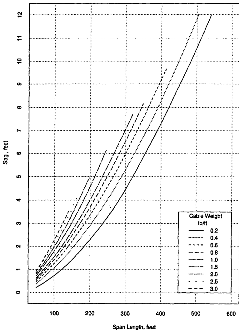
6M Strand - Medium Loading Region (Based on NESC Rule 232)
