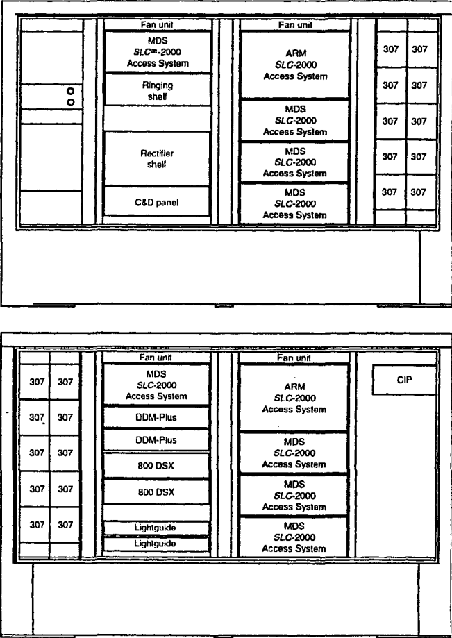
80D-HX Cabinet Configuration
