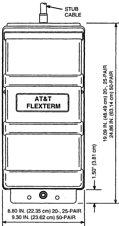
20-, 25-, and 50-Pair Pole or Wall Mounted Cable Terminal
