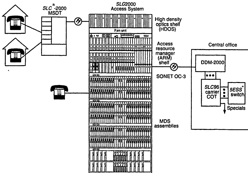
SLC R -2000 Access System Universal Configuration
