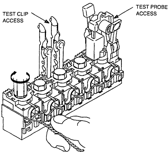
K-Series IDC Block With 22-Gauge (0.6 mm) or 24 Gauge (0.5 mm) Wire Inserted
