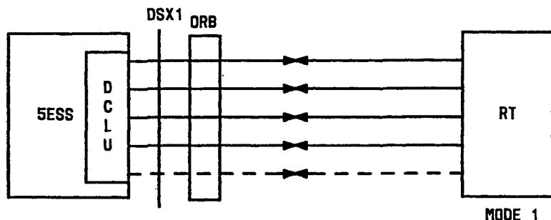
Integrated SLC 96 Carrier System
