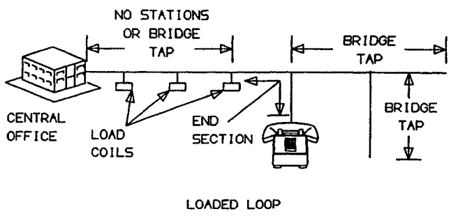
Illustration of Bridge Tap and End Section
