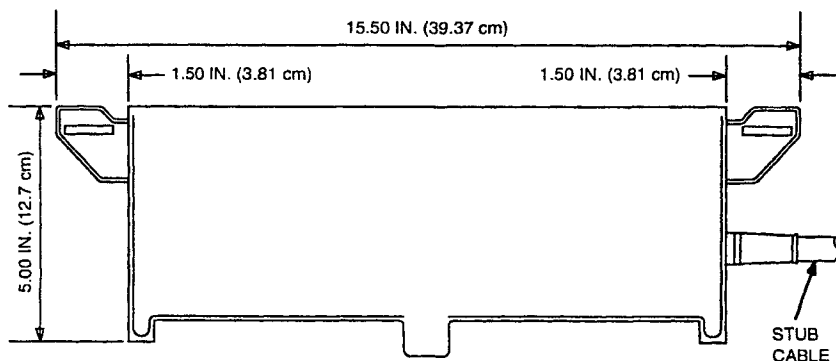
10-Pair Strand Mounted Cable Terminal (Can be Pole or Wall Mounted Using Optional Bracket)
