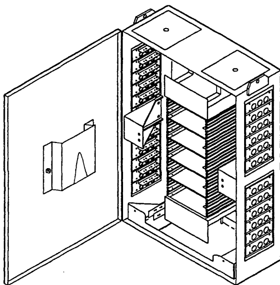
Optical Cable Entrance Facility (OCEF1-720/42)
