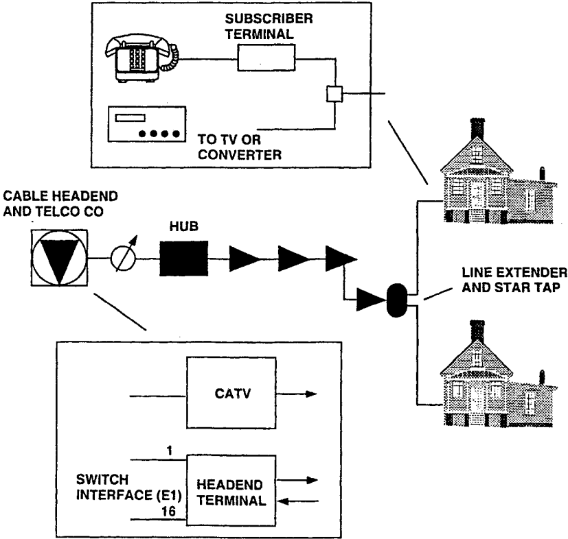
Cable Loop Carrier - 500 (CLC-500)
