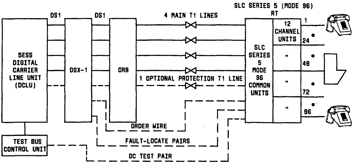
An Integrated FP-B (TR-08) RT
