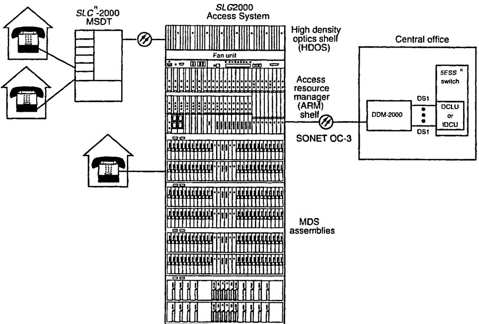
SLC ® -2000 Integrated Configuration (Mixed Metallic and Fiber Distribution)
