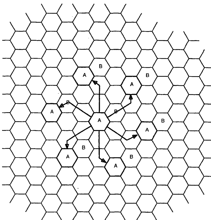
Determination of Cochannel Cells with 7-Cell Reuse Pattern
