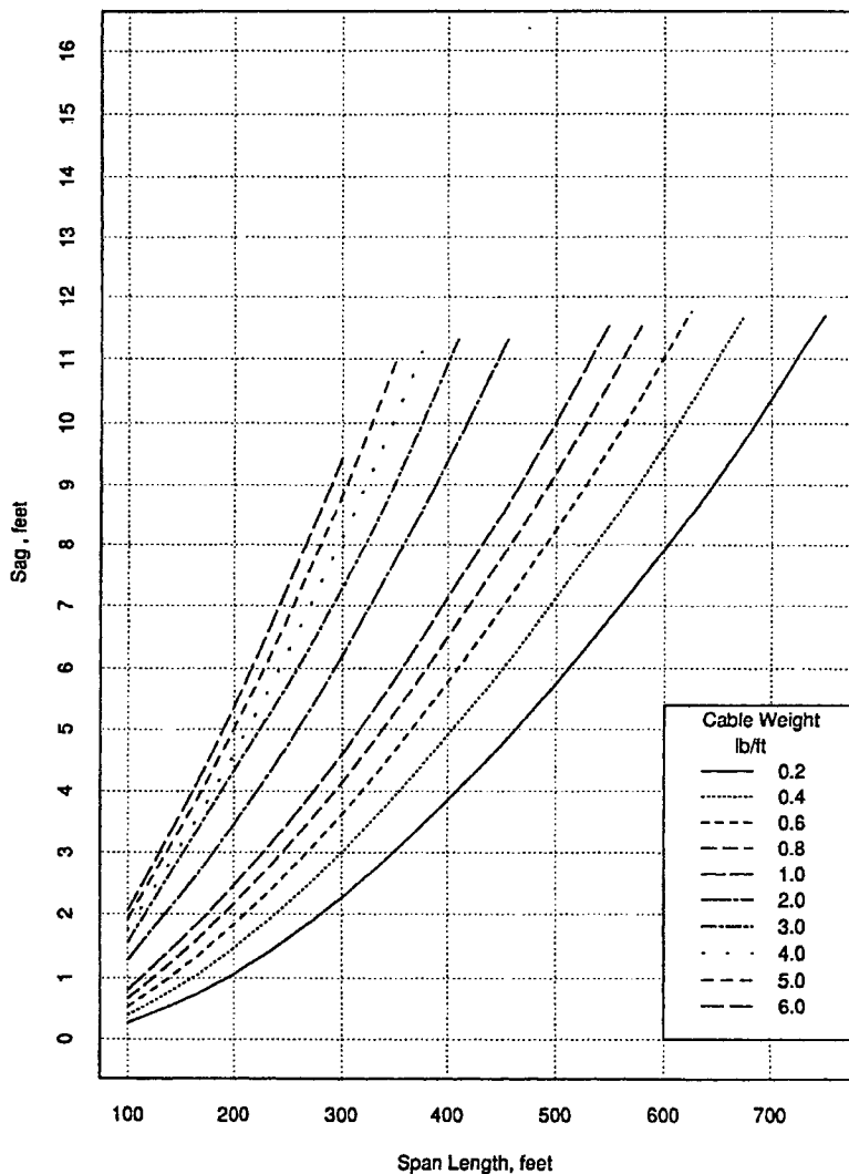
16M Strand - Light Loading Region (Based on NESC Rule 232)
