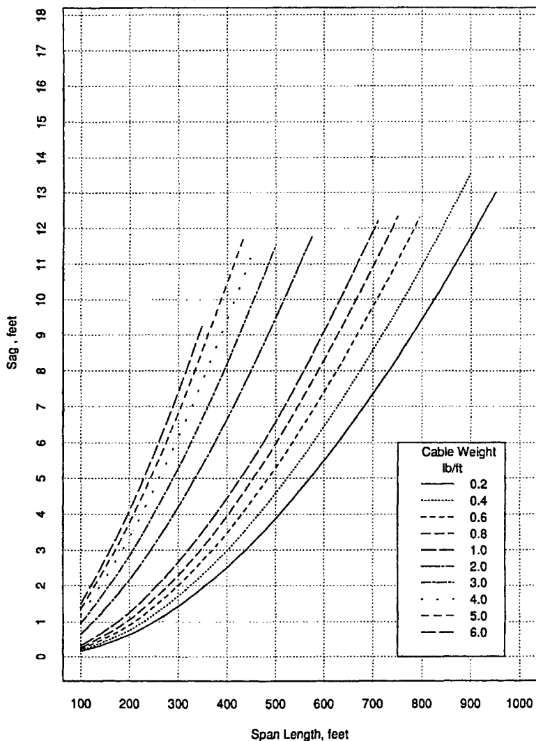
25M Strand - Medium Loading Region (Based on NESC Rule 232)
