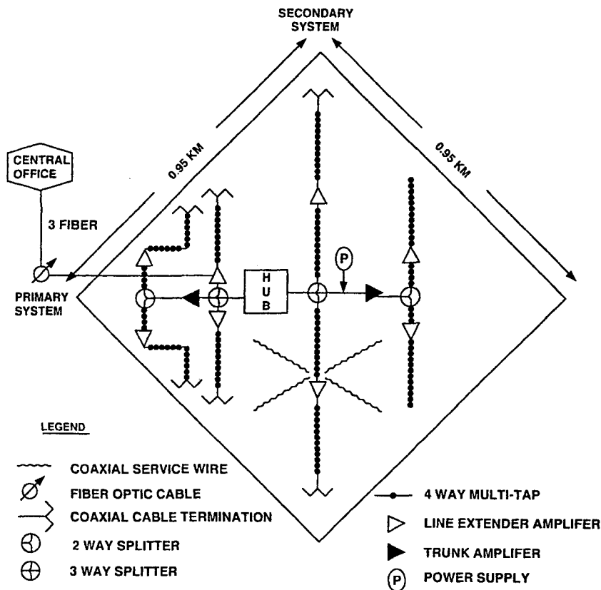
Hybrid Fiber Optic/Coax Network
