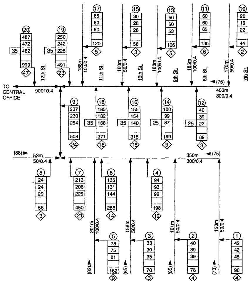
Secondary System Chart
