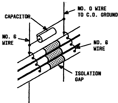
MULTI-CABLE BONDING AND GROUNDING
