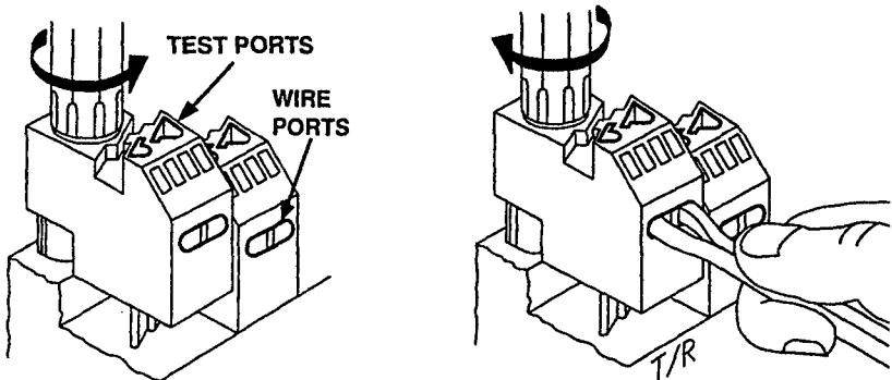
Drop Wire Insertion for J-Series IDC Block
