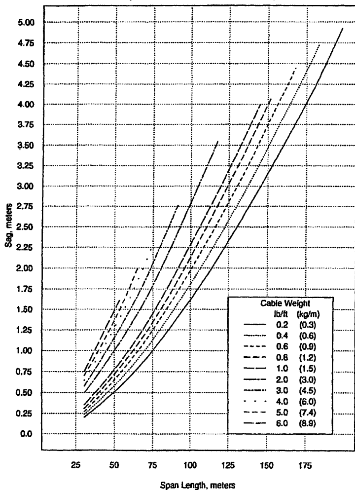
10M Strand - Heavy Loading Region (Based on NESC Rule 232)
