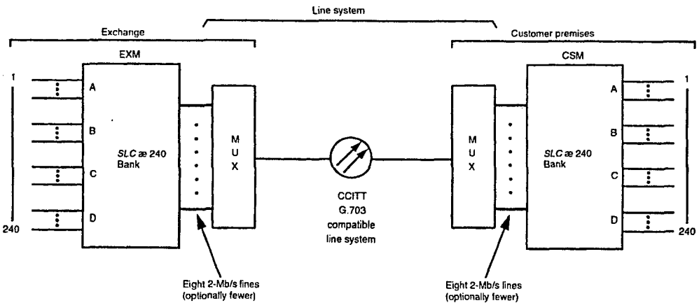
SLC R 240 System Configuration
