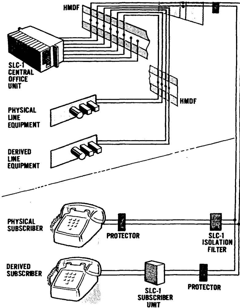
SLC 1 Carrier System
