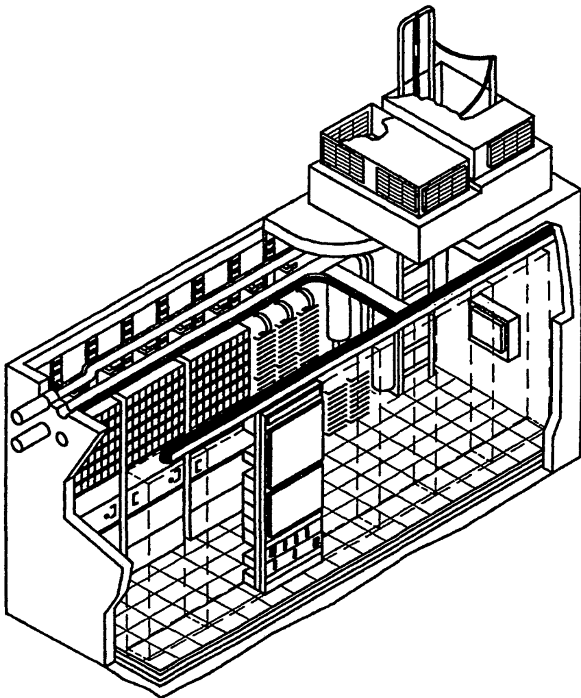
Controlled Environment Vault (CEV) Equipped With Subscriber Carrier Equipment
