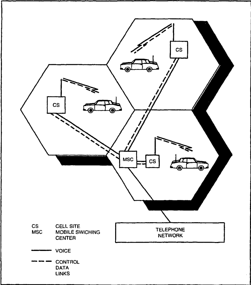
AUTOPLEX® System 1000 — Cellular Telecommunications System
