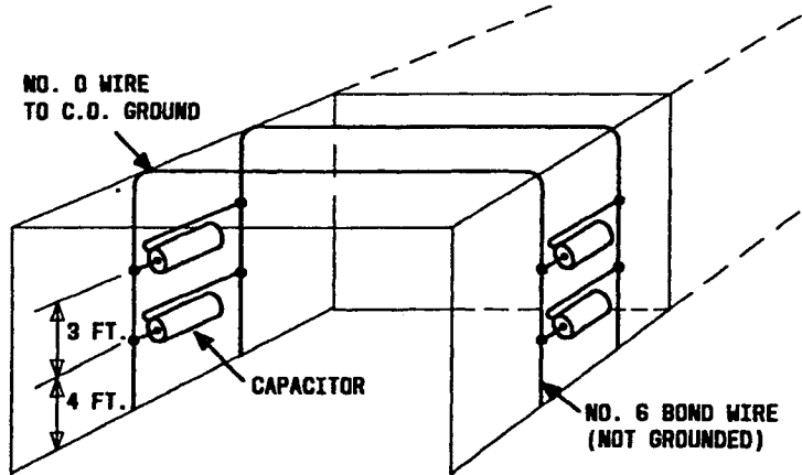
CAPACITOR INSTALLATION (CABLES NOT SHOWN)
