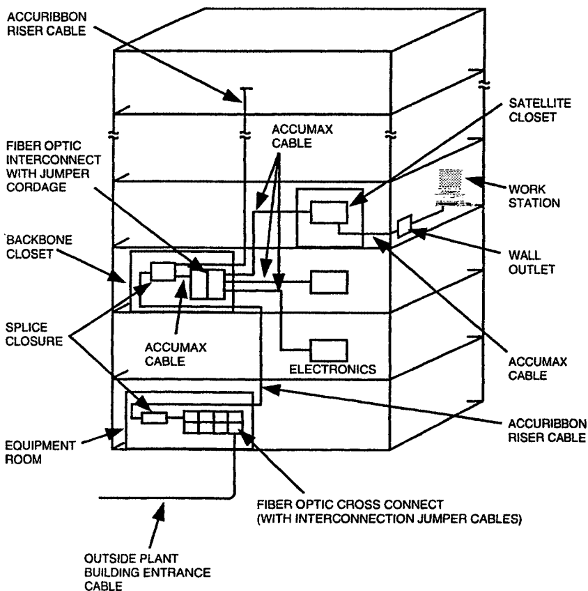
SYSTIMAX Structured Cable System
