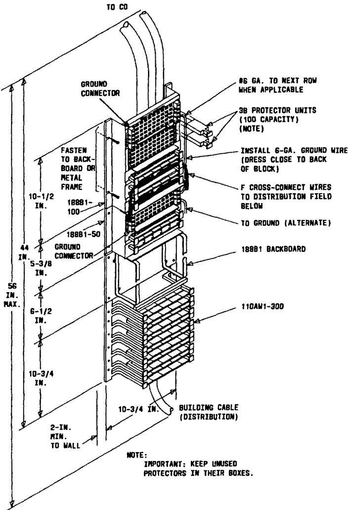
Illustration of 188-Type Protector Use
