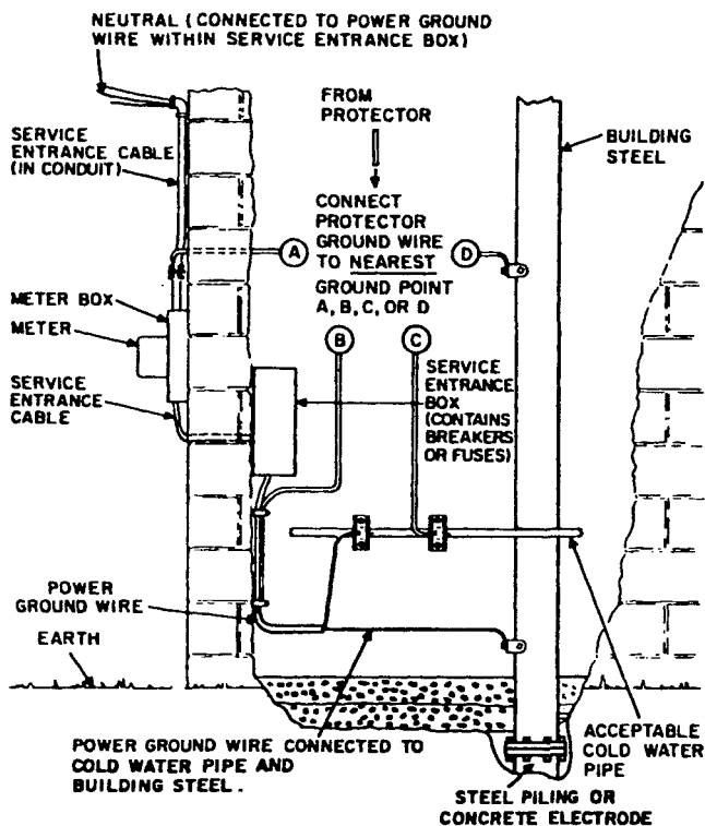
Acceptable Protector Grounding Connections to the Power Ground
