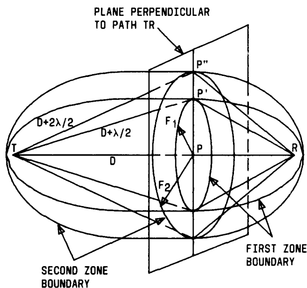
Fig. 3—Representation of Fresnel Zones in Three Dimensions
