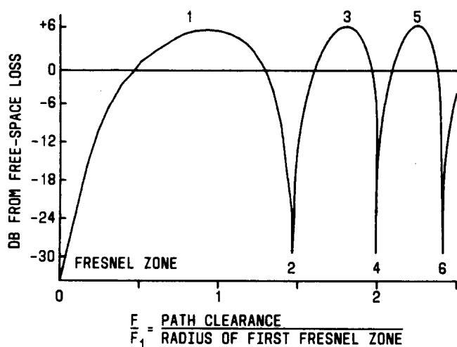
Fig. 5—Effect of Increasing Clearance on a Radio Path With Reflections
