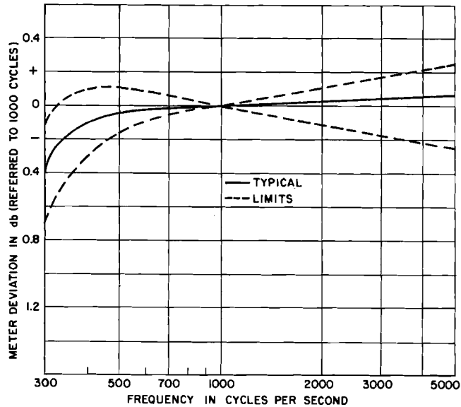
Fig. 4 – Frequency Characteristic of the 23A Transmission Measuring Set
