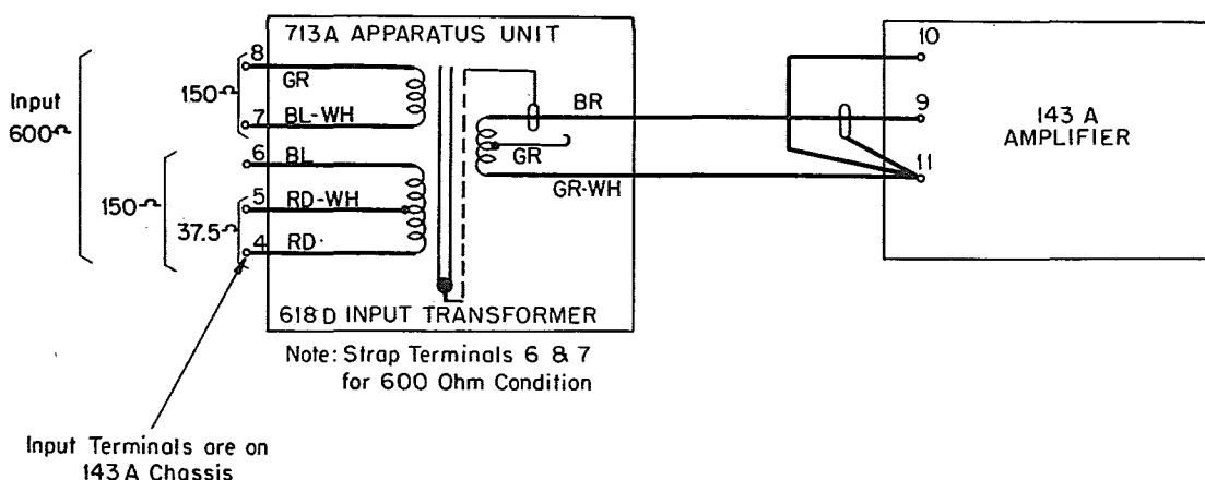
Fig. 5 - 143C Amplifier - Block Diagram
