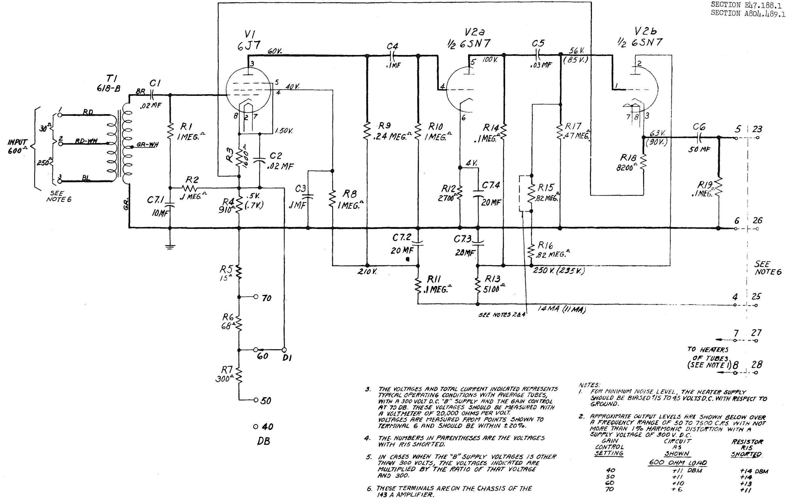
Fig. 4 - 143B Amplifier - Input Circuit Arrangement (141A Amplifier Schematic)
