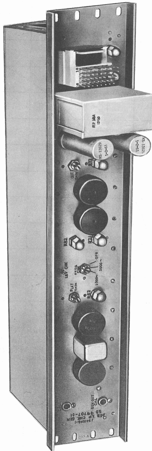
Fig. 2 - 24B Loop Checker Generator
