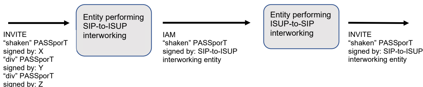
Figure 4-10: “shaken” PASSporT/“div” PASSporT transferred via ISUP UII
