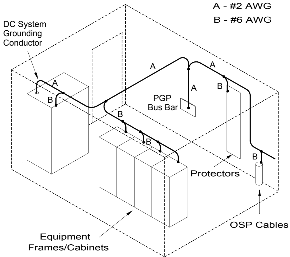
Figure 5-3 Typical Grounding Conductor Arrangement in an EEE (hut shown)
