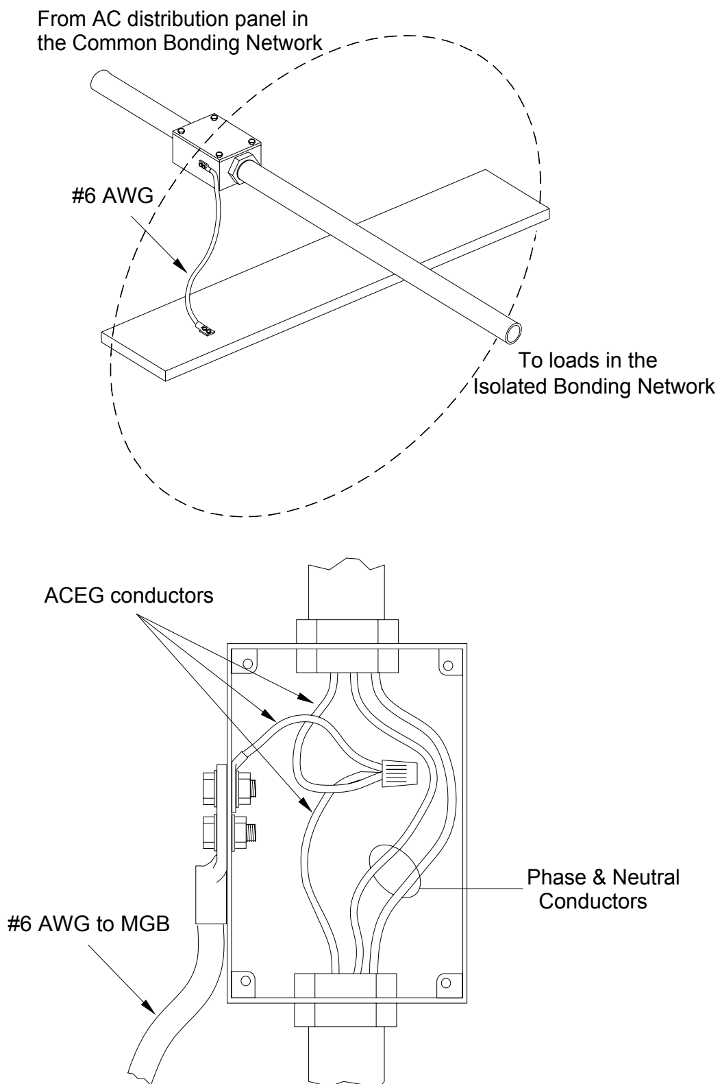
Figure 4-6 Bonding of Conduit and ACEG Conductors to MGB
