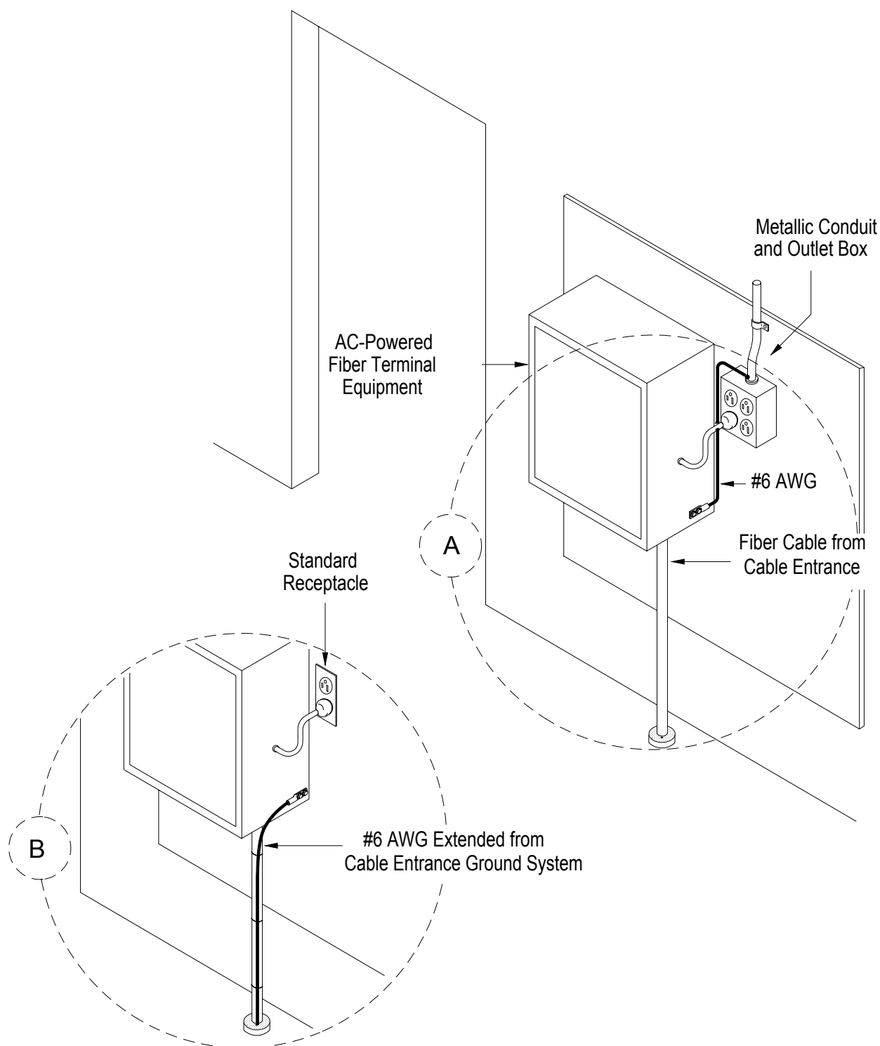
Figure 5-5 Grounding Arrangements for Wall-Mounted Customer Premises Equipment
