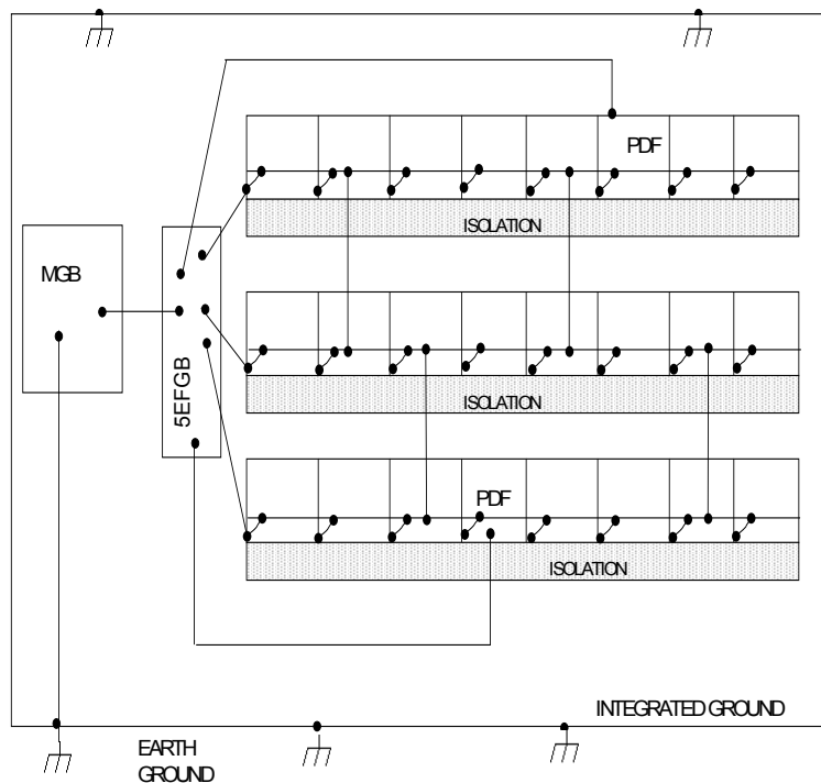
Figure 4-9(b) Lucent 5ESS IBN with 5EFG
