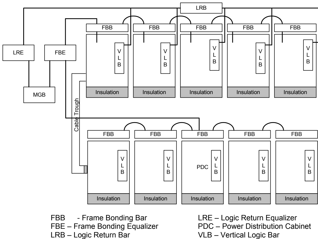
Figure 4-9(c) Nortel DMS-100 IBN
