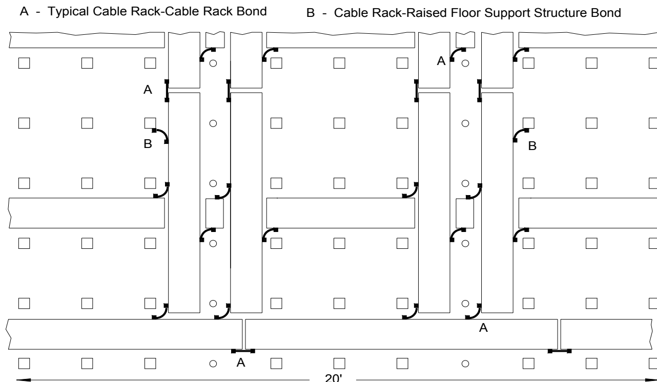
Figure 3-5 Typical Bonding Required When Cable Rack is not Secured to the Raised Floor Support Structure
