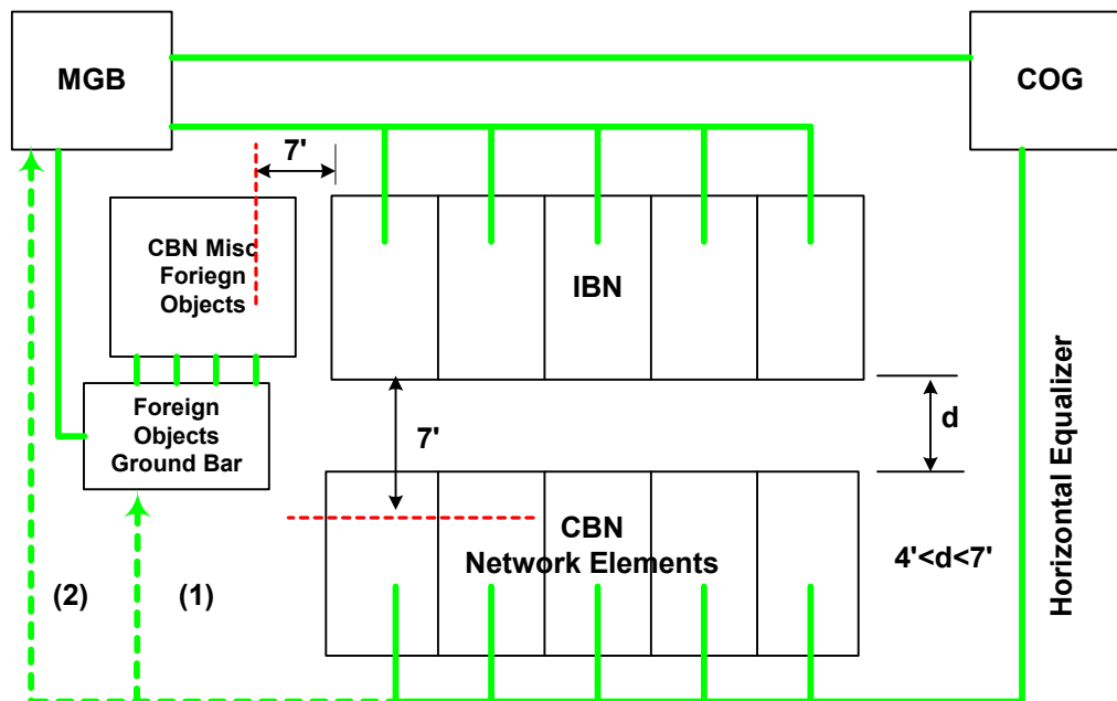
Figure 4-8 Bond of CBN Network Element as Foreign Object
