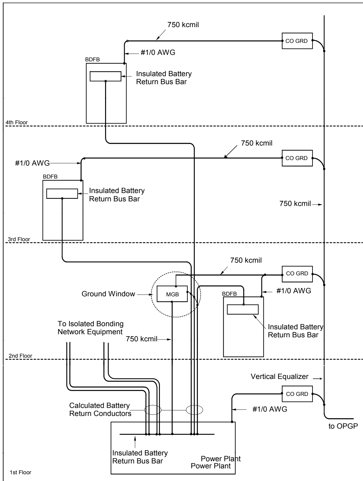
Figure 3-2 Power Plant Serving Both Common & Isolated Bonding Network Equipment
