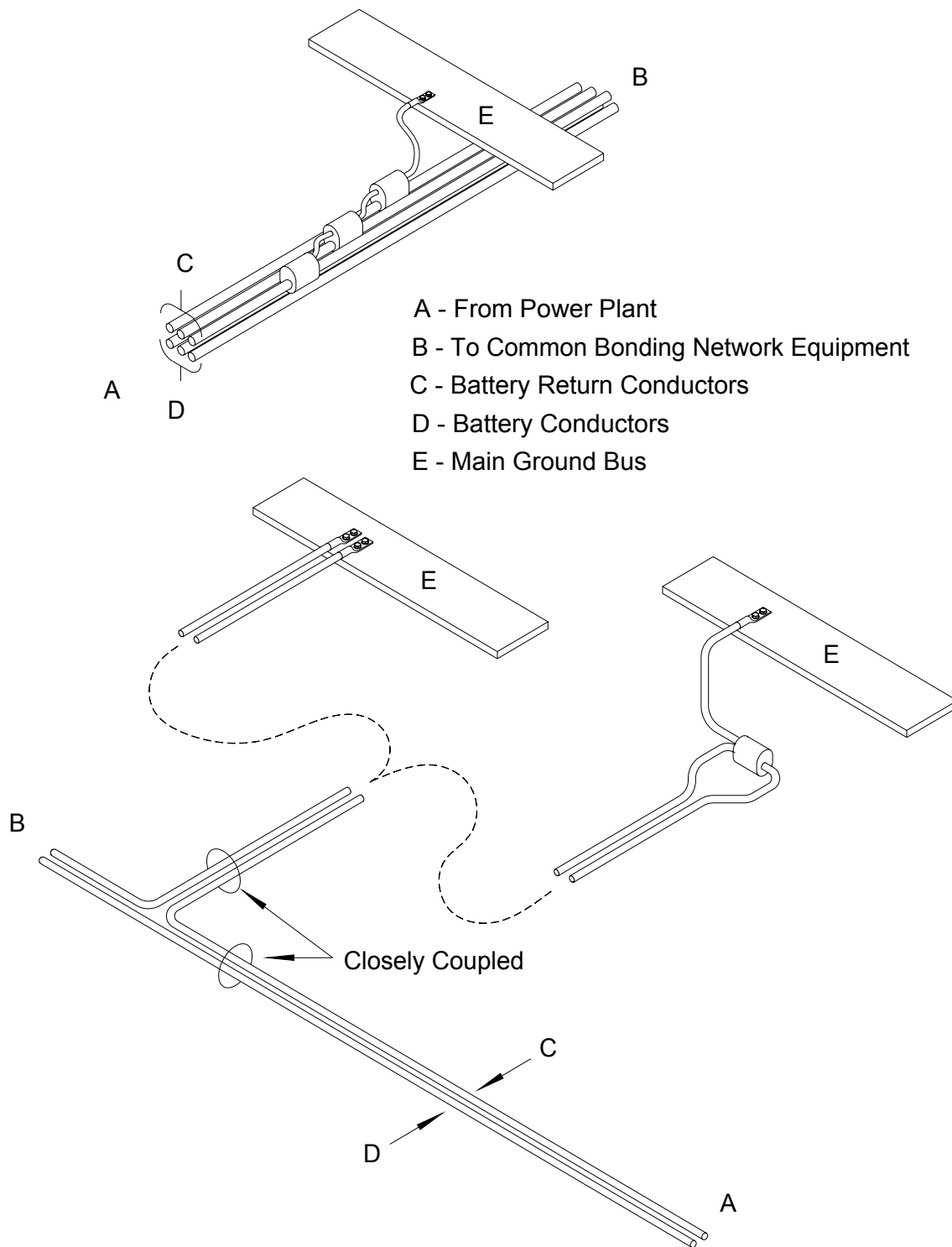
Figure 4-10 Methods of Bonding Battery Return Conductors to the MGB
