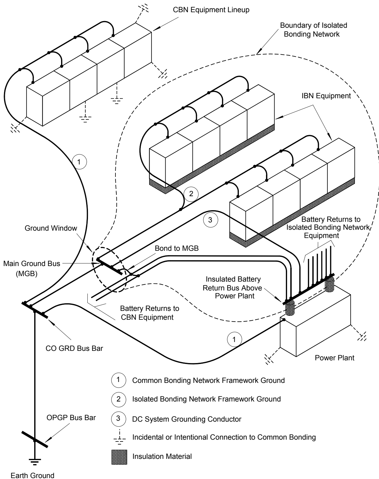
Figure 4-1 Relationship Between Common and Isolated Bonding Networks (MGB is located remote from equipment and power plant)
