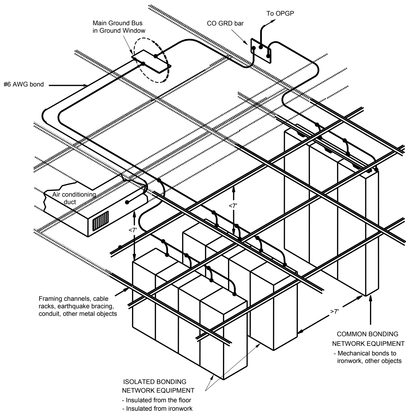
Figure 4-7 Foreign Object Bonds to Nearby Metallic Objects
