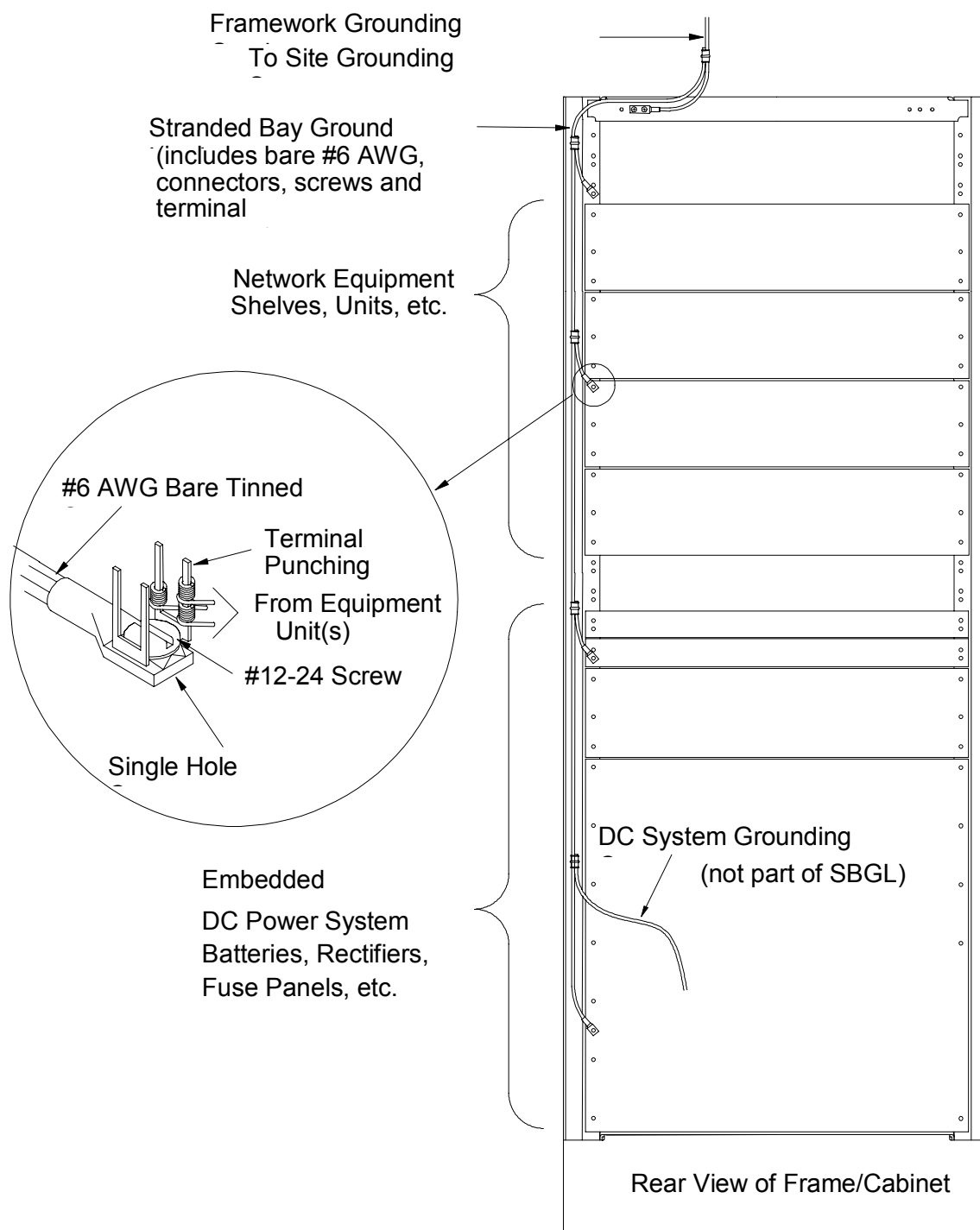
Figure 5-6 Network Equipment Frame/Cabinet Grounding Details
