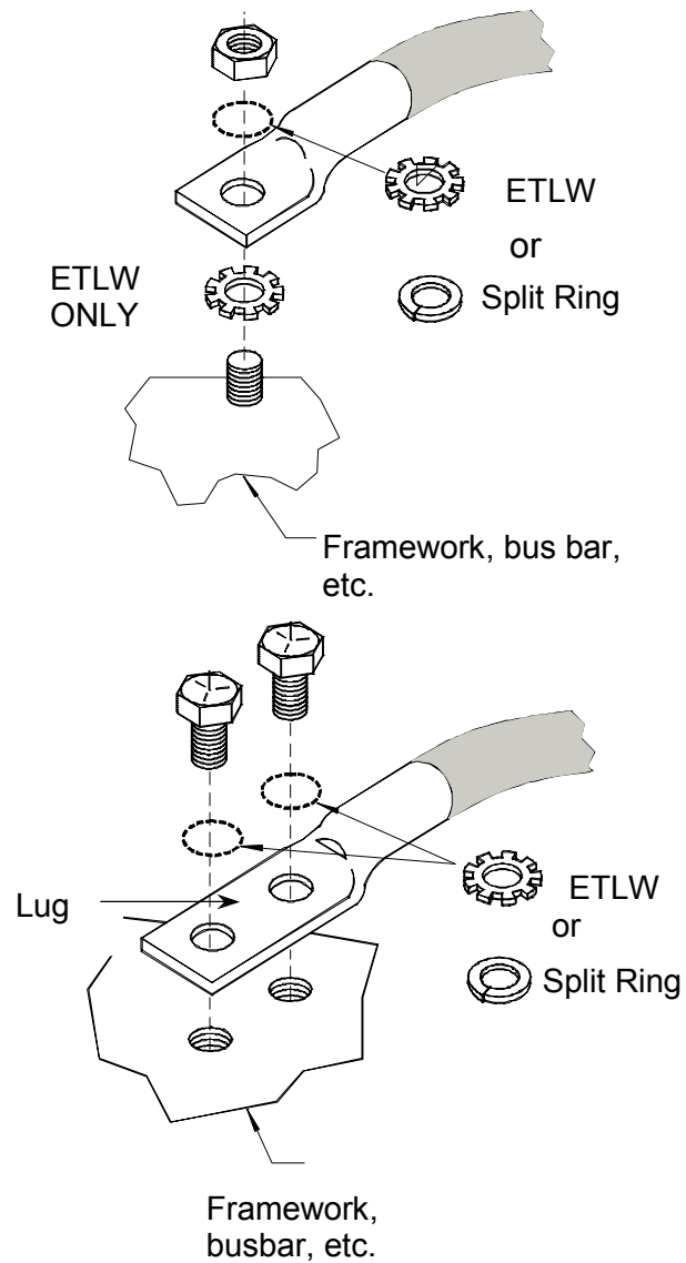
Figure 1-4 Application of Lockwashers
