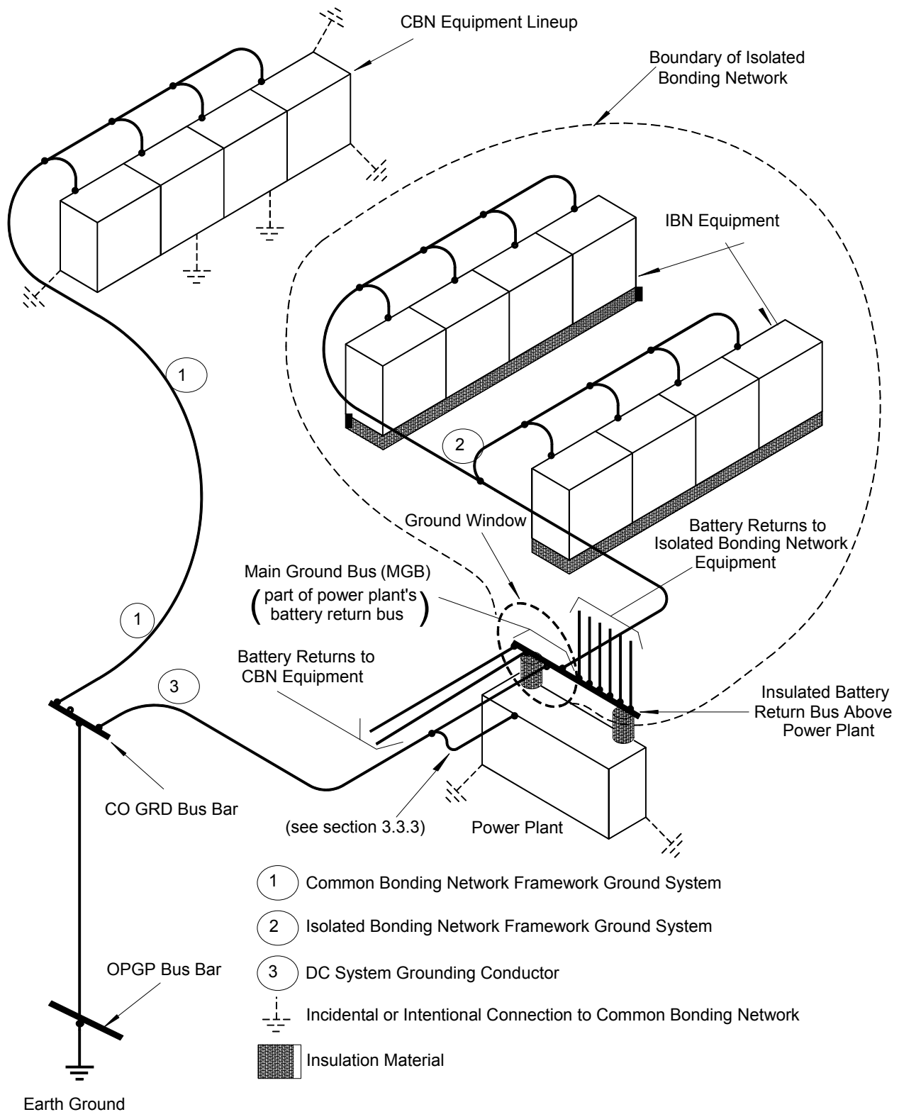
Figure 4-2 Relationship Between Common and Isolated Bonding Networks (MGB is located at power plant)
