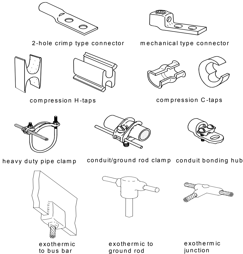
Figure 1-2 Typical Conductor Terminations
