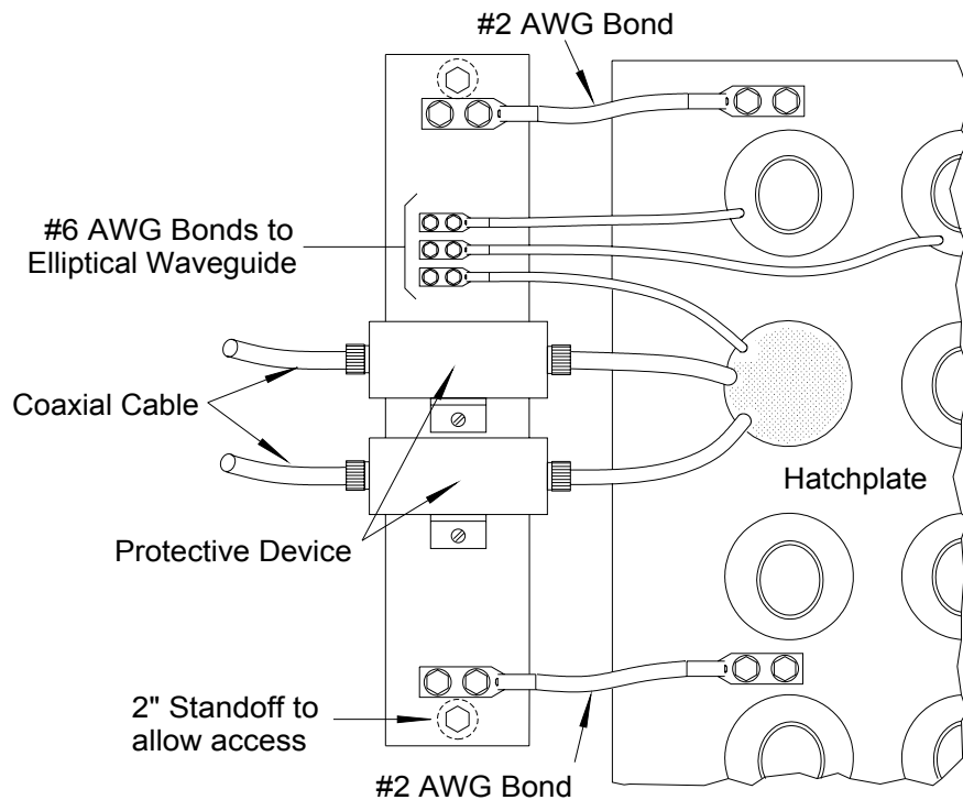
Figure 6-5 Auxiliary Bus Bar Details
