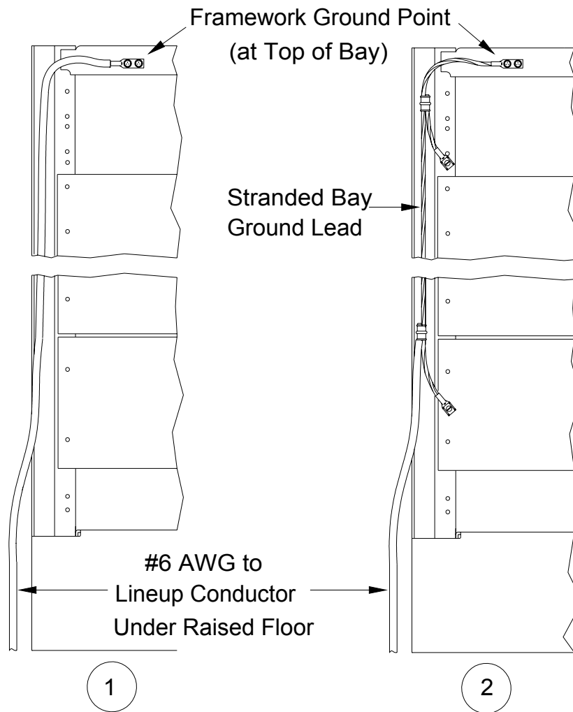
Figure 3-4 Methods of Connecting Between Lineup and Framework Ground
