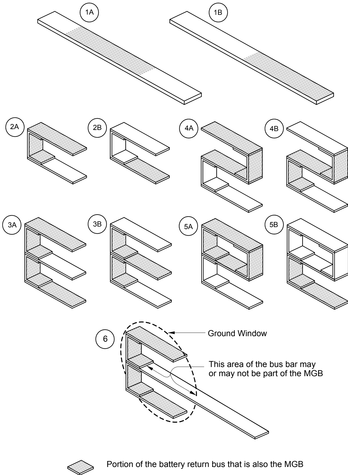
Figure 4-4 Examples of Battery Return Bus Bar/MGB Arrangements
