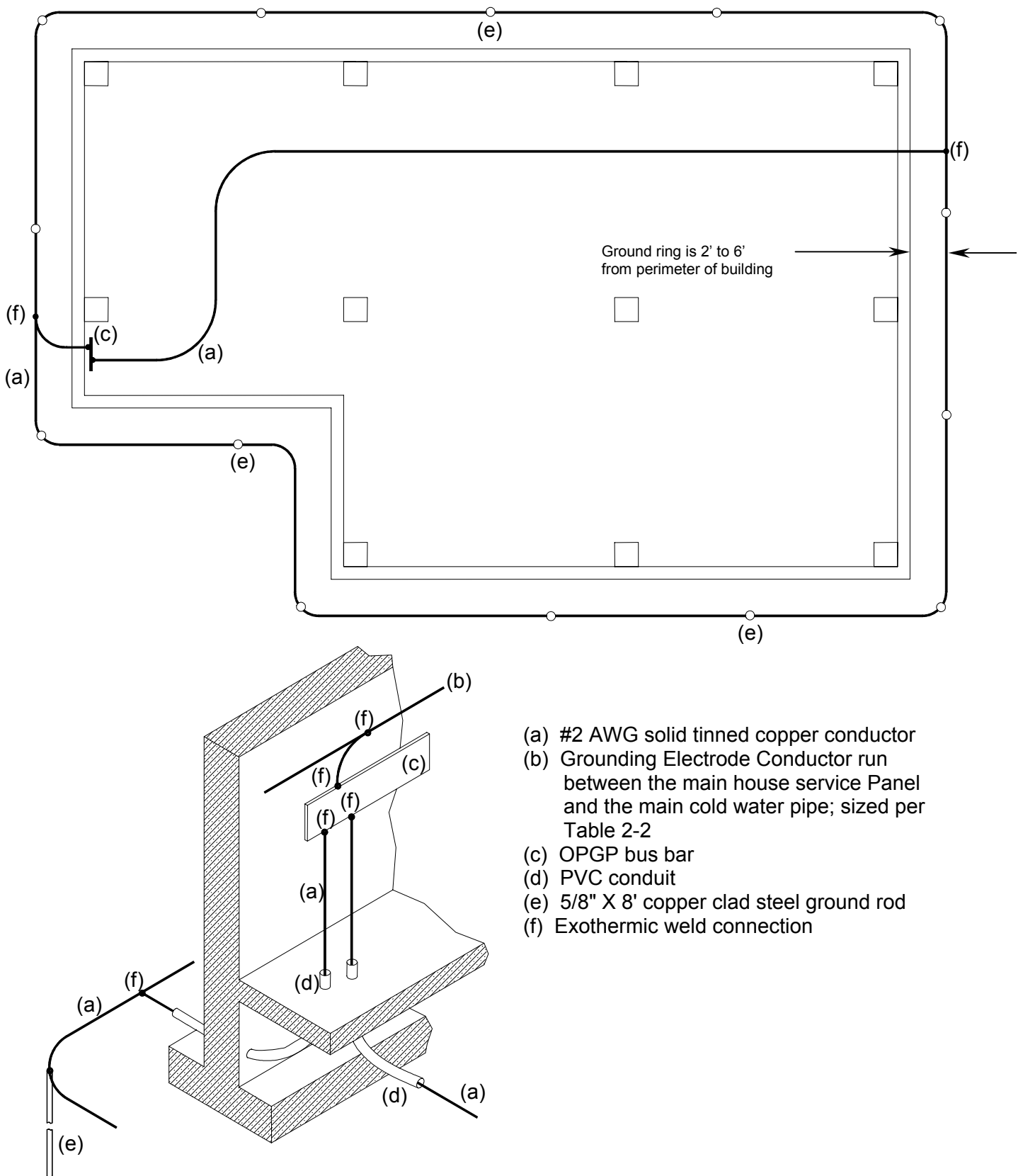
Figure 2-2 Typical Driven Ground System for Buildings Without Basements
