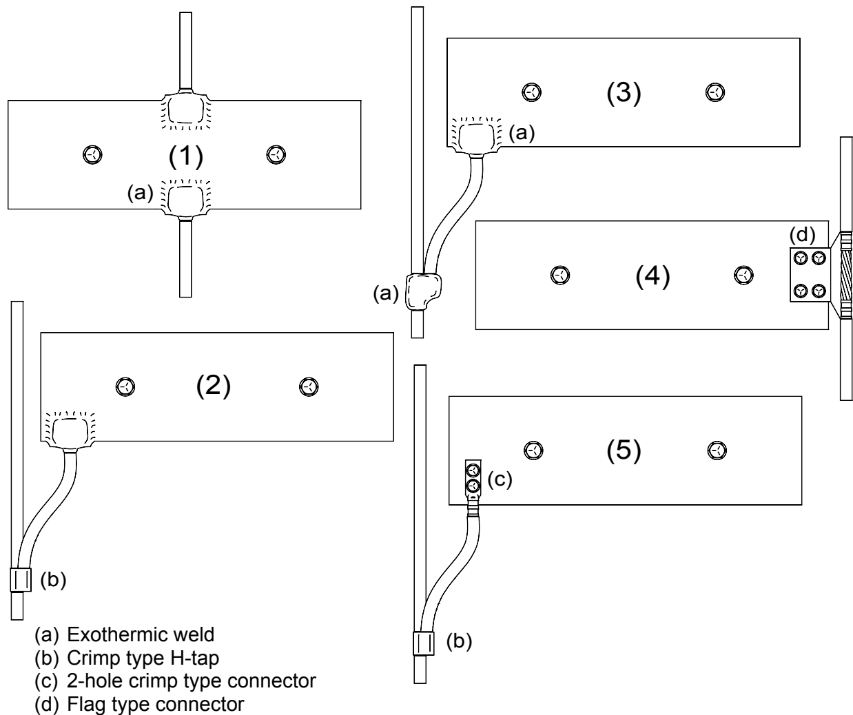
Figure 2-7 Methods of Connecting 750 kcmil Vertical Riser to CO GRD Bus Bar
