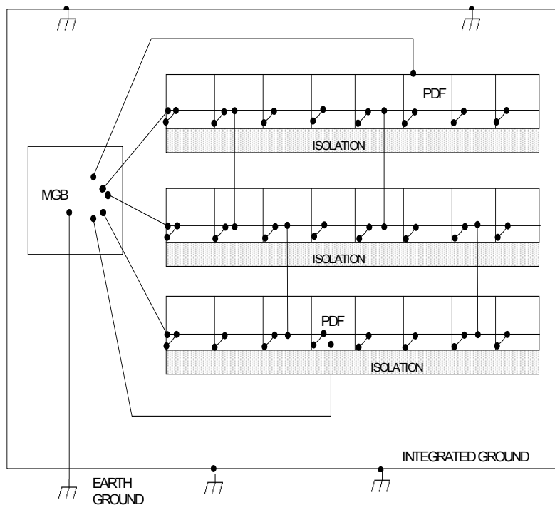
Figure 4-9(a) Lucent 5ESS IBN with Multiple Connections to the MGB
