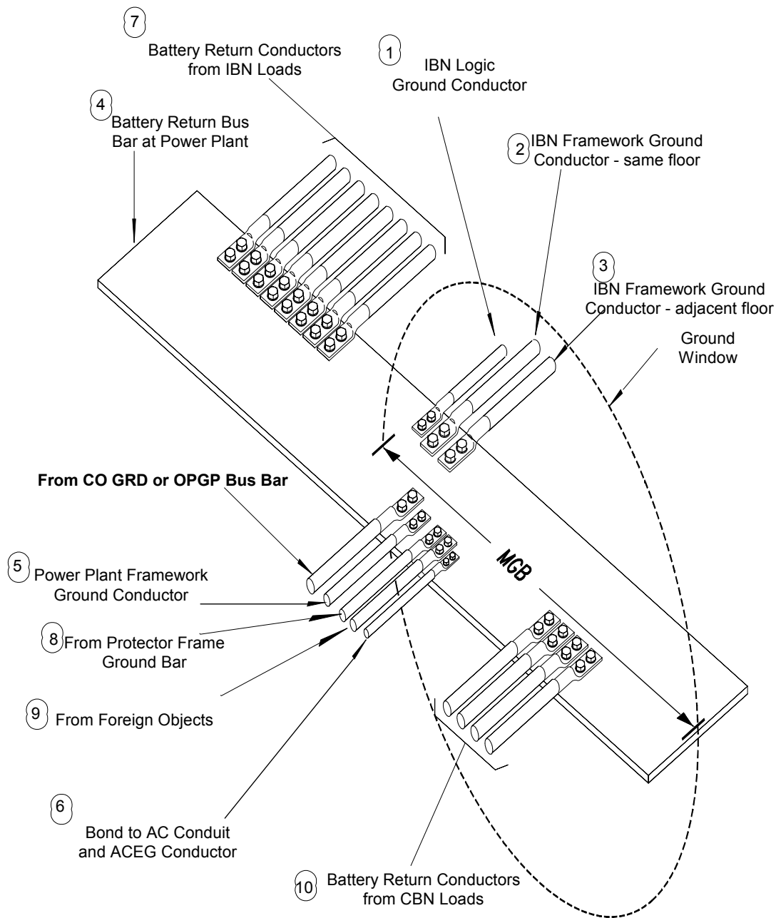
Figure 4-5 Sequencing of Conductors Along an MGB that is Part of a Power Plant's Battery Return Bus
