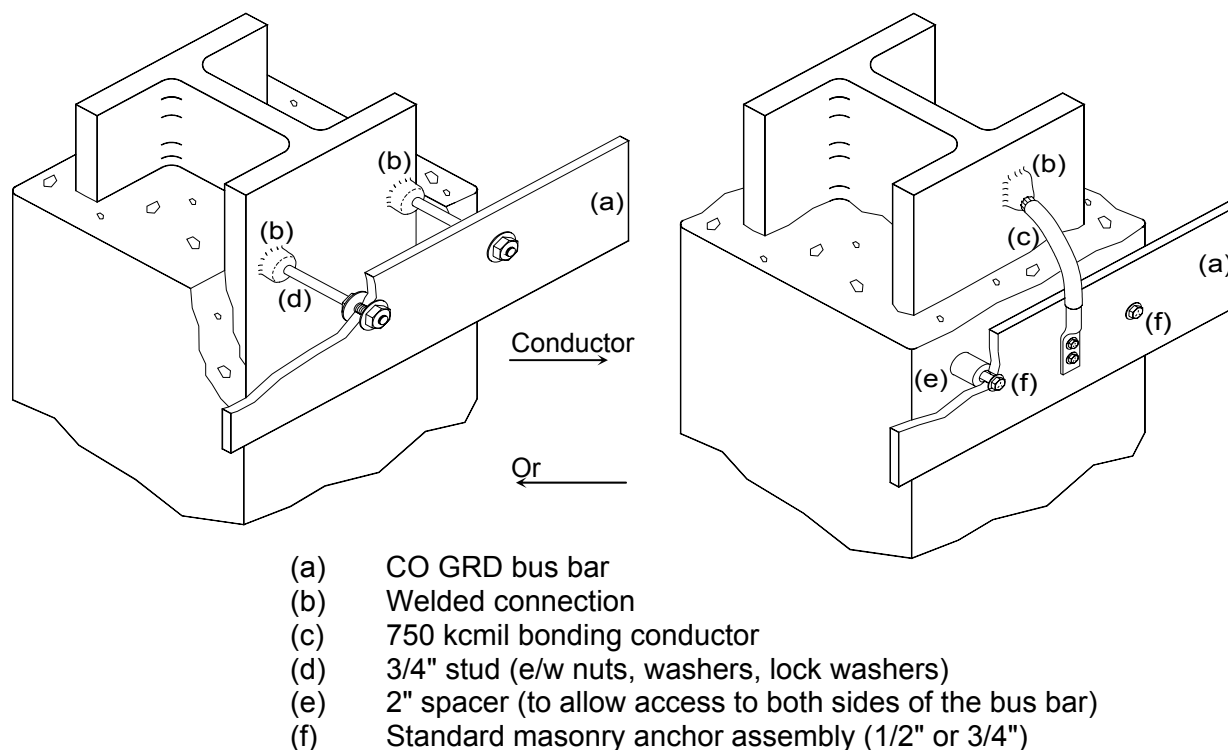
Figure 2-6 Bonding CO GRD Bus Bar to Building Steel
