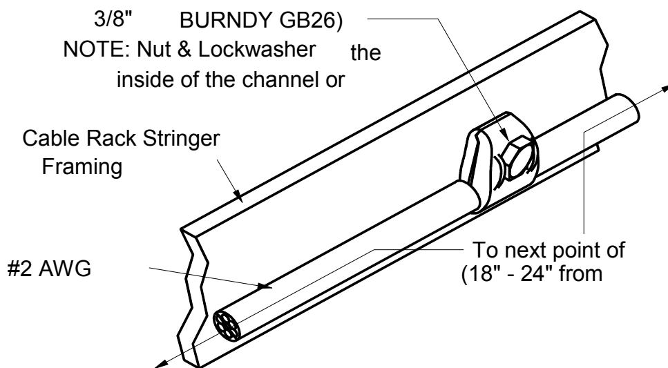
Figure 6-3 Method of Bonding Supplementary Conductor to a Framing Channel
