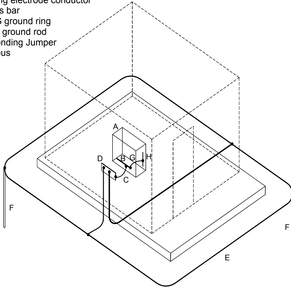
Figure 5-1 Earth Electrode System and AC Service Grounding (hut shown)
