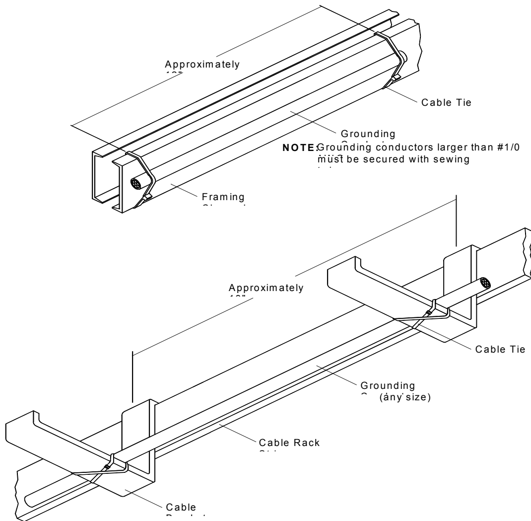
Figure 1-3 Use of Cable Ties to Secure Grounding Conductors
