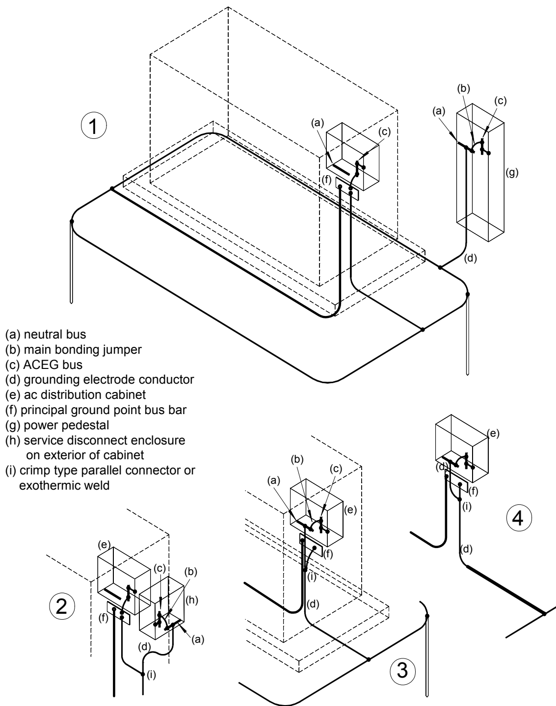
Figure 5-2 Variations of AC Service Grounding (pad-mounted cabinet shown)
