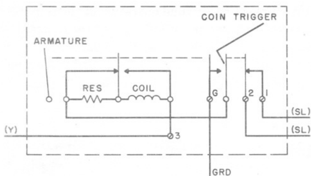
Fig. 10 — P-10E786 Single-coil, Slow-release Coin Relay
