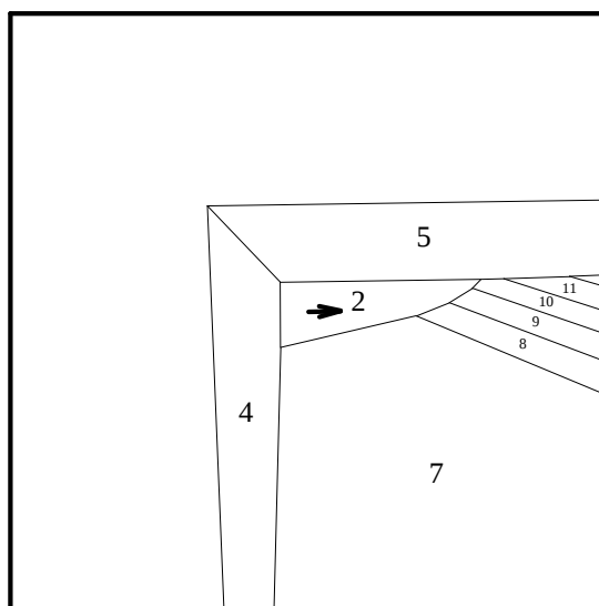
Fig. 103: pr. proj. it. 6, v = \text{center} + (.1, 0, 0)
