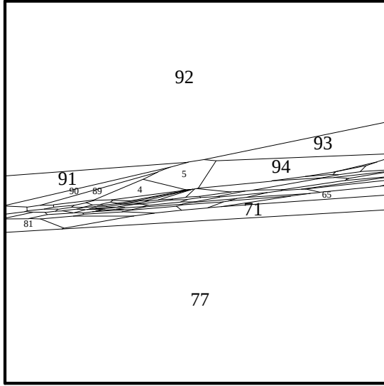
Fig. 72: dual proj. it. 14, v = \text{center}
