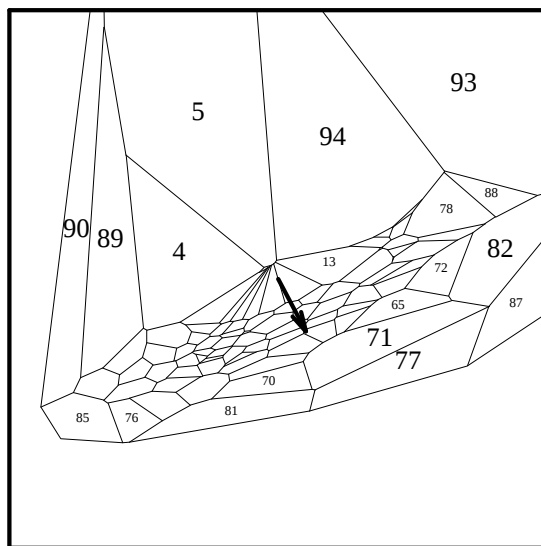
Fig. 57: dual proj. it. 6, v = \text{center} + (.2, 0, 0)
