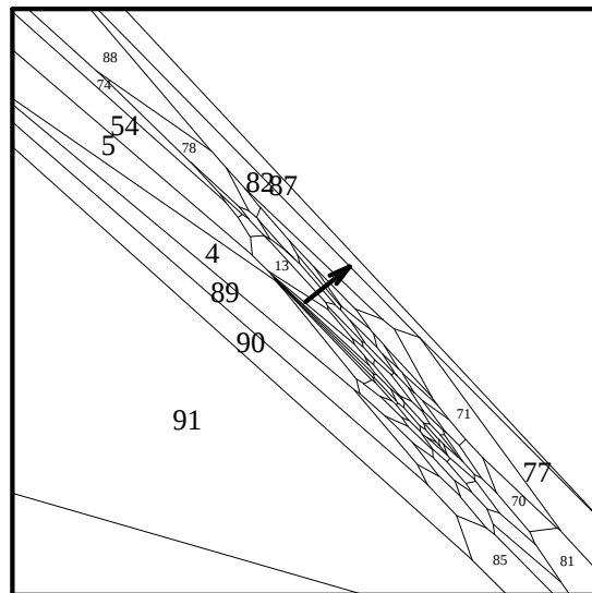
Fig. 121: pr. proj. it. 15, v = \text{center} + (.1, 0, 0)
