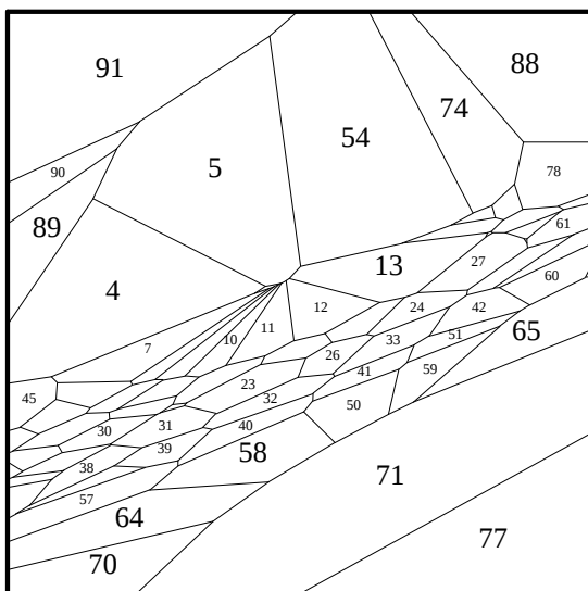
Fig. 128: pr. proj. it. 19, v = \text{center}
