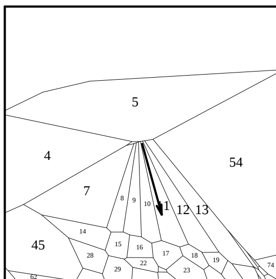
Fig. 111: pr. proj. it. 10, v = \text{center} + (.1, 0, 0)
