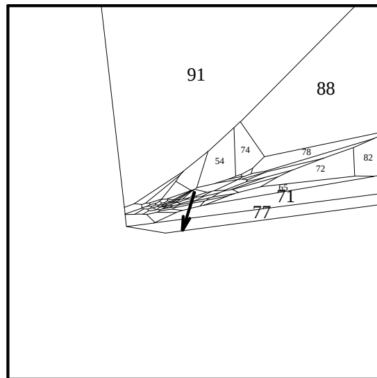
Fig. 133: pr. proj. it. 21, v = \text{center} + (.1, 0, 0)
