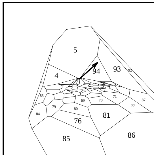
Fig. 51: dual proj. it. 3, v = \text{center} + (.2, 0, 0)
