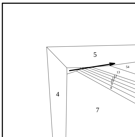
Fig. 105: pr. proj. it. 7, v = \text{center} + (.1, 0, 0)
