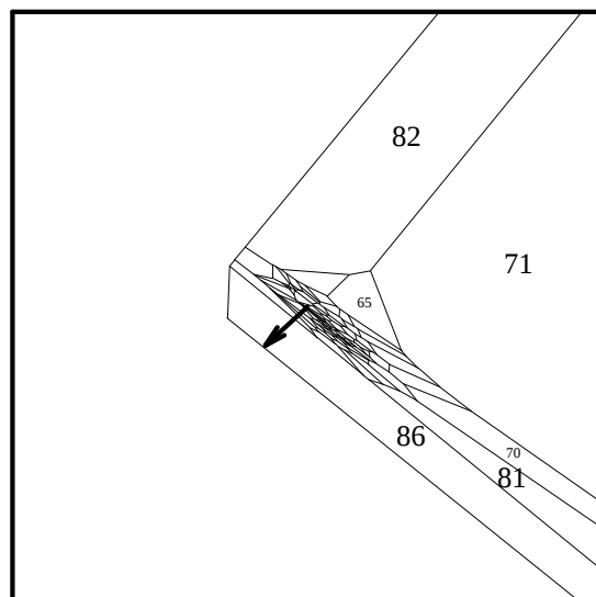
Fig. 135: pr. proj. it. 22, v = \text{center} + (.1, 0, 0)
