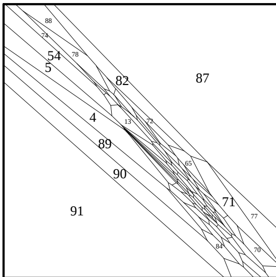
Fig. 120: pr. proj. it. 15, v = \text{center}
