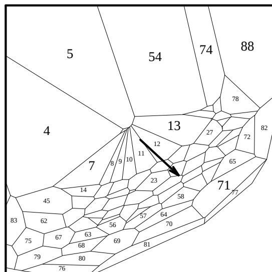
Fig. 117: pr. proj. it. 13, v = \text{center} + (.1, 0, 0)
