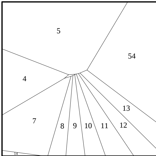
Fig. 112: pr. proj. it. 11, v = \text{center}
