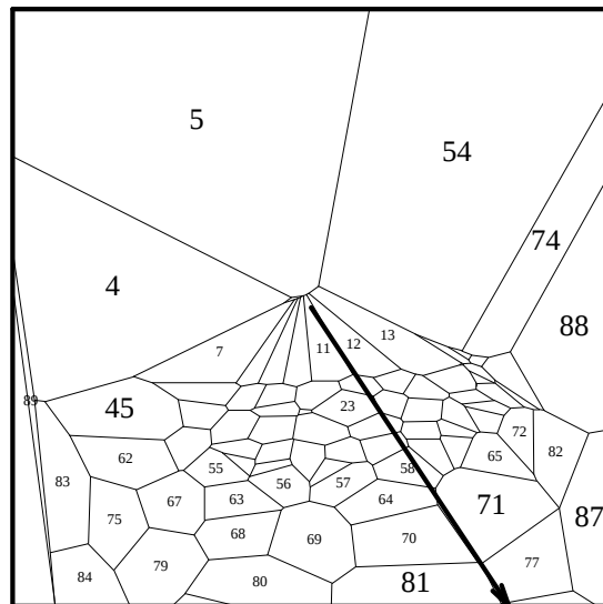
Fig. 115: pr. proj. it. 12, v = \text{center} + (.1, 0, 0)
