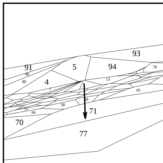
Fig. 65: dual proj. it. 10, v = \text{center} + (.2, 0, 0)
