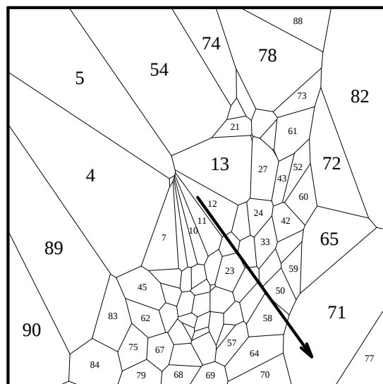
Fig. 123: pr. proj. it. 16, v = \text{center} + (.1, 0, 0)
