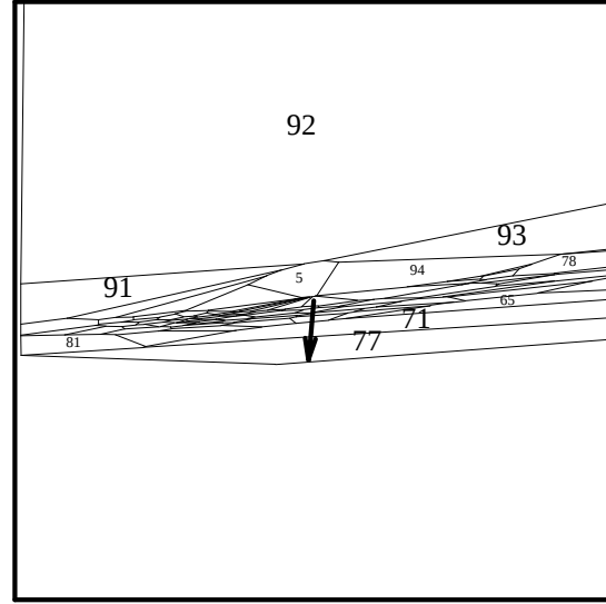
Fig. 73: dual proj. it. 14, v = \text{center} + (.2, 0, 0)
