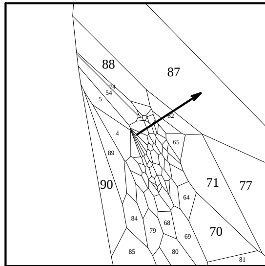
Fig. 119: pr. proj. it. 14, v = \text{center} + (.1, 0, 0)
