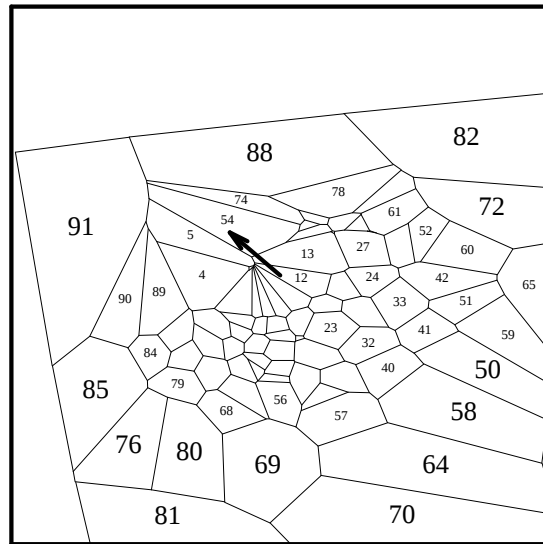
Fig. 131: pr. proj. it. 20, v = \text{center} + (.1, 0, 0)
