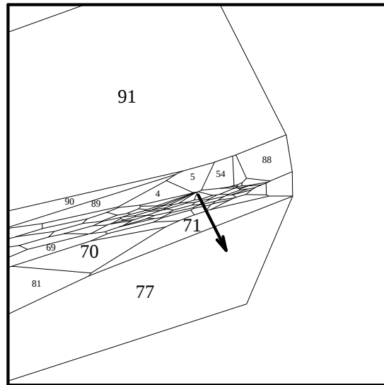
Fig. 125: pr. proj. it. 17, v = \text{center} + (.1, 0, 0)
