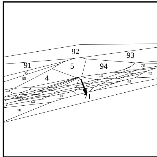
Fig. 67: dual proj. it. 11, v = \text{center} + (.2, 0, 0)
