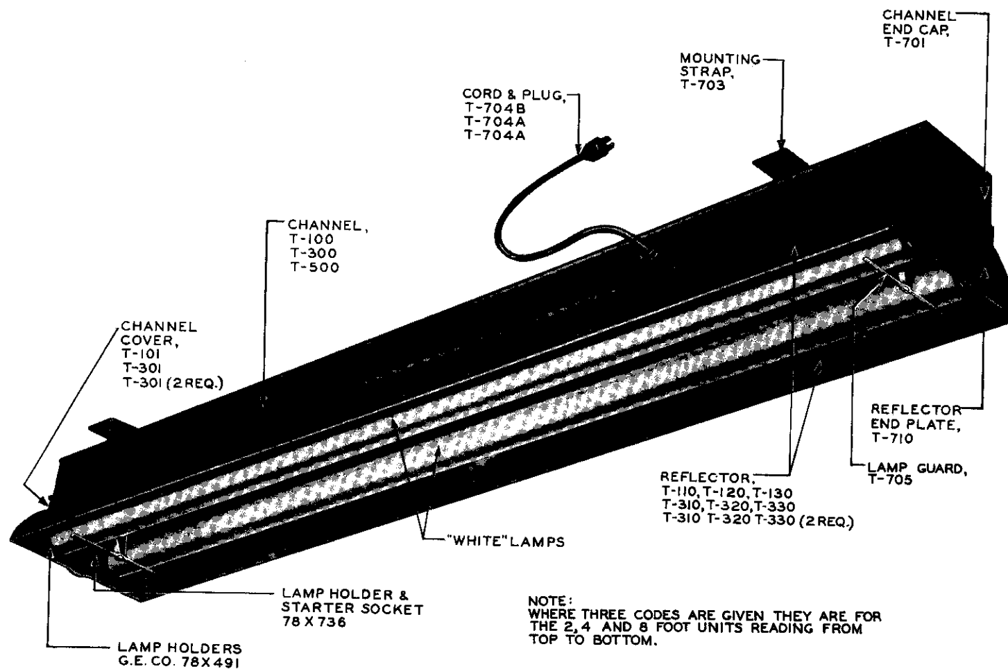
Fig. 2 - Assembly
