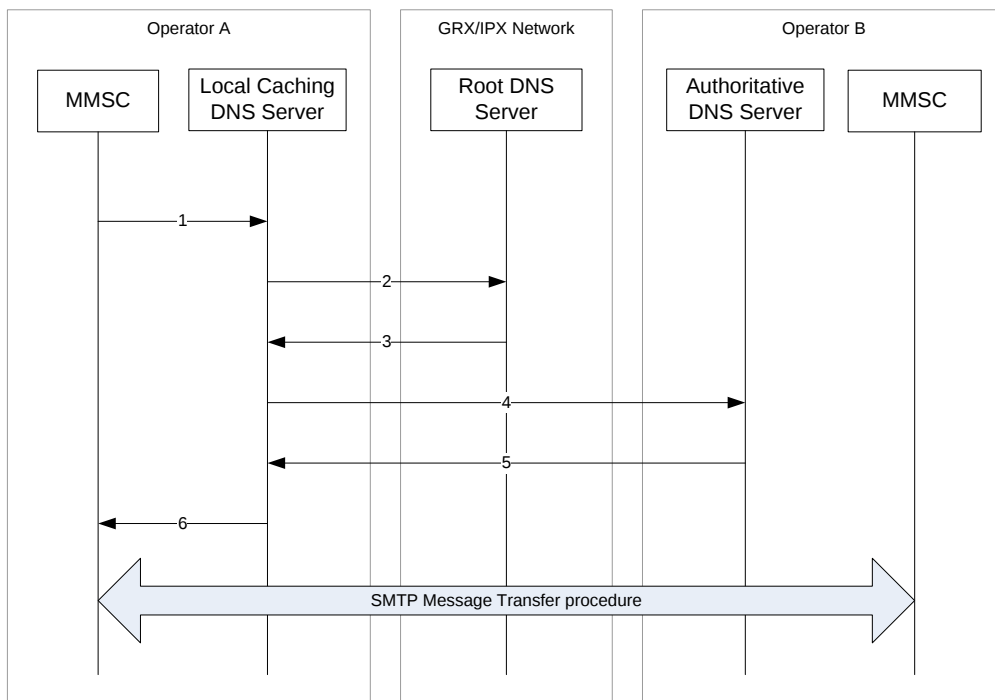
Figure 9: MMS Direct Inter-network Delivery
