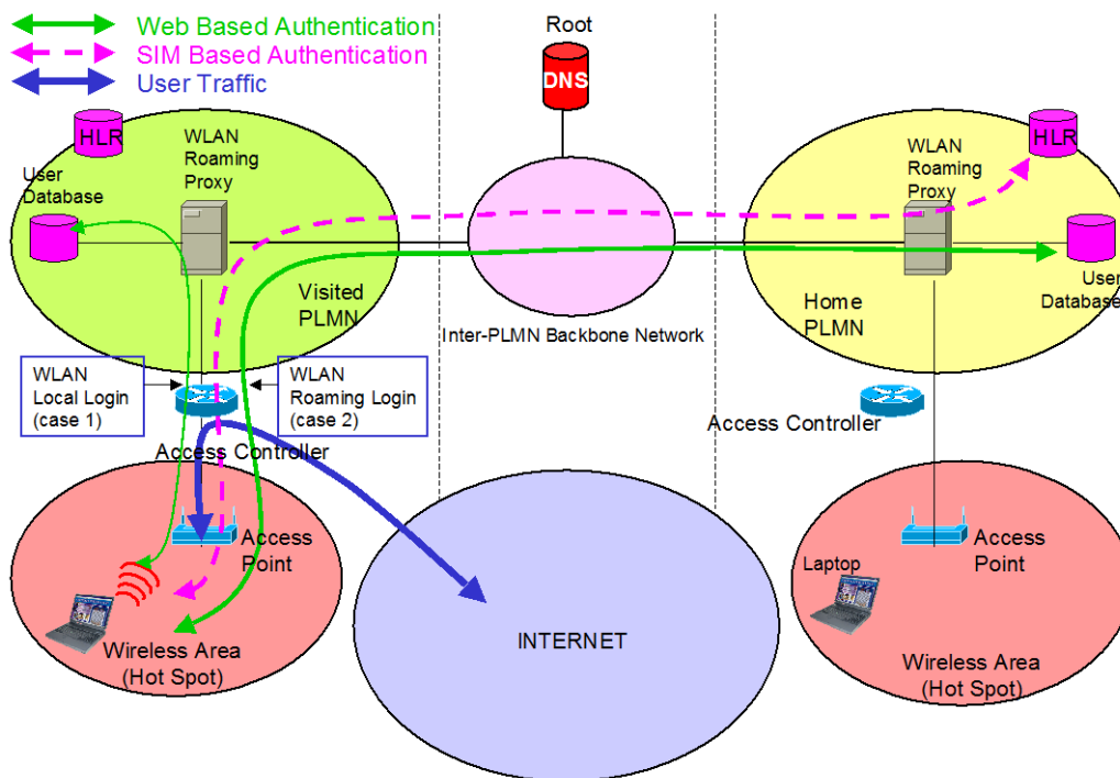
Figure 11: WLAN user authentication mechanism
