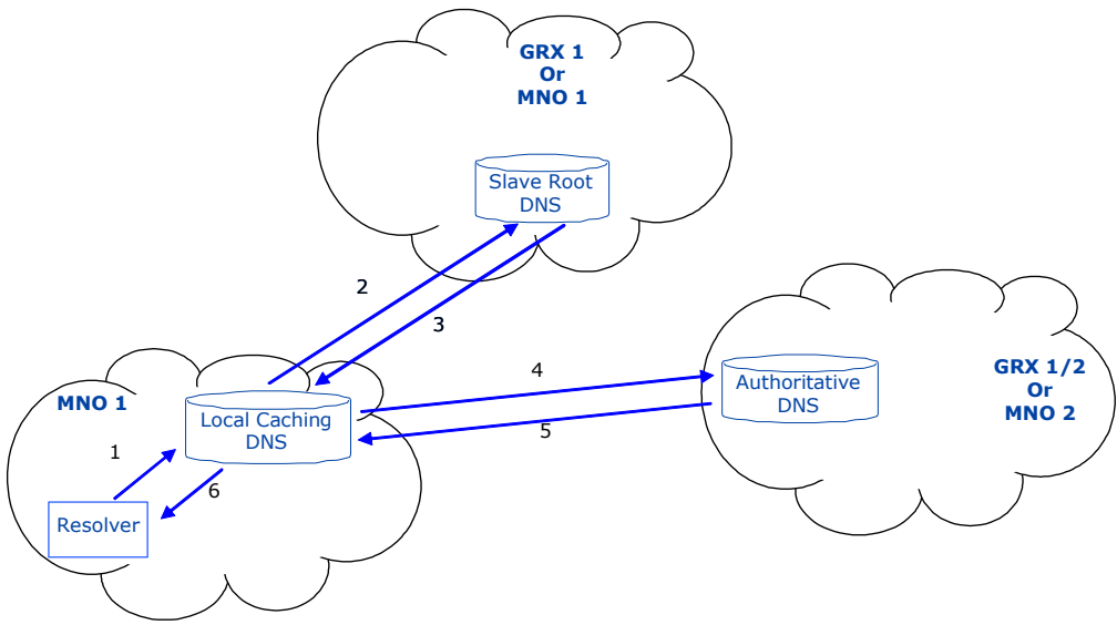
Figure 3: Resolver Architecture
