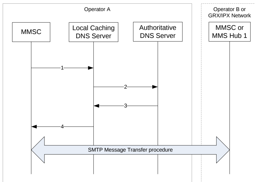
Figure 10: MMS Inter-operator Delivery
