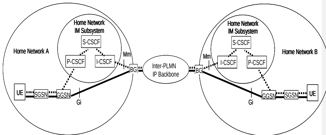
Figure 12: IMS Session Inter-working
