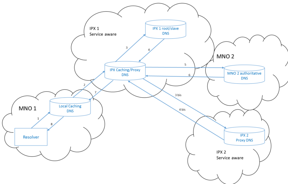
Figure 5 Service aware network resolver architecture
