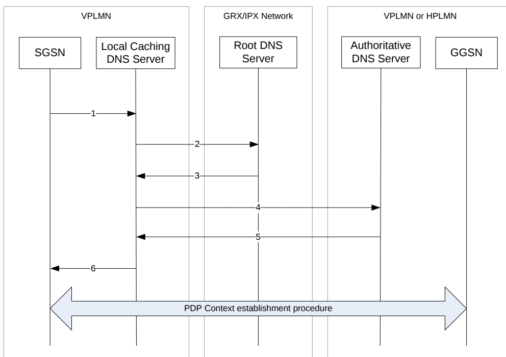
Figure 7: DNS message flow for PDP Context activations
